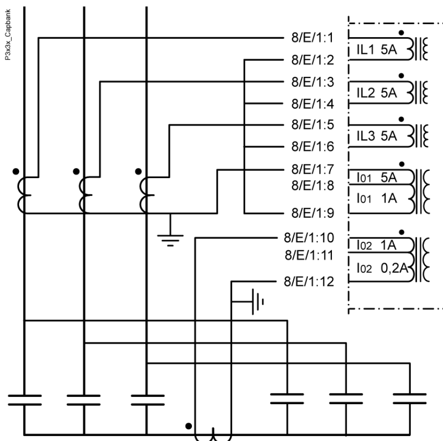
Figure 6.45: Typical capacitor bank protection application with Easergy P3 relays
