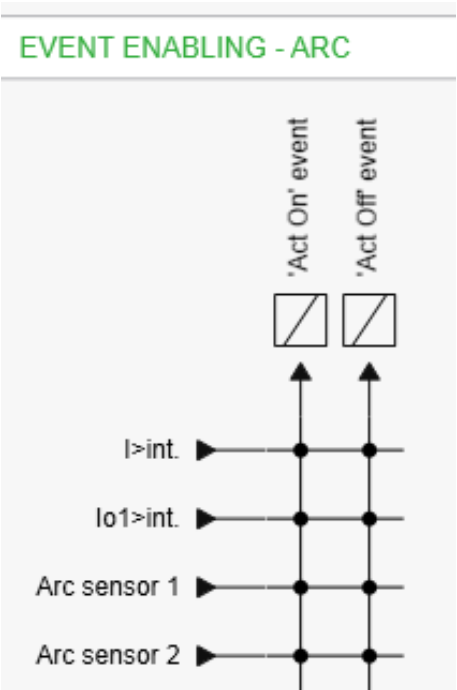
Figure 6.86: Example view of Arc event enabling
