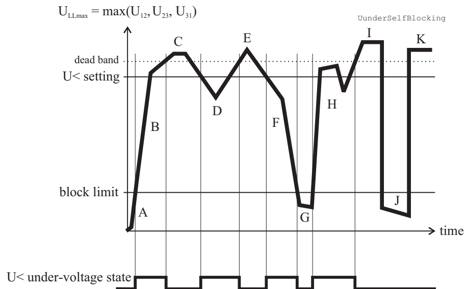
Figure 6.30: Under voltage state and block limit
