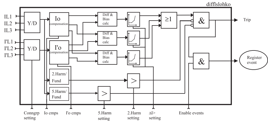
Figure 6.78: Block diagram of the differential overcurrent stage \Delta I >
