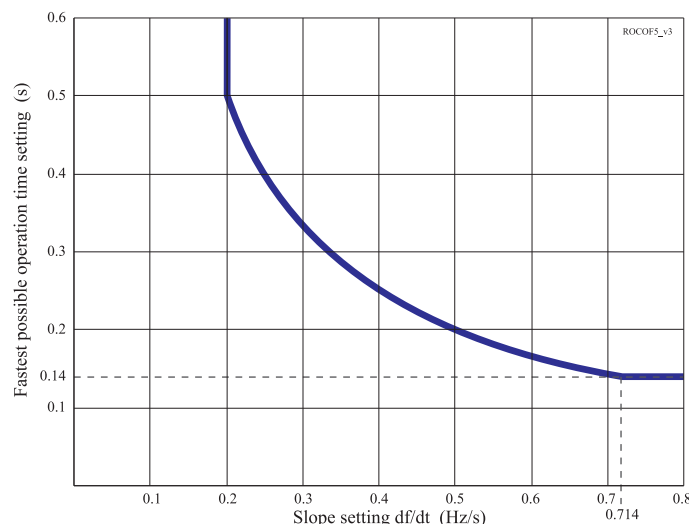
Figure 6.71: At very sensitive slope settings the fastest possible operate time is limited.
