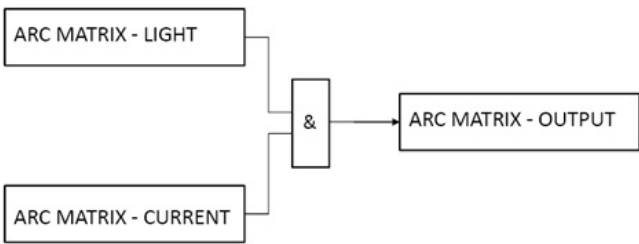
Figure 6.85: Matrix correlation principle with the logical AND operator
