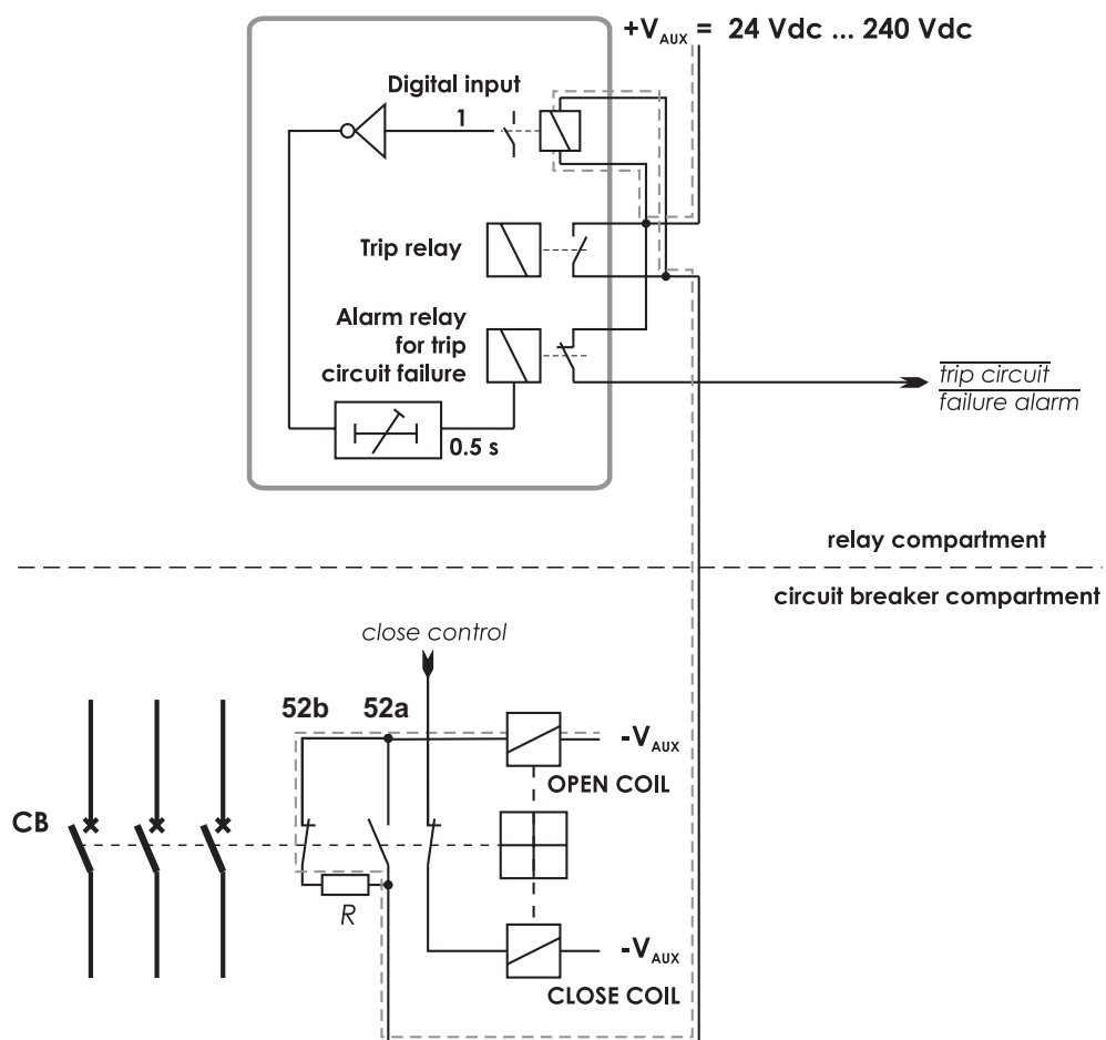
Figure 7.14: Trip circuit supervision using a single digital input when the circuit breaker is in open position.
