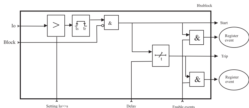
Figure 6.44: Block diagram of the earth fault stages overcurrent I_0 >> , I_0 >>> , I_0 >>>>
