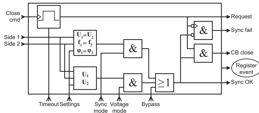
Figure 6.27: Synchrocheck function
