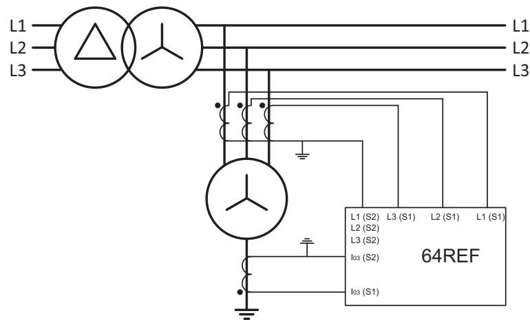
Figure 6.57: Restricted earth fault protection of a shunt reactor
