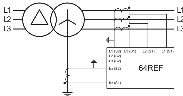
Figure 6.55: Restricted earth fault protection of a solidly-earthed transformer
