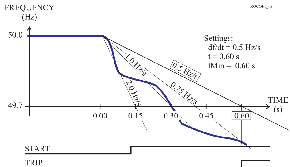
Figure 6.70: An example of definite time df/dt operate time. At 0.6 s, which is the delay setting, the average slope exceeds the setting 0.5 Hz/s and a trip signal is generated.
