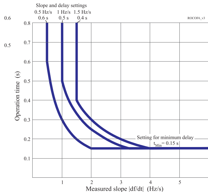
Figure 6.72: Three examples of possible dependent df/dt operate time characteristics. The slope and operation delay settings define the knee points on the left. A common setting for t_{\text{Min}} has been used in these three examples. This minimum delay parameter defines the knee point positions on the right.
