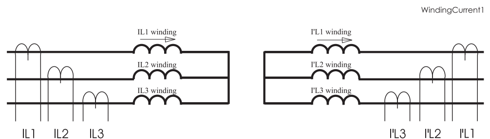
Figure 6.76: Winding currents in connection group Yy0
