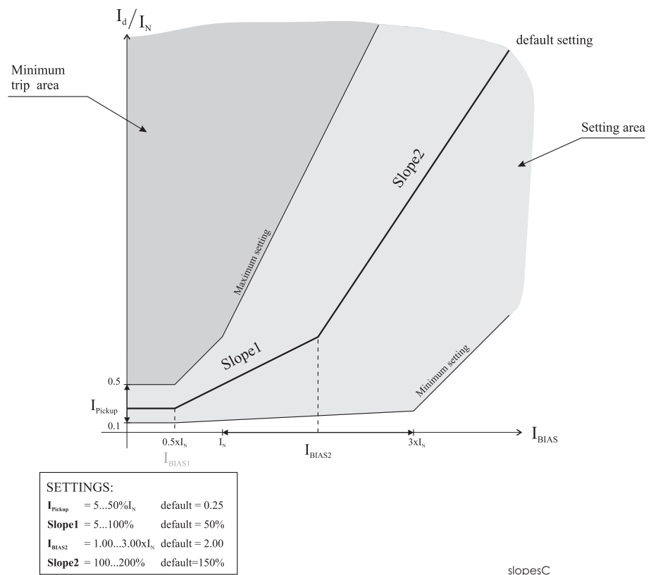
Figure 6.79: Example of differential overcurrent characteristics
