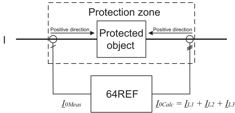
Figure 6.59: Differential protection principle applied to REF protection
