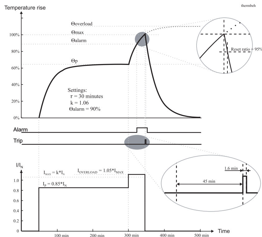
Figure 6.33: Example of the thermal model behaviour.
