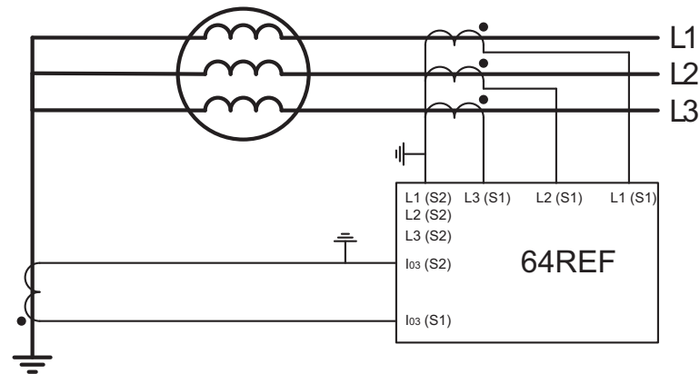
Figure 6.58: Restricted earth fault protection of a rotating machine
