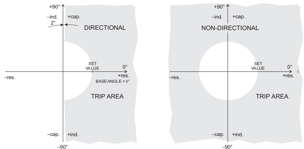
Figure 6.64: Difference between directional mode and non-directional mode. The grey area is the trip region.
