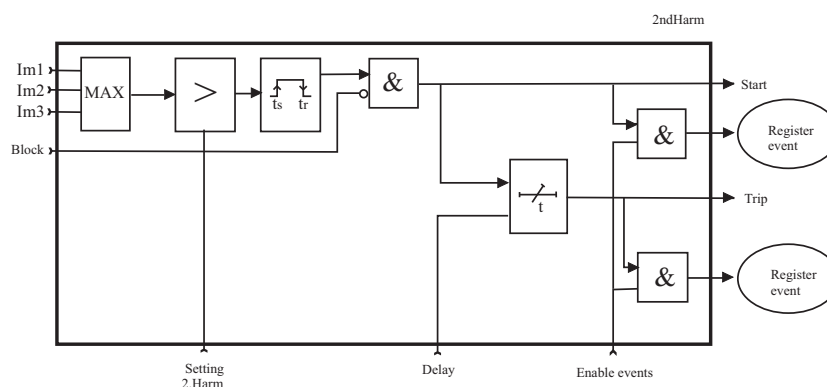
Figure 6.69: Block diagram of the magnetishing inrush detection stage
