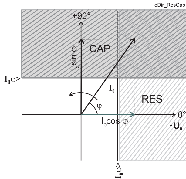
Figure 6.67: Operation characteristic of the directional earth fault protection in Res or Cap mode. Res mode can be used with compensated networks and Cap mode is used with unearthed networks.
