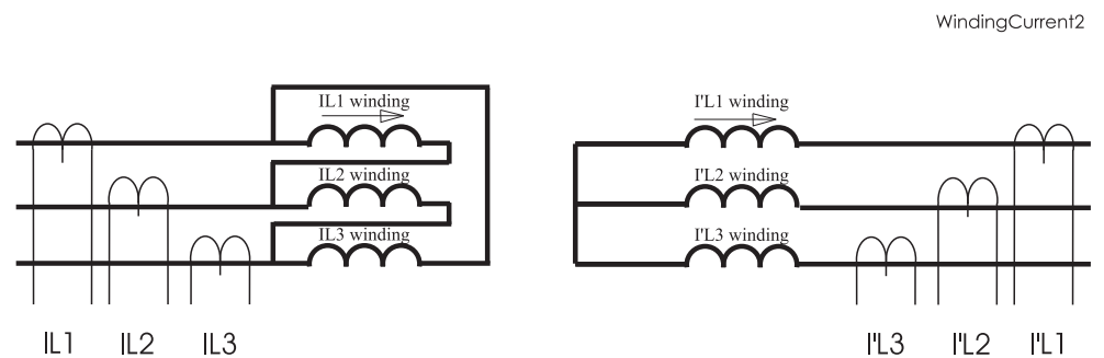
Figure 6.77: Winding currents in connection group Dy11
