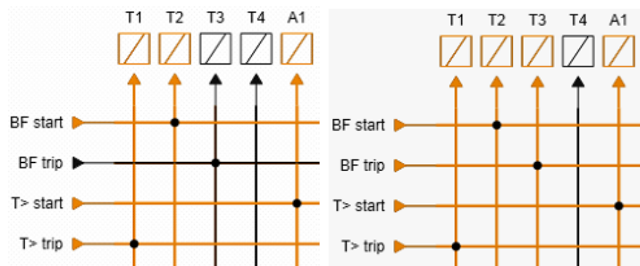
Figure 6.36: Both the trip and CBFP start signals activate simultaneously (left picture). If T> trip fails to control the CB through T1, the CBFP activates T3 after the breaker failure operate time.
