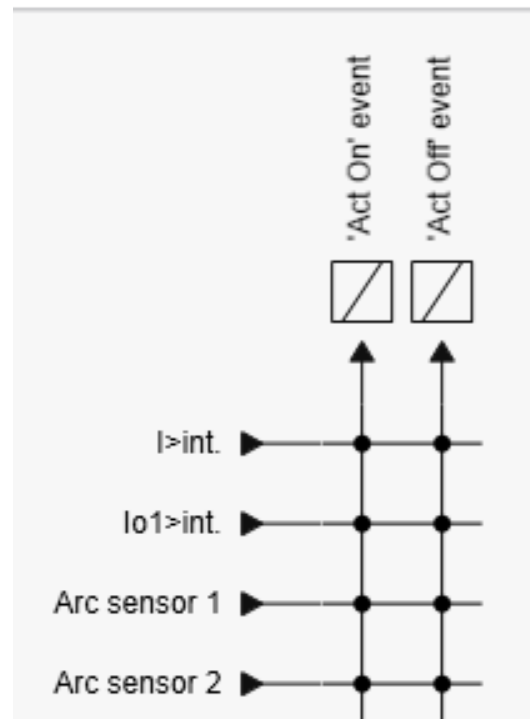
Figure 6.92: Configuring the arc events – an example
