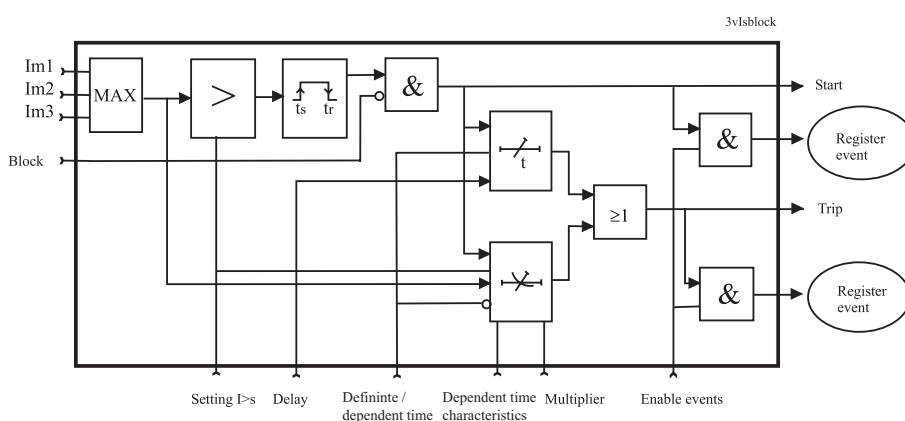
Figure 6.34: Block diagram of the three-phase overcurrent stage I>
