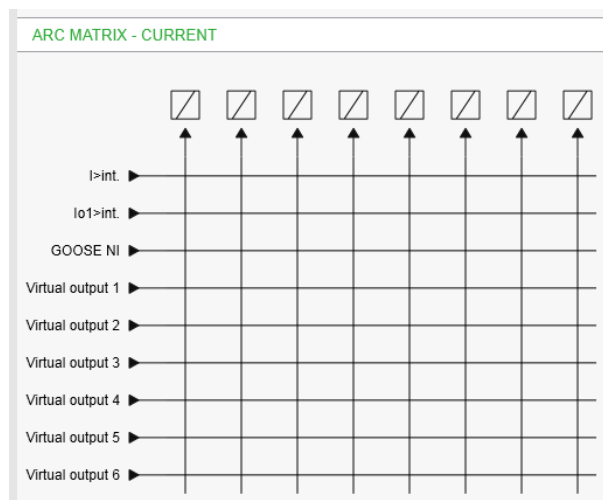
Figure 6.82: Example view of Arc matrix – current
