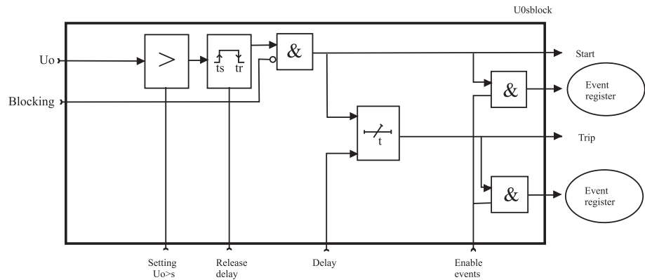
Figure 6.54: Block diagram of the neutral voltage displacement stages U_0> , U_0>>
