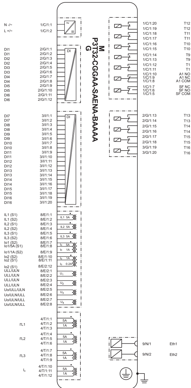
Figure 10.13: Typical block diagram for P3M32, P3T32 and P3G32 relays
