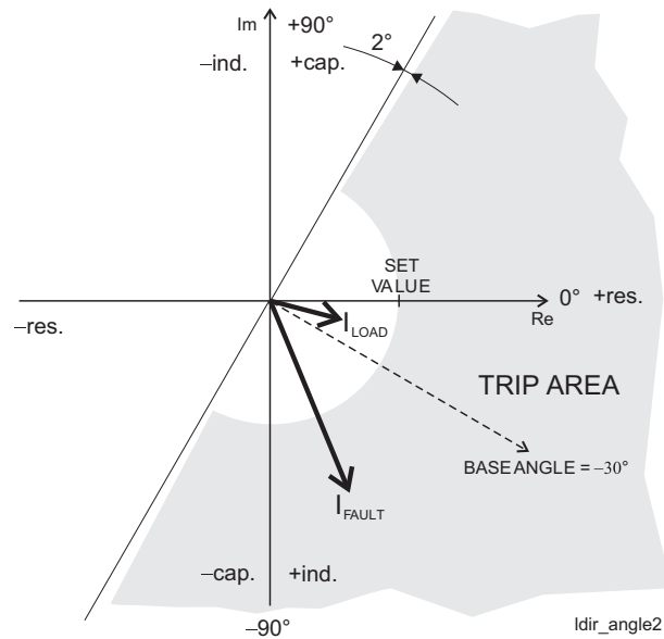
Figure 6.63: Example of the directional overcurrent function's protection area
