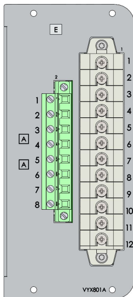
Figure 10.15: Example of Terminal 8/E/1 and 8/E/2
