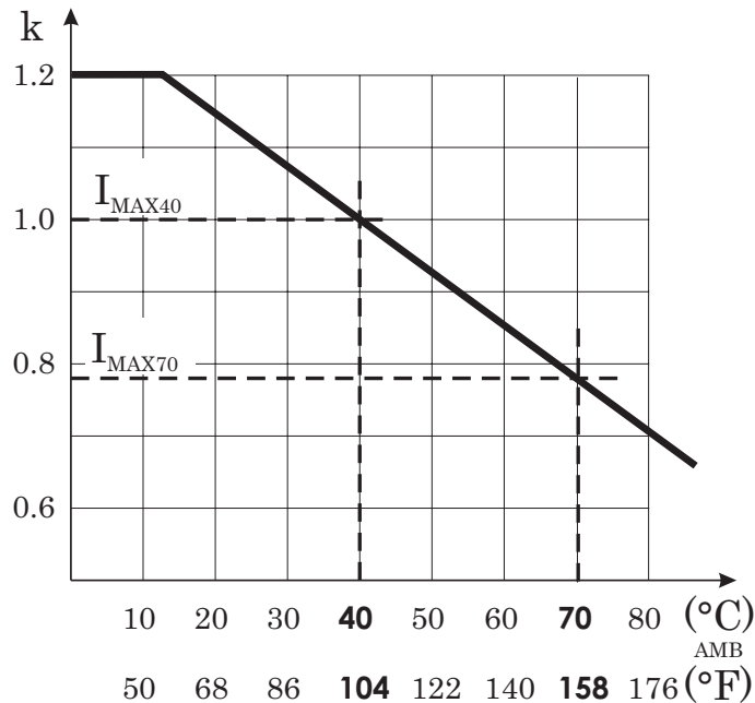
Figure 6.32: Ambient temperature correction of the overload stage T >
