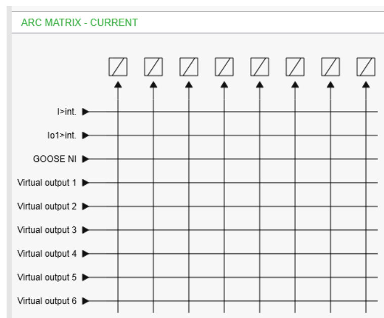
Figure 6.89: Configuring the current matrix – an example
