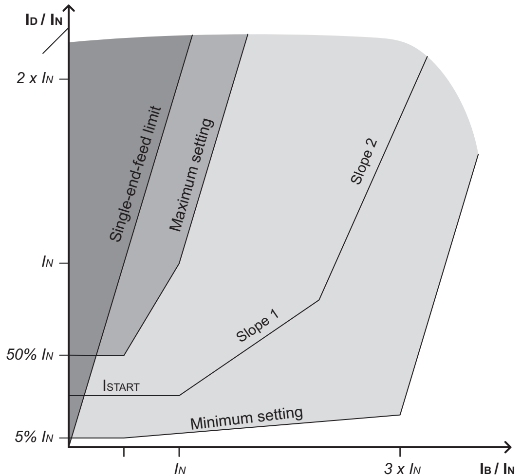
Figure 6.61: Restricted earth fault protection operating characteristics
