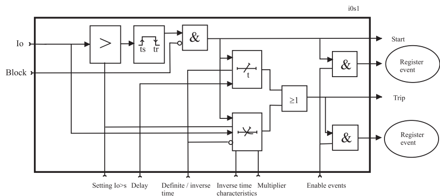
Figure 6.43: Block diagram of the earth fault stage overcurrent I_0 >
