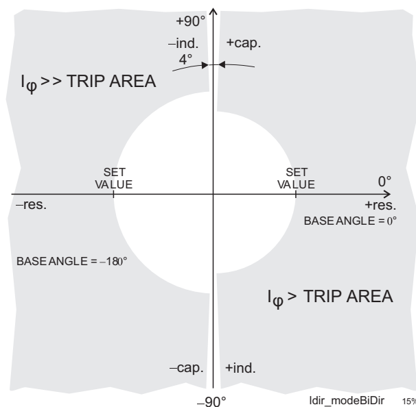
Figure 6.65: Bi-directional application with two stages I_{\phi}> and I_{\phi}>> .
