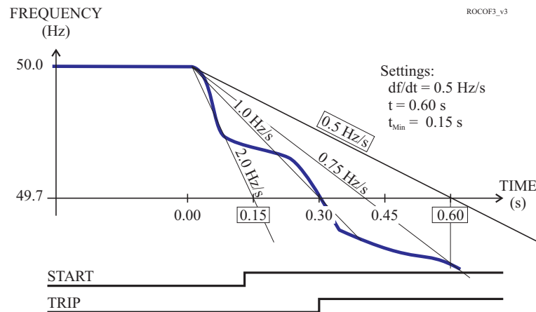
Figure 6.73: An example of dependent df/dt operate time. The time to trip will be 0.3 s, although the setting is 0.6 s, because the average slope 1 Hz/s is steeper than the setting value 0.5 Hz/s.
