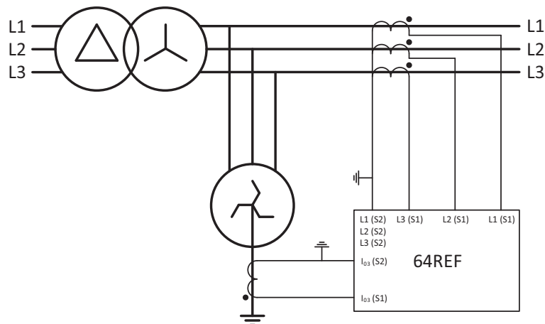
Figure 6.56: Restricted earth fault protection of a transformer and neutral point reactor
