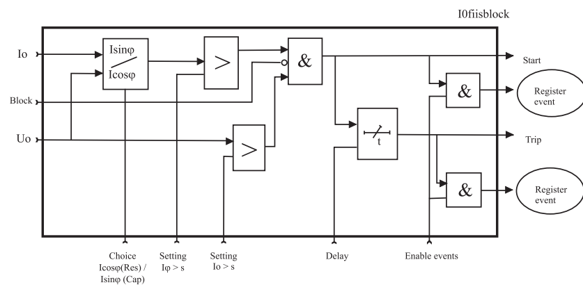
Figure 6.66: Block diagram of the directional earth fault overcurrent stages I_{0\phi} > , I_{0\phi} >>
