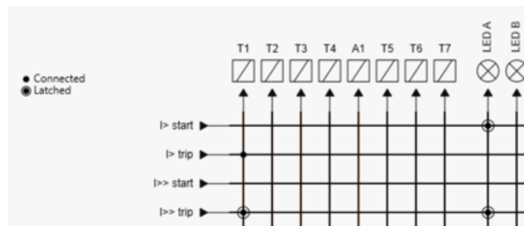
Figure 6.74: The lockout programmed for LED A and I>> trip signals. The latched signal is identified with a dot and circle in the matrix signal line crossing.
