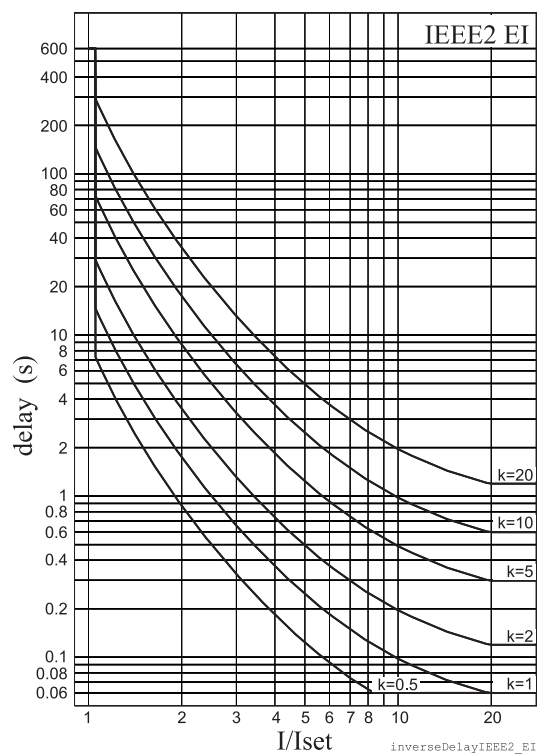
Figure 6.23: IEEE2 extremely inverse delay
