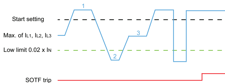
Figure 6.42: Switch-onto-fault function operates when the CB has detected open and the fault current reaches start setting value.
