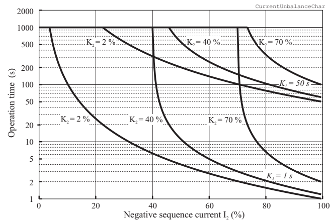
Figure 6.31: Dependent operation delay of negative sequence overcurrent I_2> (ANSI 46). The longest delay is limited to 1000 seconds (=16min 40s).
