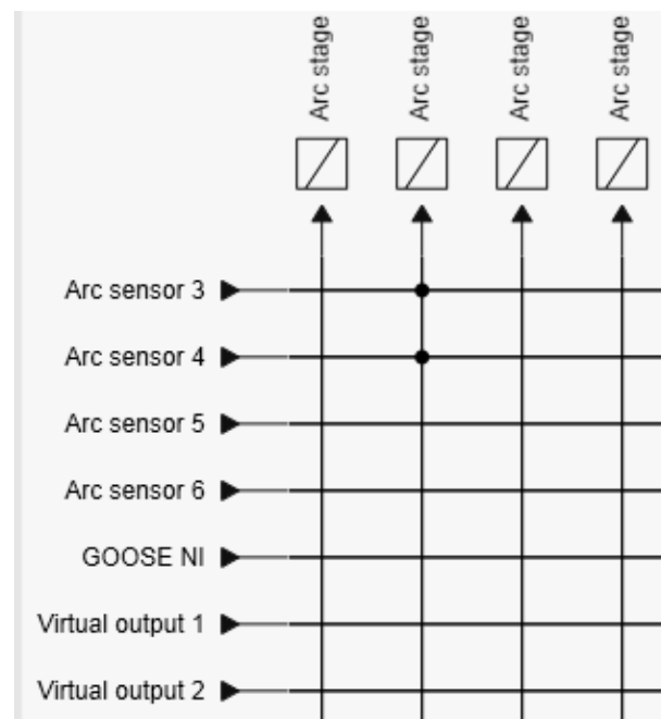
Figure 6.90: Configuring the light arc matrix
