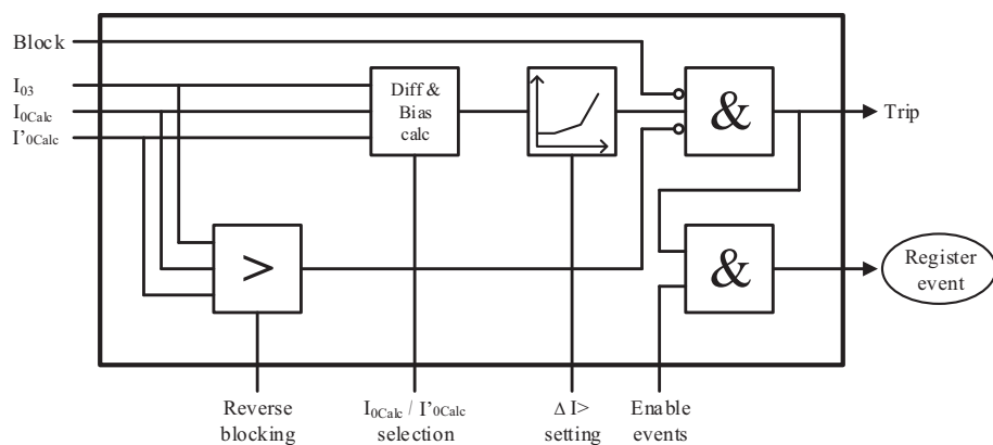
Figure 6.62: Block diagram of REF protection stage
