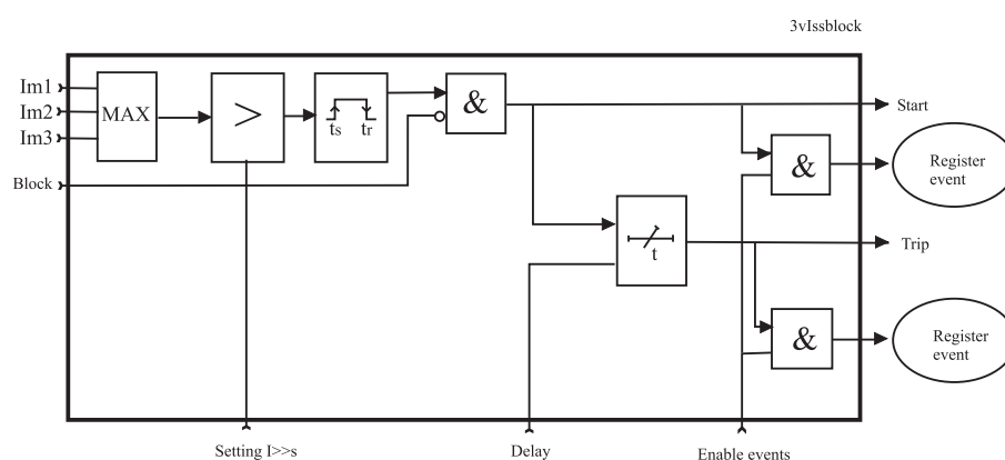
Figure 6.35: Block diagram of the three-phase overcurrent stage I>> and I>>>
