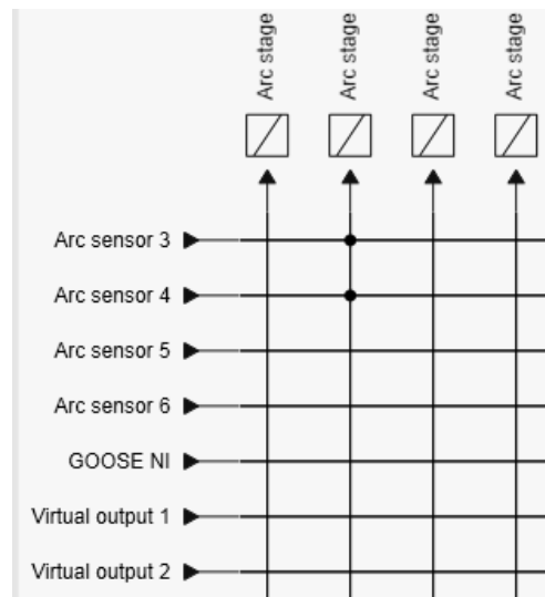
Figure 6.83: Example view of Arc matrix – light
