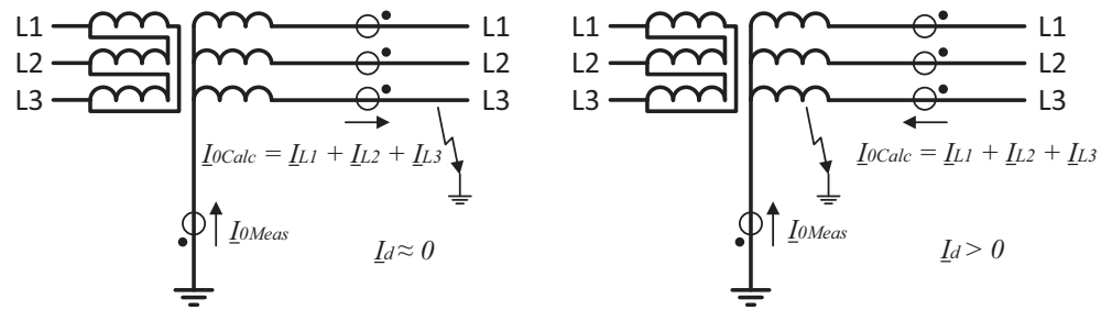
Figure 6.60: Through-fault condition (left) and earth fault in protected zone (right)
