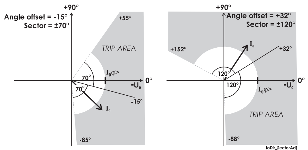
Figure 6.68: Two example of operation characteristics of the directional earth fault stages in sector mode. The drawn I_0 phasor in both figures is inside the trip area. The angle offset and half sector size are user's parameters.
