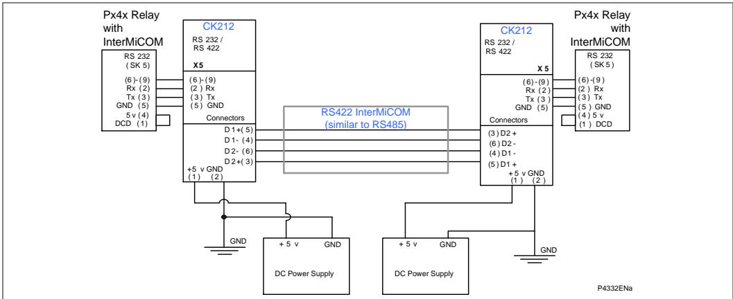
Figure 96 - MODEM InterMiCOM teleprotection via a RS422 protocol
