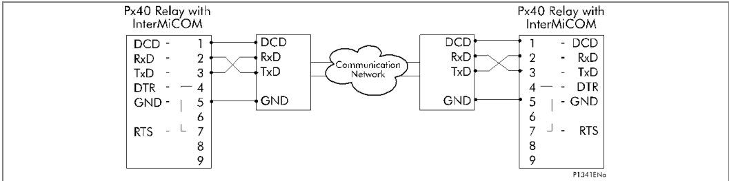
Figure 95 - InterMiCOM teleprotection via a MODEM link
