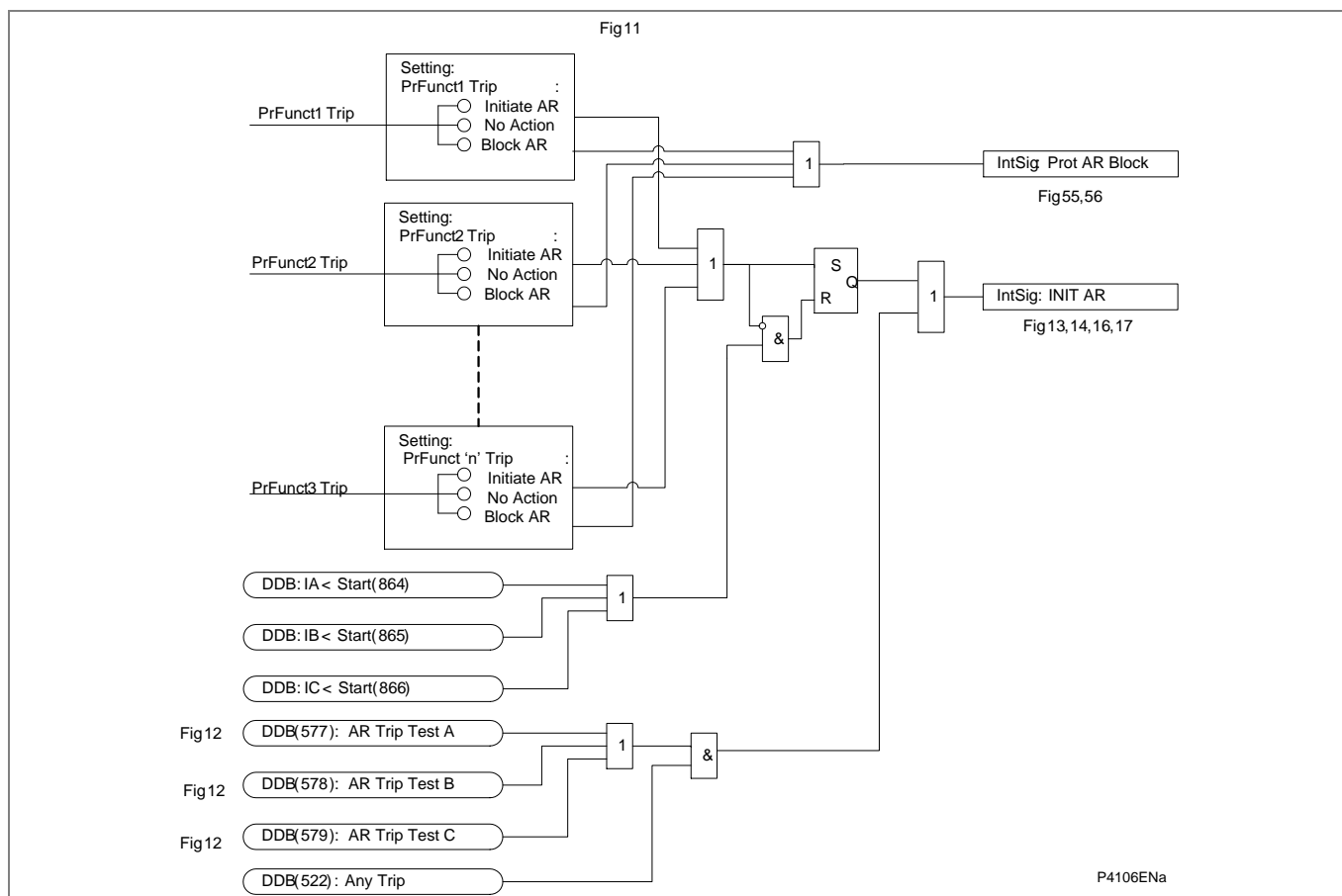
Figure AR-12 - Auto-reclose initiation
