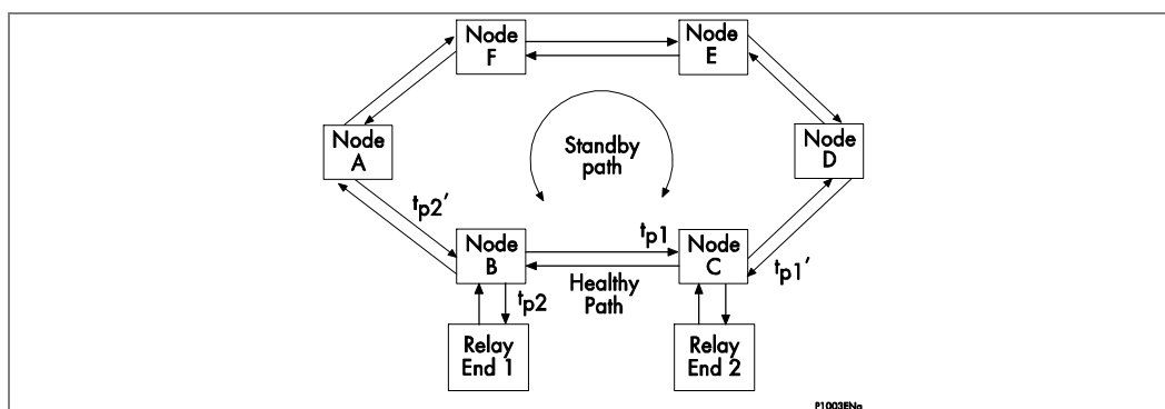
Figure 4 - Example of switched synchronous digital hierarchy
