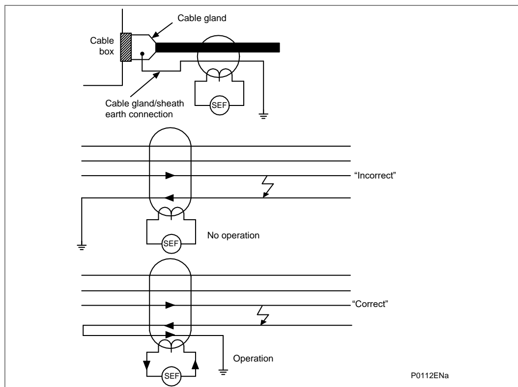
Figure 20 - Positioning of core balance current transformers
