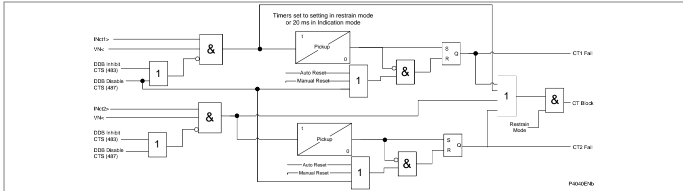
Figure 104 - Standard CTS
