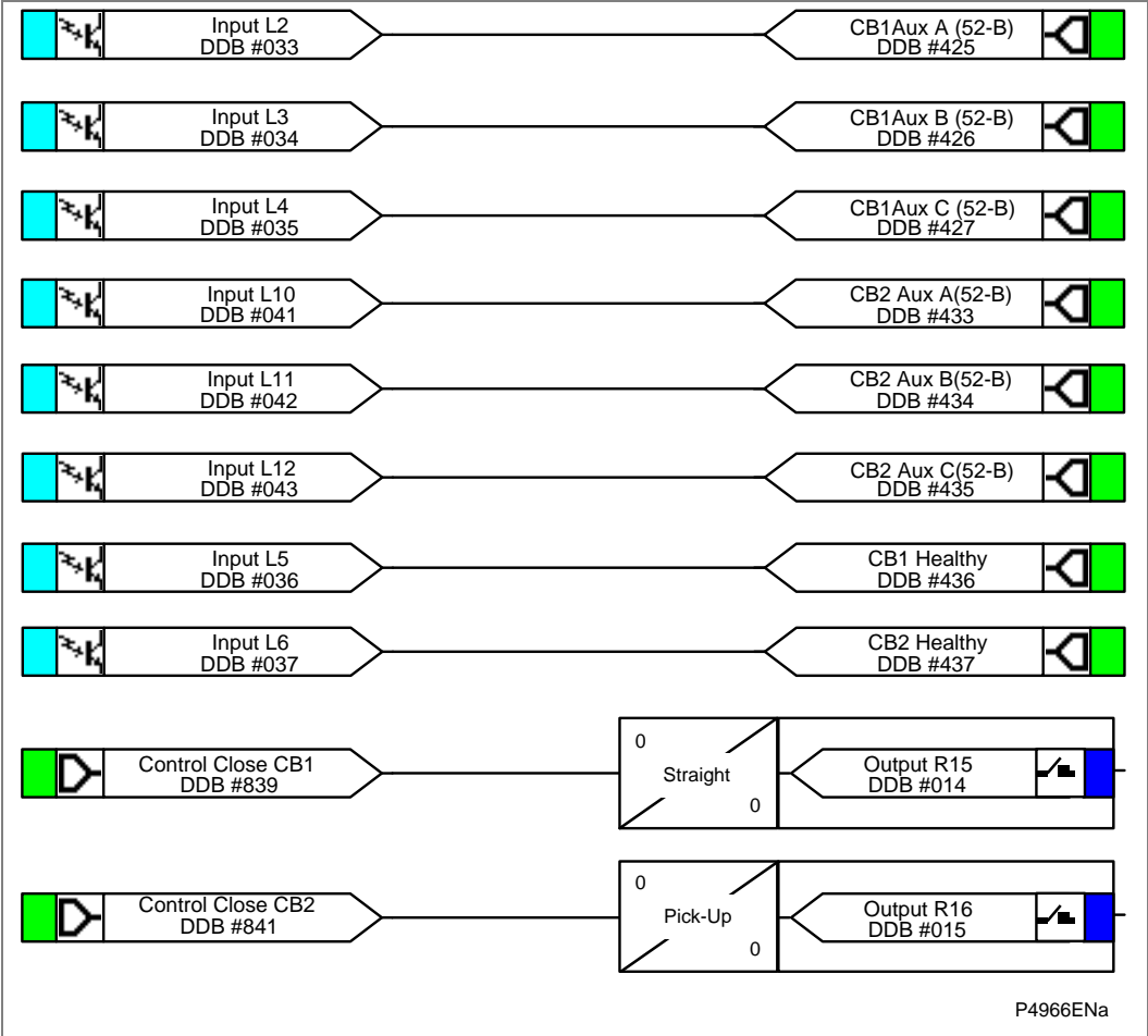
Figure 36 - PSL mapping of some of the opto inputs and relay outputs
