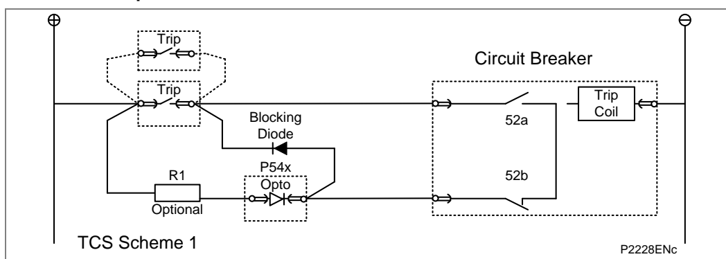
Figure 31 - TCS scheme 1
