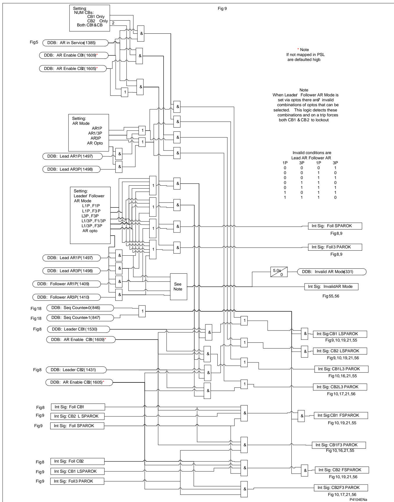
Figure AR-10 - Leader &amp; follower AR modes enable
