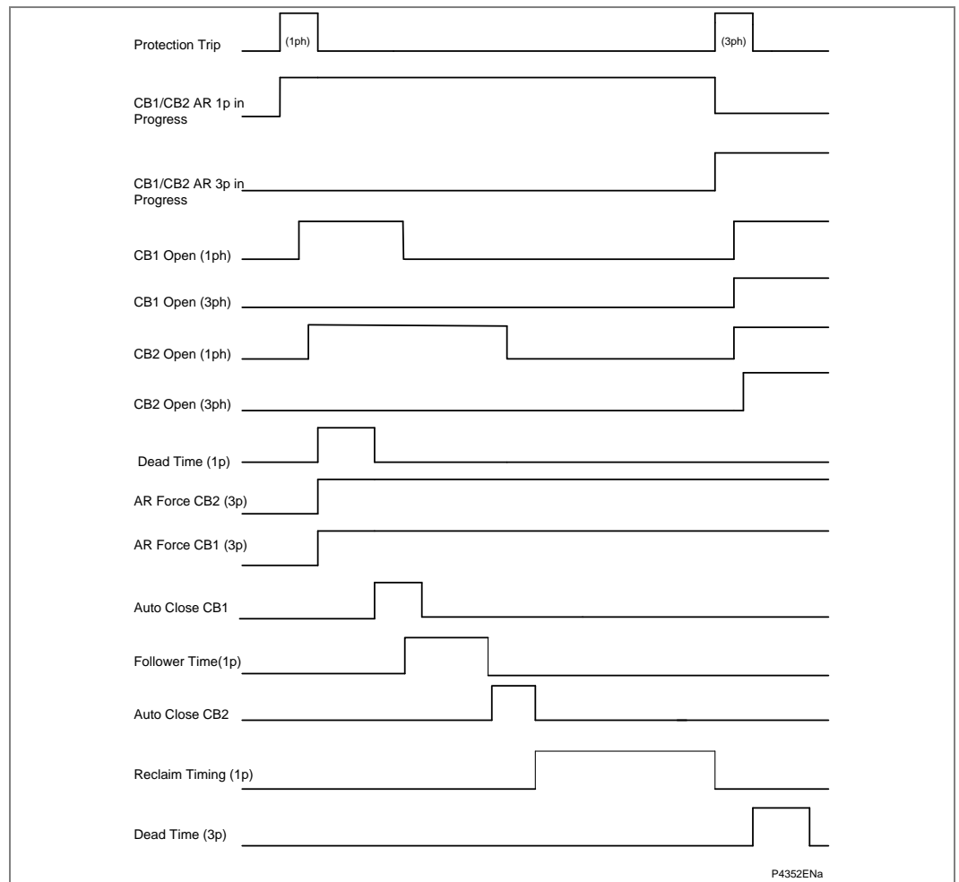
Figure 139 - Auto-reclose timing diagram – repeated fault inception
