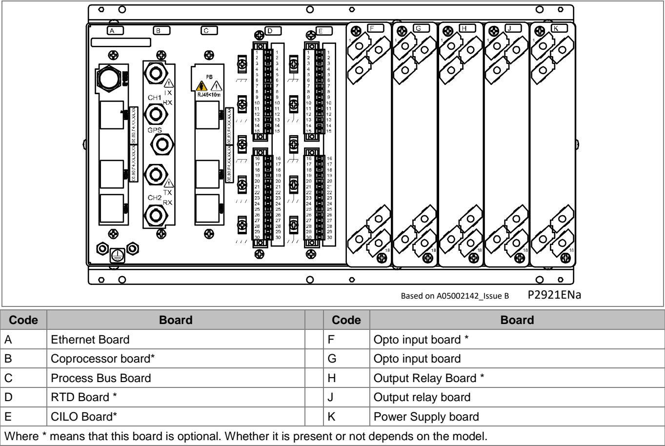
Figure 30 – MiCOM Px40 process bus – rear view
