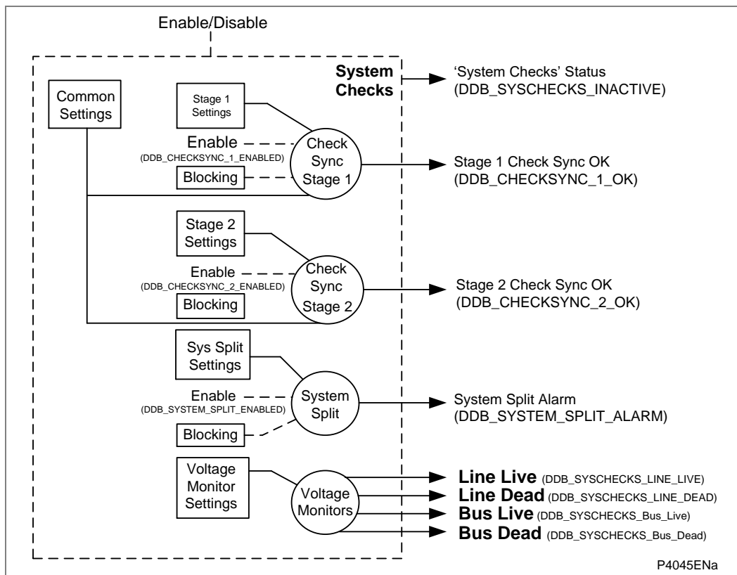
Figure 121 - Check sync (P543/P545)
