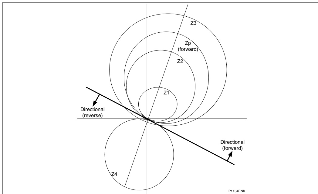
Figure 18 - Phase fault Mho characteristics (Distance option only)
