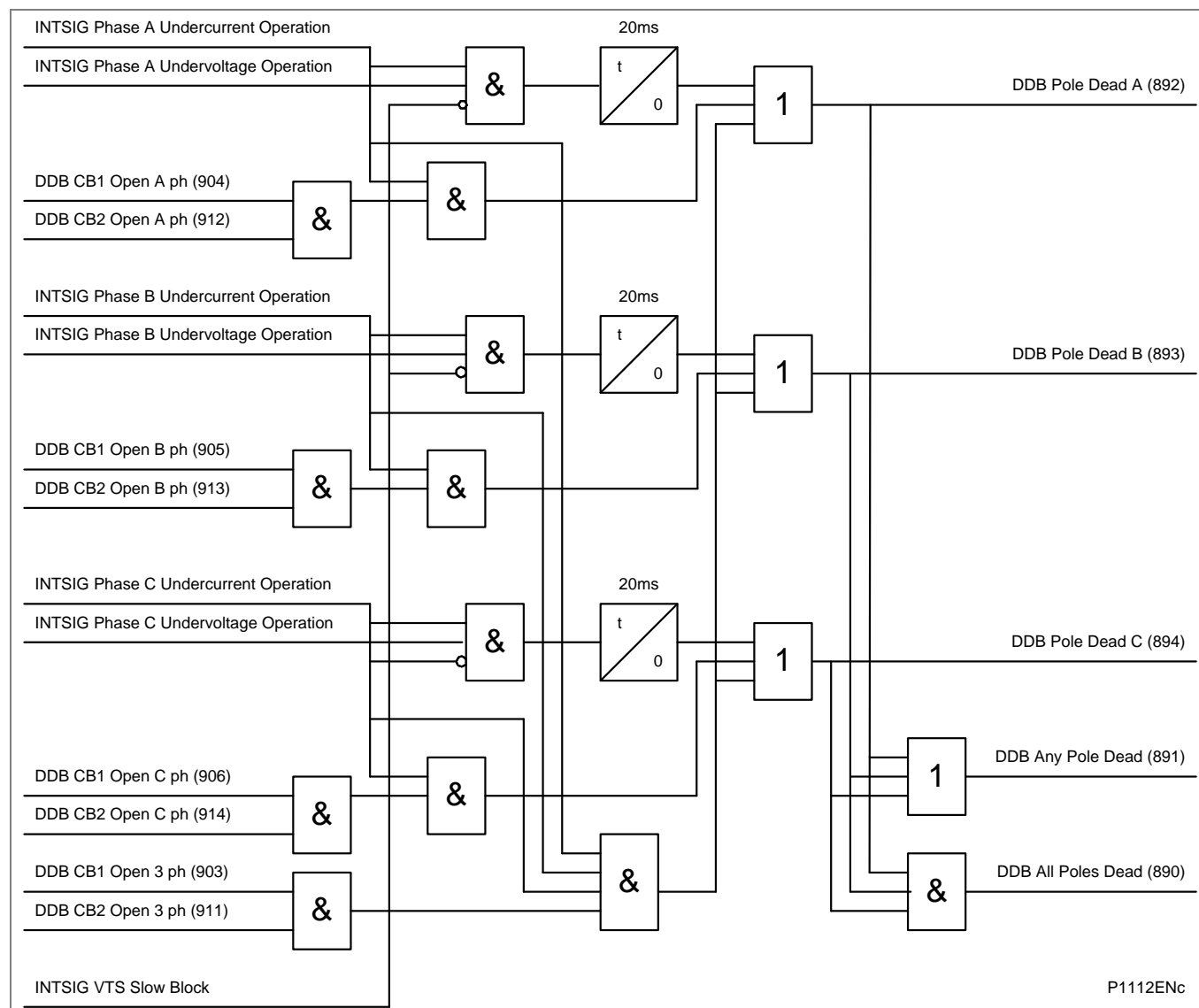
Figure 17 - Pole dead logic for P544/P546
