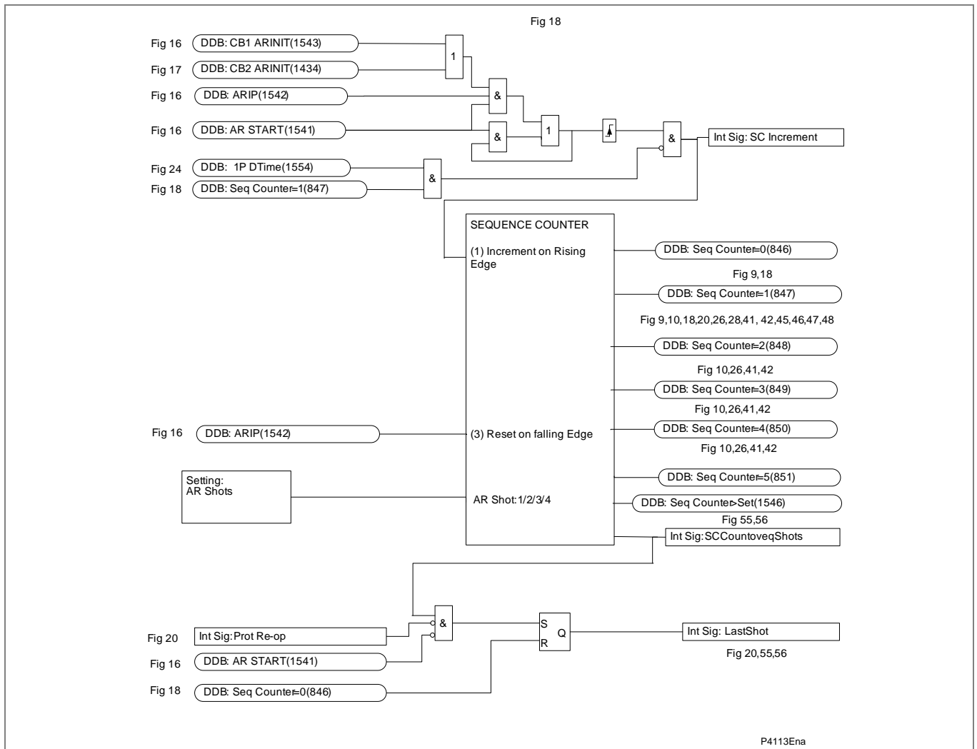
Figure AR-19 - Sequence counter
