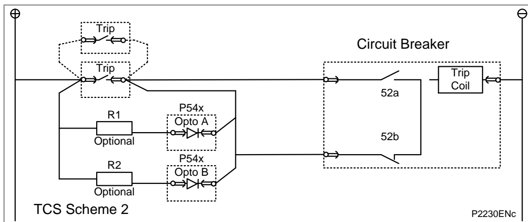
Figure 33 - TCS scheme 2
