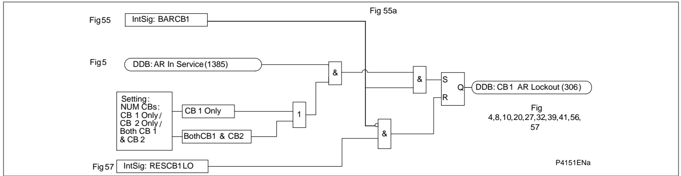
Figure AR-54 - Auto-reclose lockout – CB1
