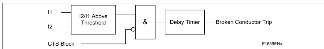
Figure 74 - Broken conductor logic
