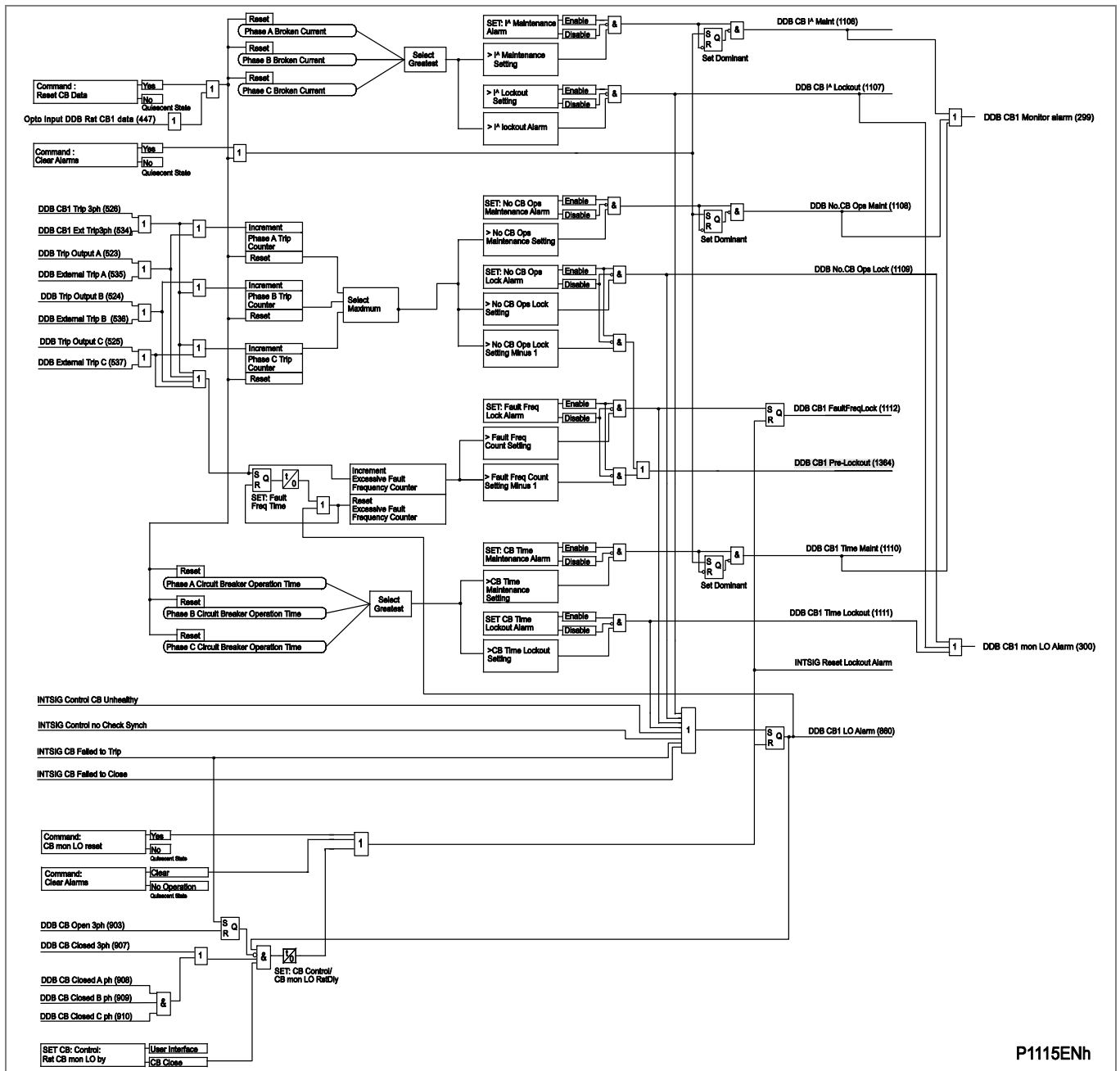
Figure 134 - Circuit breaker 1 – monitoring
