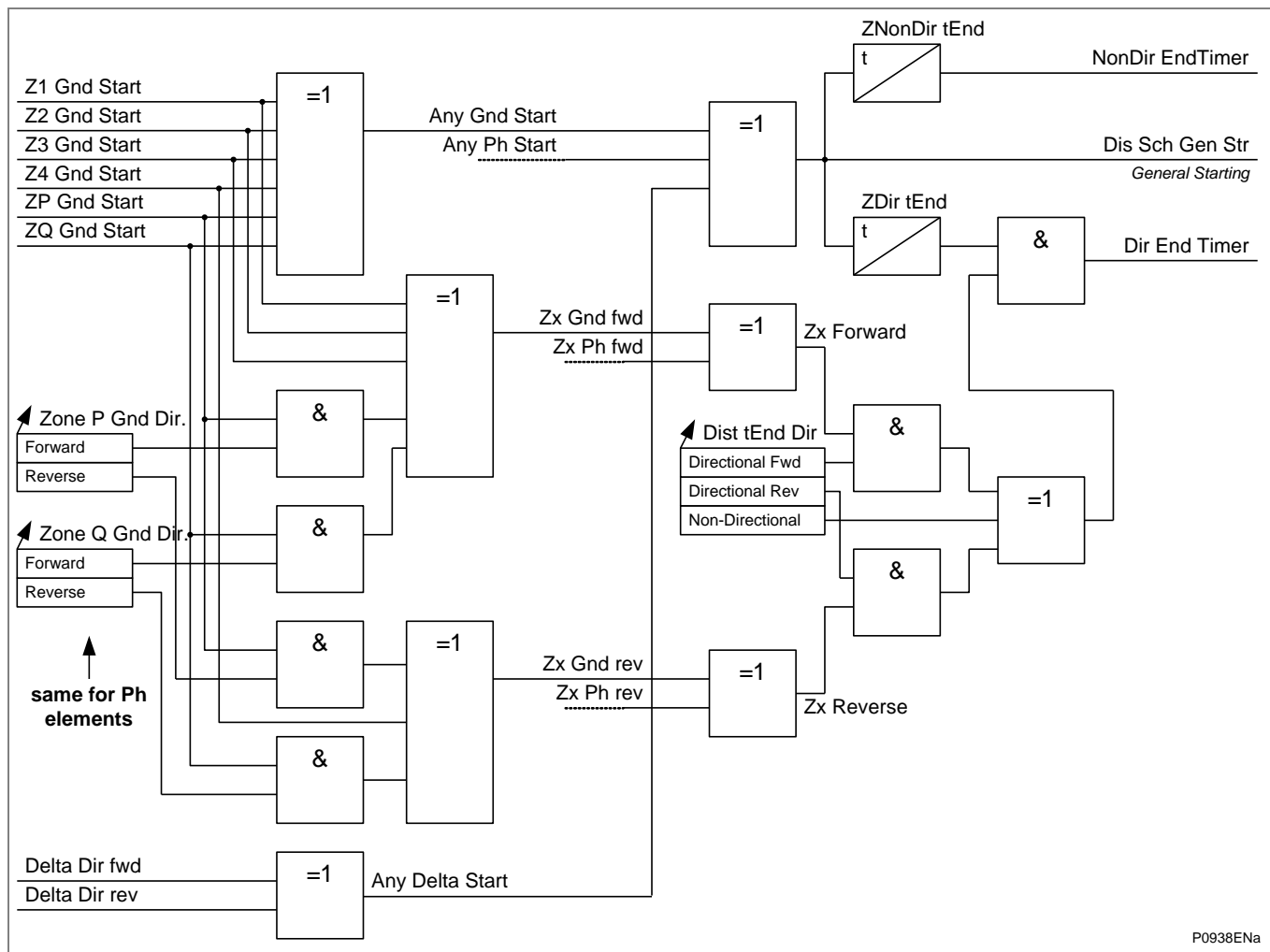
Figure 20 – General starting logic and end timers
