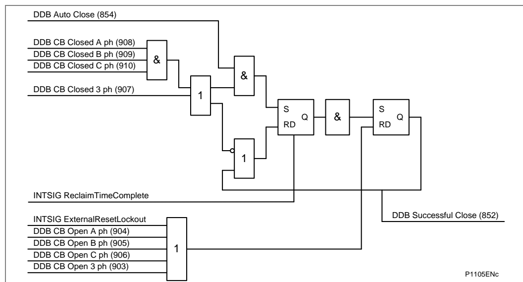
Figure 118 - Auto-reclose close notify (P543/P545)
