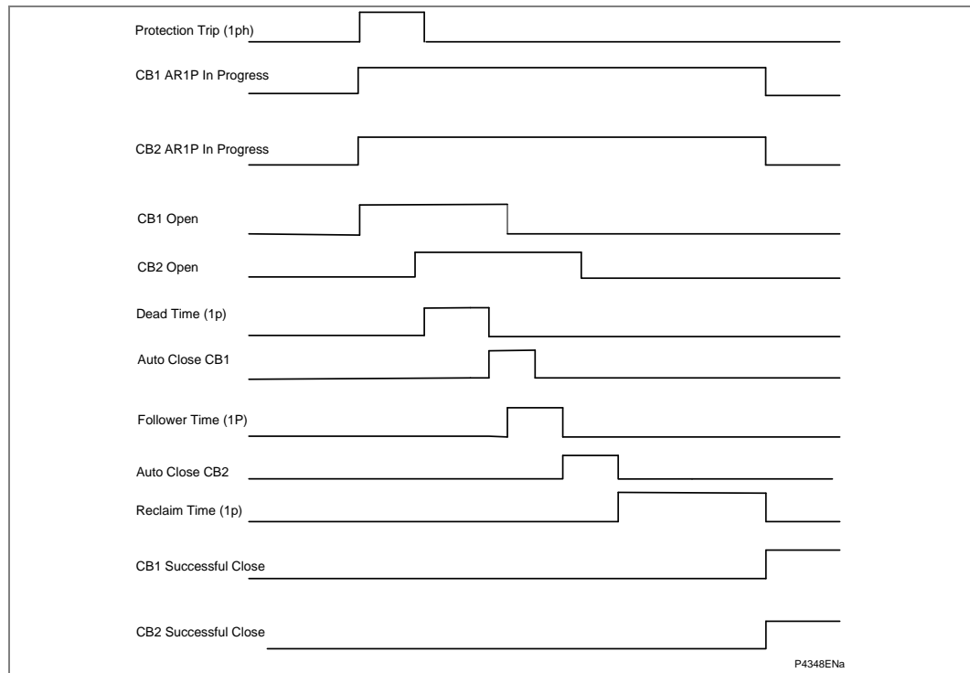
Figure 140 - Auto-relapse timing diagram leader/follower (1ph)
