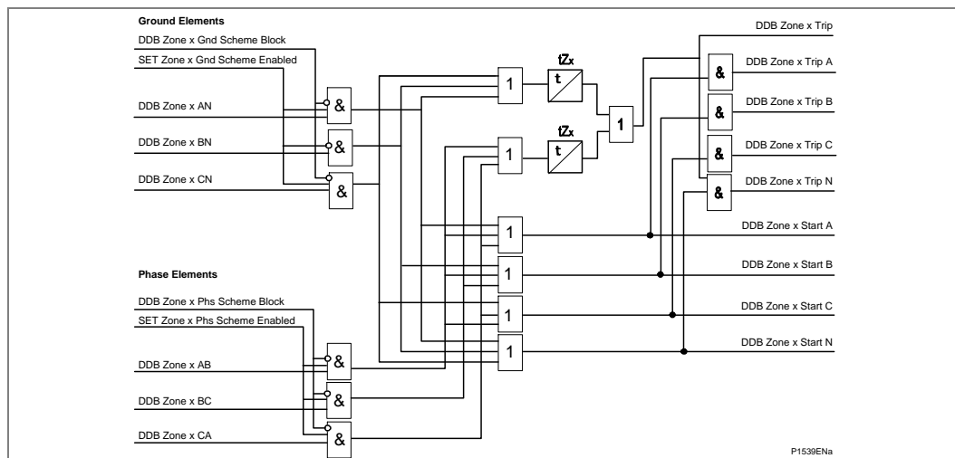
Figure 28 - Basic scheme delayed trip (Distance option only)
