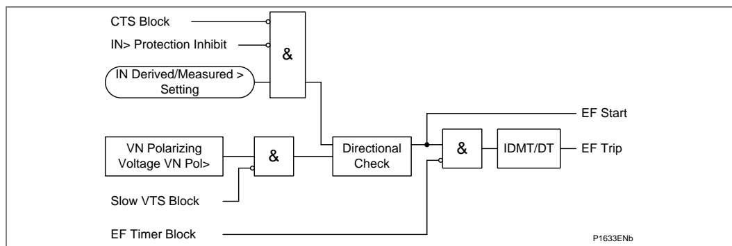
Figure 63 - Directional EF with neutral voltage polarization (single stage)
