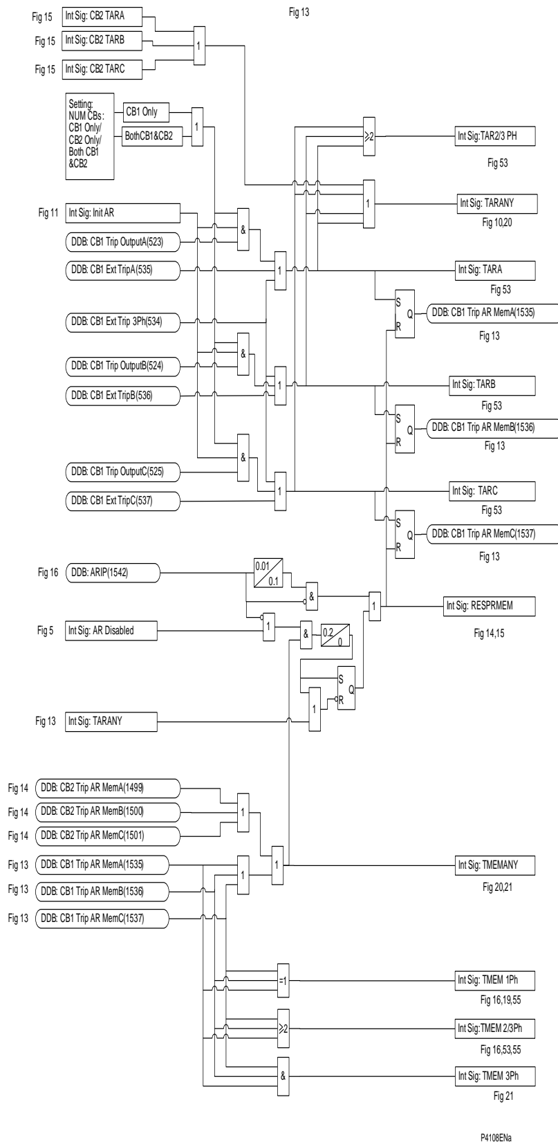
Figure AR-14 - CB1 1pole / 3-pole trip + AR initiation
