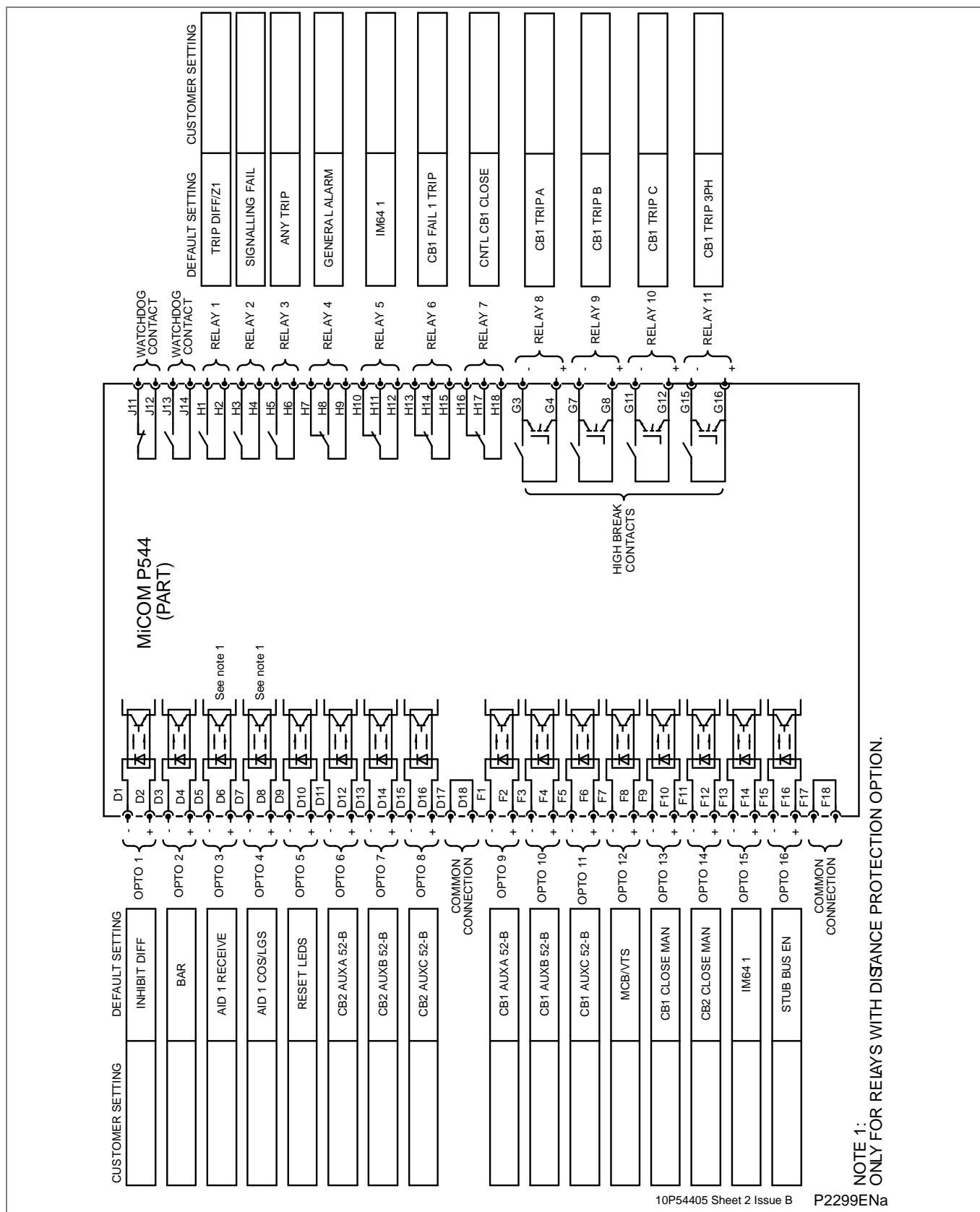
Figure 13 - P544 - 16 inputs/outputs default mapping - 7 standard &amp; 4 high-break outputs
