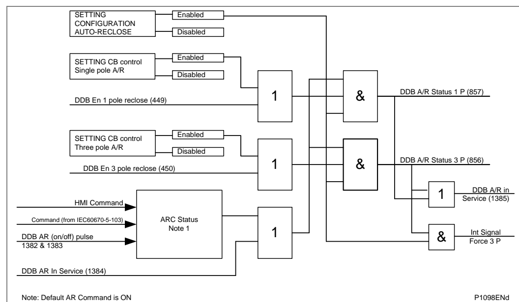
Figure 111 - Auto-reclose enable logic
