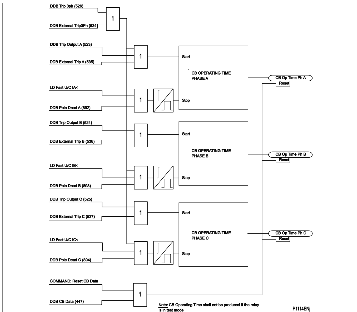
Figure 124 - Circuit breaker condition monitoring - operation time (P543/P545)
