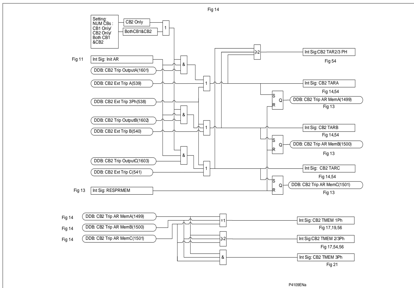
Figure AR-15 - CB2 1 pole / 3-pole trip + AR initiation
