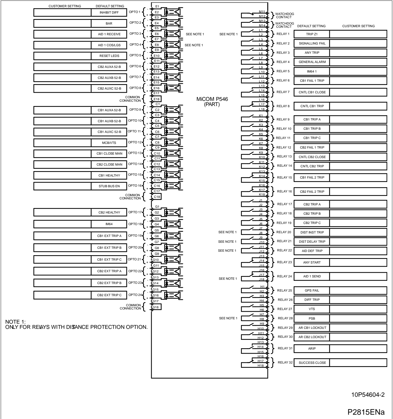
Figure 22 - P546 - 24 opto inputs/32 outputs default mapping - standard & high-break outputs
