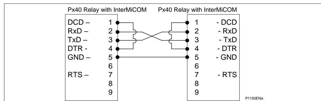
Figure 94 - Direct connection within the local substation
