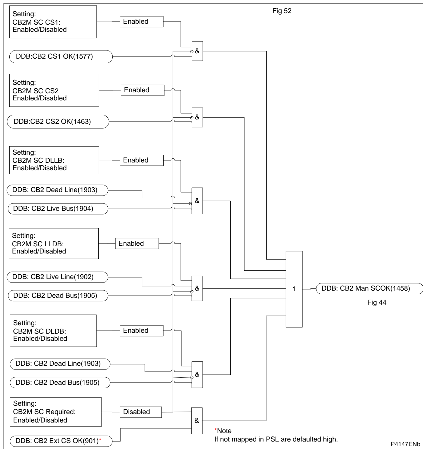
Figure AR-49 - CB2 man. close system check
