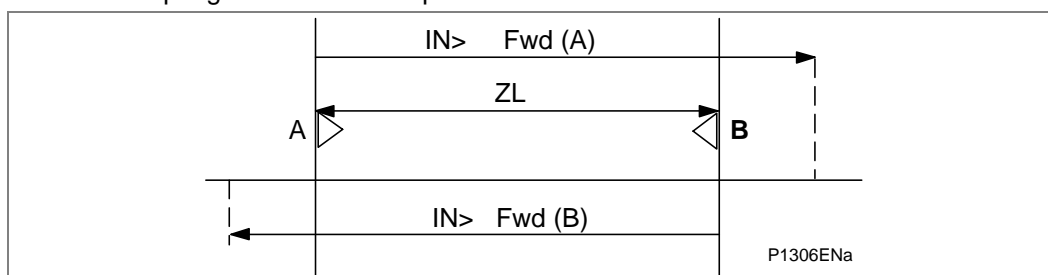
Figure 48 - The DEF permissive scheme (Distance option only)
