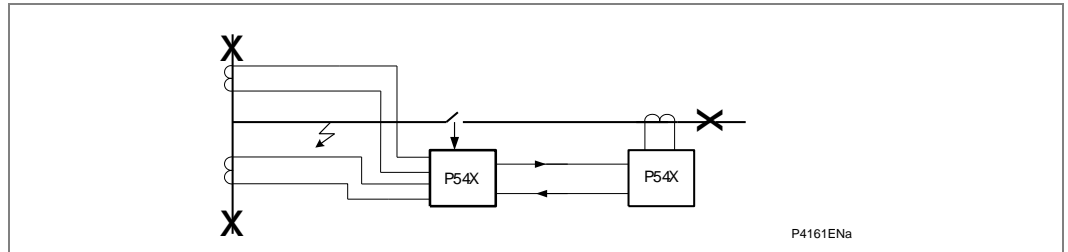
Figure 14 - Stub bus protection
