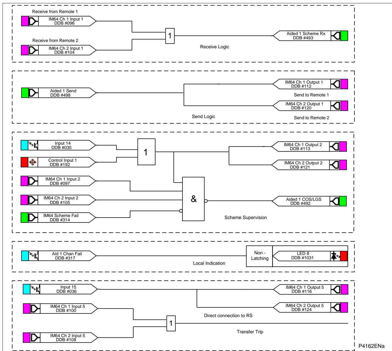
Figure 34 - InterMiCOM 64 mapping in a three ended application
