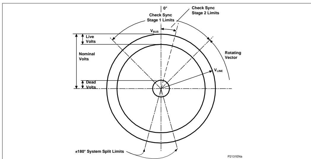
Figure 142 - Synchro check functionality (P544/P546)
