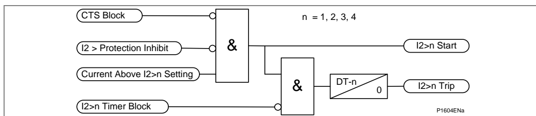
Figure 65 - Negative sequence overcurrent non-directional operation
