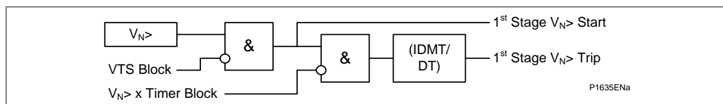
Figure 69 - Residual overvoltage logic (single stage)
