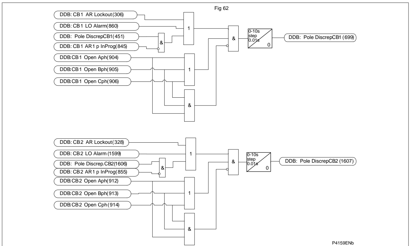
Figure AR-64 – Pole discrepancy (for P546 only)
