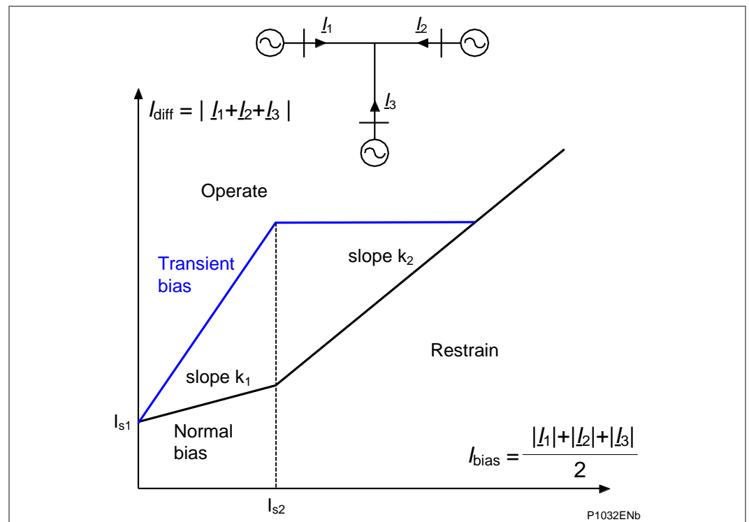
Figure 87 - Transient bias characteristic
