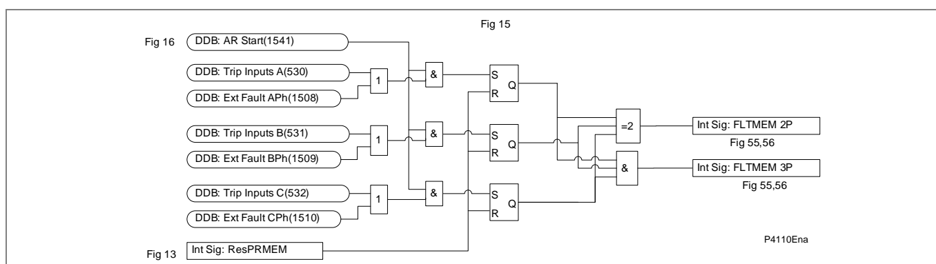
Figure AR-16 - 1Ph, 2Ph &amp; 3Ph fault memory
