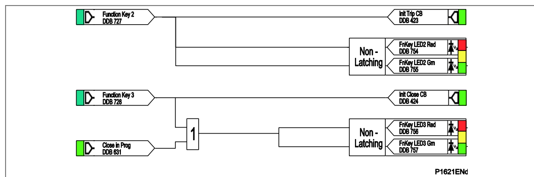
Figure 137 - Circuit breaker control via function keys default PSL
