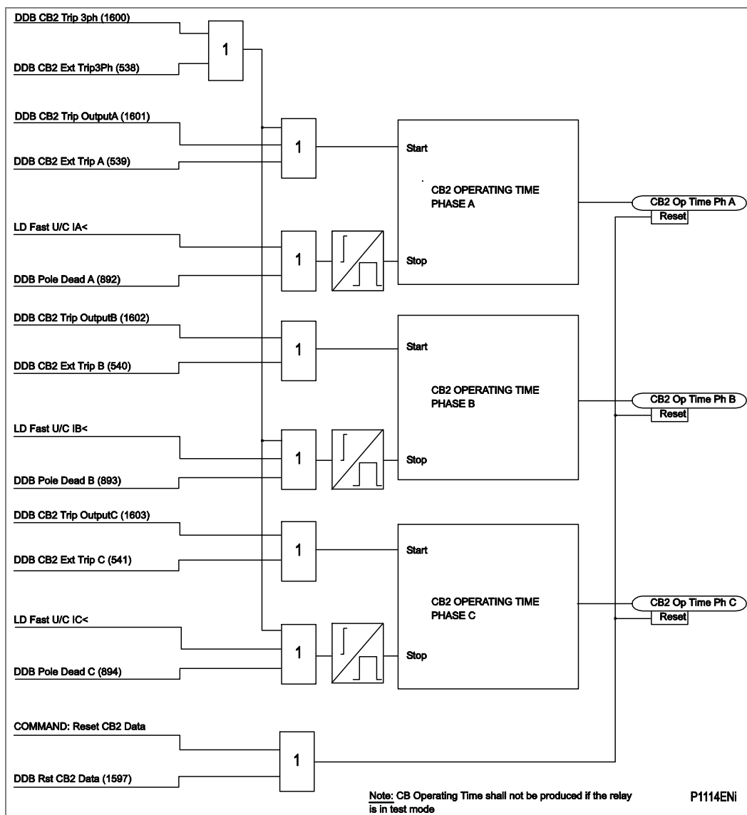
Figure 133 - CB2 condition monitoring – operation time
