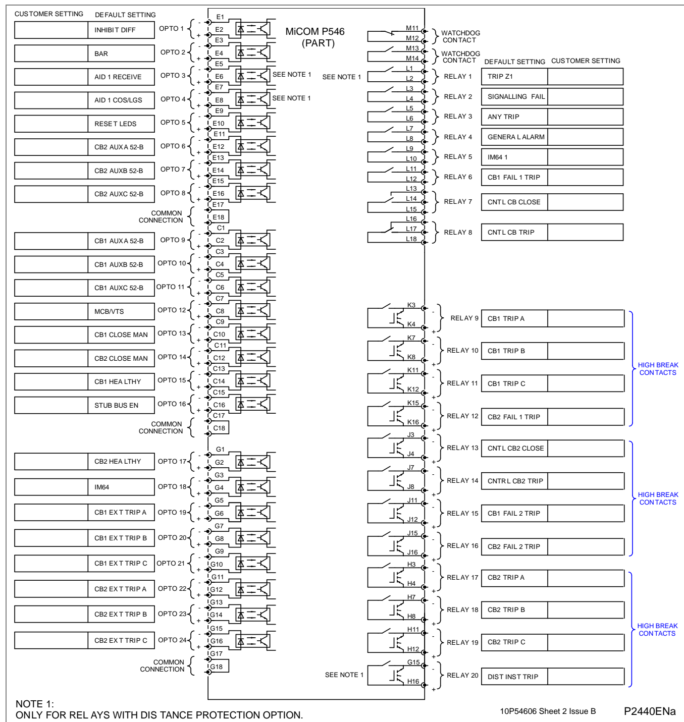
Figure 26 - P546 - 24 inputs/outputs default mapping – 8 Standard &amp; 12 high-break outputs
