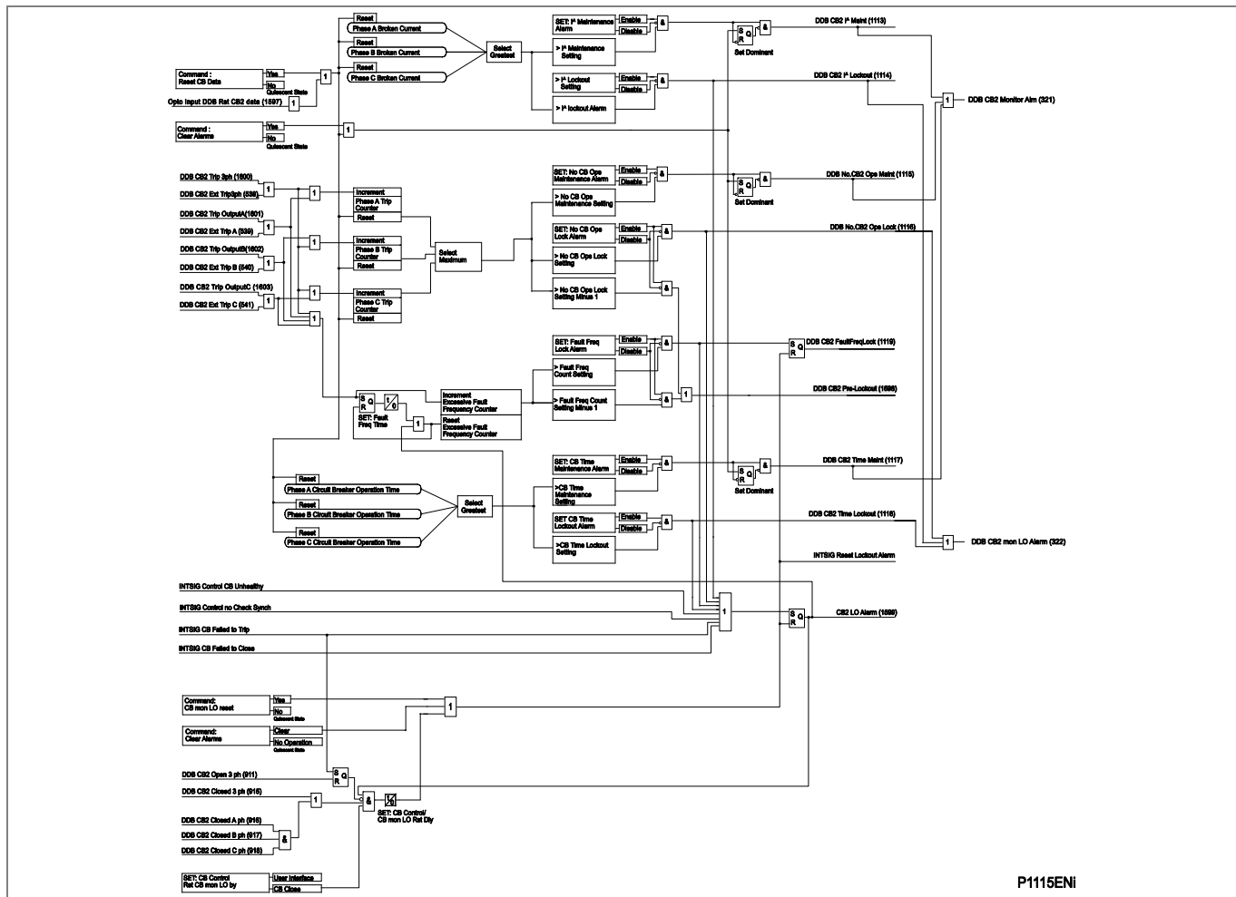
Figure 135 - Circuit breaker 2 – monitoring
