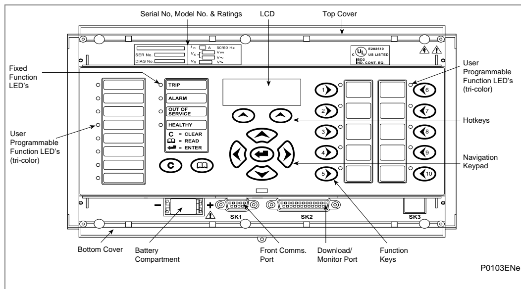
Figure 1 - Relay front view
