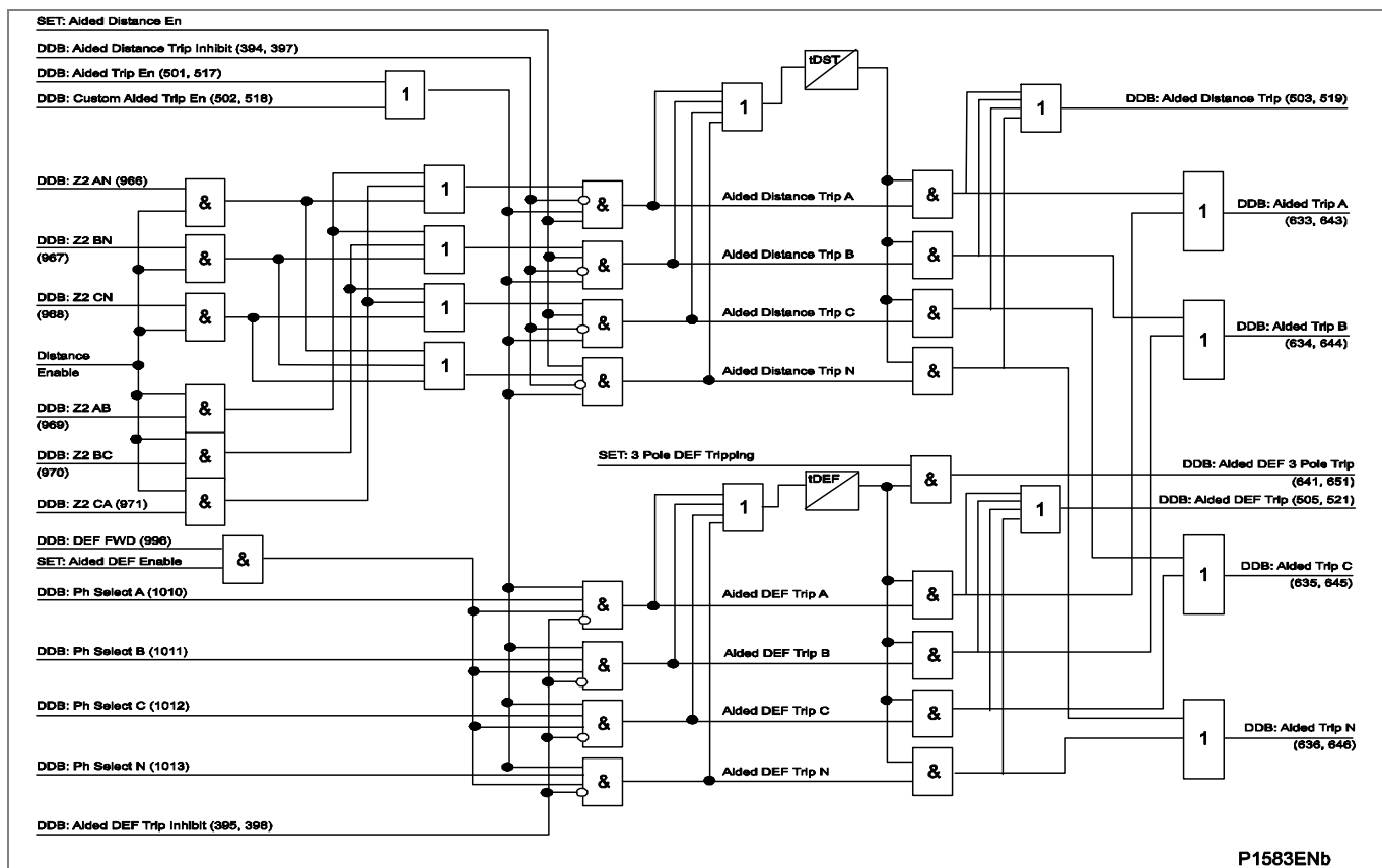
Figure 39 - Aided tripping logic
