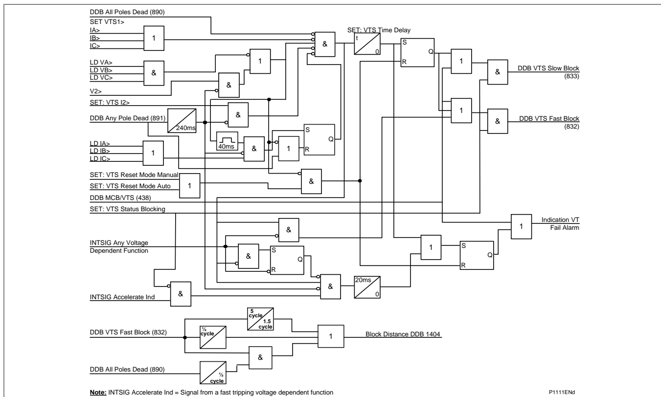
Figure 101 - VTS logic
