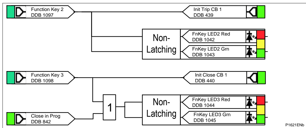
Figure 129 - CB control via function keys default PSL
