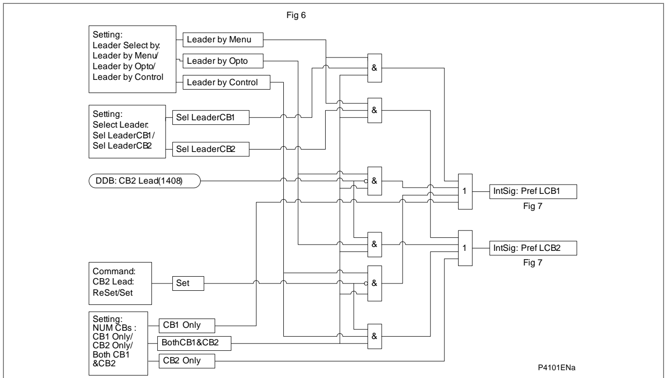
Figure AR-6 - Lead &amp; follower circuit breaker selection
