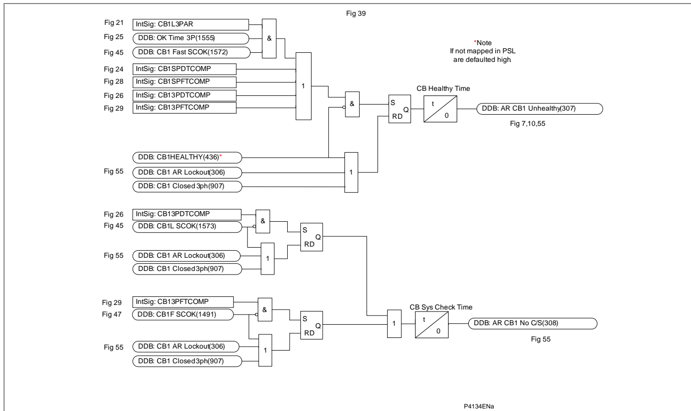
Figure AR-38 - CB healthy &amp; system check timers
