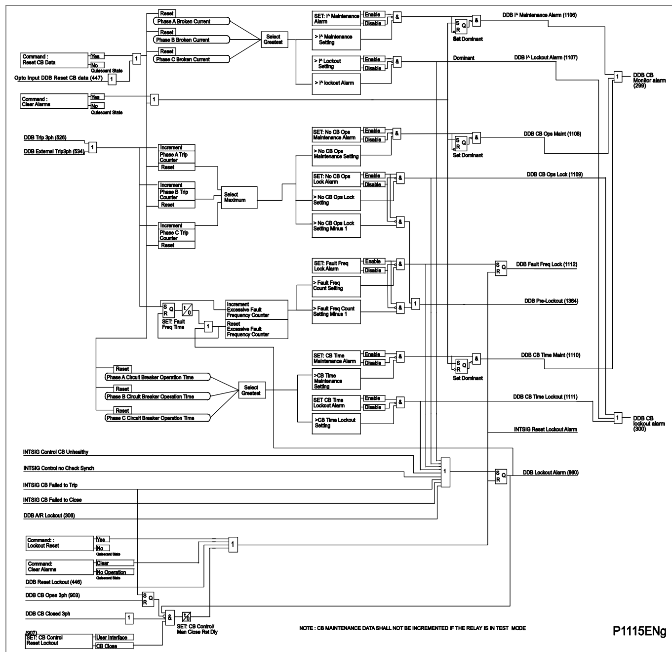
Figure 125 - CB monitoring (P543/P545)
