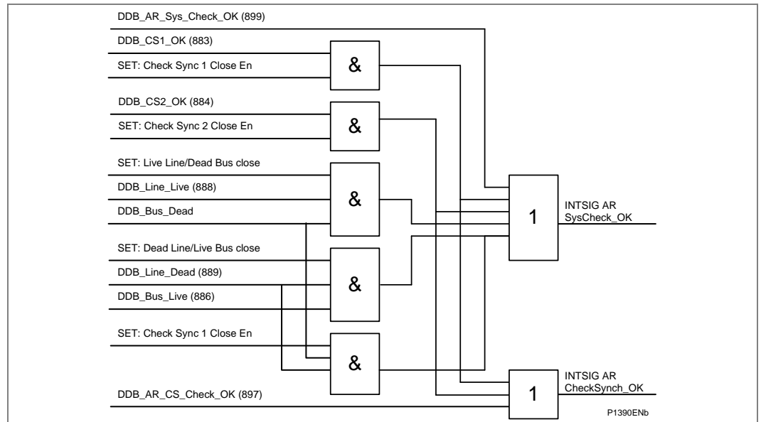
Figure 122 - Auto-reclose/check sync interface (P543/P545)
