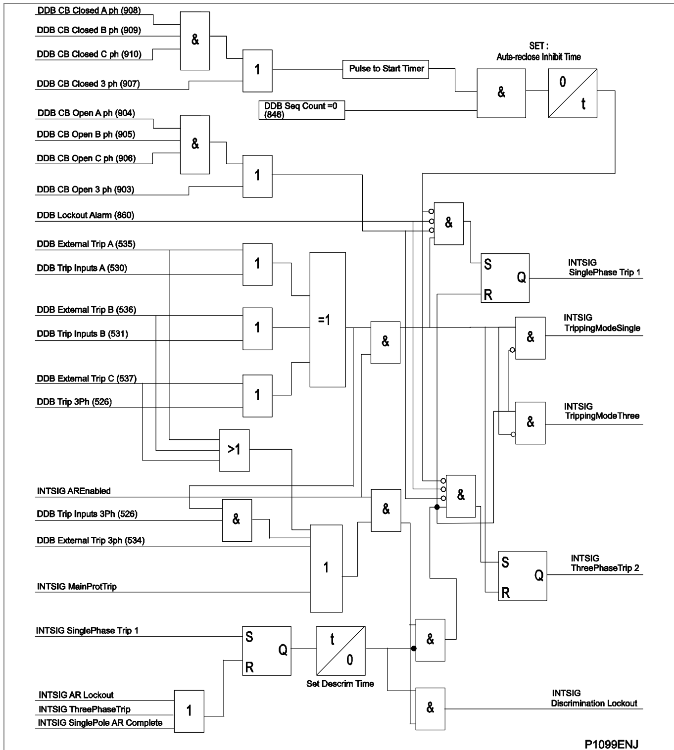
Figure 112 - Auto-reclose single/three pole tripping
