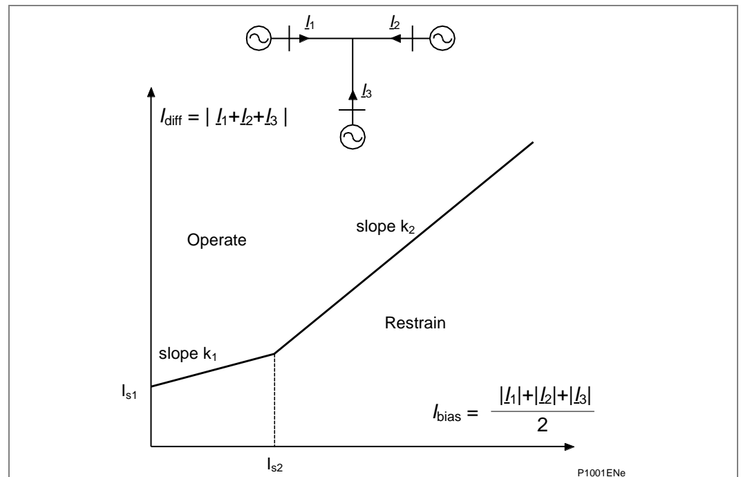
Figure 1 - Relay bias characteristic
