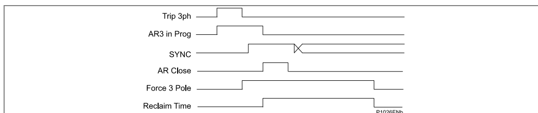
Figure 109 - Auto-reclose timing diagram - fault with system synchronism
