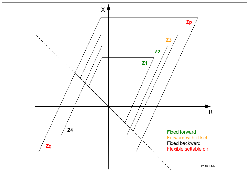
Figure 19 - Earth fault quadrilateral characteristics (Distance option only)
