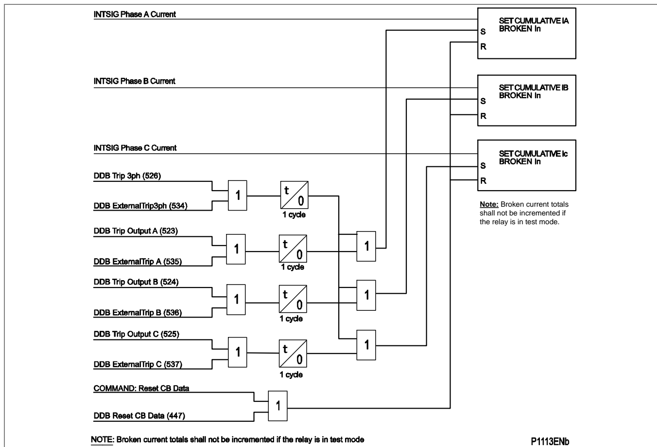
Figure 123 - Circuit breaker condition monitoring - broken current (P543/P545)
