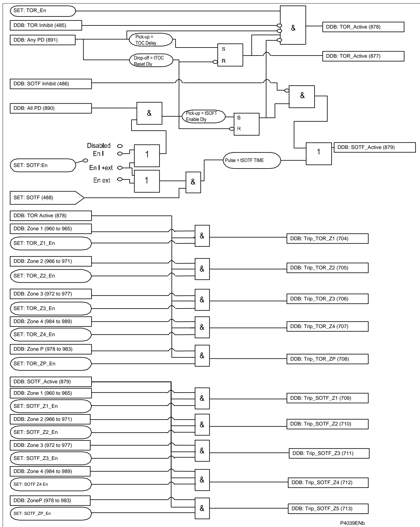
Figure 33 - Trip on close (Distance option only)
