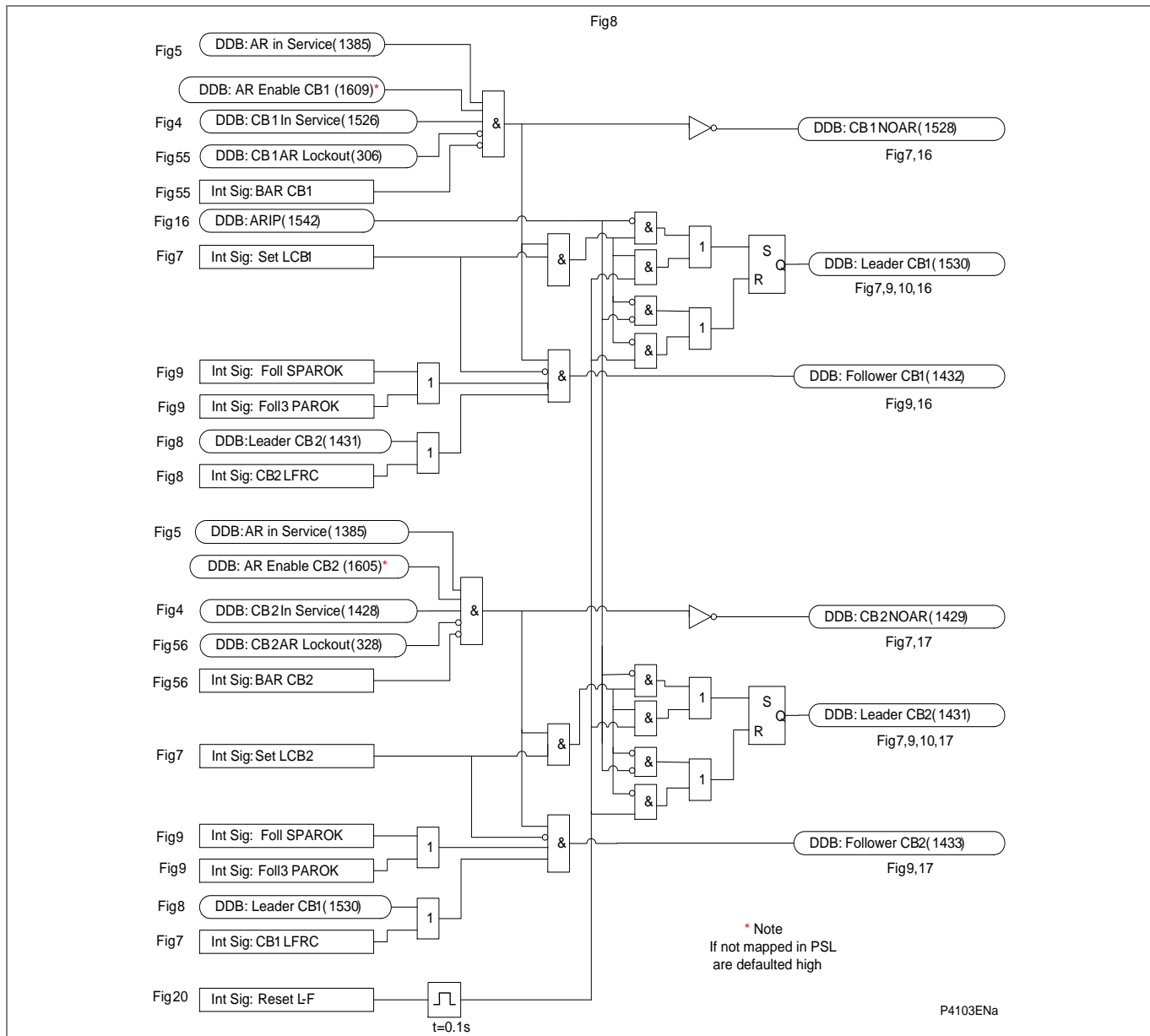
Figure AR-9 - Leader/follower logic – 2
