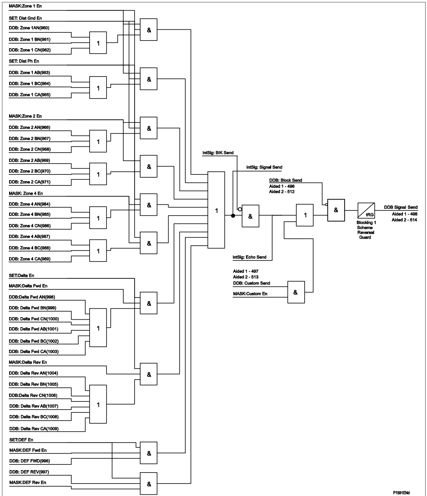
Figure 37 - Send logic (Distance option only)
