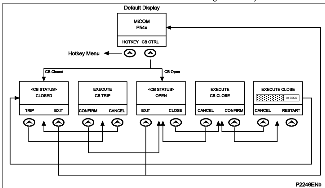
Figure 128 - CB control hotkey menu
