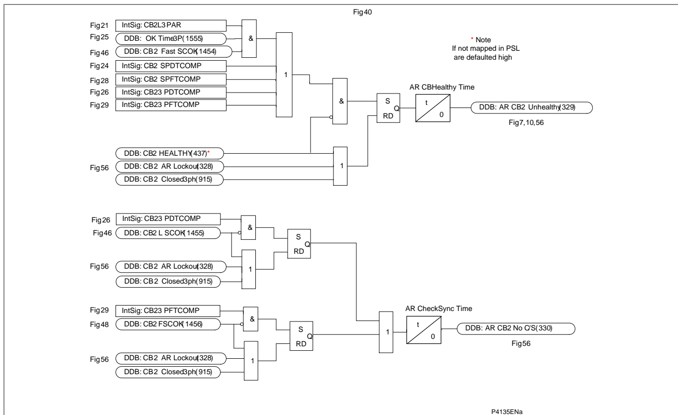
Figure AR-39 - CB2 healthy &amp; system check timers
