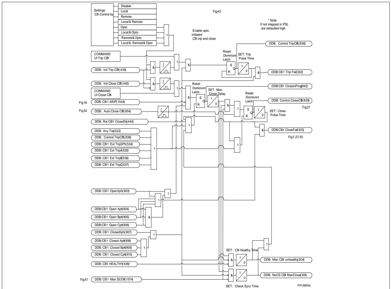
Figure AR-42 - CB1 circuit breaker control
