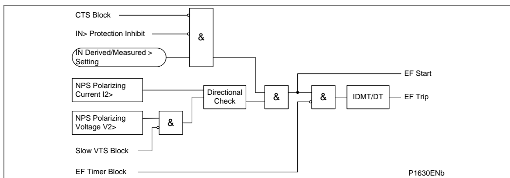
Figure 64 - Directional EF with negative sequence polarization (single stage)
