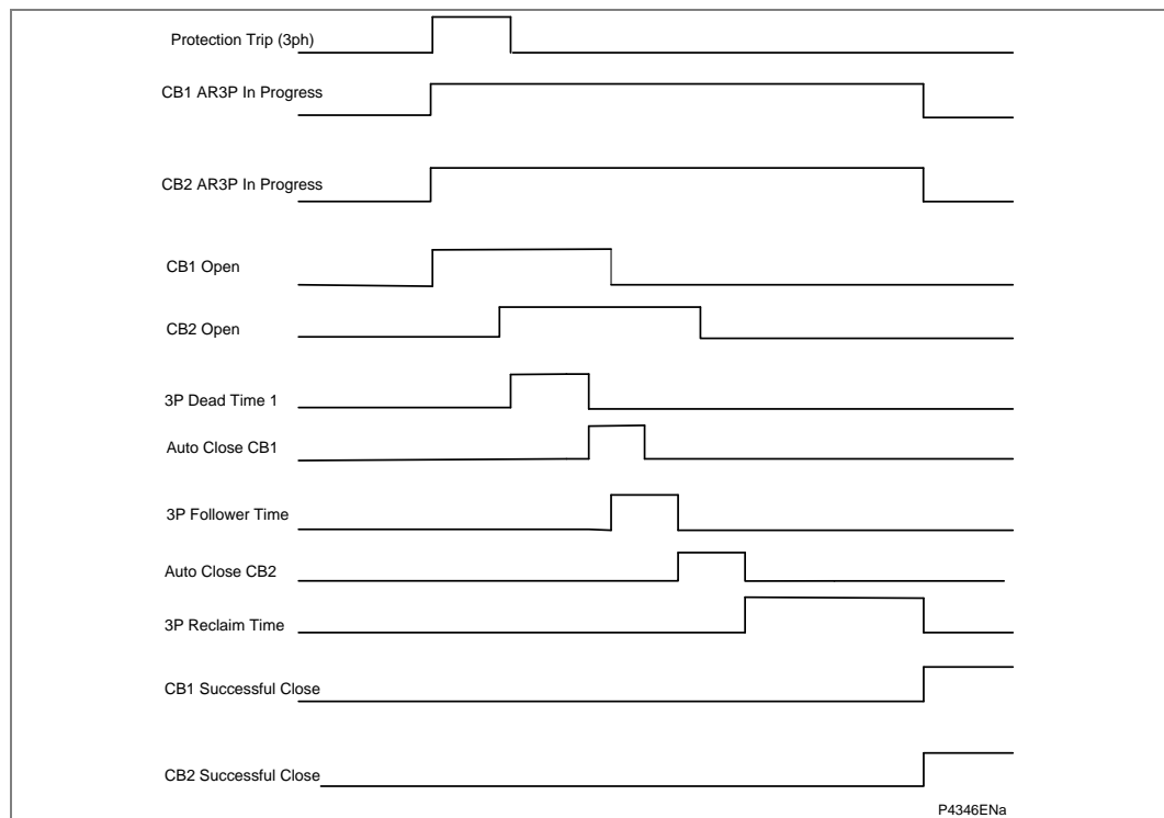
Figure 141 - Auto-relapse timing diagram leader/follower (3ph)
