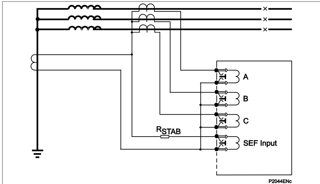
Figure 62 - High impedance REF relay/CT connections
