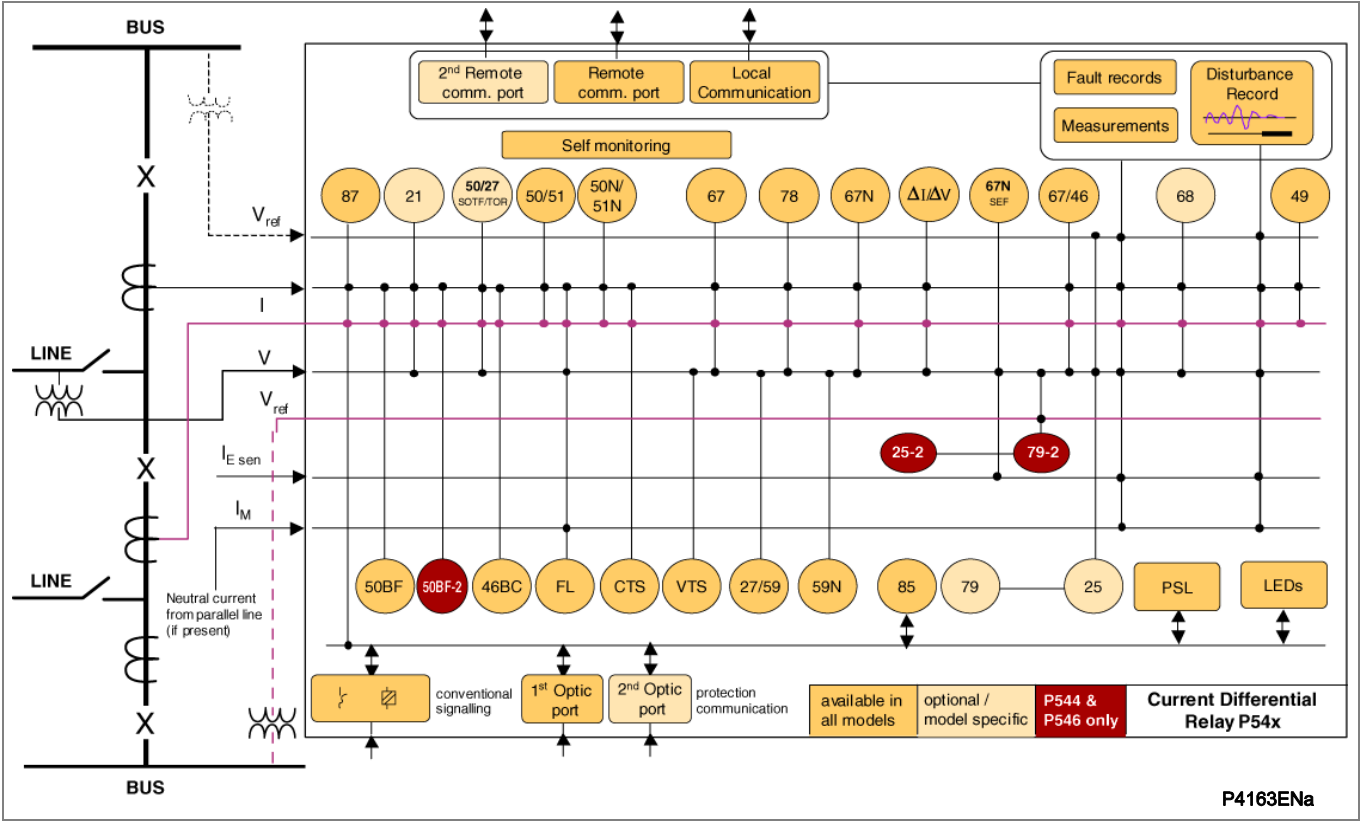
Figure 2 - Functional diagram
