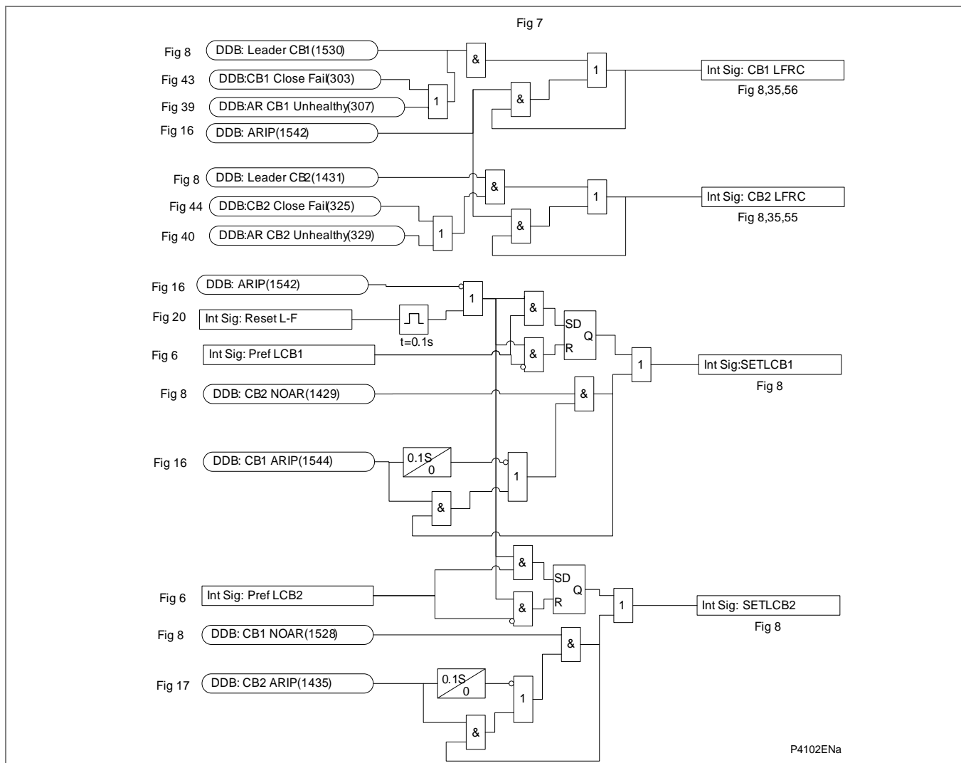
Figure AR-7 - Leader/follower logic – 1 (for Software Versions BEFORE H1)
