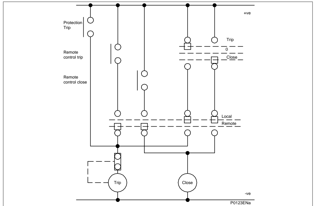
Figure 126 - Remote control of circuit breaker (P543/P545)
