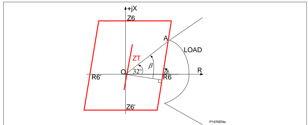
Figure 15 - R6_{MAX} determination
