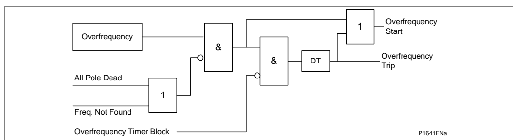
Figure 76 -Overfrequency logic (single stage)
