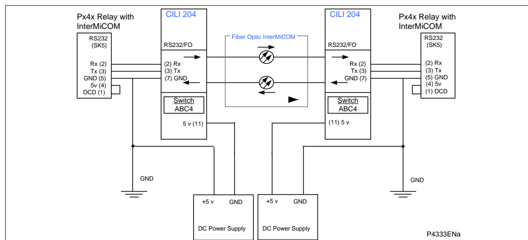
Figure 97 - MODEM InterMiCOM teleprotection via fiber optic
