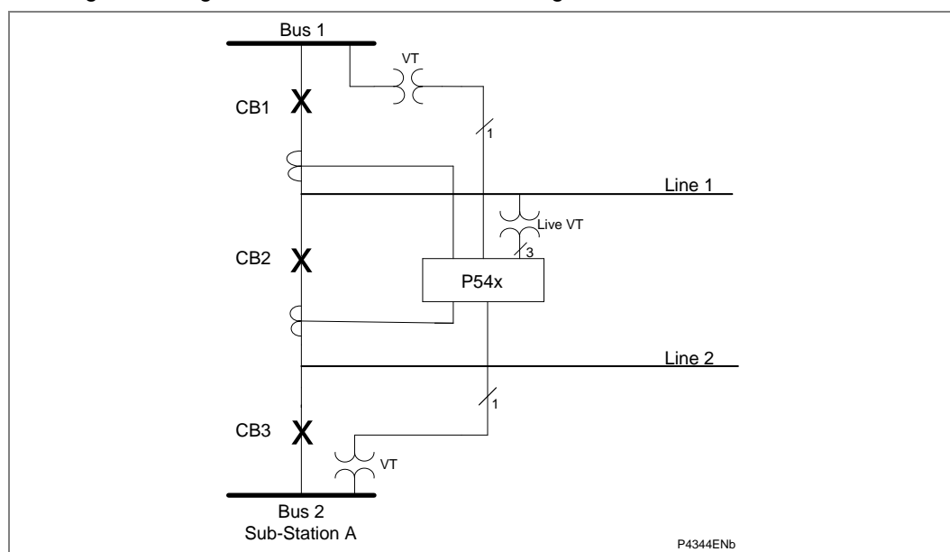
Figure 35 - Two circuit breaker auto-reclose application
