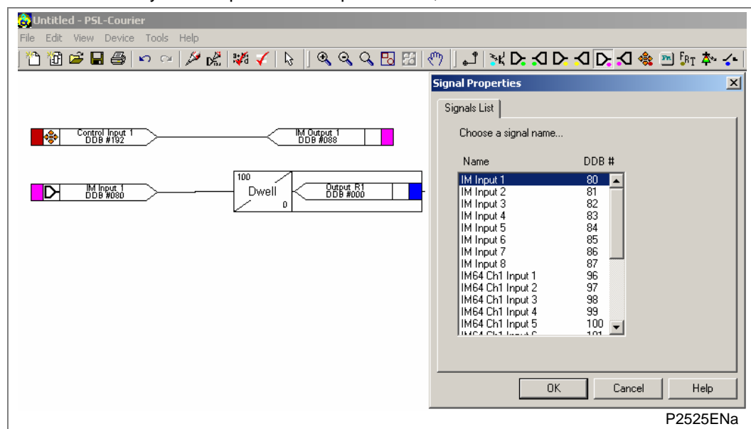
Figure 98 - Example assignment of signals within the PSL
