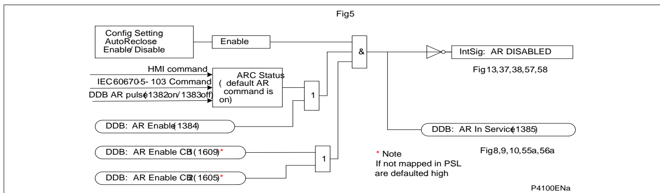
Figure AR-5 - Auto-reclose enable
