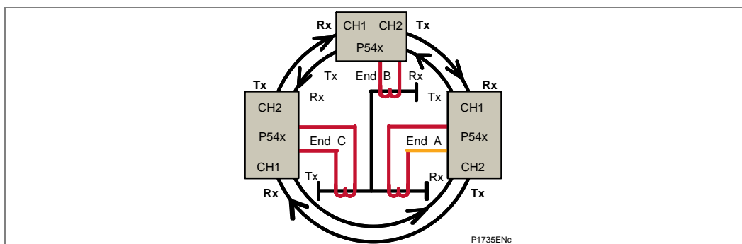
Figure 99 - Triangulated InterMiCOM 64 application
