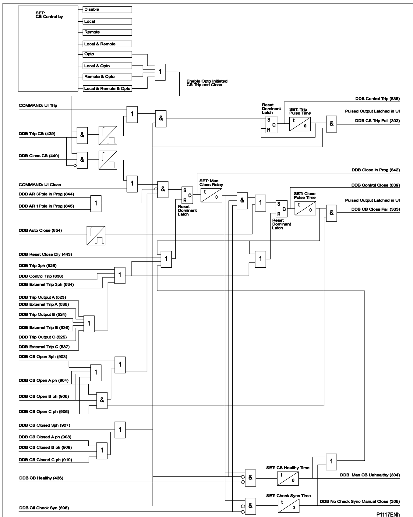
Figure 127 - Circuit breaker control (P543/P545)
