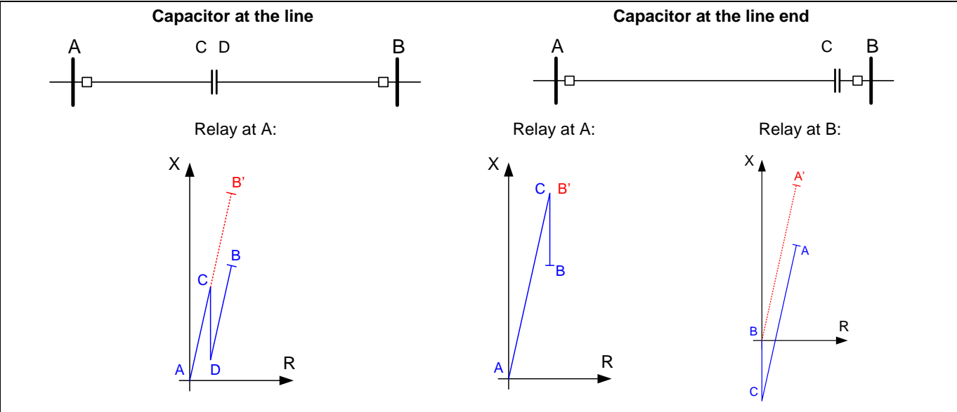
Figure 18 - Effect of series capacitor location to apparent impedance for faults along the line A-B Depending upon the spark gap operation (solid line = capacitor active; dashed line = capacitor bypassed) a fault at the remote line end will be seen with different reaches. In case the capacitor is at the line end and in front of the relay, the apparent impedance becomes negative for close faults.
