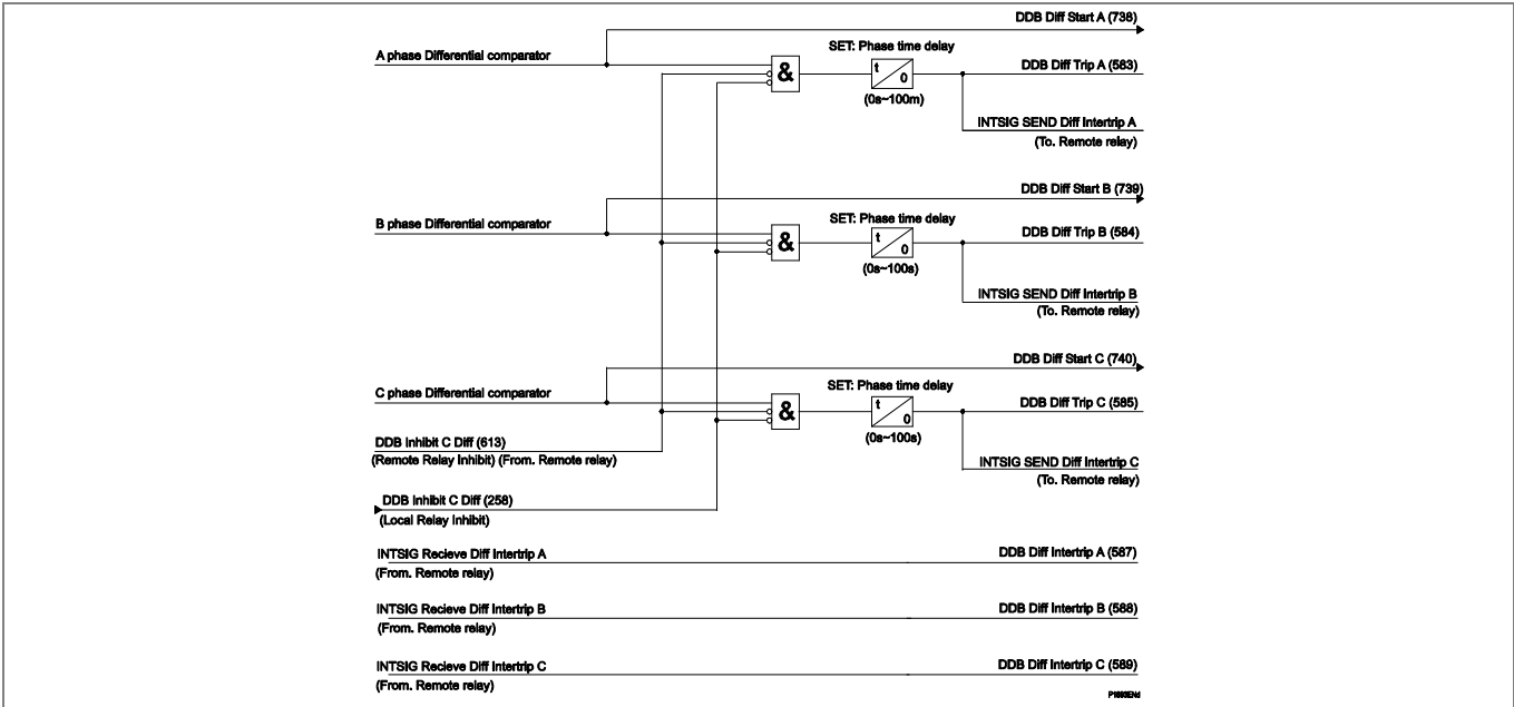
Figure 2 - Differential logic diagram
