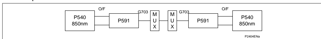
Figure 88 - P54x connection to P591
