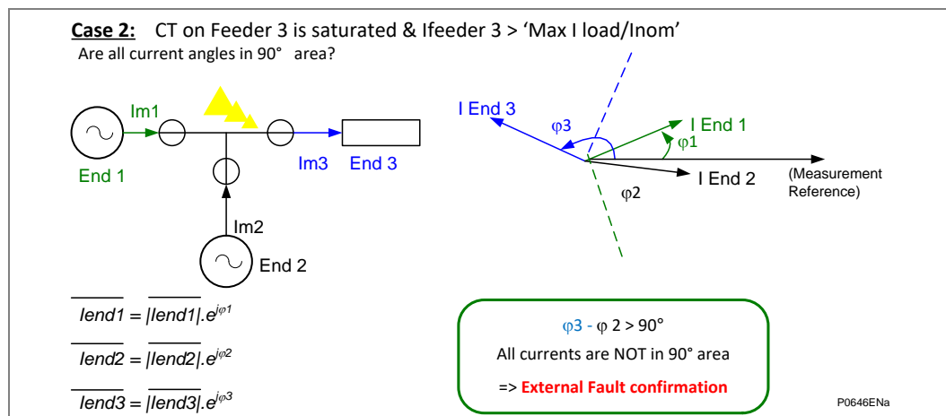
Figure 2 - Differential 3-terminal scheme - external fault
