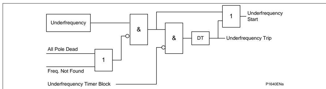
Figure 75 - Underfrequency logic (single stage)
