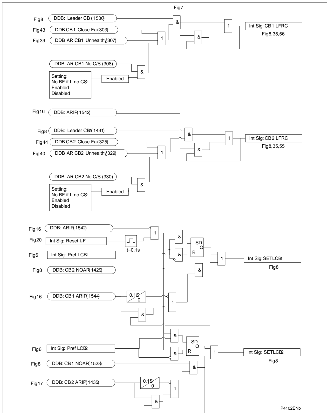
Figure AR-8 - Leader/follower logic – 1 (for Software Versions H1 and later)
