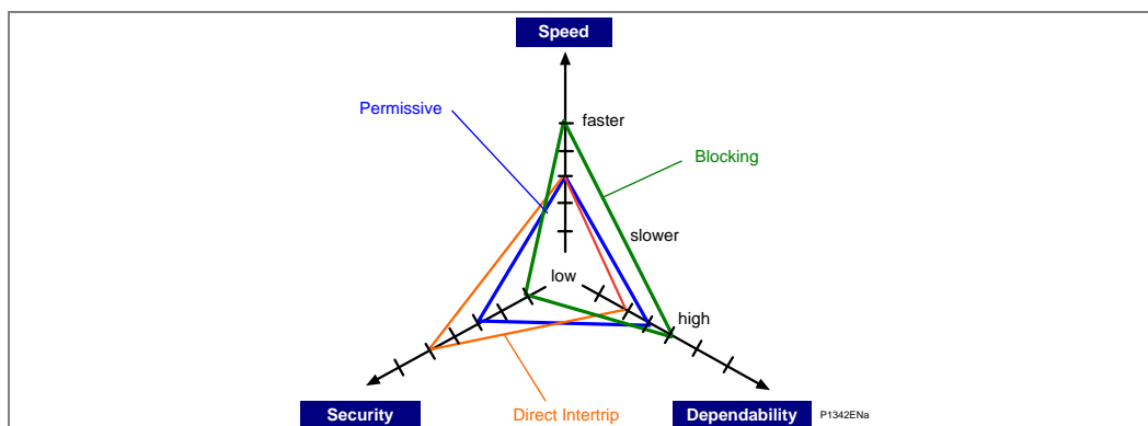
Figure 92 - Pictorial comparison of operating modes
