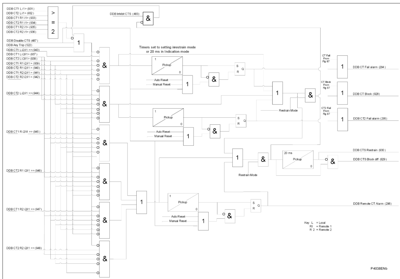
Figure 102 - Differential CTS
