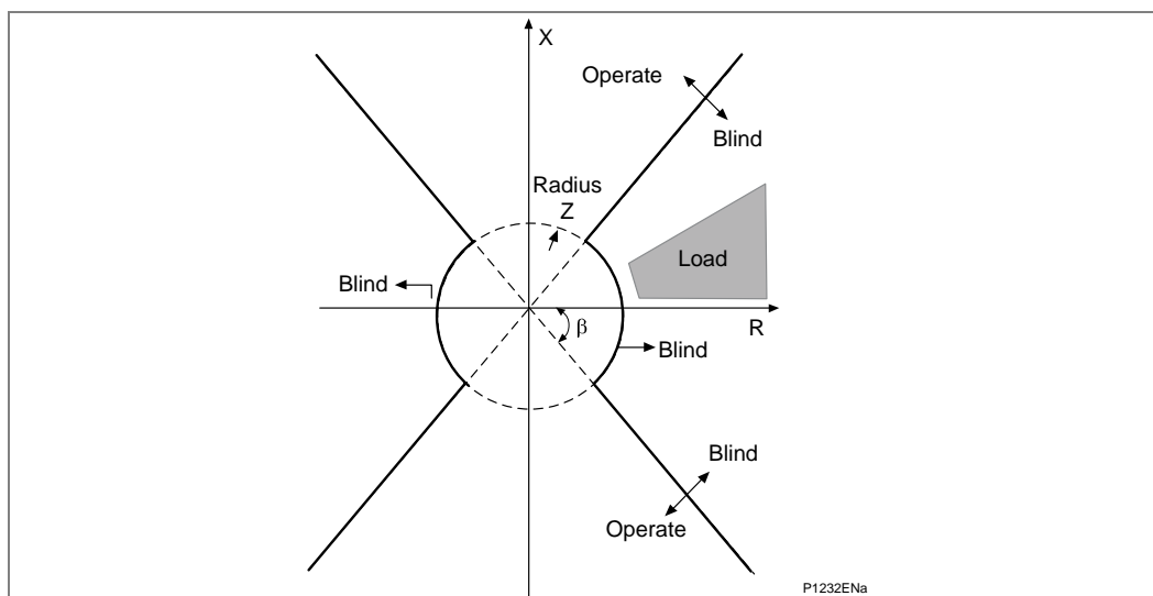
Figure 27 - Load blinder characteristics
