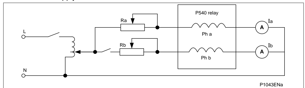
Figure 5 - Connection for bias characteristic testing
