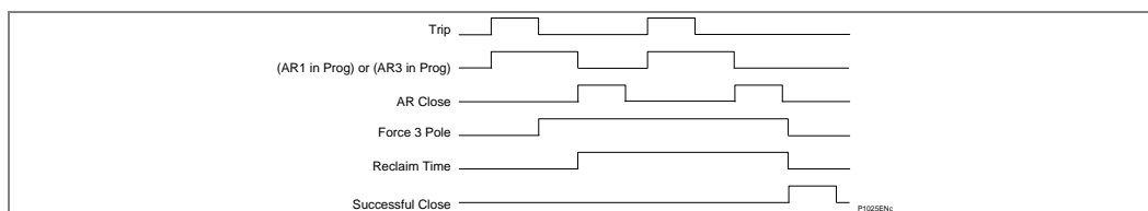
Figure 108 - Auto-reclose timing diagram - repeated fault inception
