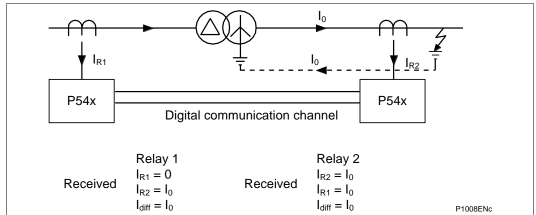
Figure 12 - Need for zero-sequence current filtering
