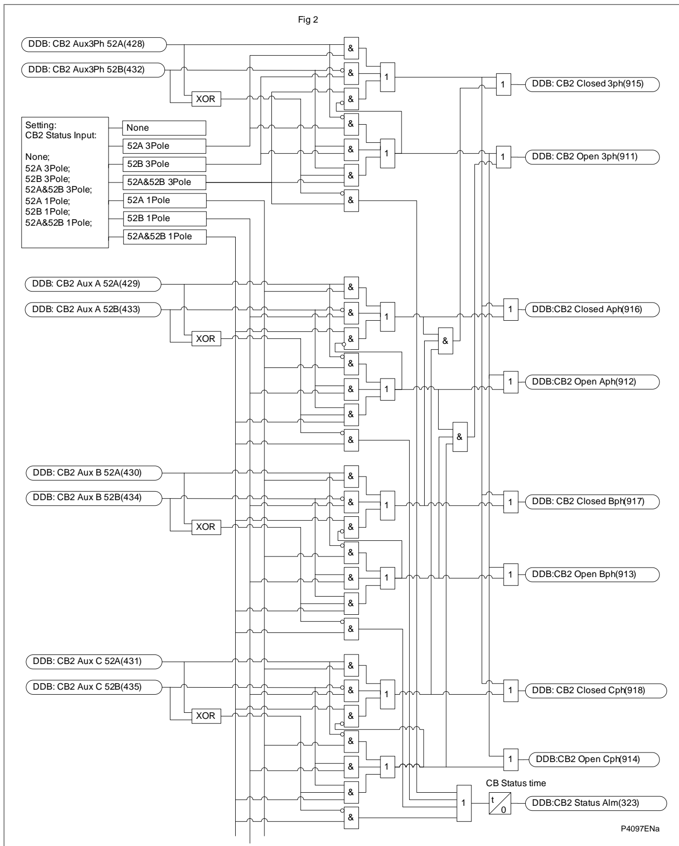
Figure AR-2 - Circuit breaker 2 - state monitor
