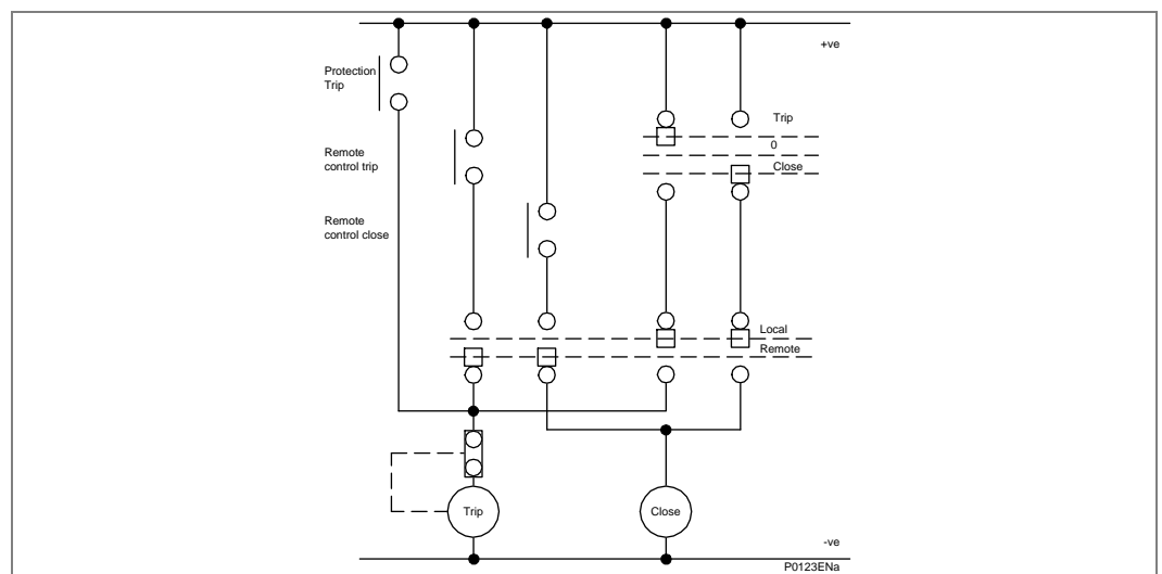
Figure 136 - Remote control of circuit breaker
