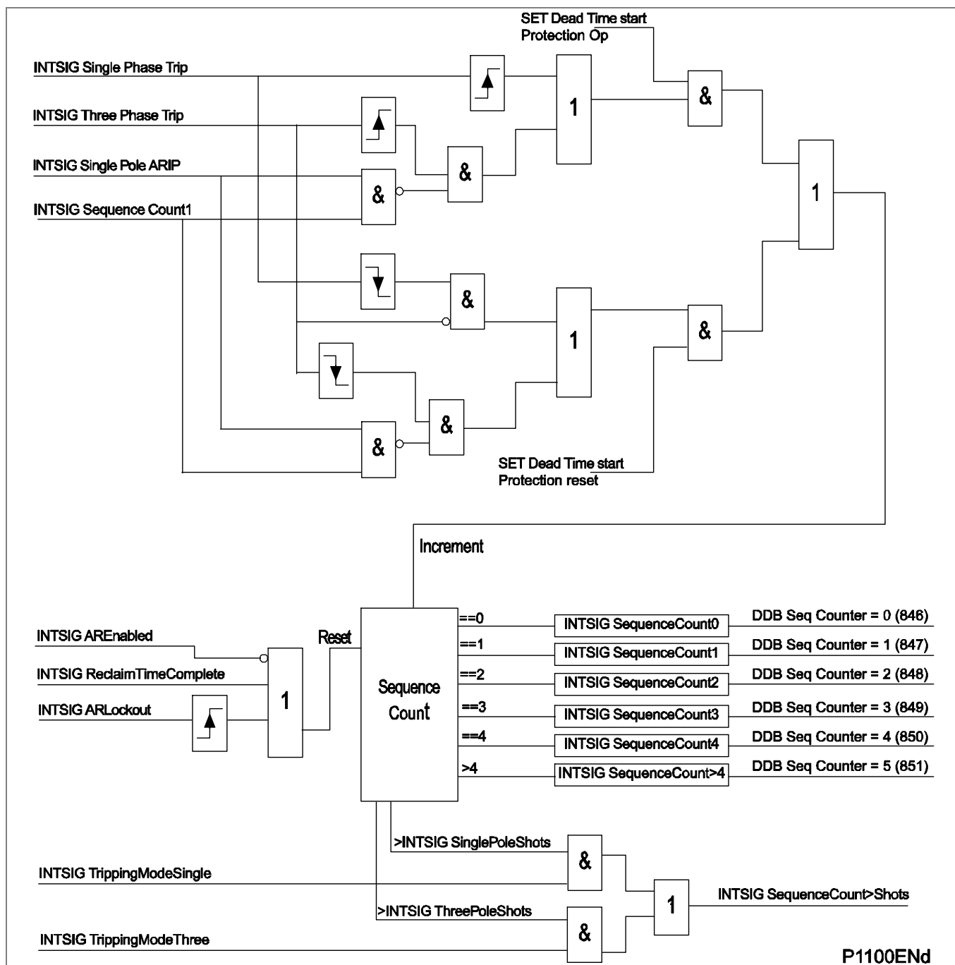
Figure 113 - Auto-reclose inhibit sequence count (P543/P545)
