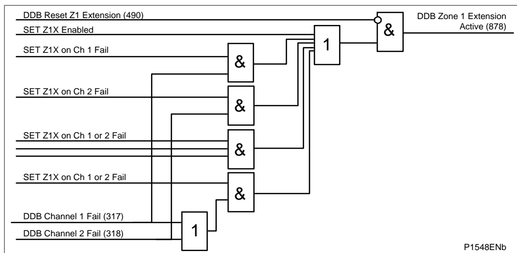
Figure 55 - Zone 1 extension
