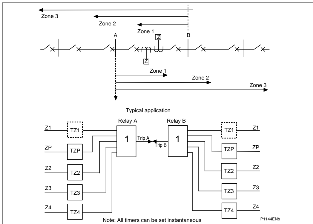
Figure 12 - Basic time stepped distance scheme
