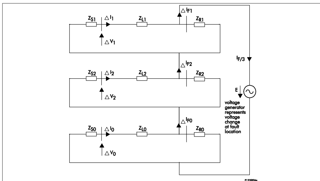
Figure 35 - Sequence networks connection for an internal A-N fault (Distance option only)
