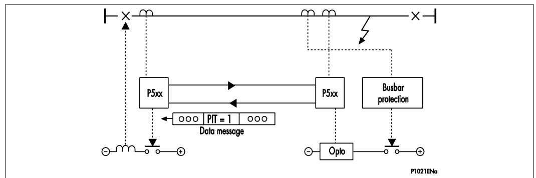
Figure 100 - Permissive intertrip
