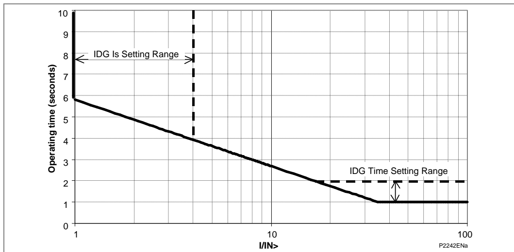
Figure 60 - IDG characteristic
