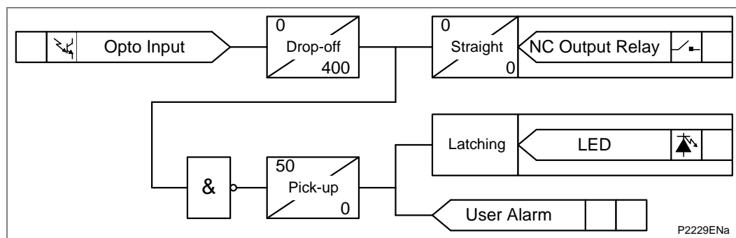
Figure 32 - PSL for TCS schemes 1 and 3
