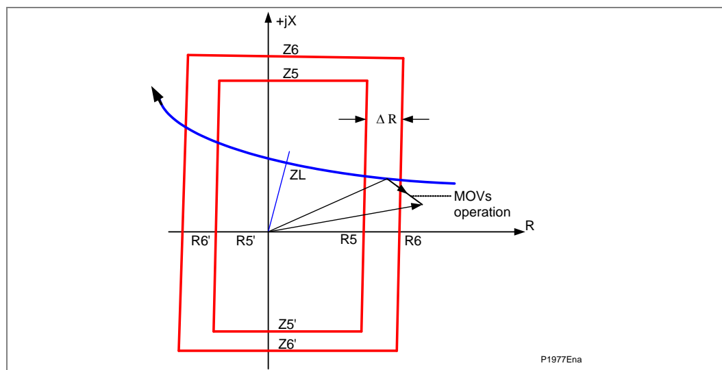
Figure 16 - Example of timer reset due to MOVs operation
