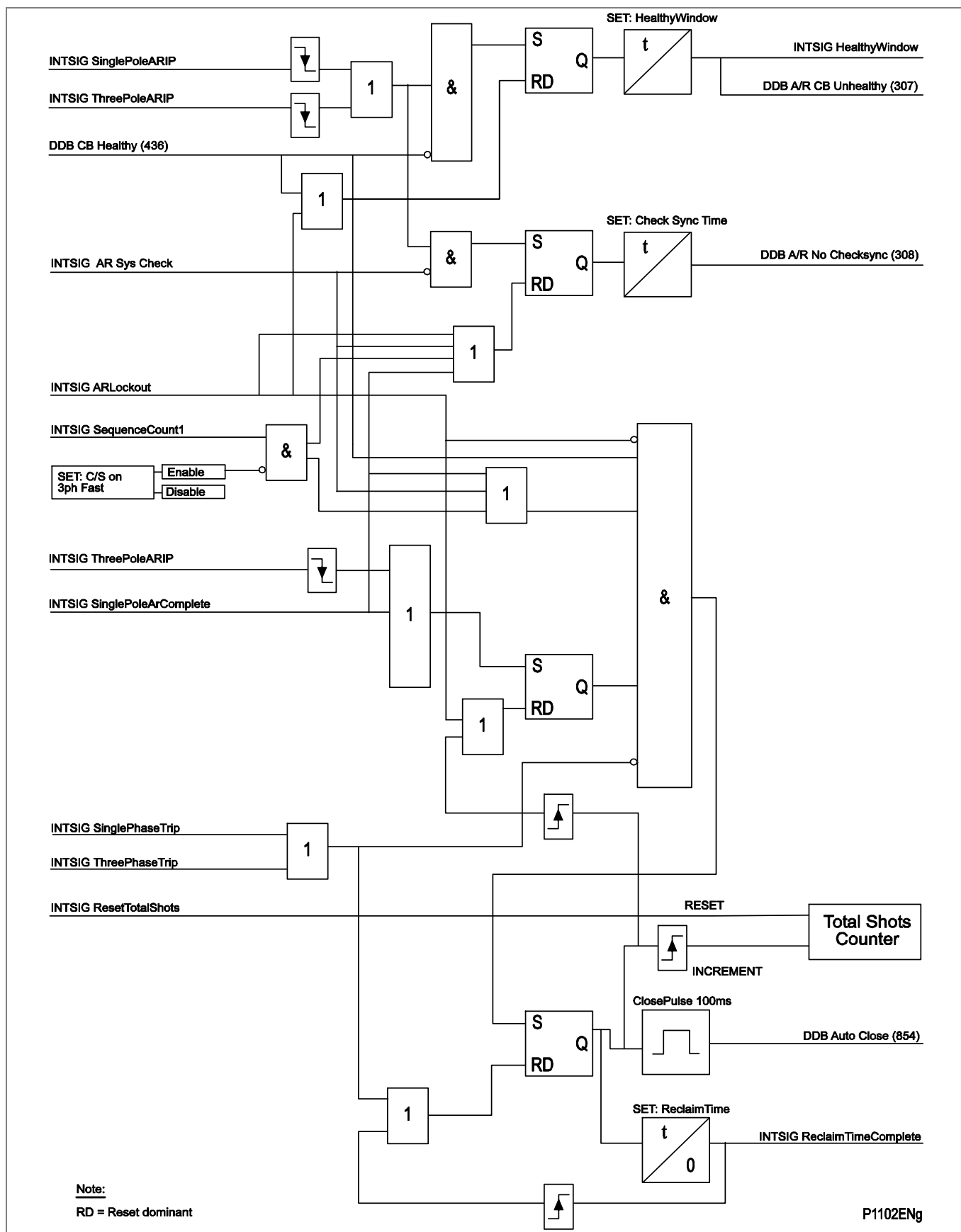
Figure 115 - Auto-reclose close
