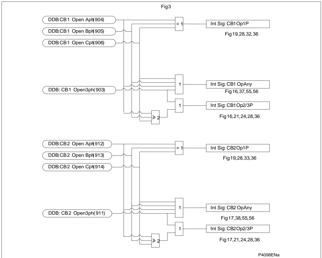
Figure AR-3 - CB1 &amp; CB2 Open 1P, 2P, 2/3P, Any
