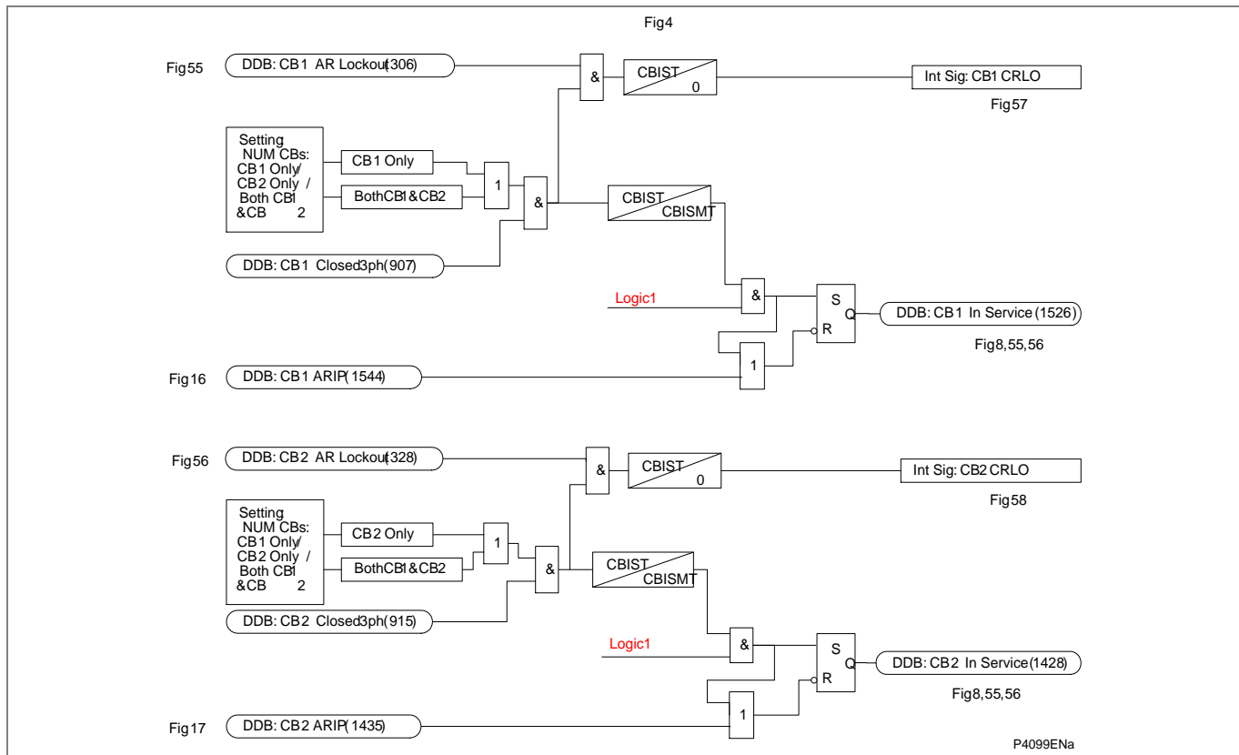
Figure AR-4 - Circuit breaker in service
