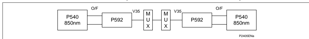
Figure 89 - P54x connection to P592
