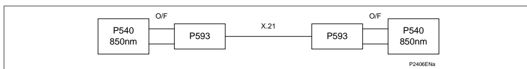
Figure 90 - P54x connection to P593
