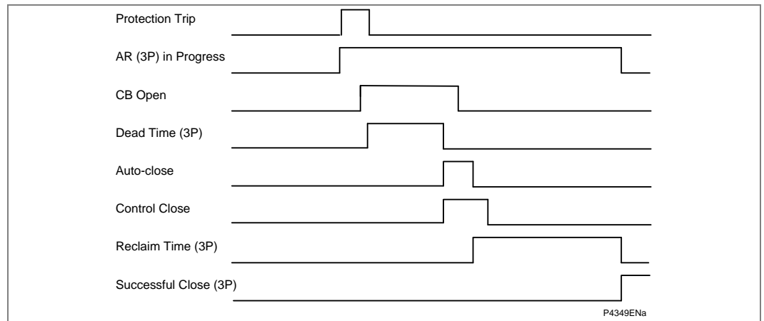
Figure 138 - Auto-reclose timing diagram – single breaker, single fault
