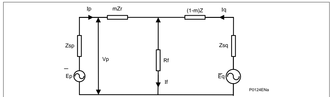
Figure 105 - Two-machine equivalent circuit
