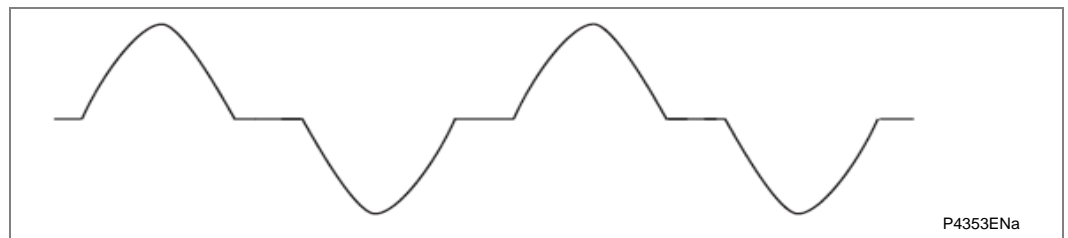
Figure 6 - Typical overflux current waveform
