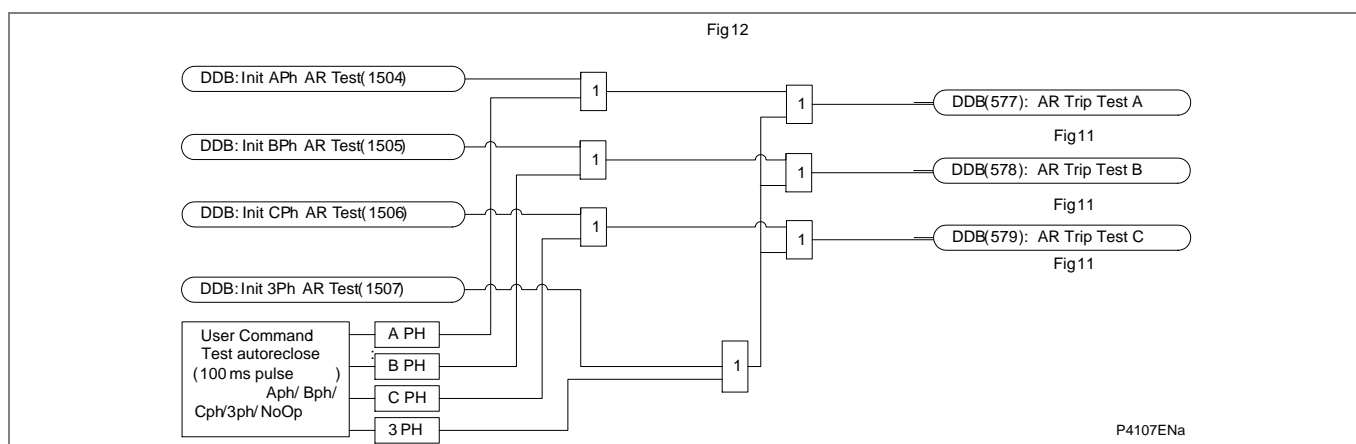
Figure AR-13 - Test trip &amp; AR initiation
