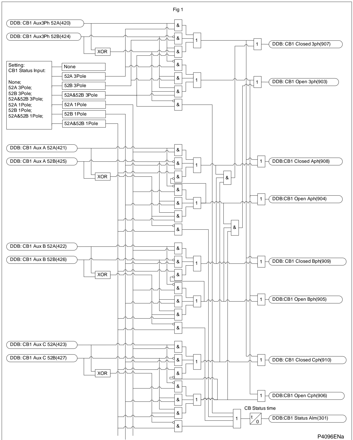
Figure AR-1 - Circuit breaker 1 - state monitor
