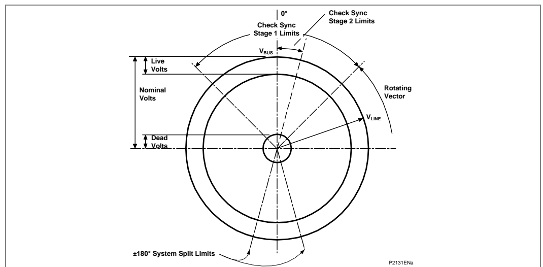
Figure 120 - Synchro check and synchro split functionality (P543/P545)
