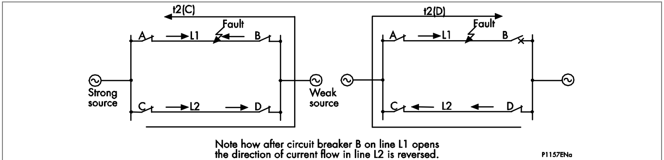
Figure 45 - Example of fault current reverse of direction
