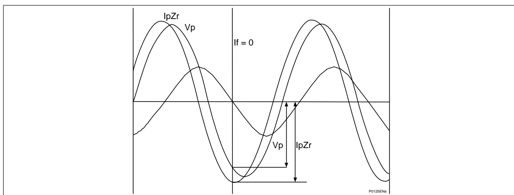
Figure 106 - Fault locator selection of fault current zero
