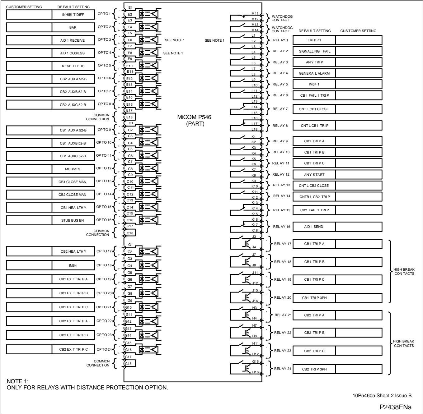
Figure 24 - P546 - 24 inputs/outputs default mapping – 16 standard & 8 high-break outputs
