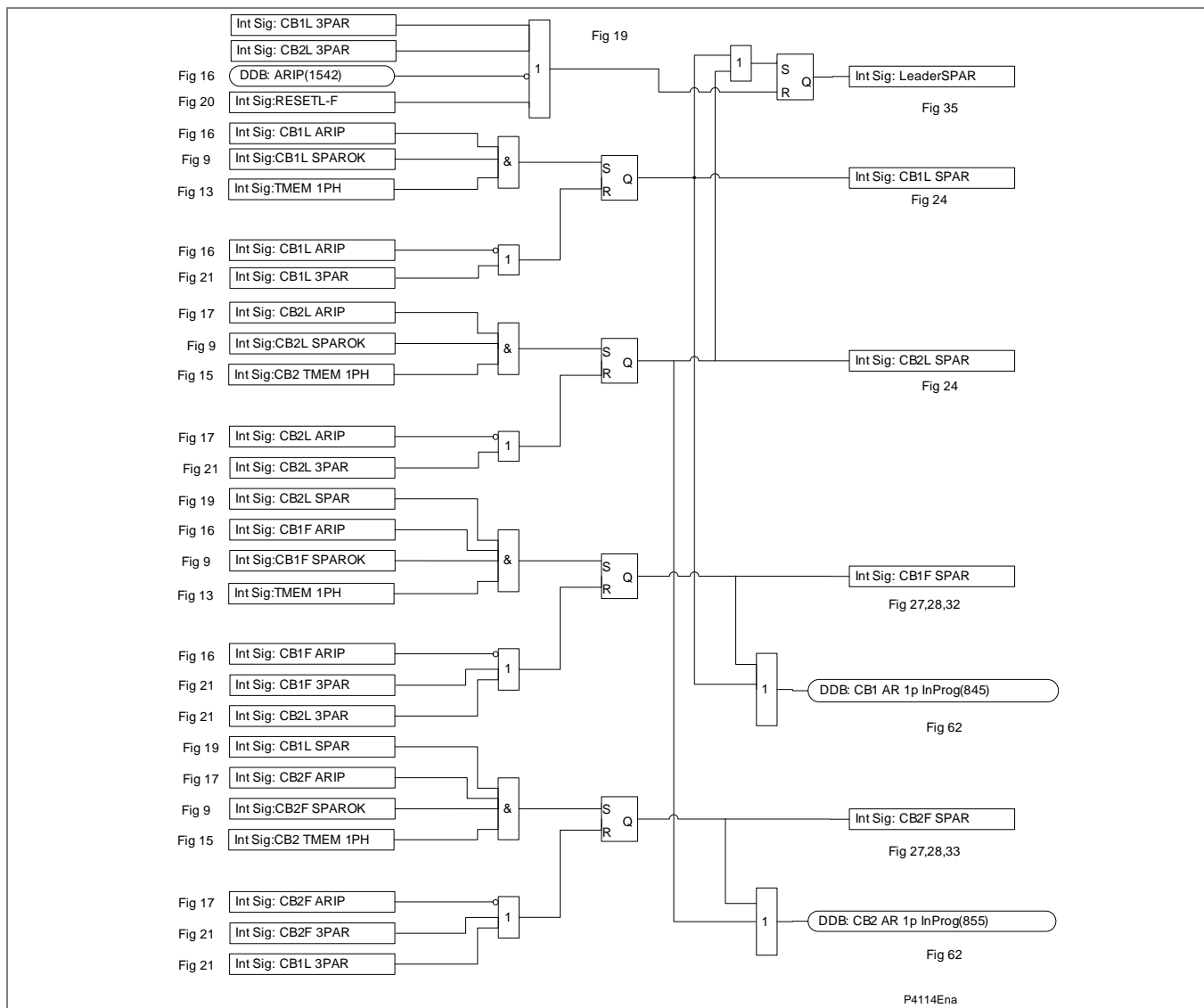
Figure AR-20 - Single phase AR cycle selection
