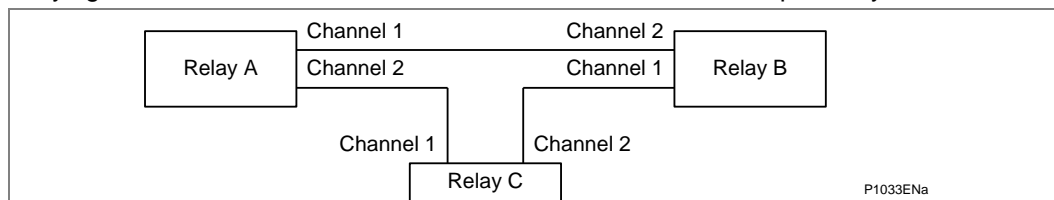
Figure 91 - 3-terminal system connection
