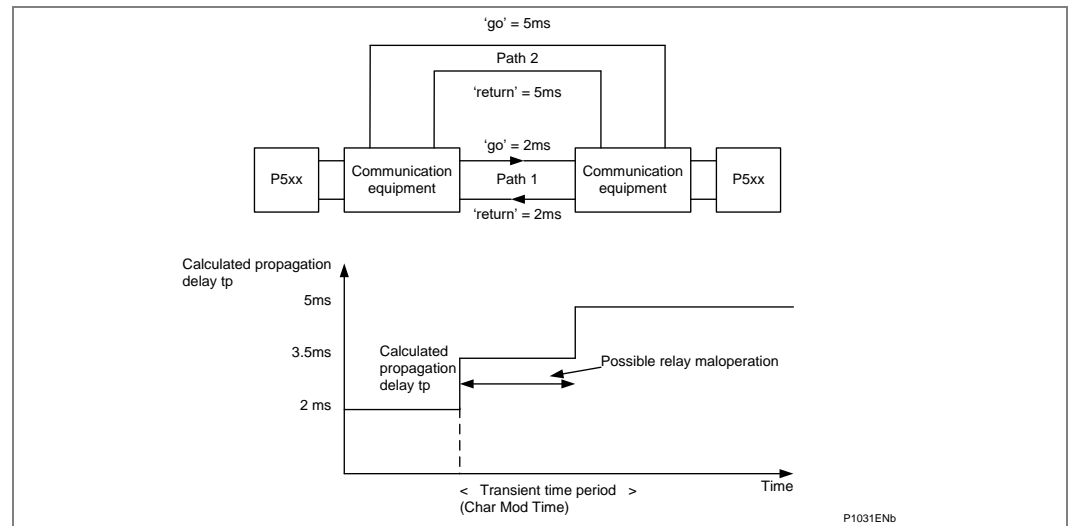
Figure 86 - Switched communication network
