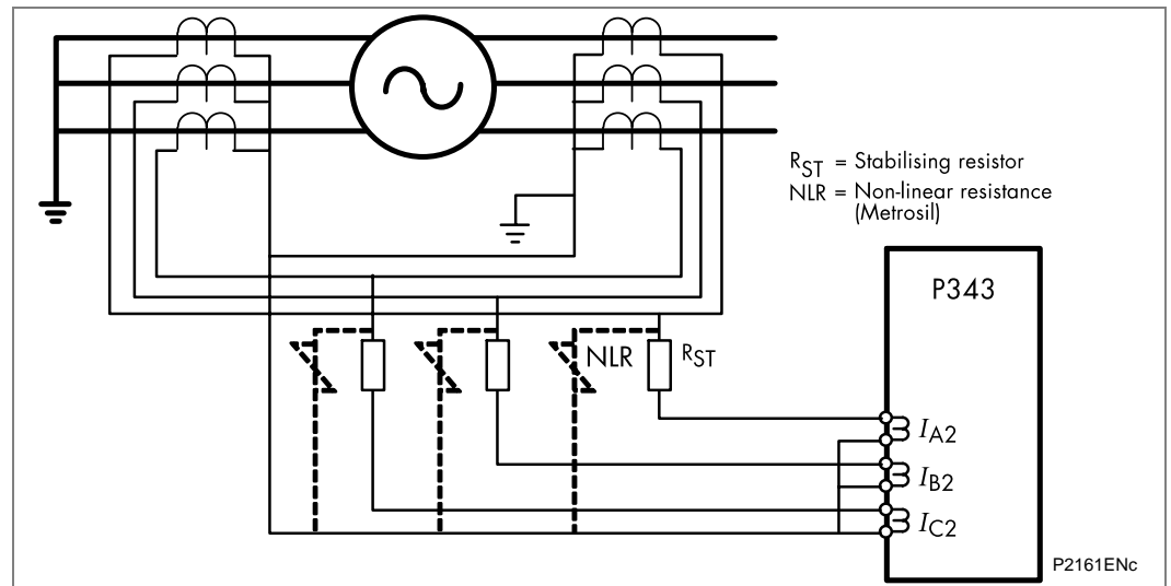
Figure 6 - Relay connections for high impedance differential protection
