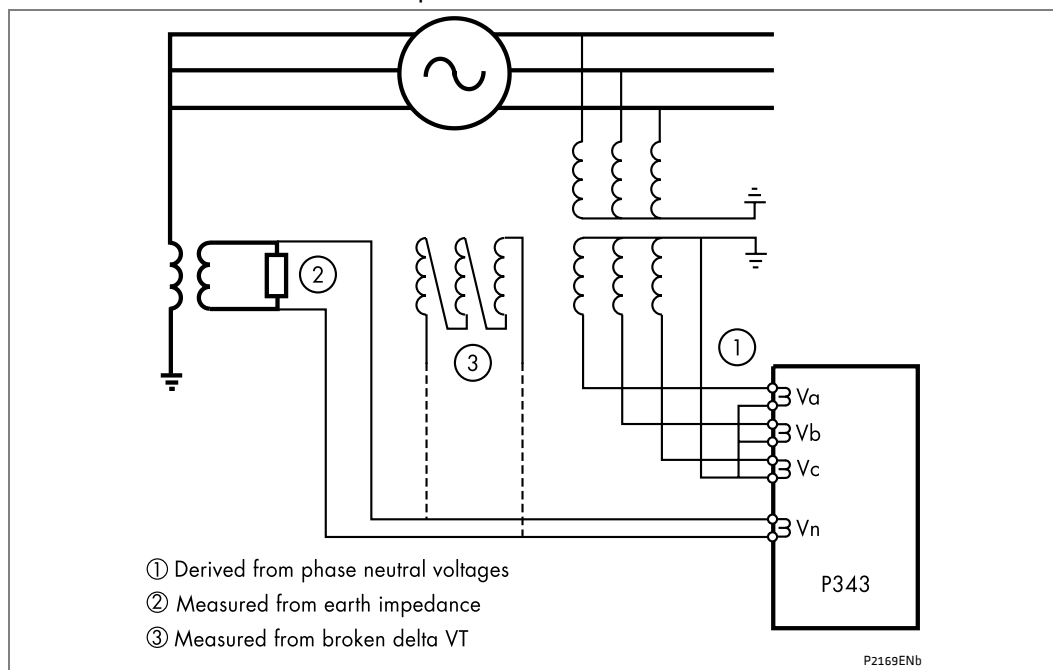
Figure 45 - Alternative relay connections for residual overvoltage/NVD protection
