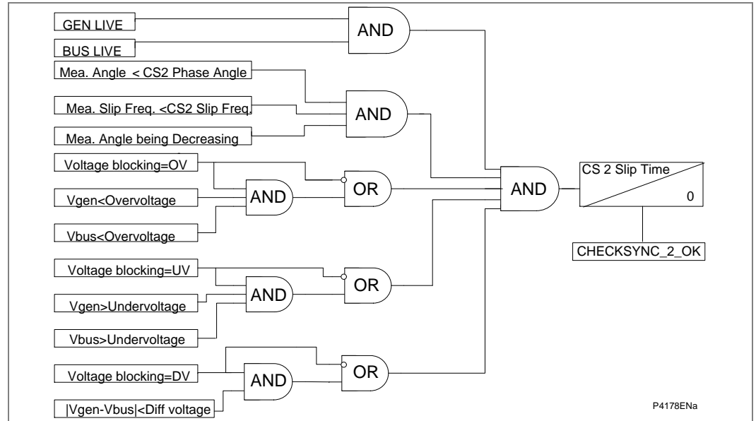
Figure 66 - Check synchron. 2 functional diagram
