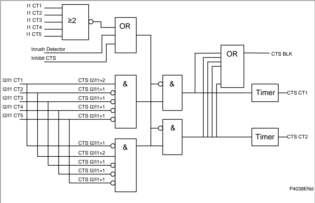
Figure 89 - Differential CTS logic diagram
