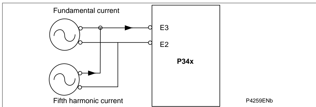
Figure 13 - Fifth-harmonic (1A and 60TE)
