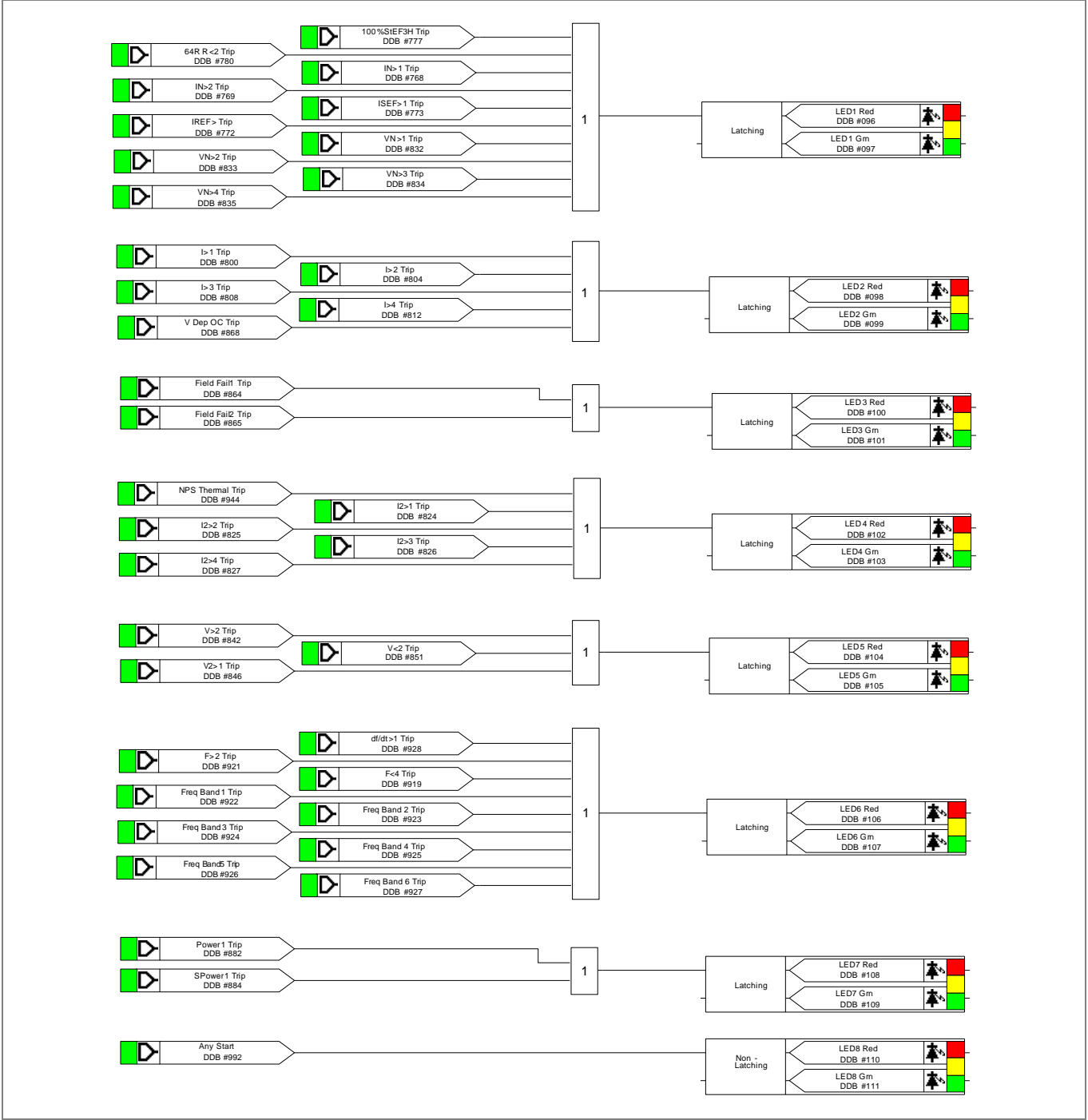
Figure 18 - LED output mapping
