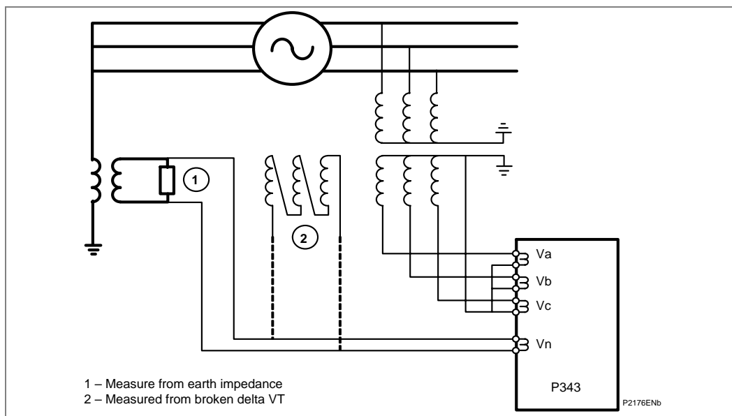
Figure 37 - Connection for 3rd harmonic undervoltage and overvoltage for 100% stator earth fault protection
