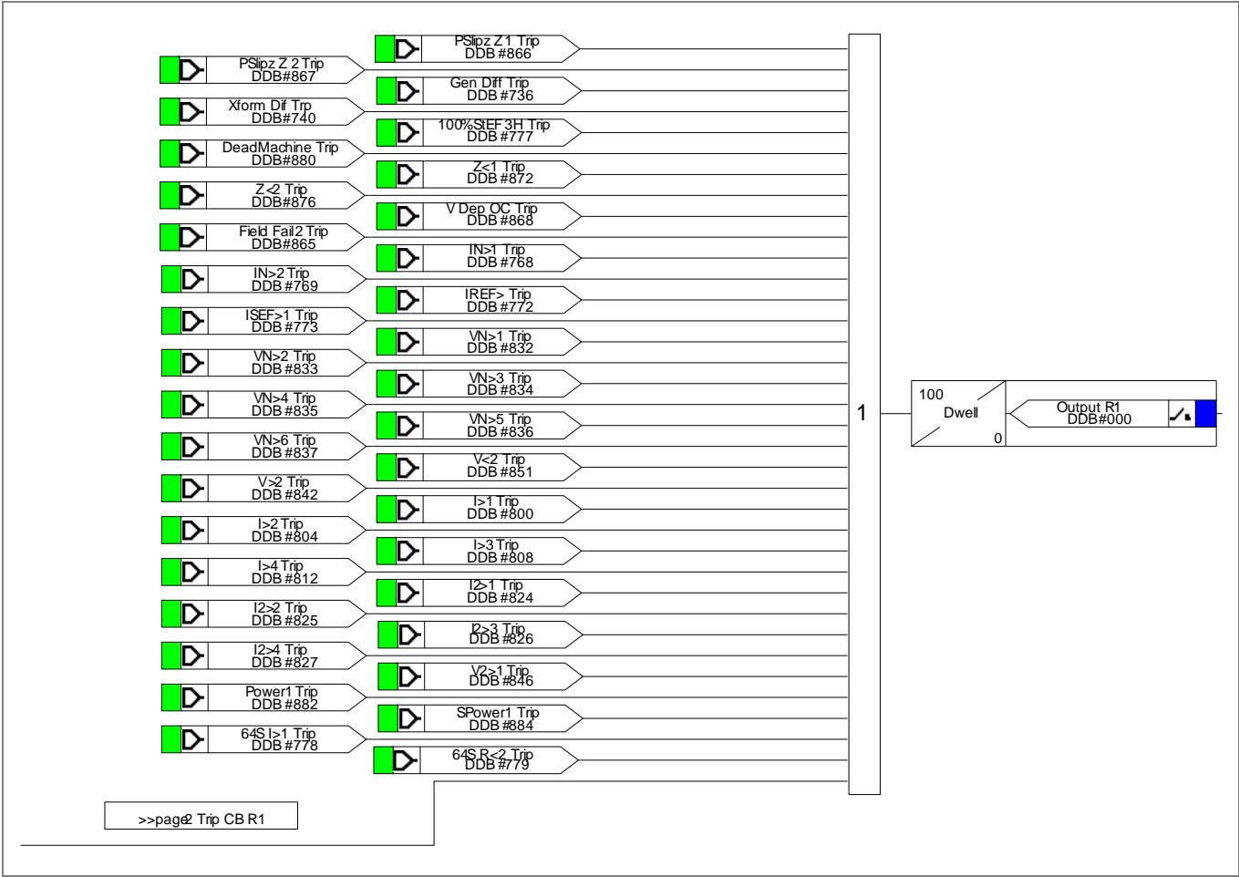
Figure 36 - Output relay R2 (Trip Prime Mover) mappings
