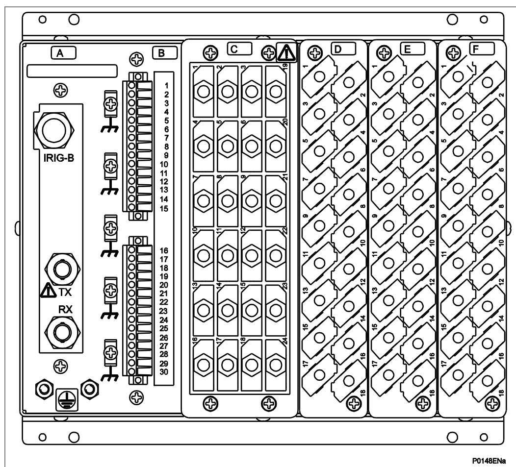
Figure 1 - Rear terminal blocks on size 40TE case
