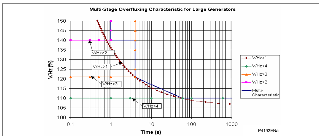
Figure 41 - Multi-stage overfluxing characteristic for large generators
