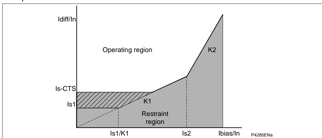
Figure 88 - CTS I_1 setting applied to the differential protection
