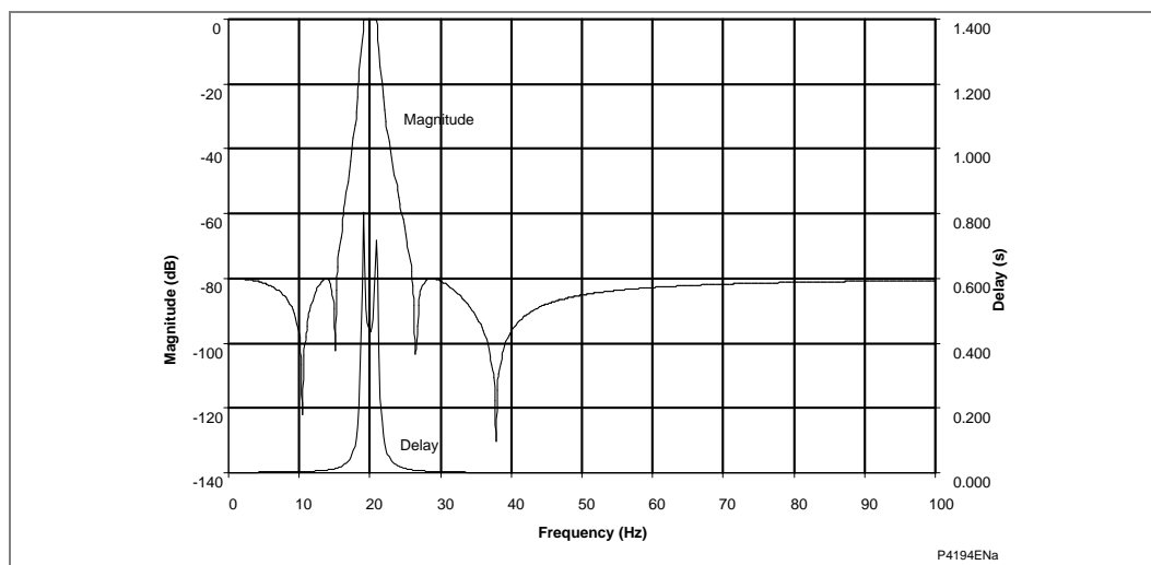
Figure 59 - 64S Elliptic 4th order band pass filter discrete frequency response
