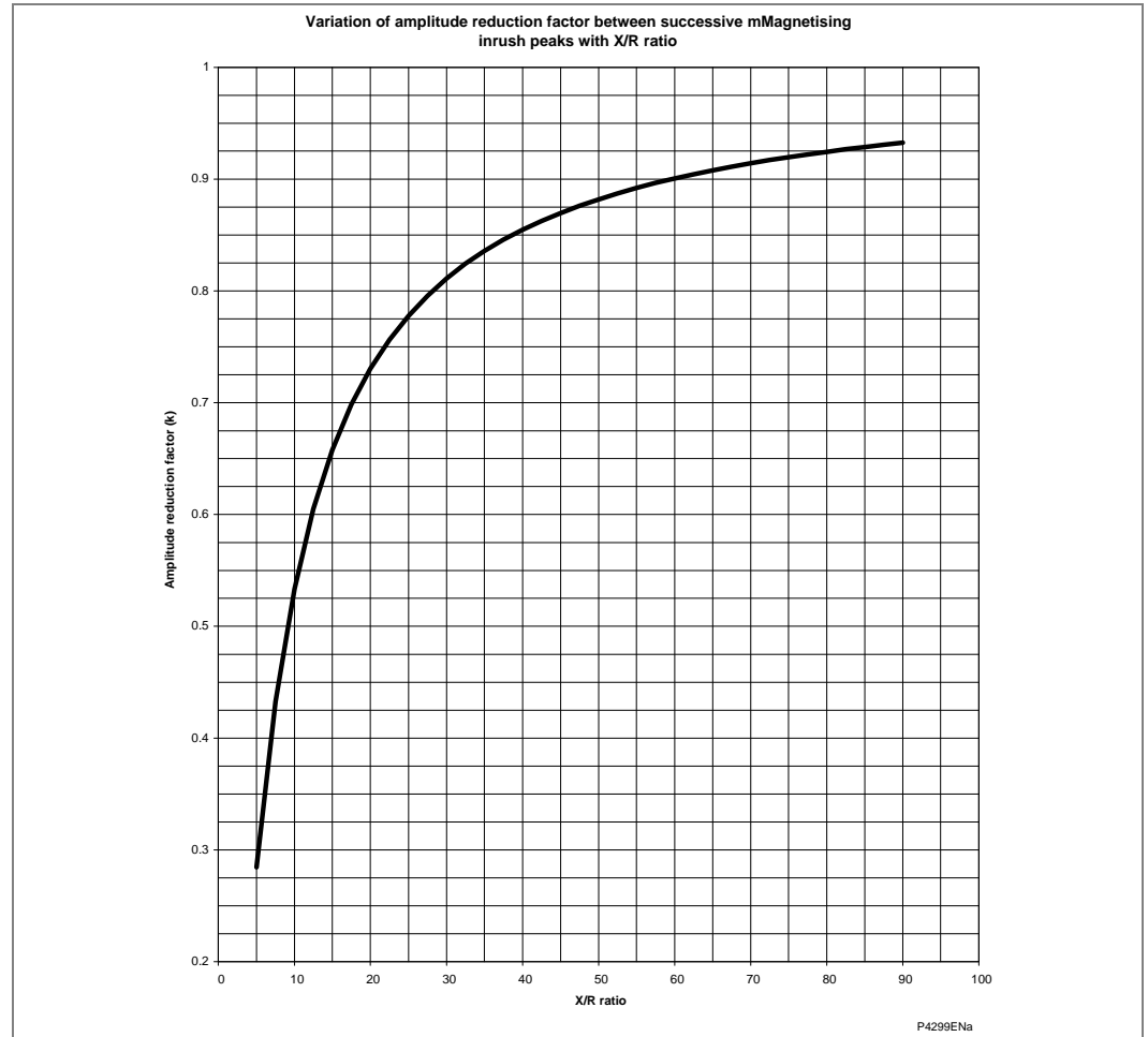
Figure 27 - Variation of amplitude reduction factor
