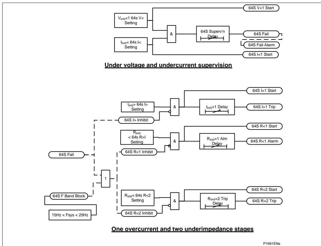
Figure 56 - 64S 100% stator earth fault logic diagram
