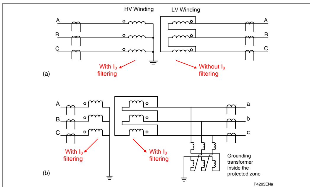
Figure 23 - Zero sequence current filtering
