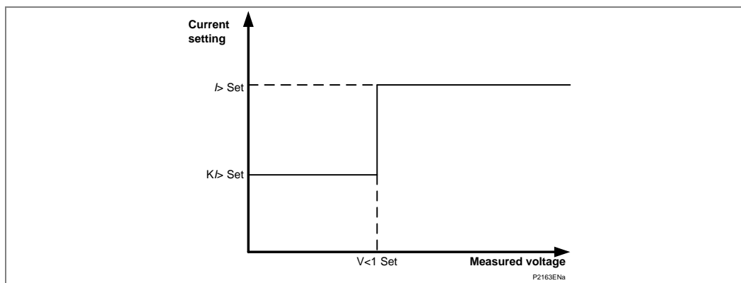
Figure 26 - Current pickup level for voltage controlled overcurrent protection
