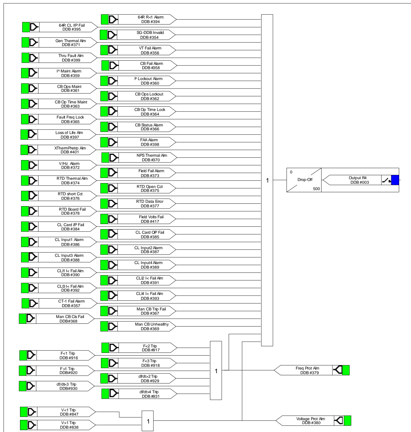
Figure 5 - Output relay R4 (General Alarm) mappings
