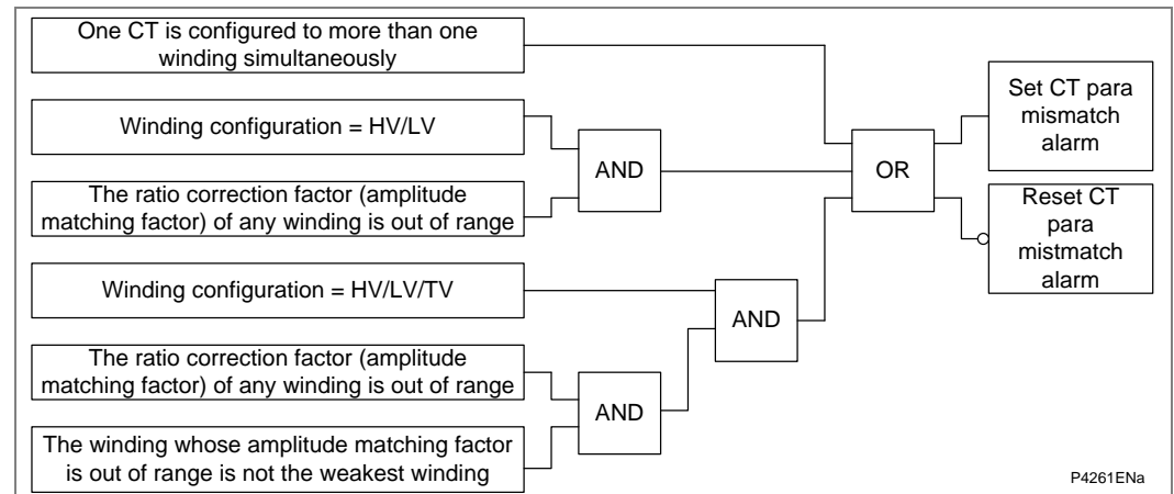
Figure 8 - CT parameter mismatch logic diagram
