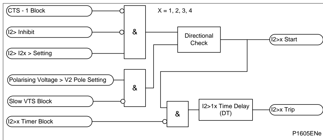
Figure 24 - Directionalizing the negative phase sequence overcurrent element
