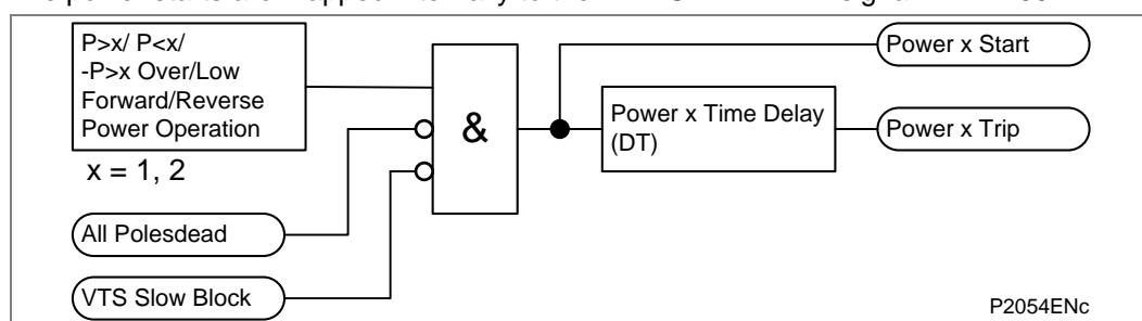
Figure 41 - Power logic diagram
