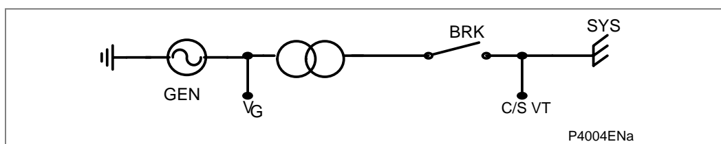
Figure 62 - Typical connection between system and generator-transformer unit
