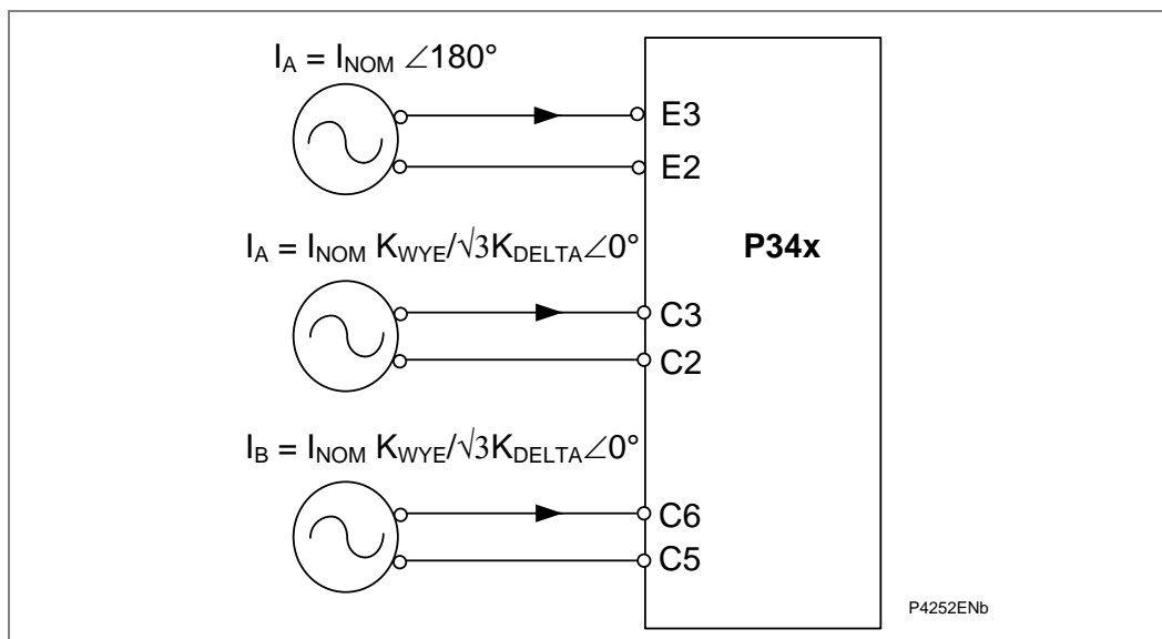
Figure 6 - Test equipment connection for a Yd1 transformer (1A and 60TE)
