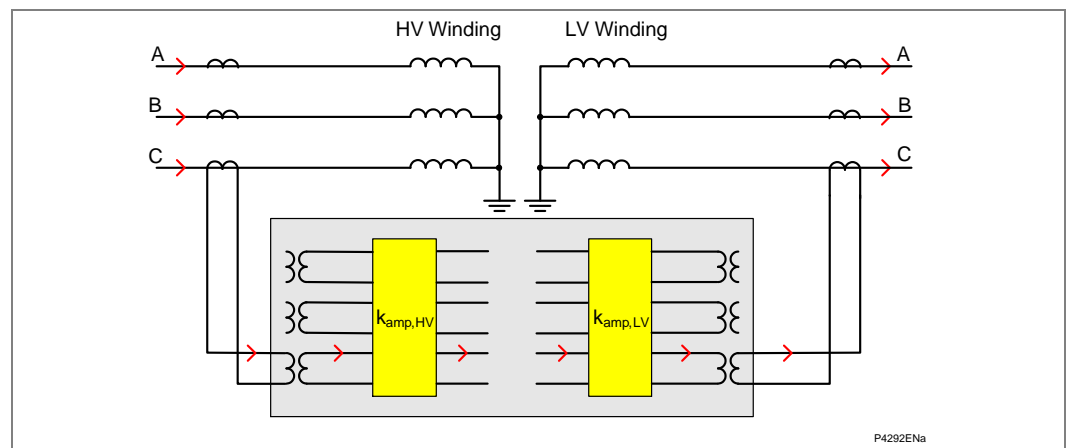
Figure 20 - Ratio correction or amplitude matching factor
