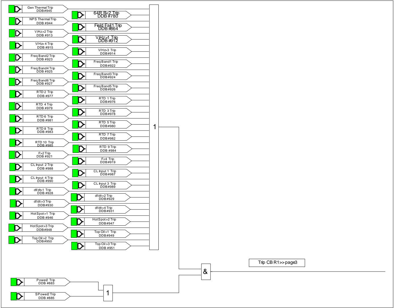
Figure 35 - Output relay R1 (Trip CB) mappings
