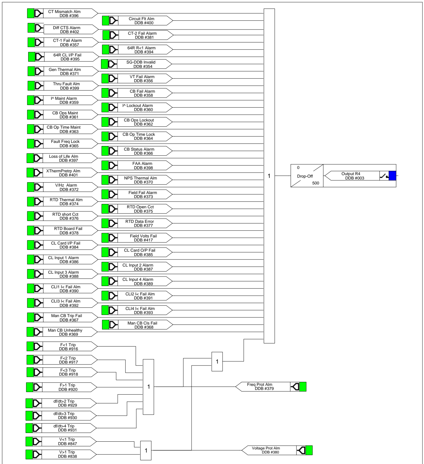
Figure 15 - Output relay mappings
