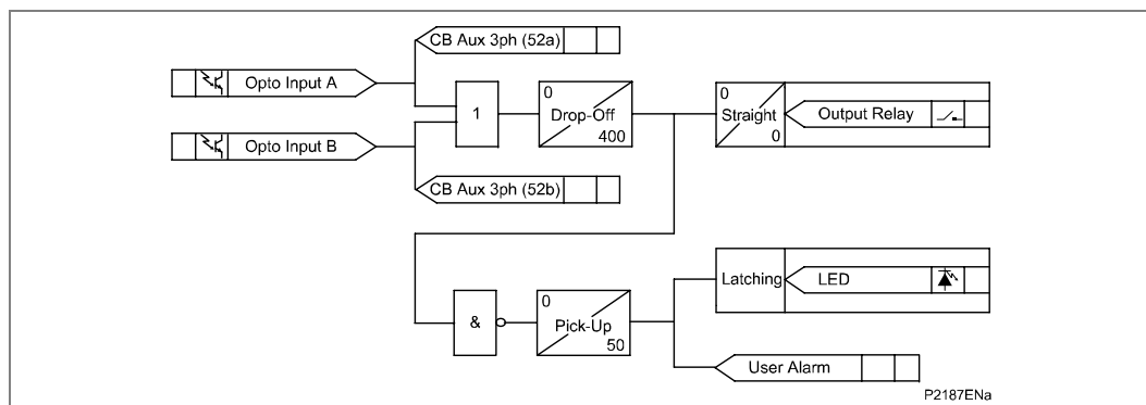
Figure 71 - PSL for TCS scheme 2
