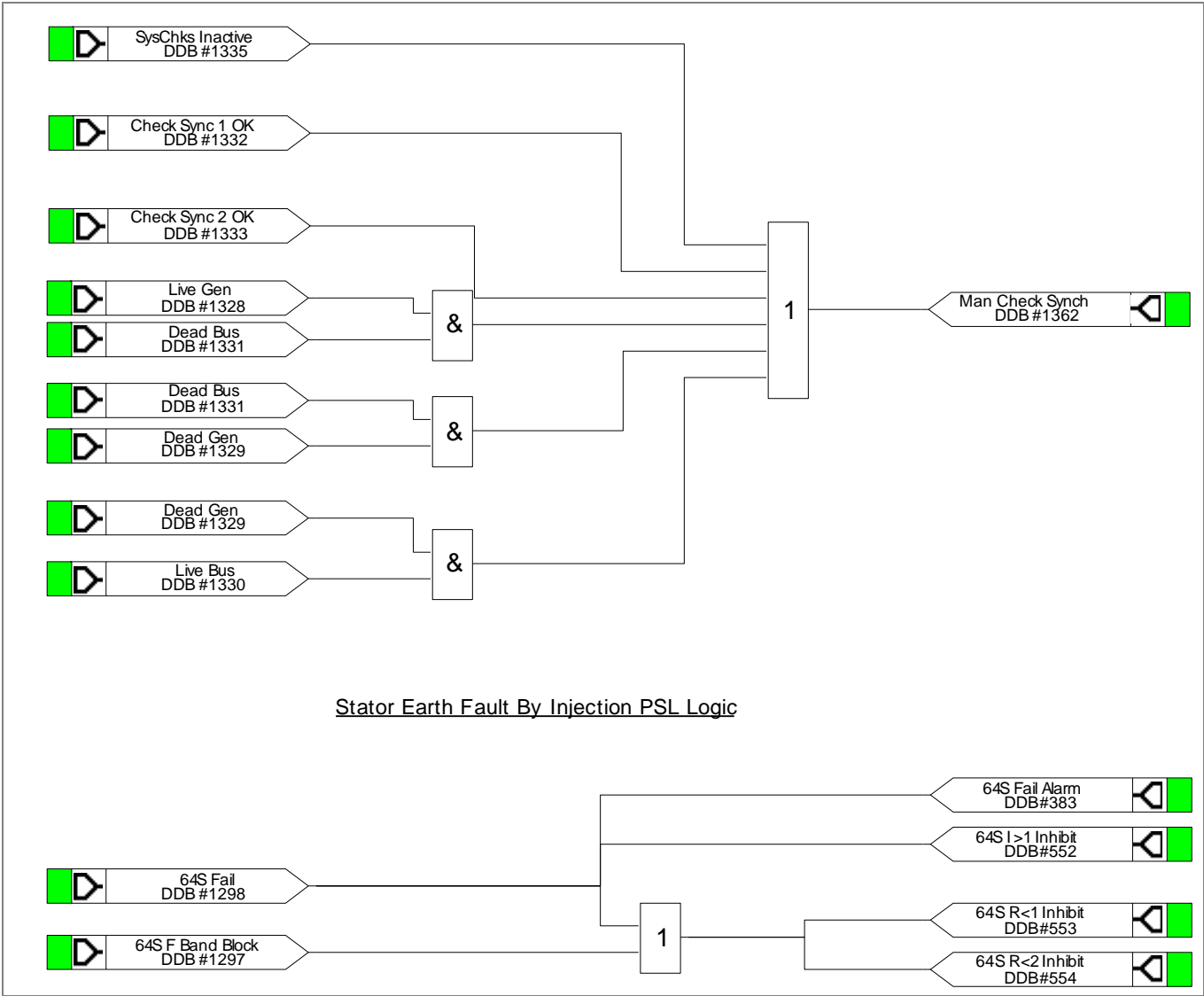
Figure 46 - Check synch and VOL monitor mapping
