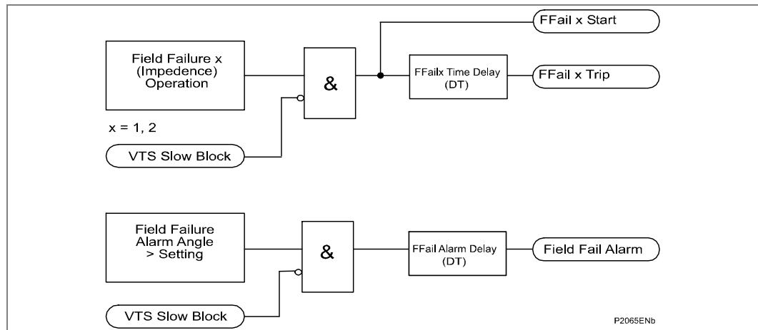
Figure 38 - Field failure logic diagram
