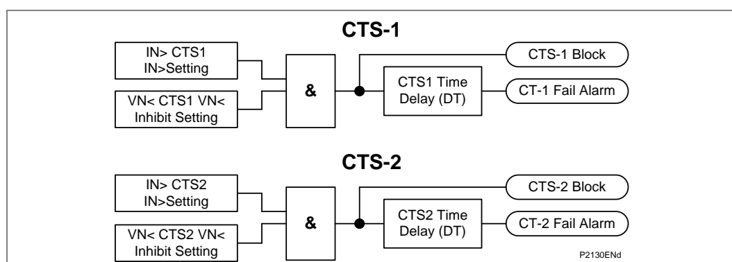
Figure 87 - CT supervision diagram
