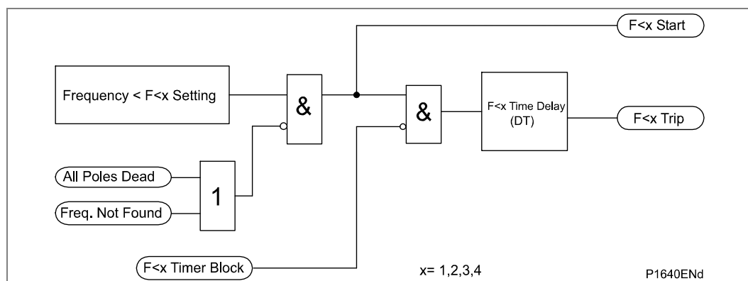
Figure 33 - Underfrequency logic (single stage)
