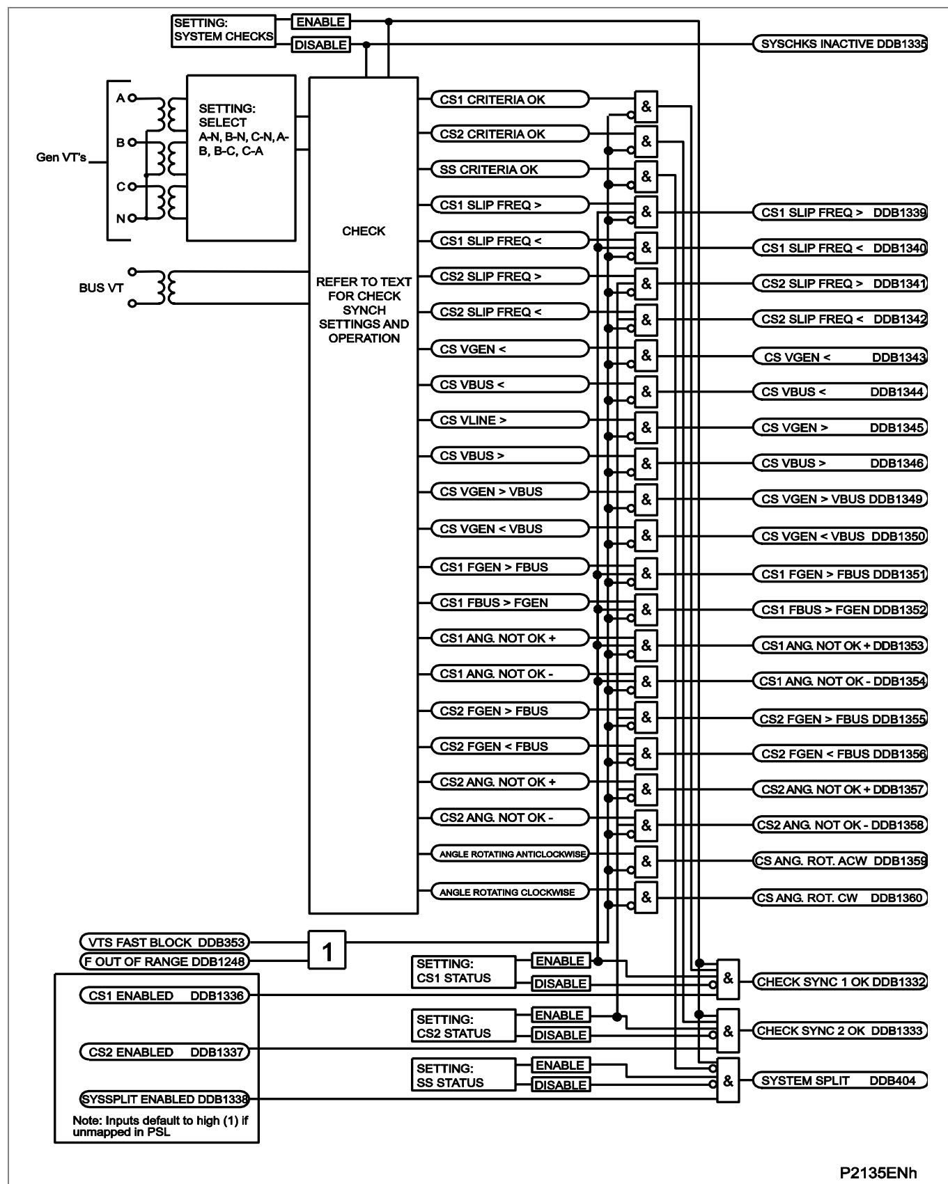
Figure 85 - System checks functional logic diagram
