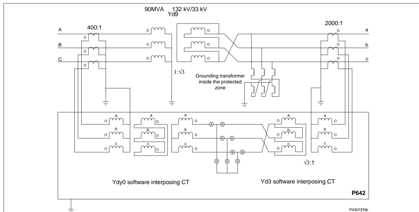
Figure 29 - P34x & P391 used to protect a Generator-Transformer unit
