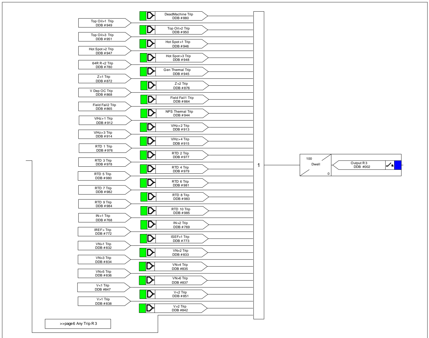
Figure 27 - Output relay mappings
