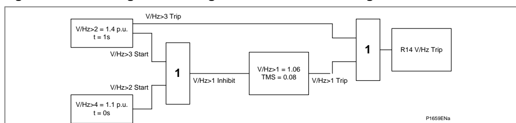
Figure 44 - Scheme logic for small generator multi-stage overfluxing characteristic
