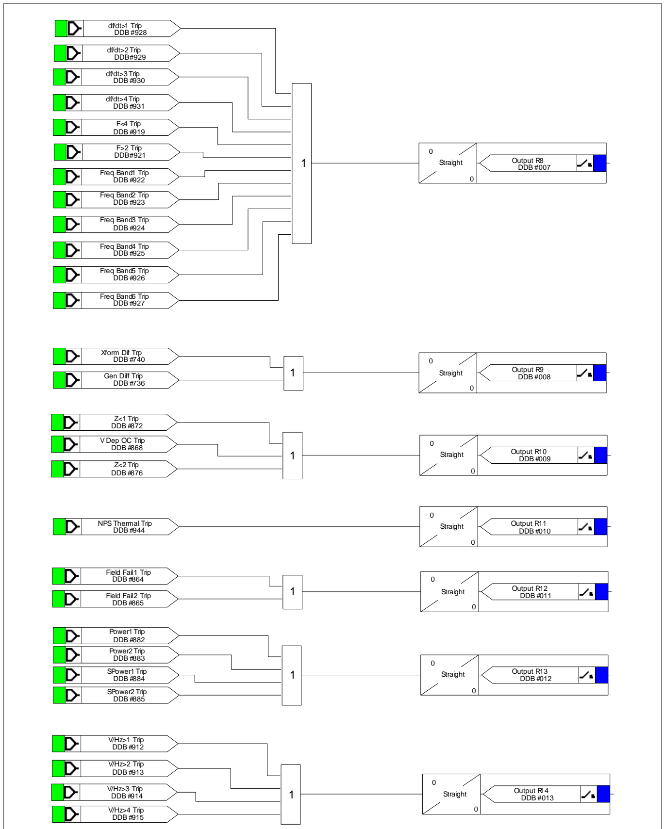
Figure 43 - Output relay mappings
