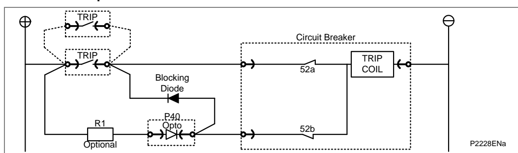
Figure 68 - TCS scheme 1
