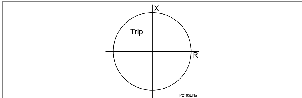
Figure 28 - Under impedance element tripping characteristic
