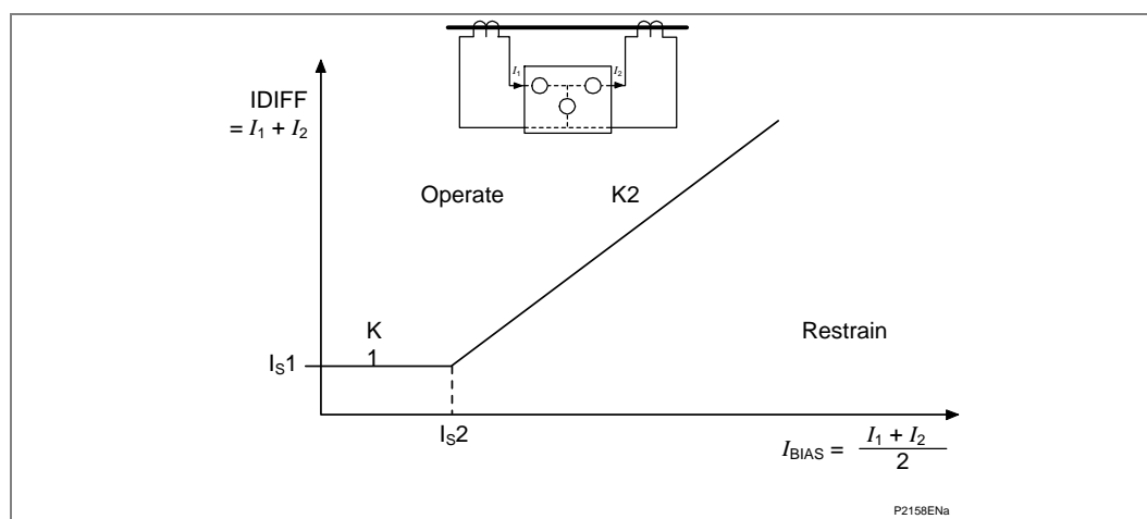
Figure 3 - Biased differential protection operating characteristic
