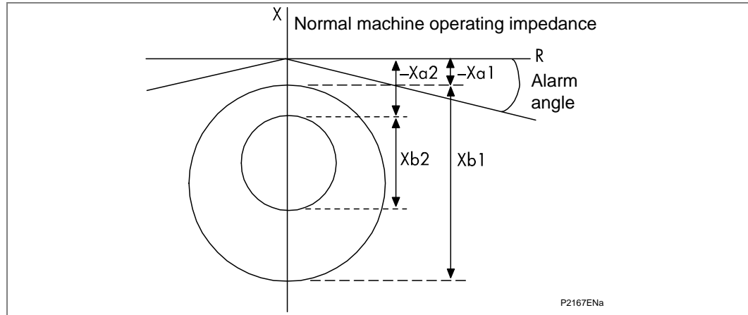
Figure 37 - Field failure protection characteristics
