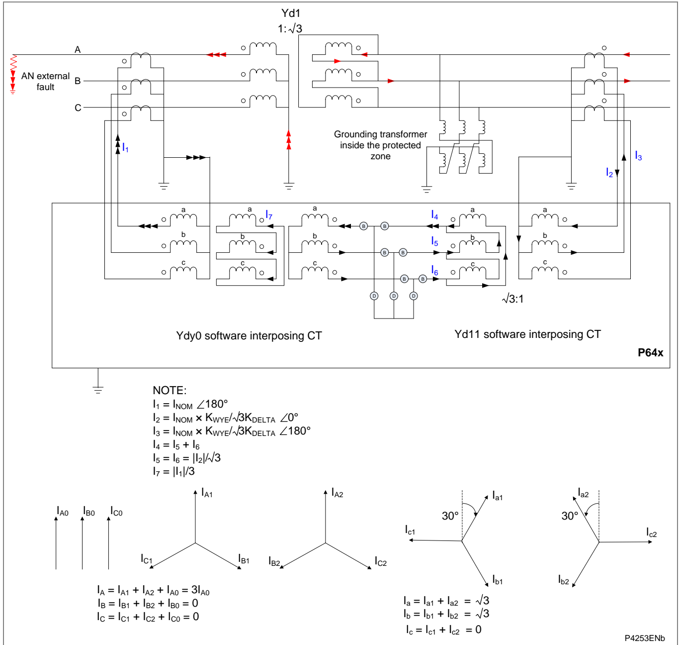
Figure 7 - Yd9 configuration AN external fault current distribution
