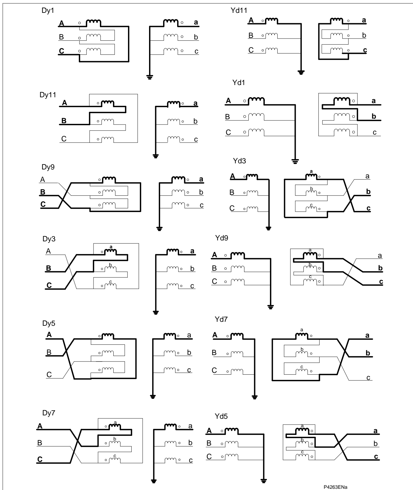
Figure 12 - Yd or Dy transformer connections
