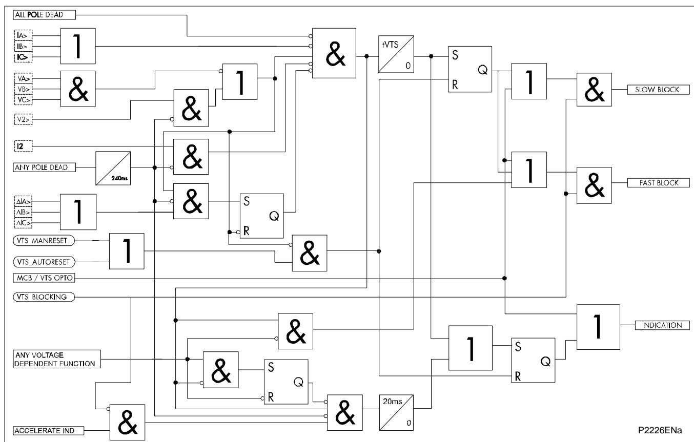
Figure 86 - VTS logic
