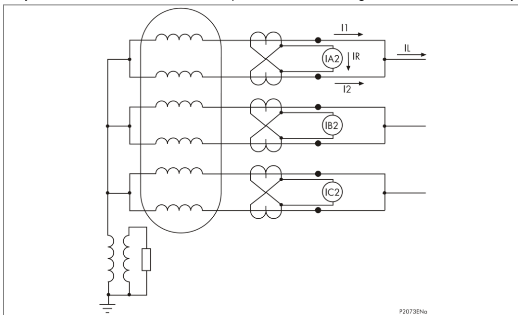
Figure 9 - Generator interturn protection using separate CTs
