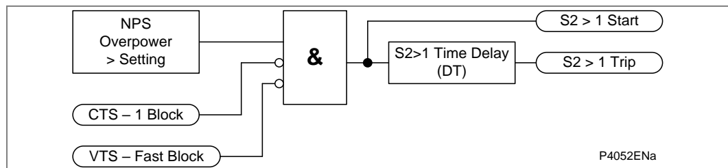
Figure 20 - NPS overpower logic diagram
