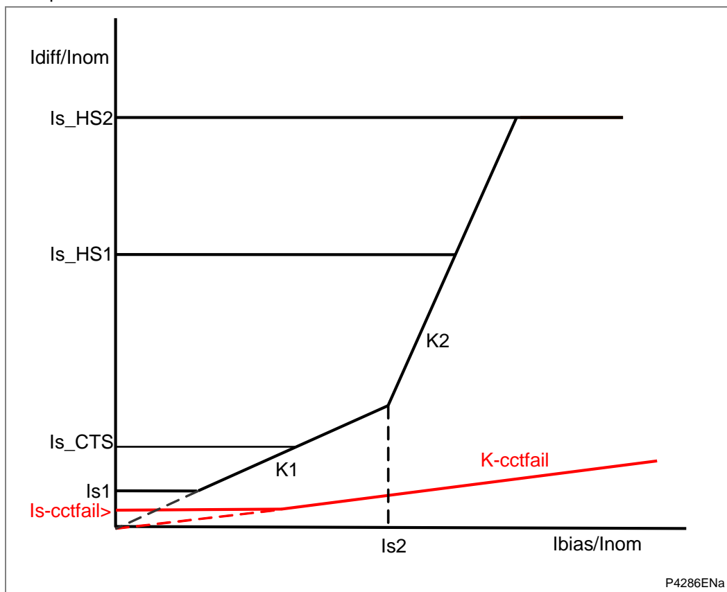
Figure 90 - Circuitry fail alarm fault characteristic
