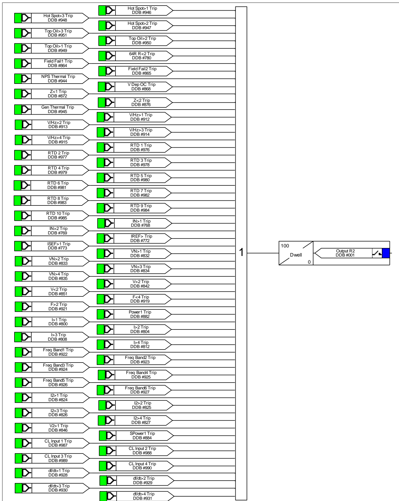
Figure 3 - Output relay R2 (Trip Prime Mover) mappings
