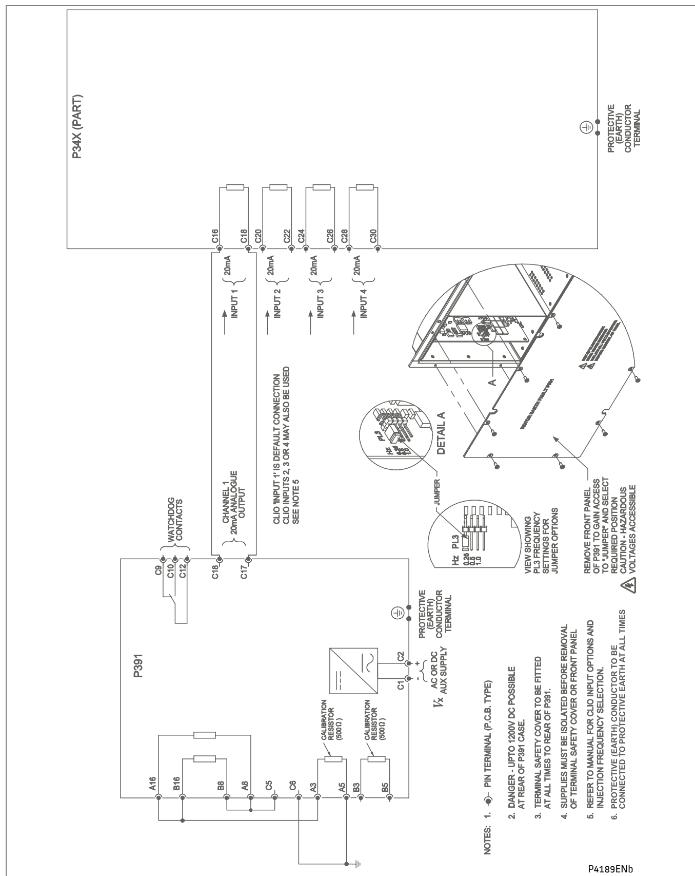
Figure 15 - Calibration circuit for the 64R rotor earth fault protection
