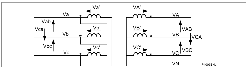
Figure 63 - Typical connection between system and generator-transformer unit Transformer connection
