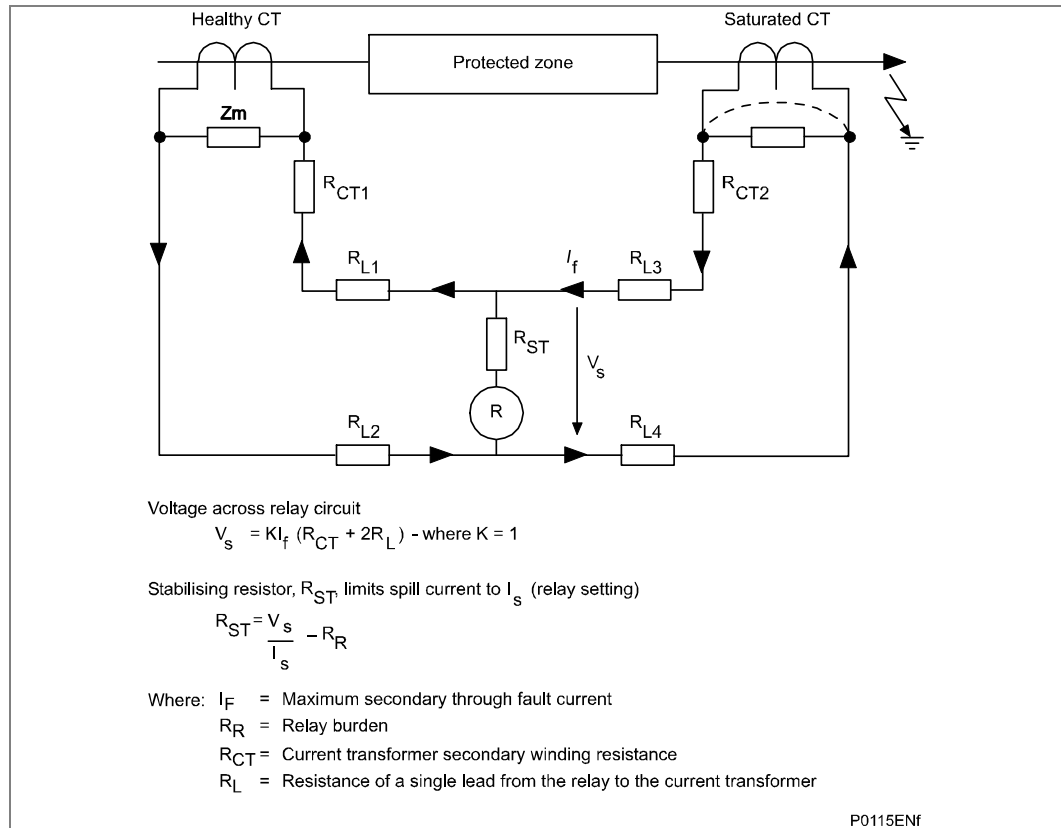
Figure 52 - Principle of high impedance differential protection
