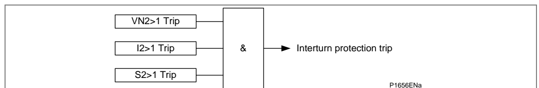
Figure 15 - Interturn protection interlocking PSL logic
