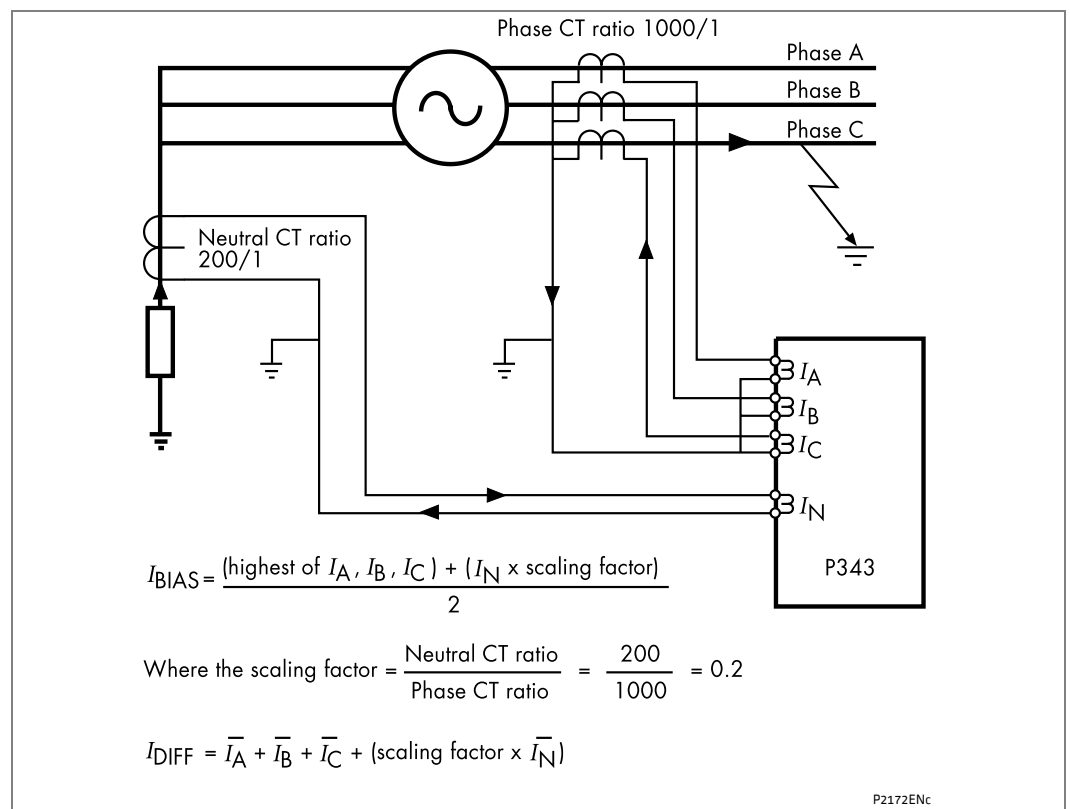
Figure 51 - Neutral scaling for biased REF protection
