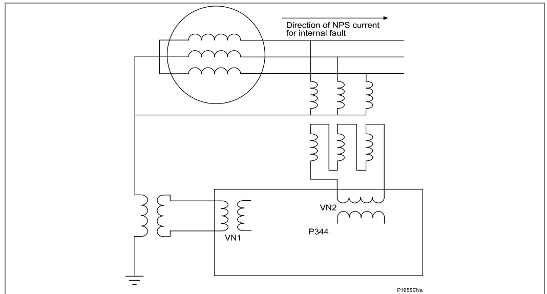
Figure 14 - Interturn protection (VN2) and earth fault protection (VN1) by zero sequence voltage measurement
