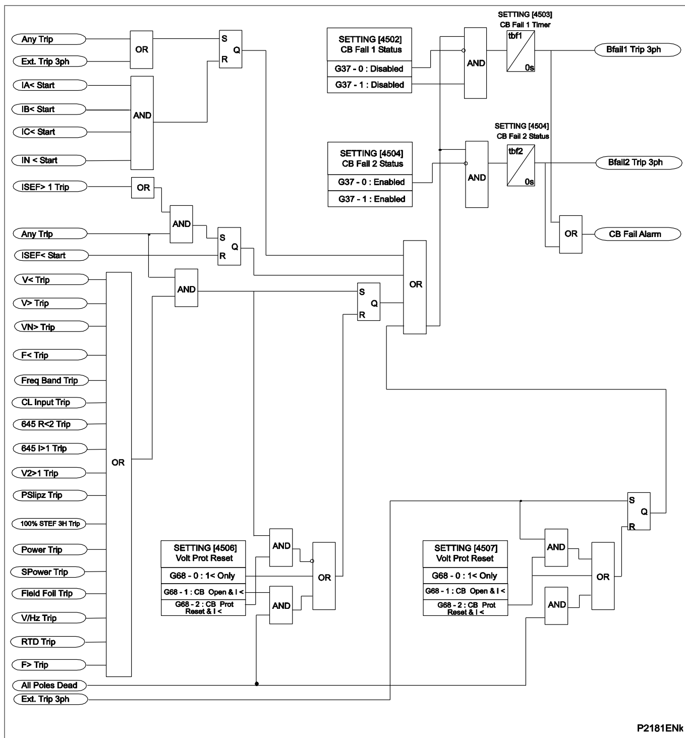
Figure 74 - CB fail logic
