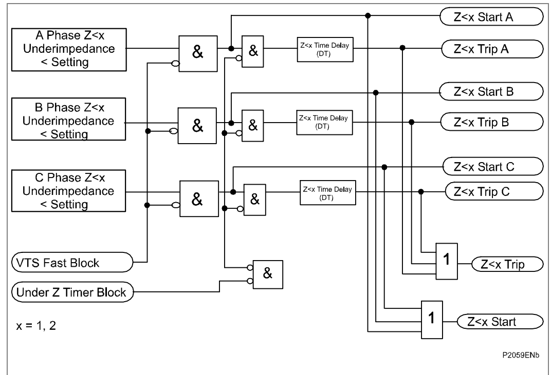
Figure 29 - Under impedance logic diagram
