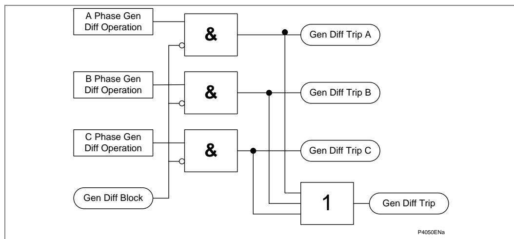
Figure 2 - Generator differential logic diagram
