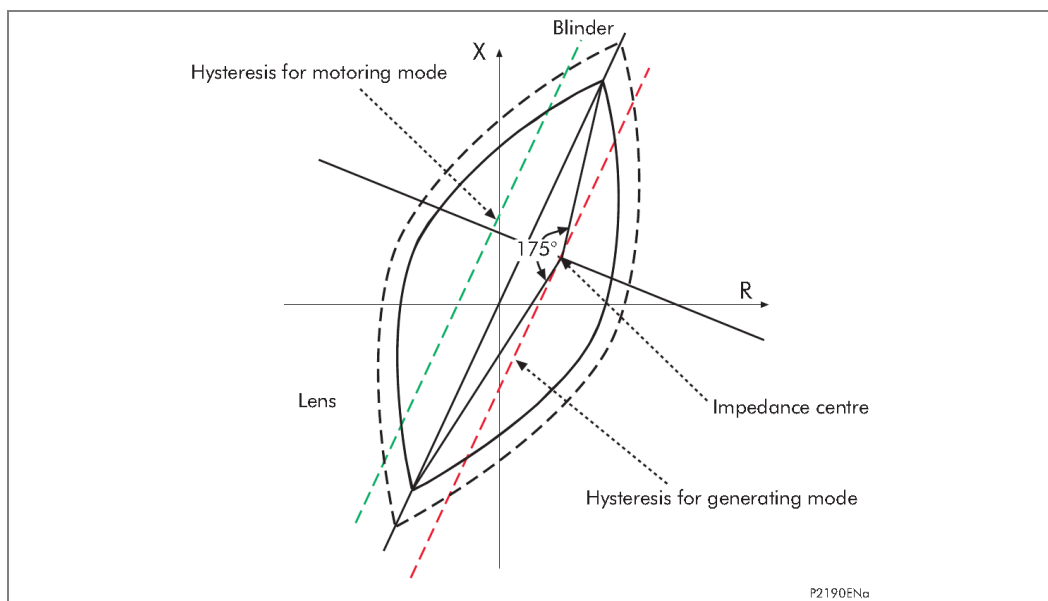
Figure 1 - Hysteresis of the pole slipping characteristic
