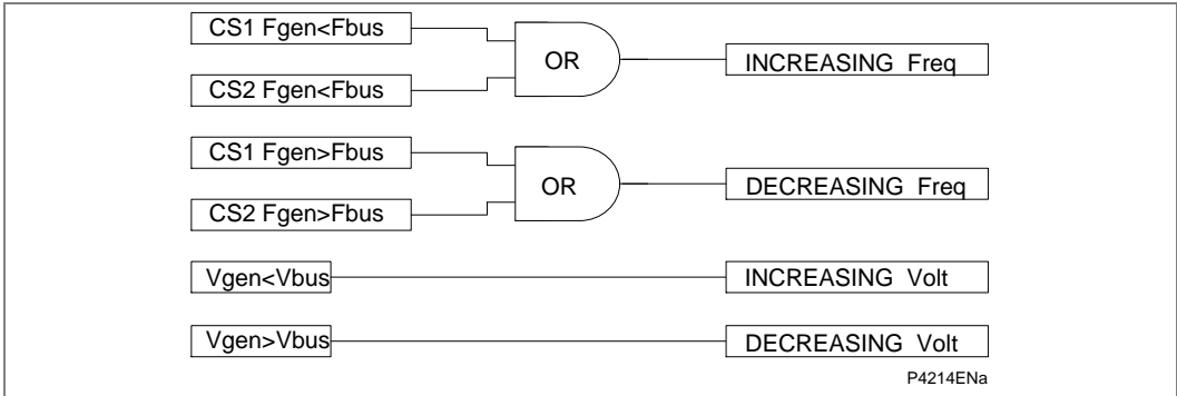
Figure 67 - Freq/Volt control functional diagram
