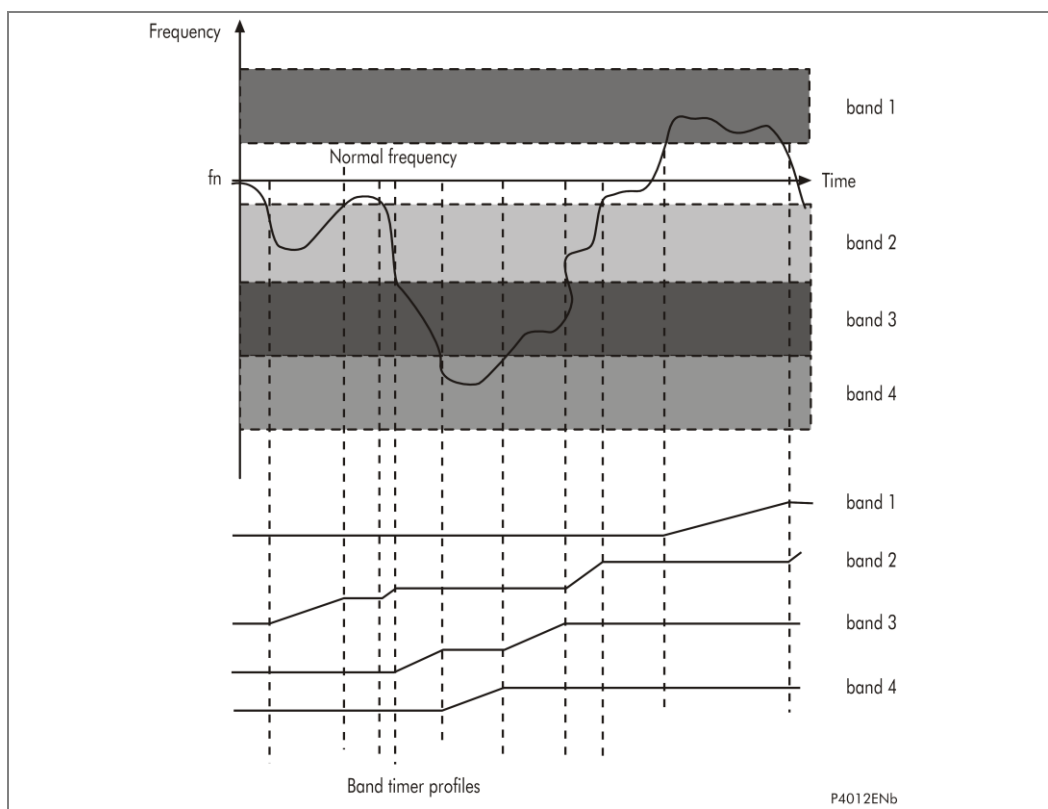
Figure 35 - Generator abnormal frequency protection
