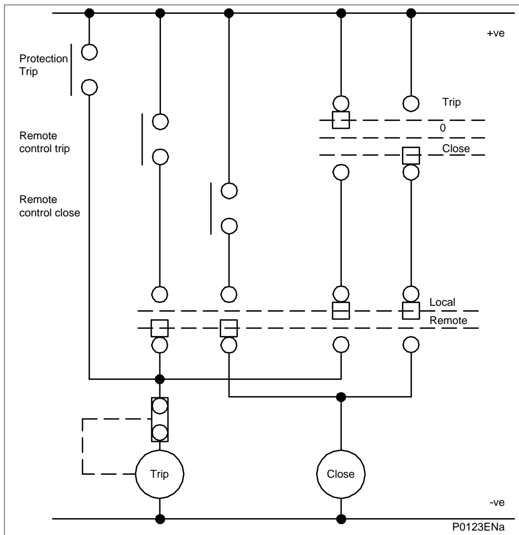
Figure 93 - Remote control of circuit breaker
