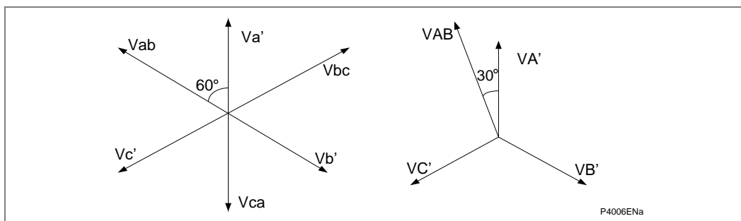
Figure 64 - Transformer vector diagram
