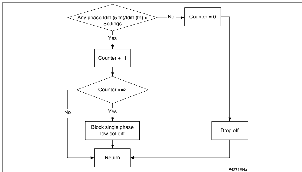
Figure 18 - Overfluxing restraint
