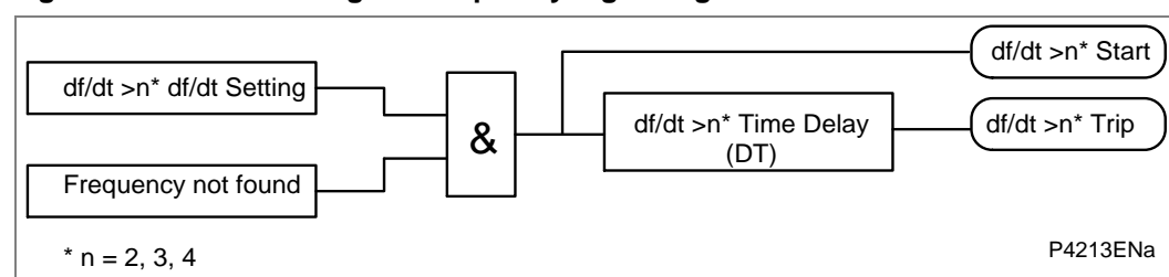
Figure 62 - Rate of change of frequency logic diagram for df/dt>2, 3, 4
