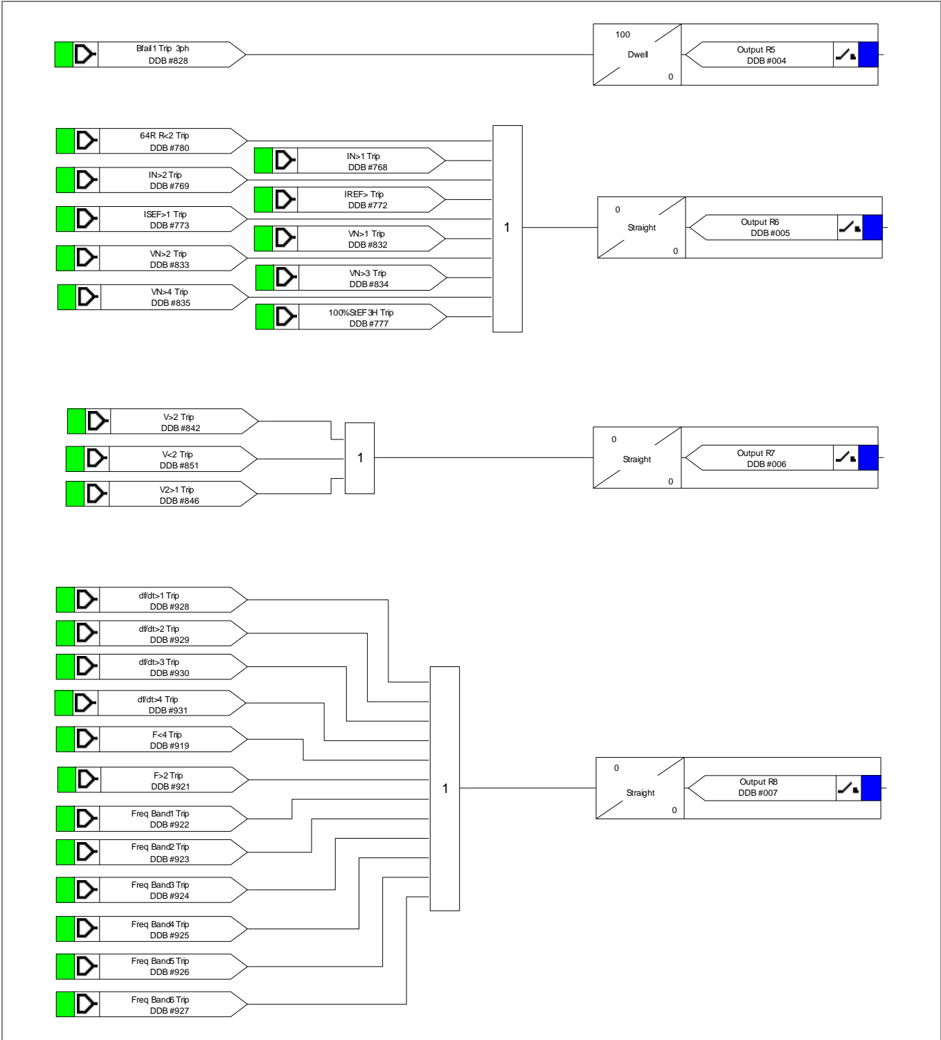
Figure 16 - Output relay mappings
