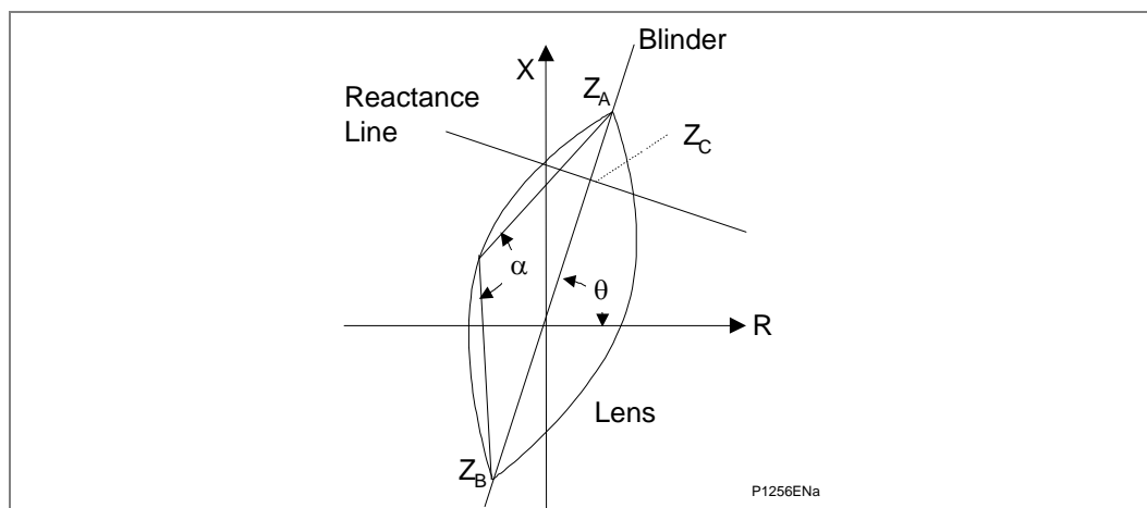
Figure 67 - Pole slipping protection using blinder and lenticular characteristic
