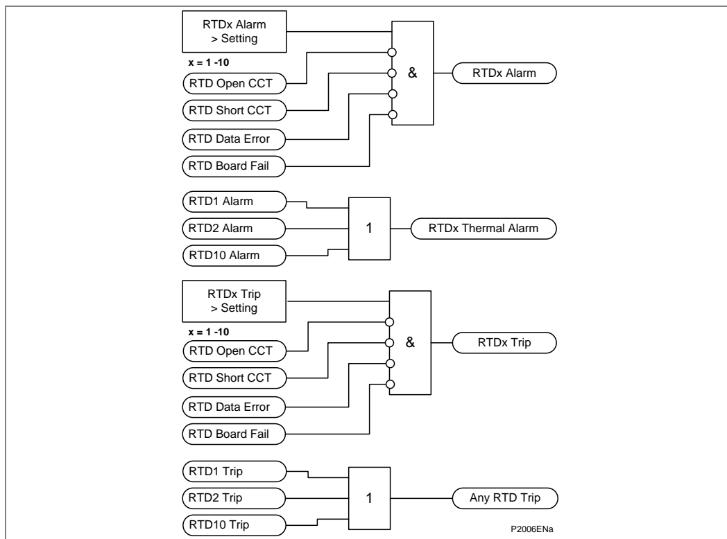
Figure 65 - RTD logic diagram
