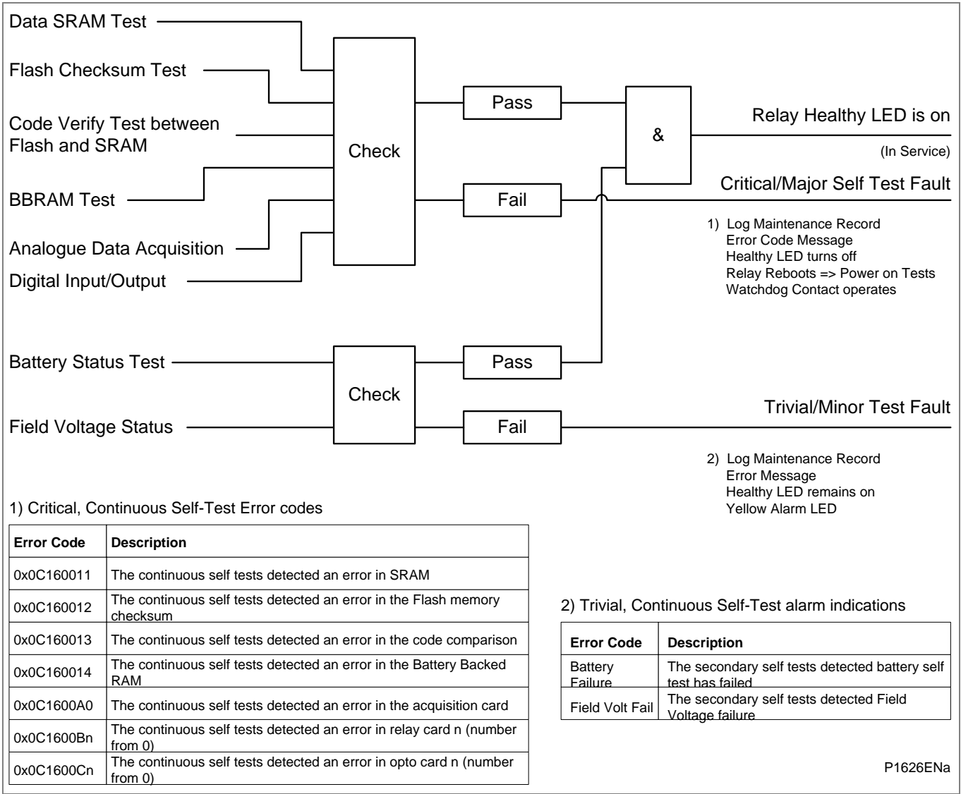
Figure 11 - Continuous self-testing logic
