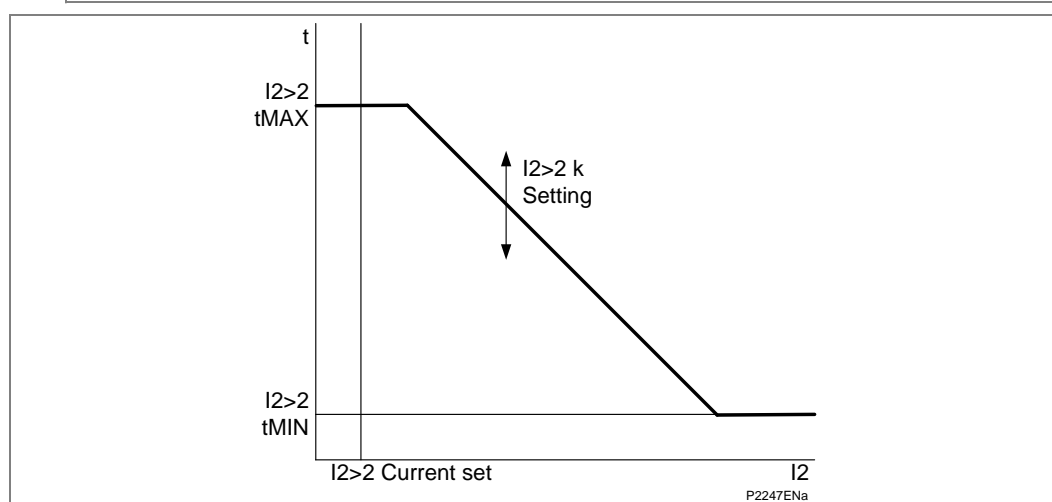
Figure 2 - Negative phase sequence thermal characteristic
