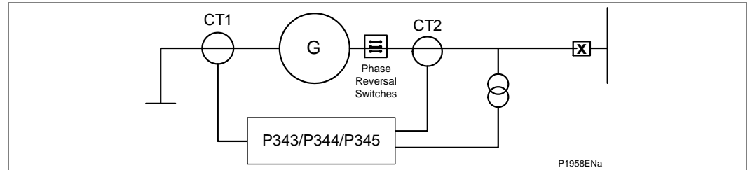
Figure 8 - Case 2 - phase reversal switches affecting CT1 only
