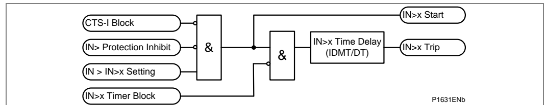
Figure 43 - Non-directional EF logic (single stage)
