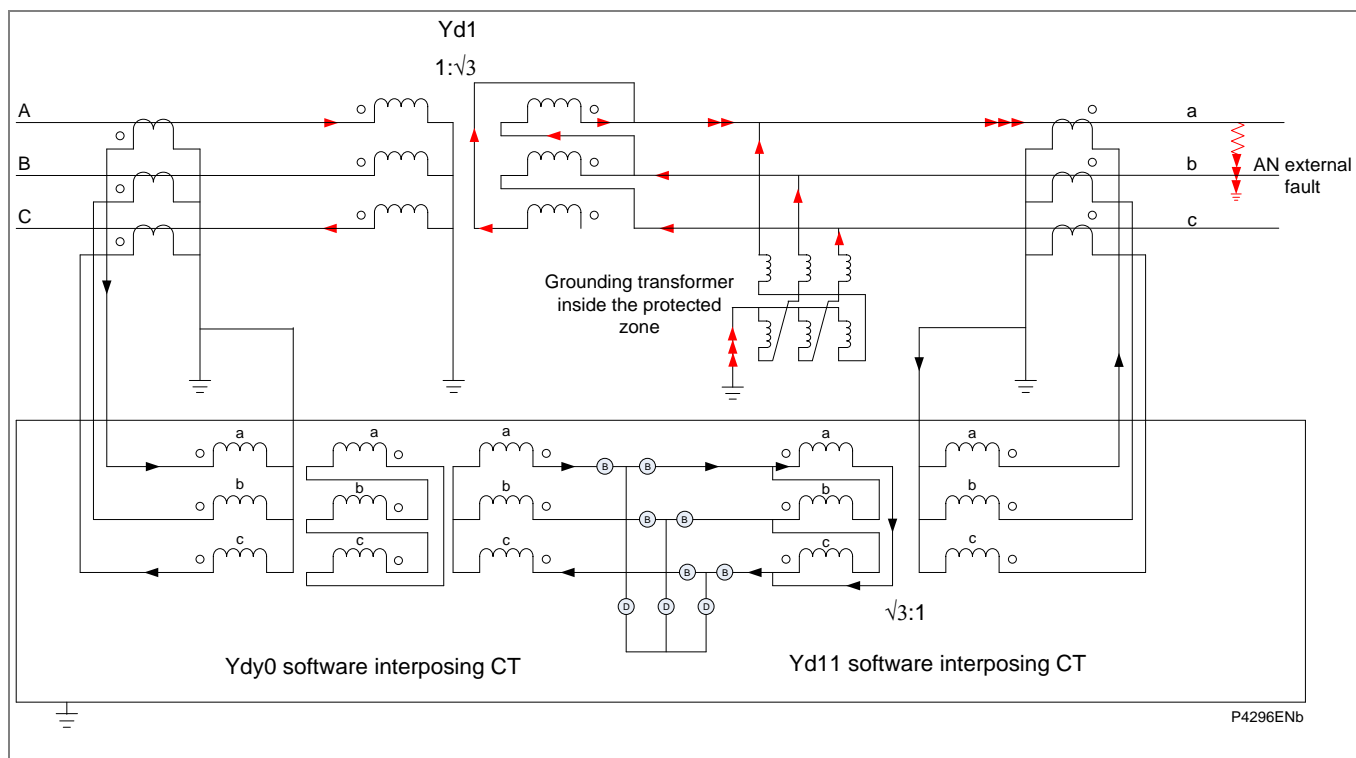
Figure 24 - Current distribution for an external fault on the delta side of a Yd1 transformer
