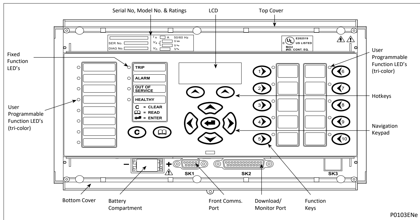
Figure 2 - Relay front view (P343/P344/P345) (60TE case)
