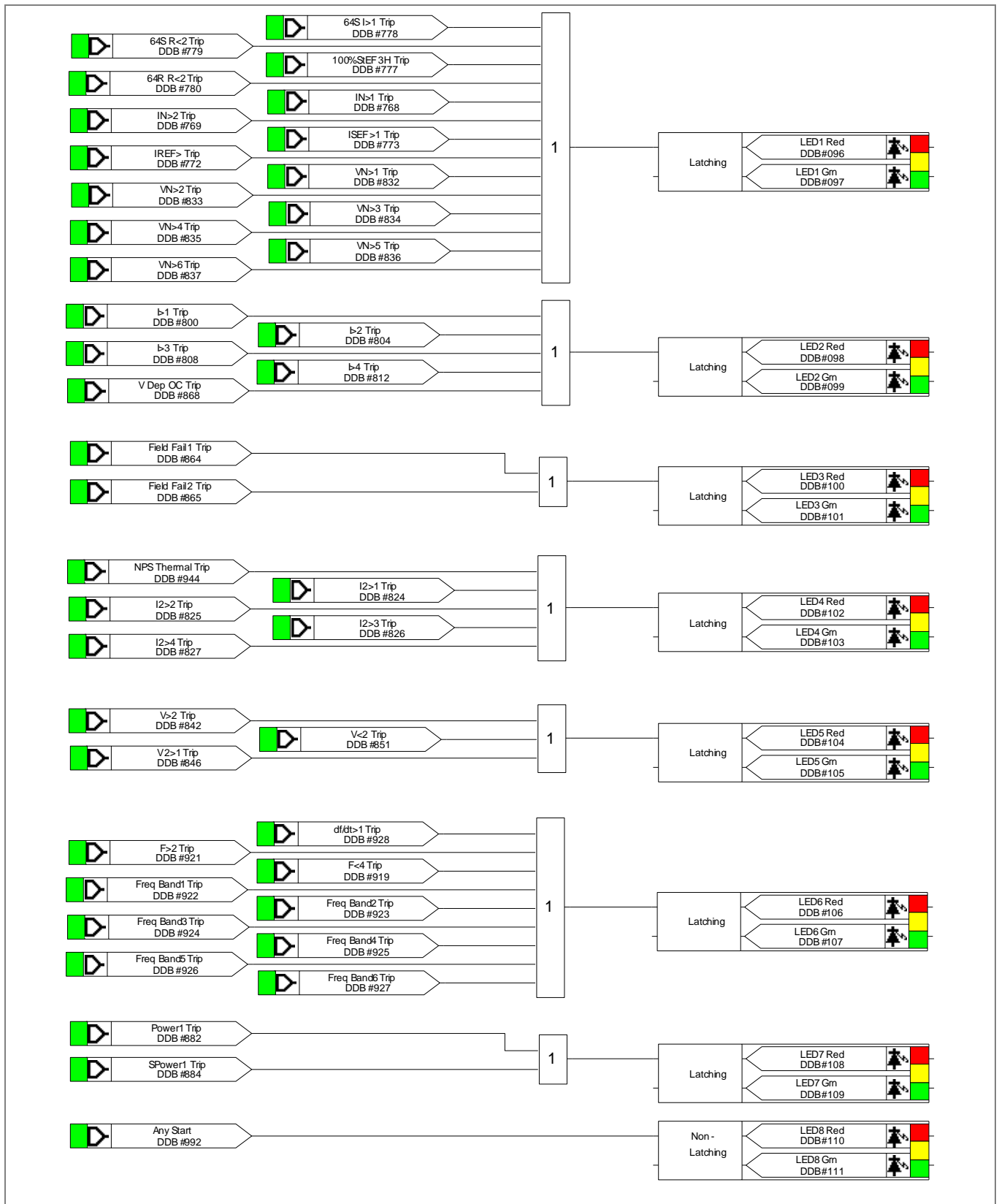
Figure 45 - LED output mapping
