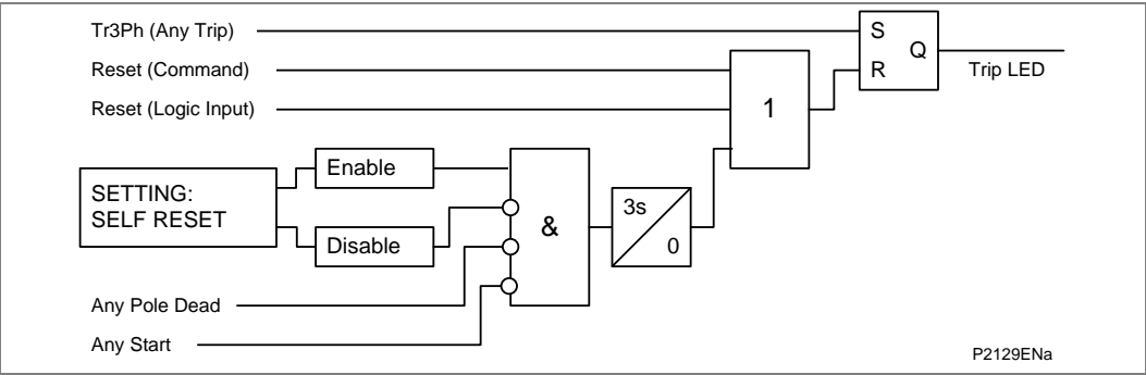
Figure 94 - Trip LED logic diagram
