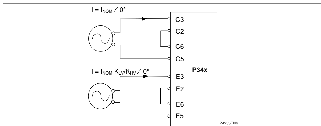
Figure 9 - Test equipment connection for a Dd0 transformer (1A and 60TE)
