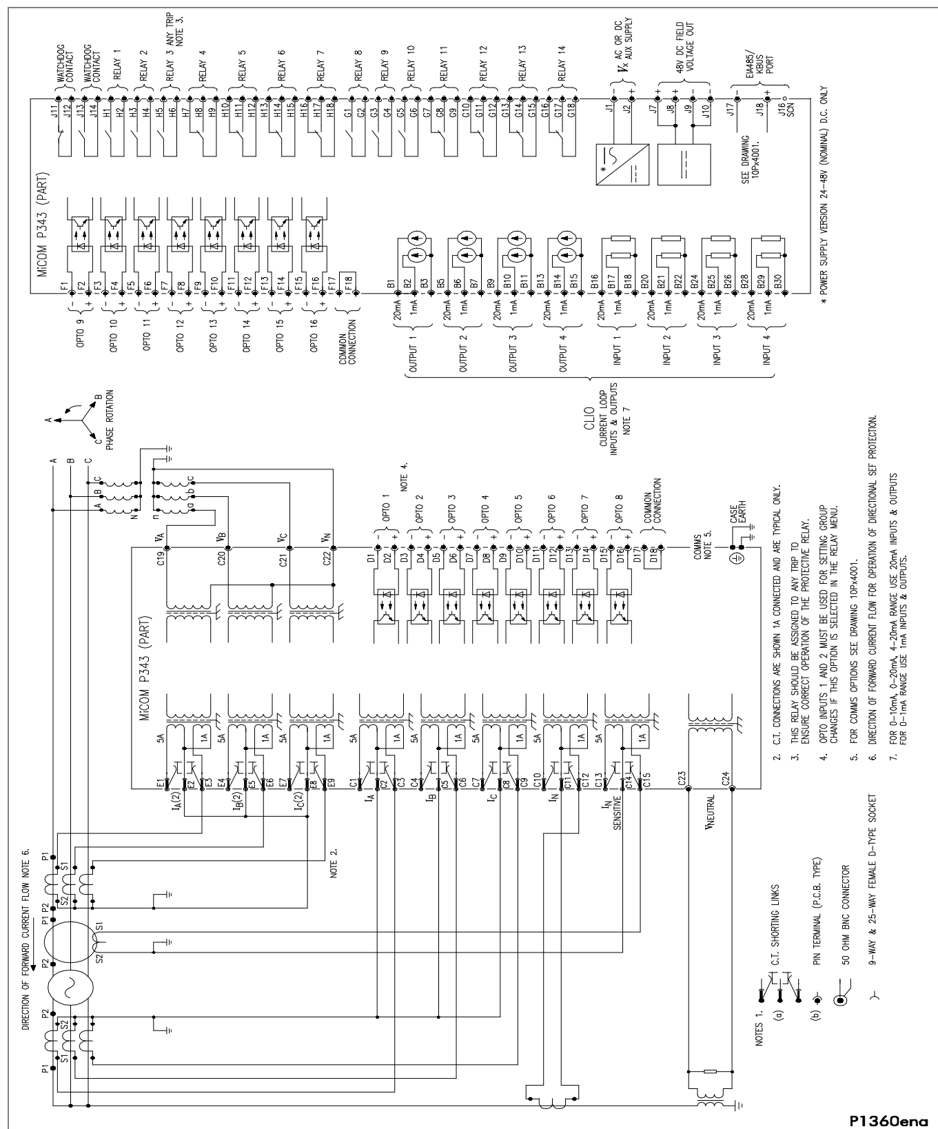
Figure 28 - P343 (60TE) with biased differential (16 I/P &amp; 14 O/P &amp; CLIO)
