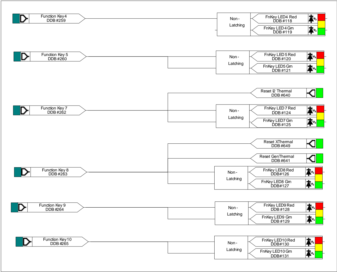
Figure 44 - Function key and function LED mapping
