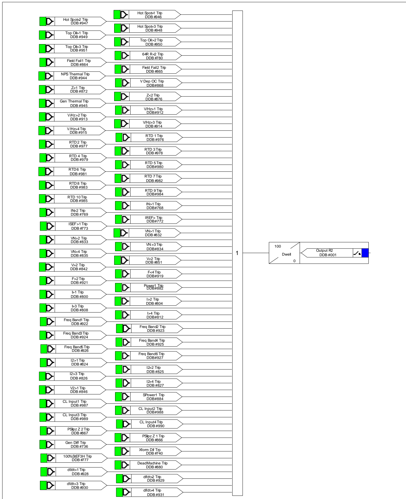
Figure 12 - Output relay R2 (Trip Prime Mover) mappings
