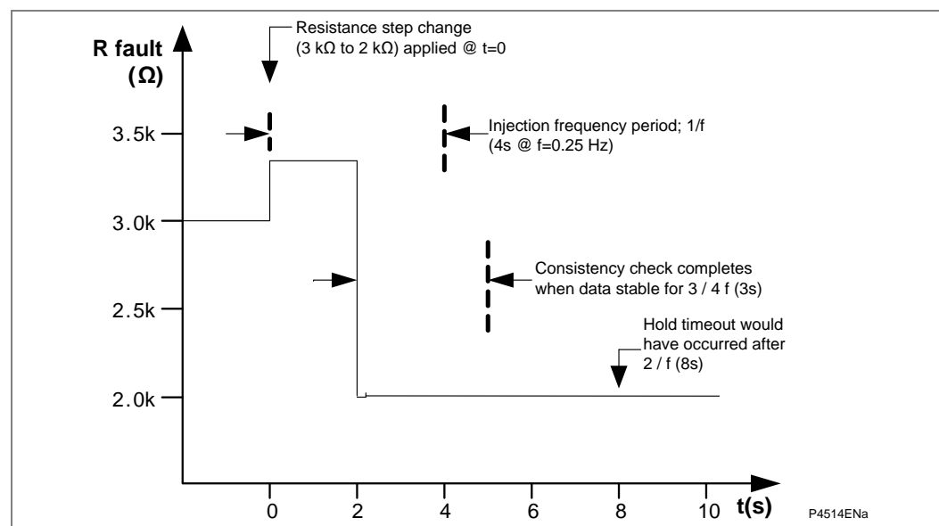
Figure 82 - Stability recovery via consistent data @ 0.25 Hz
