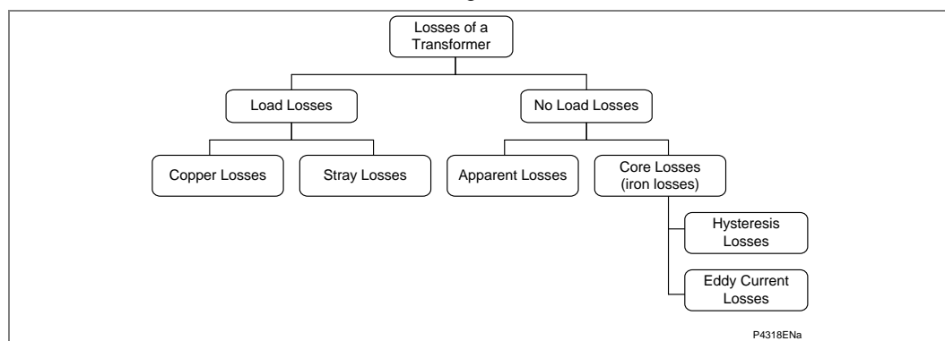
Figure 56 - Transformer losses
