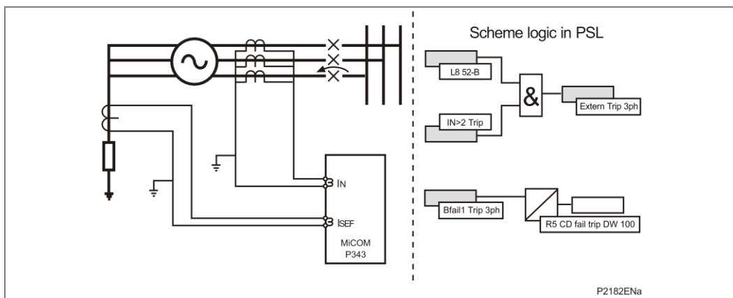
Figure 57 - Breaker flashover protection for directly connected machine
