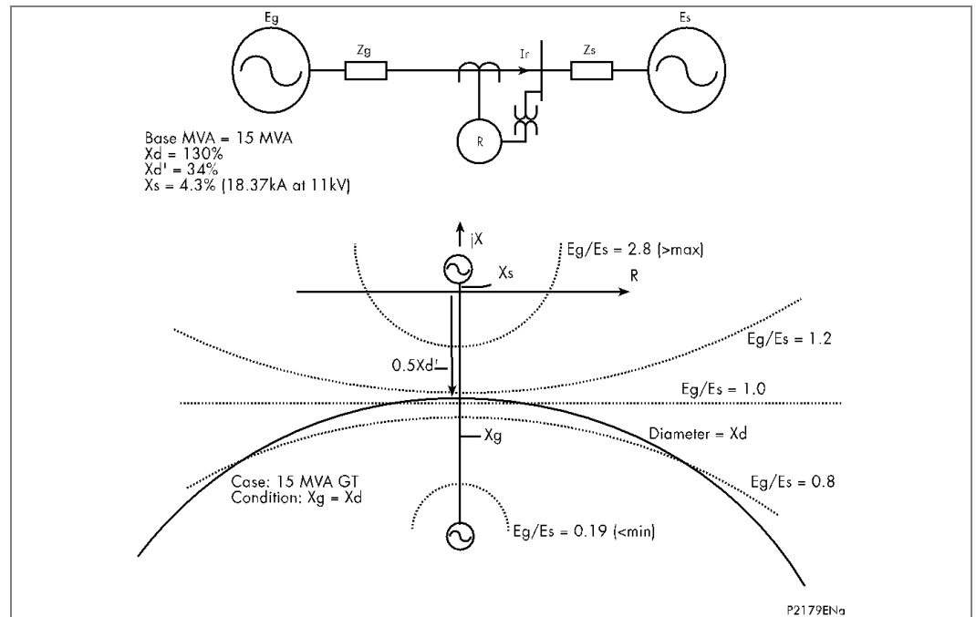
Figure 49 - Field failure protection function characteristics (small co-generator)
