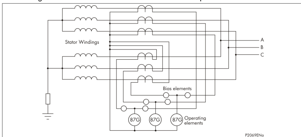
Figure 11 - Transverse biased differential protection for double wound machines
