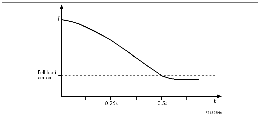
Figure 32 - Typical generator fault current decrement curve
