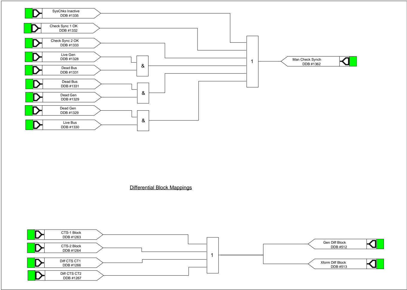
Figure 20 - Check synch and voltage monitor mapping
