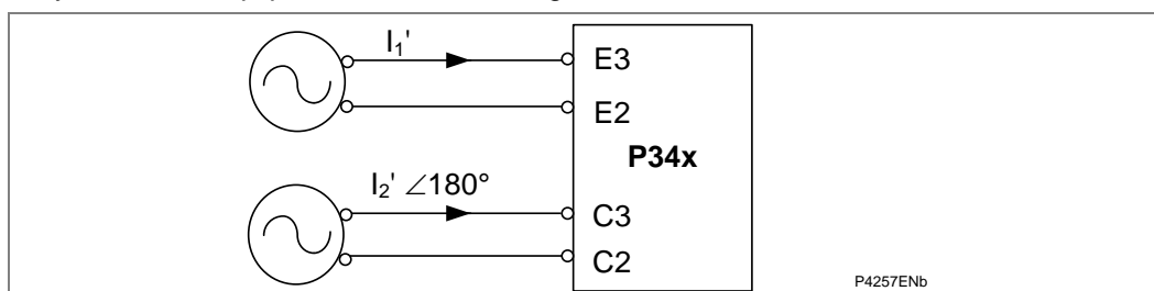
Figure 11 - Low set element bias characteristic test equipment connection(1A and 60TE)
