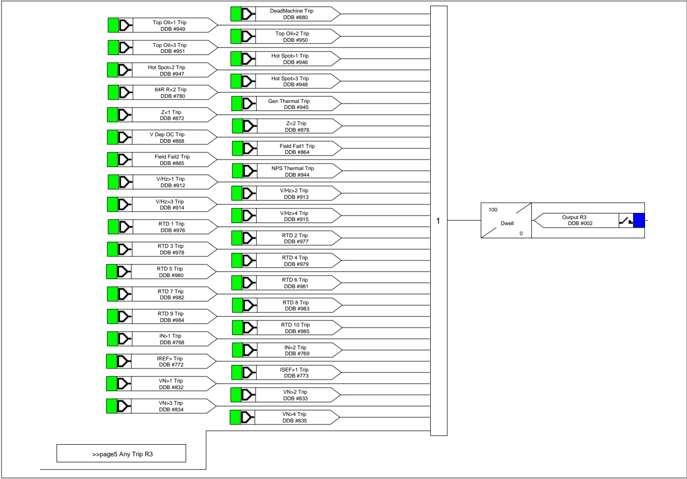
Figure 14 - Output relay R4 (General Alarm) mappings
