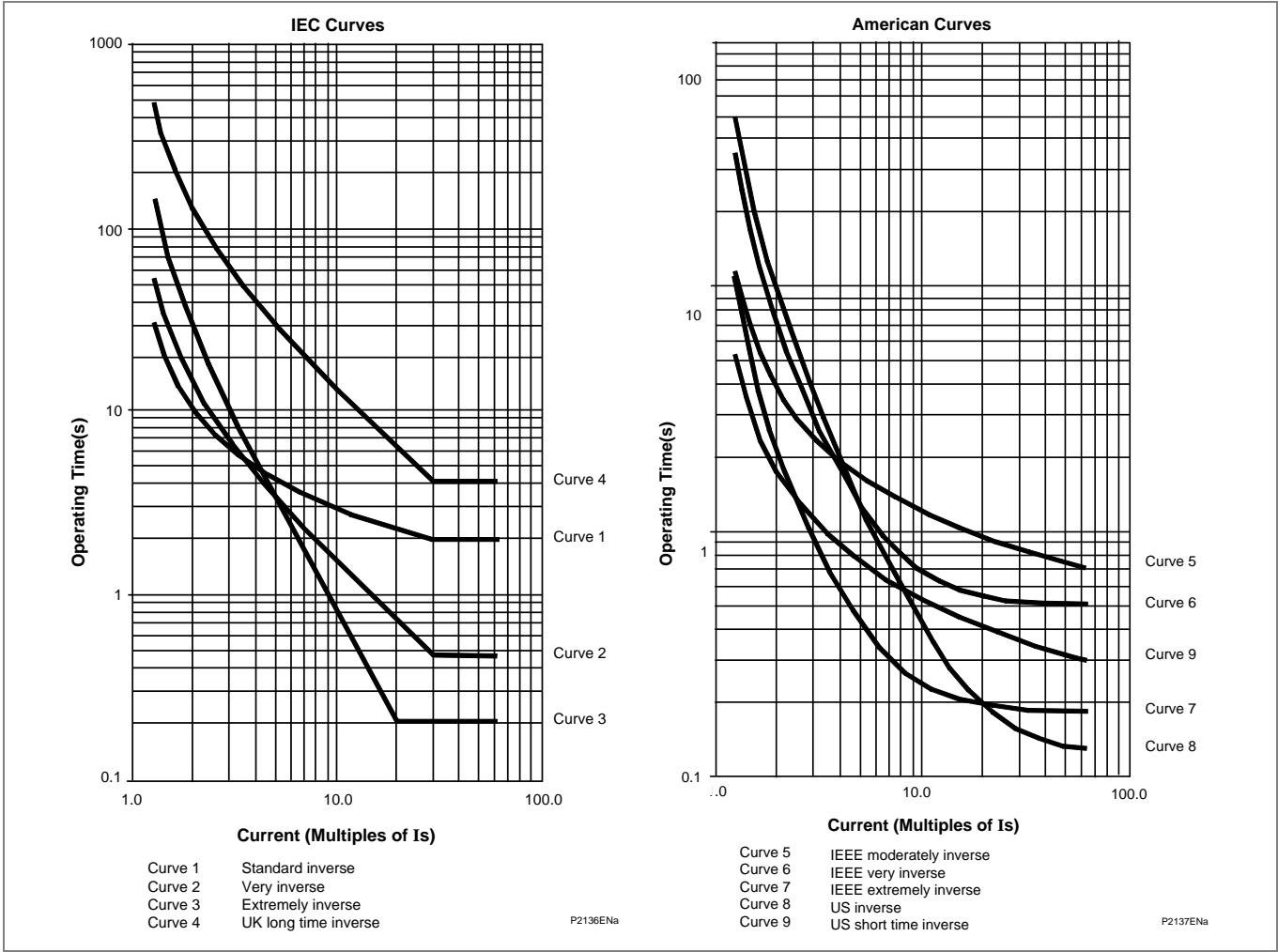
Figure 3 - Current/Time Curves
