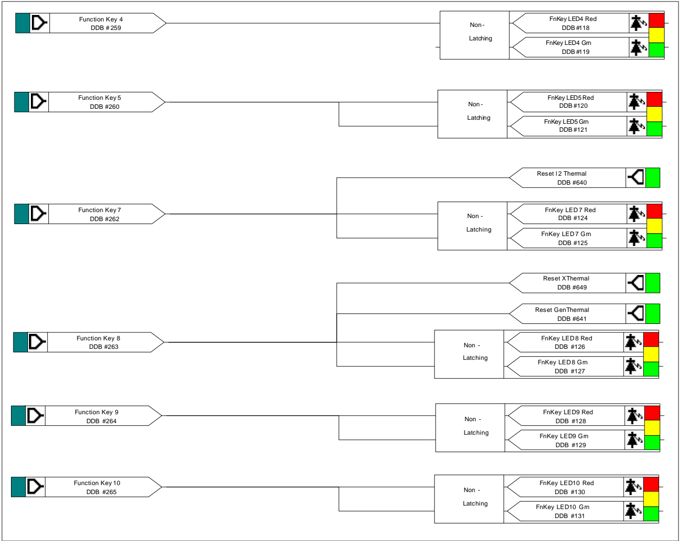
Figure 31 - Function key and function LED mapping
