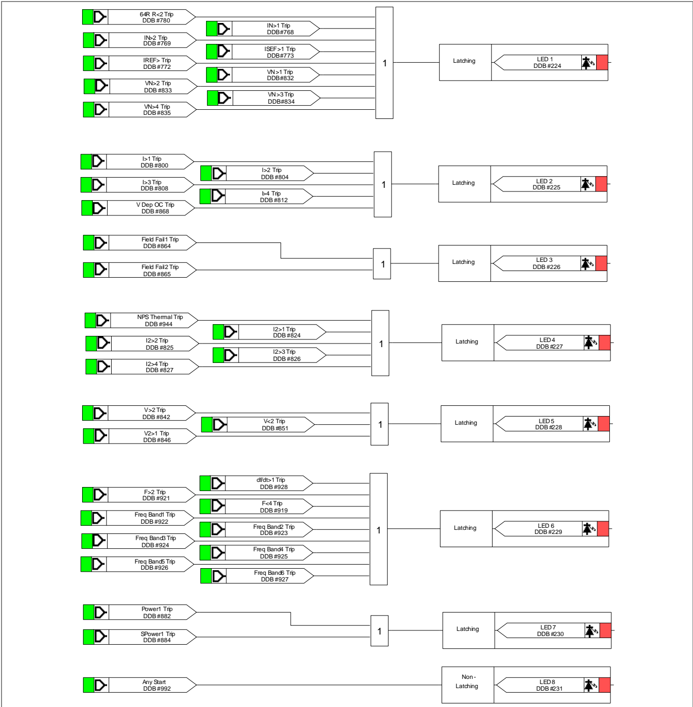
Figure 8 - LED output mappings
