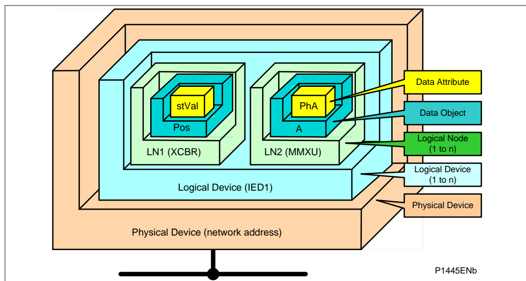
Figure 16 - Data model layers in IEC 61850
