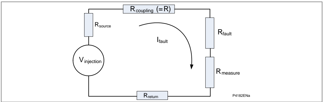
Figure 80 - Rotor earth fault equivalent circuit diagram
