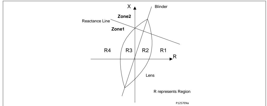
Figure 69 - Regions and zones definition (generating mode)
