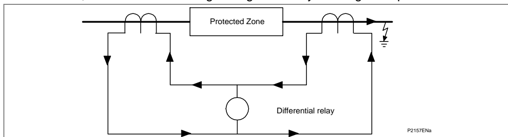
Figure 1 - Principle of circulating current differential protection
