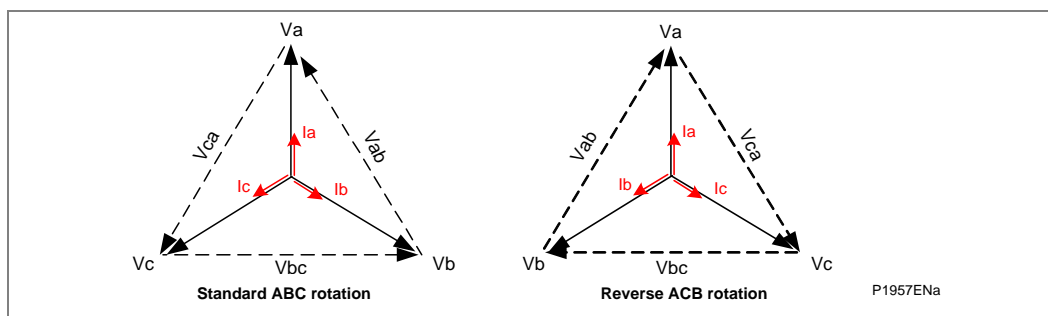
Figure 7 - Standard and reverse phase rotation
