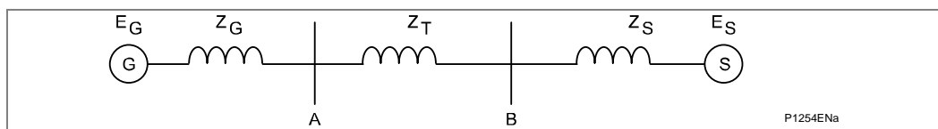
Figure 50 - Simplified two machine system
