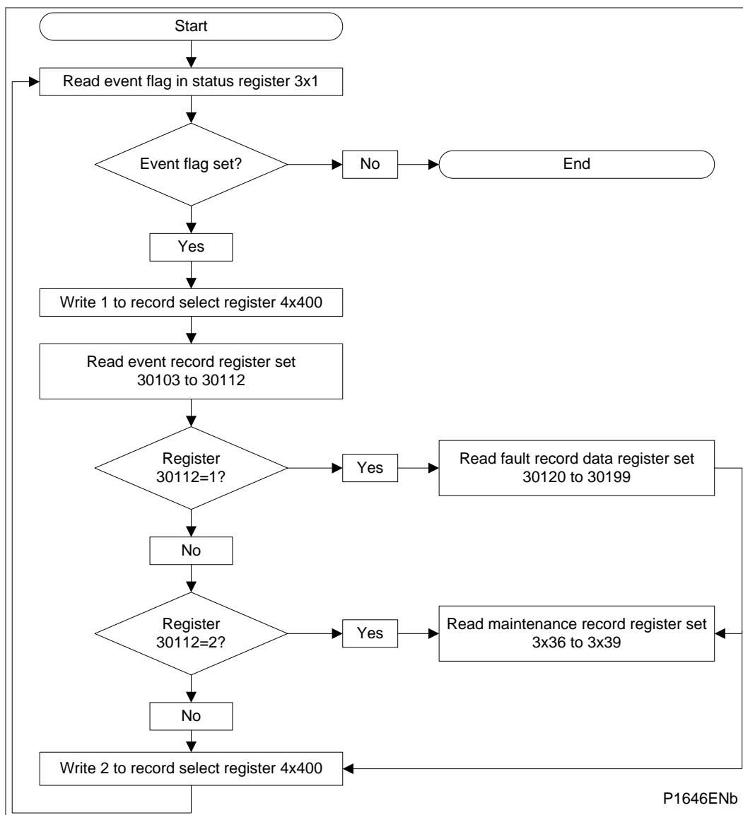
Figure 9 - Automatic event extraction procedure
