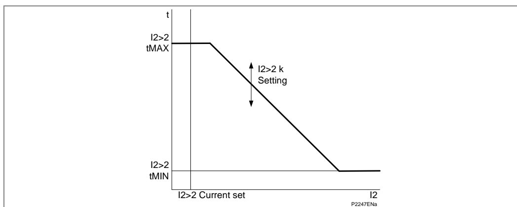
Figure 39 - Negative phase sequence thermal characteristic
