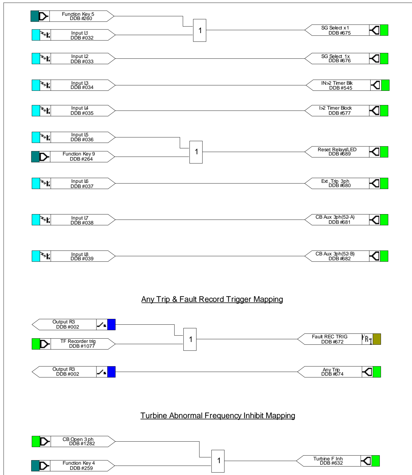
Figure 34 - Opto input mappings
