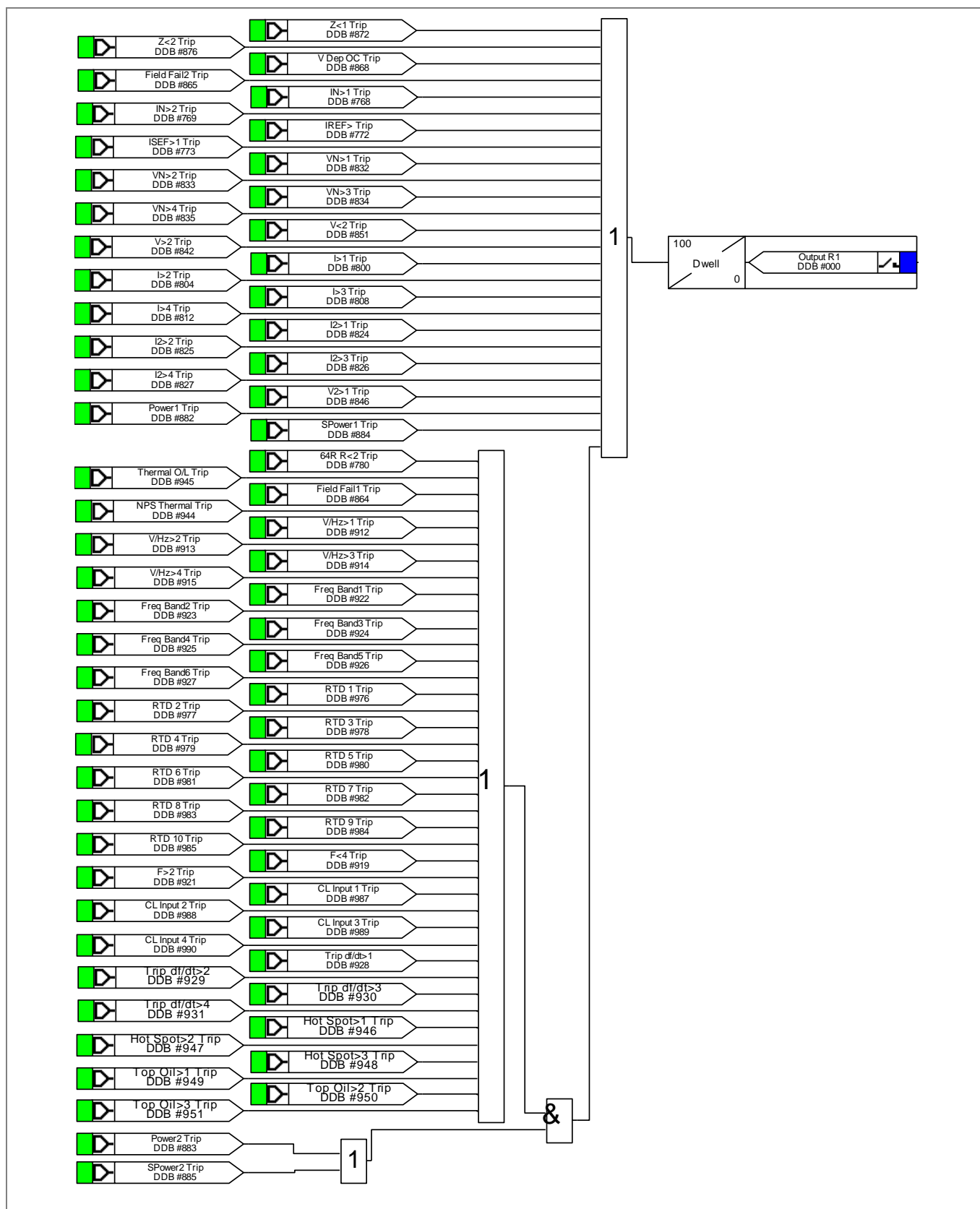
Figure 2 - Output relay R1 (Trip CB) mappings
