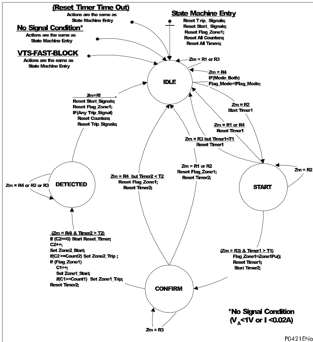
Figure 68 - State machine
