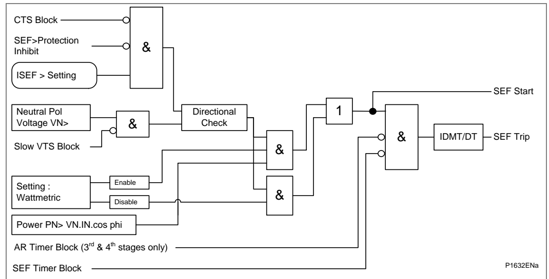
Figure 47 - Directional SEF with VN polarization
