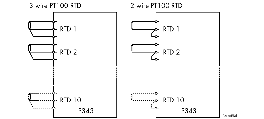
Figure 64 - Connection for RTD thermal probes
