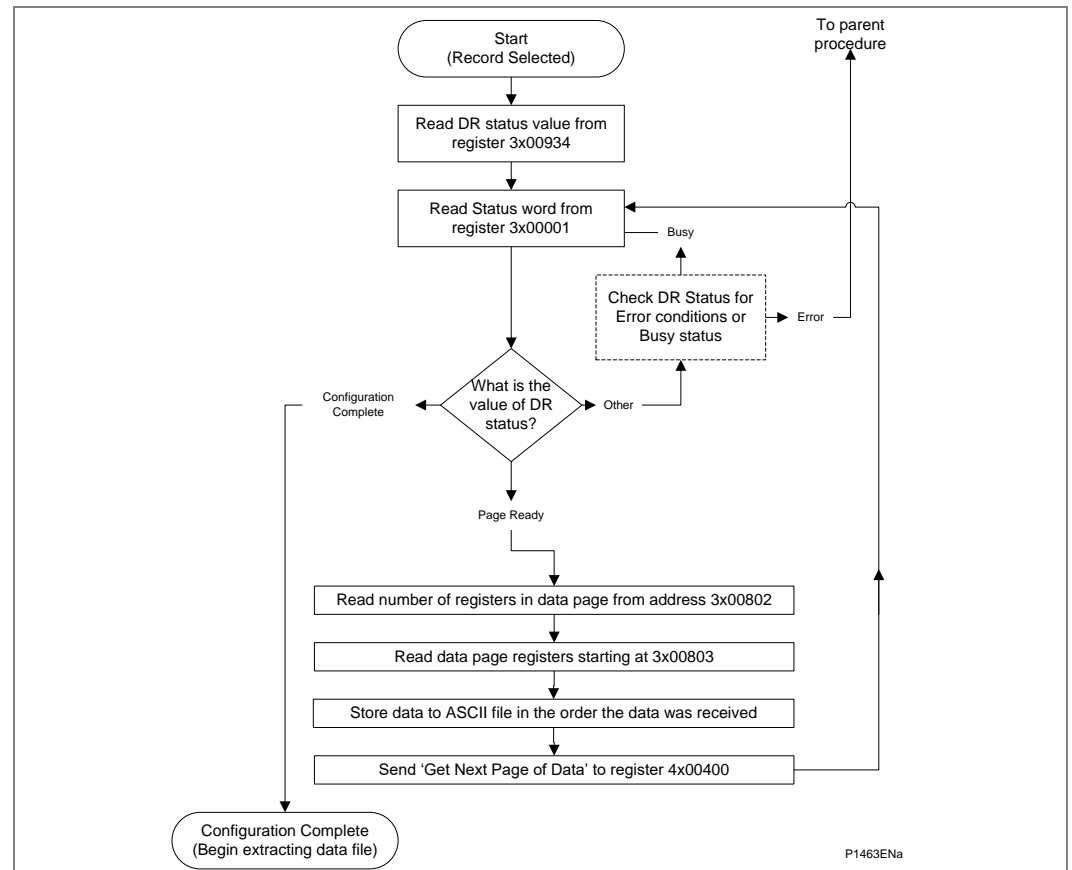
Figure 13 - Extracting the COMTRADE configuration file
