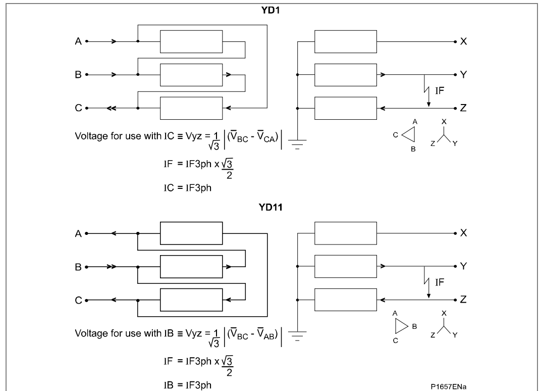
Figure 33 - Voltage vector transformation for a delta-star transformer
