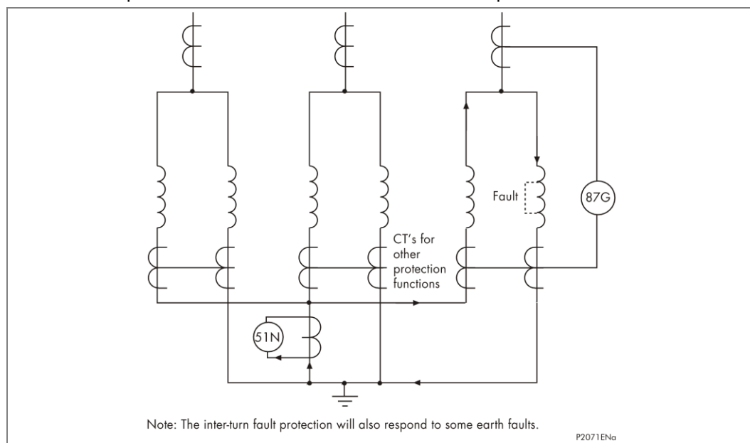
Figure 13 - Overcurrent interturn protection
