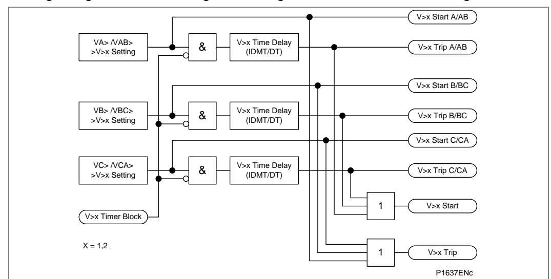
Figure 31 - Overvoltage - single and three phase tripping mode (single stage)
