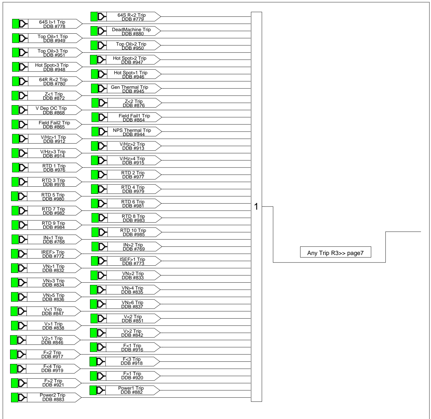
Figure 39 - Output relay mappings
