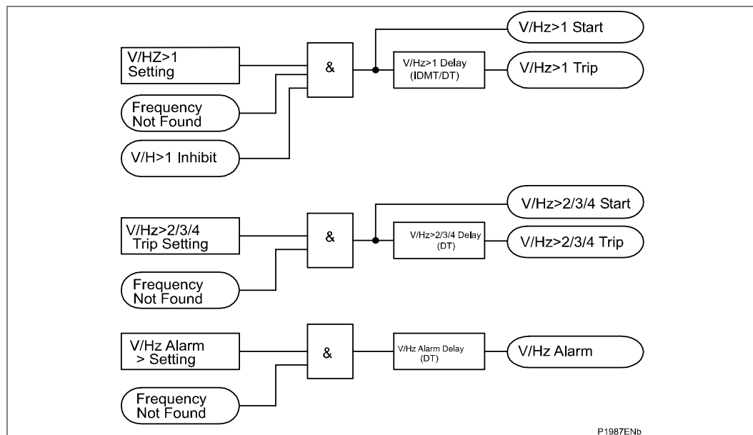
Figure 60 - Overfluxing logic diagram
