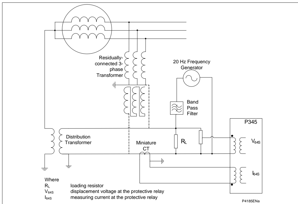
Figure 55 - 100% stator earth fault protection with earthing (broken delta) transformer or neutral transformer
