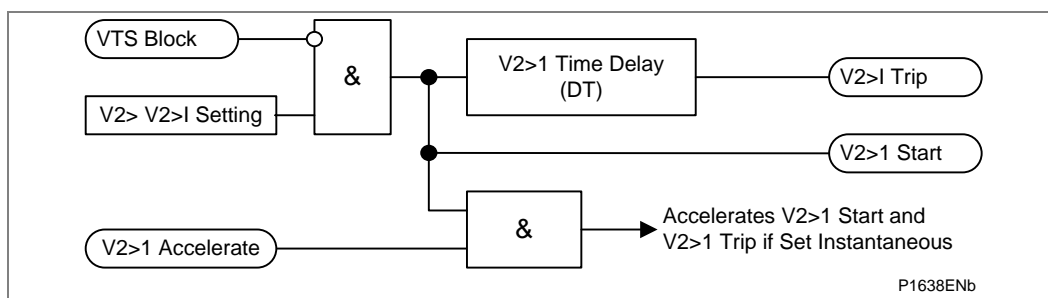
Figure 32 - Negative sequence overvoltage element logic
