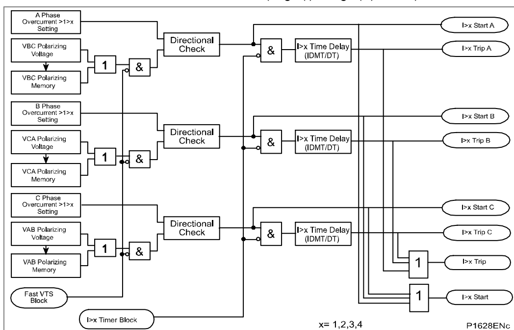
Figure 22 - Directional overcurrent logic
