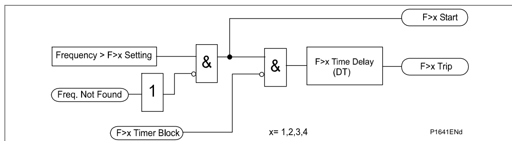
Figure 34 - Overfrequency logic (single stage)
