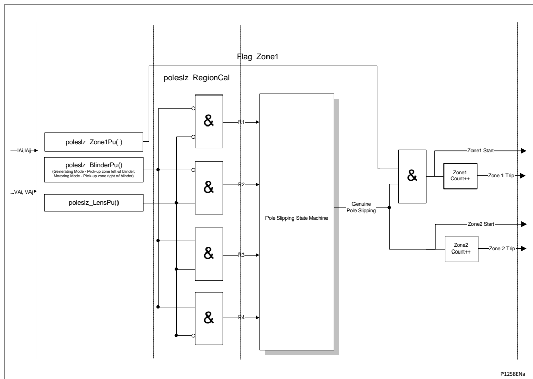
Figure 70 - Logic structure of pole slipping module
