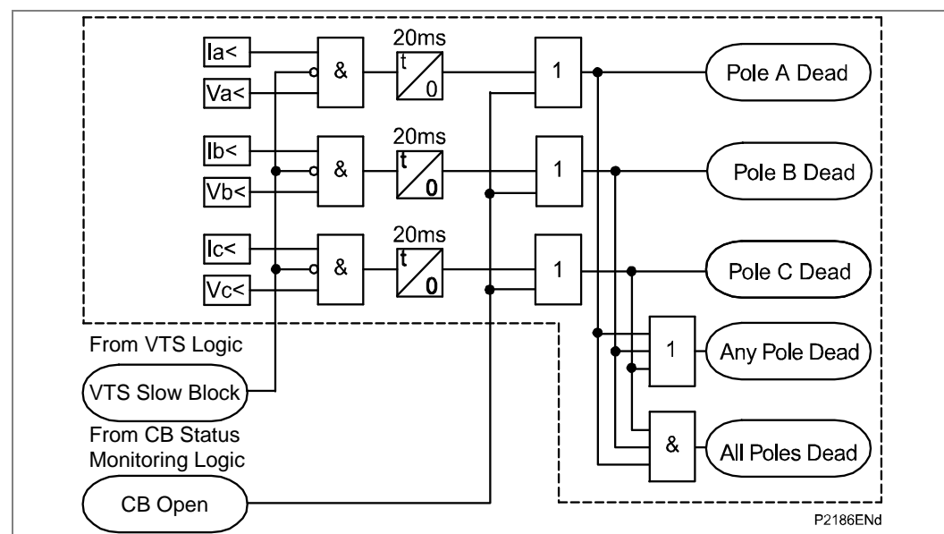
Figure 92 - Pole dead logic
