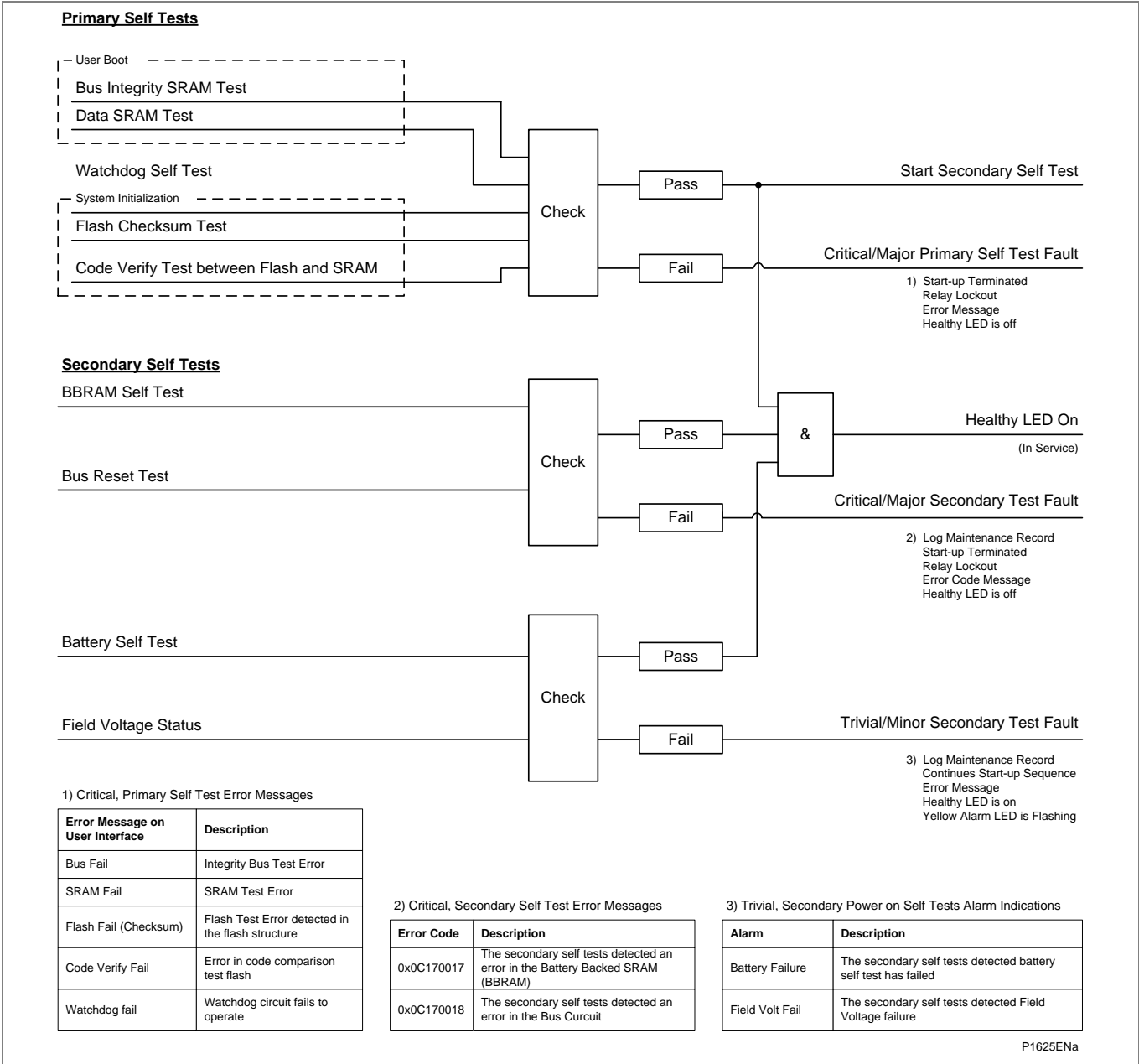
Figure 10 - Start-up self-testing logic
