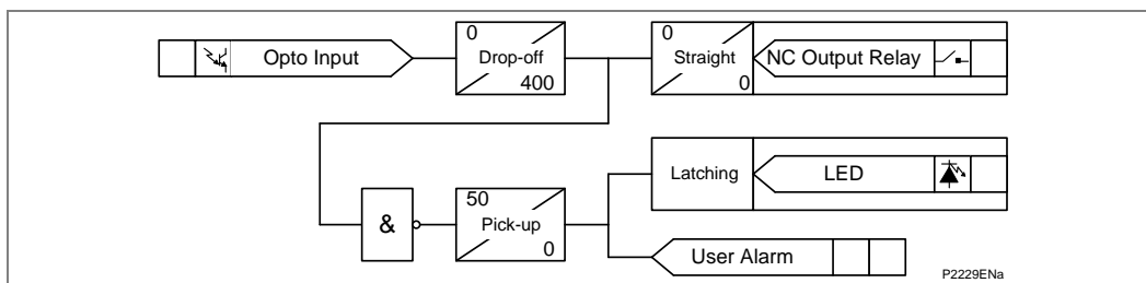
Figure 69 - PSL for TCS schemes 1 and 3
