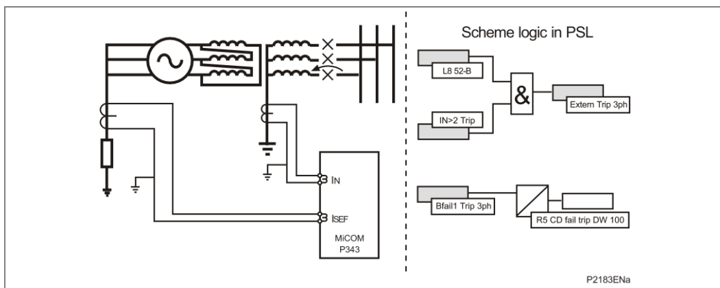
Figure 58 - Breaker flashover protection for indirectly connected machine
