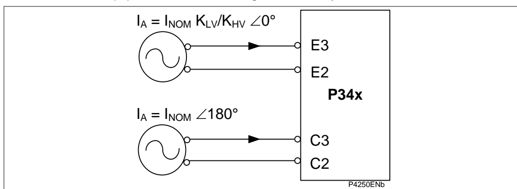
Figure 4 - Test equipment connection for a Yy0 transformer (1A and 60TE)
