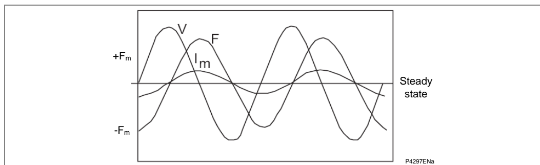
Figure 25 - Steady state magnetizing inrush current
