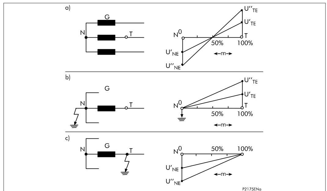
Figure 36 - Distribution of the 3rd harmonic component along the stator winding of a large generator
