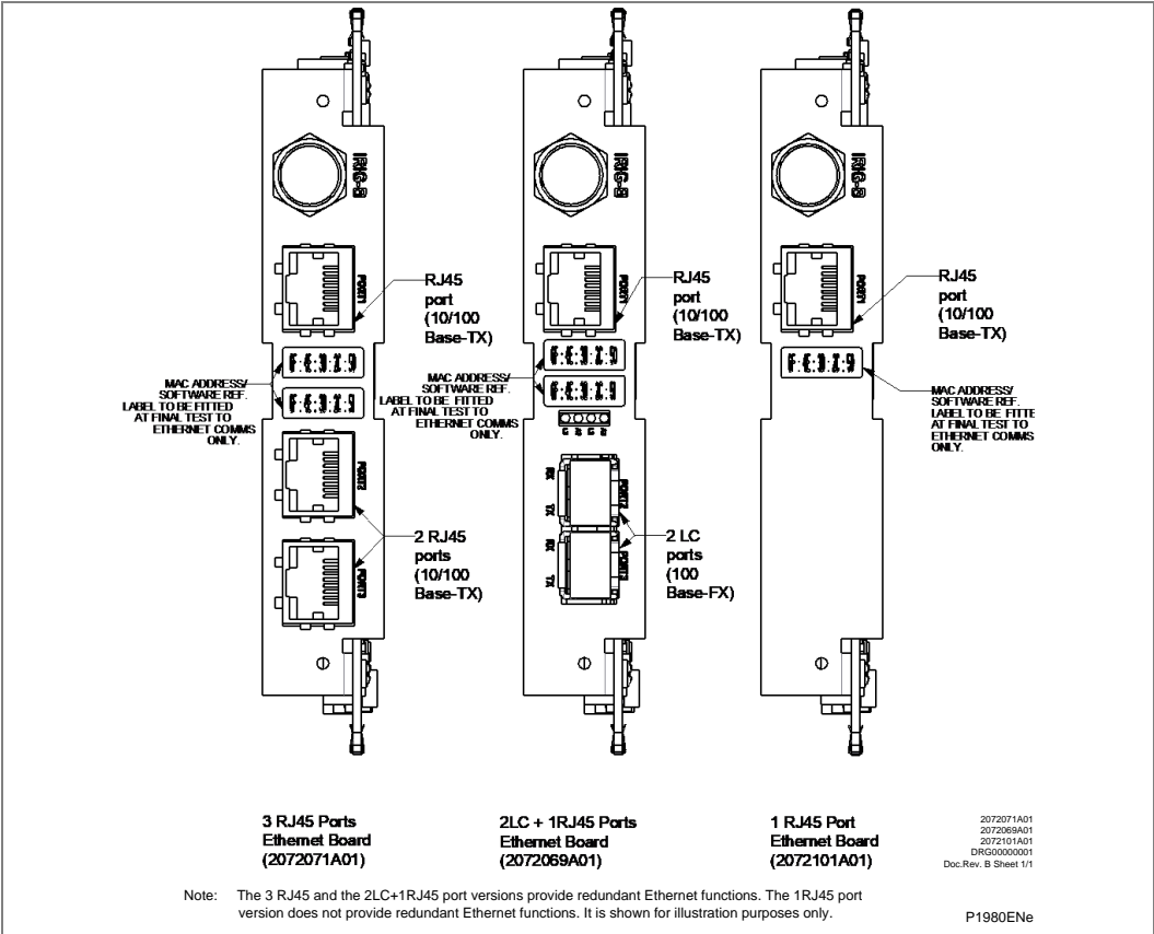
Figure 6 - Ethernet board connectors (3 RJ45 or 2 LC + RJ45 or 1 RJ45)
