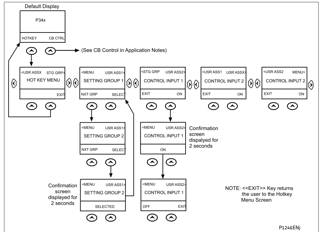
Figure 7 - Hotkey menu navigation
