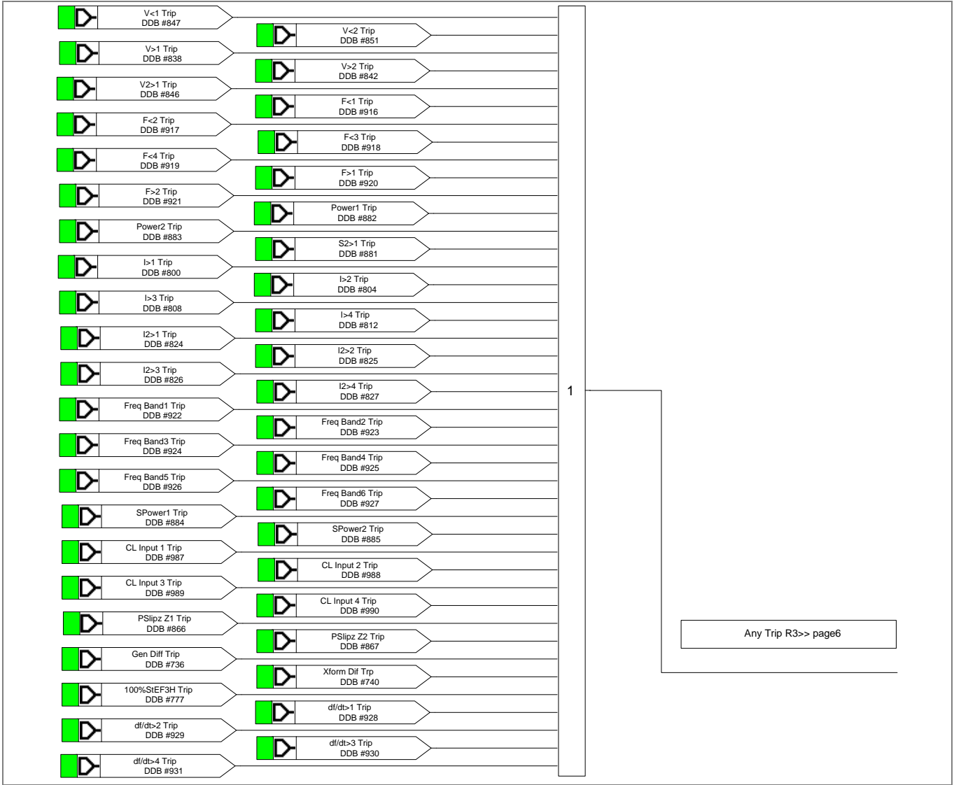
Figure 13 - Output relay R3 (Any Trip) mappings
