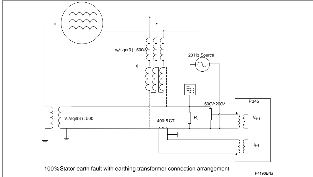
Figure 39 - 64S Connection for generators earthed via earthing transformer
