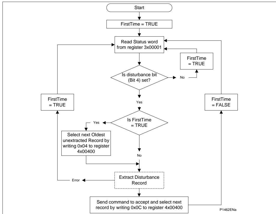
Figure 12 - Automatic selection of a disturbance - option 2
