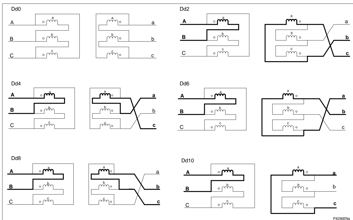
Figure 10 - Dd transformer connections
