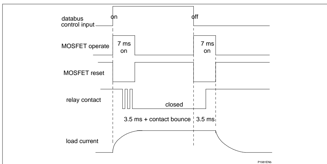
Figure 3 - High break contact operation
