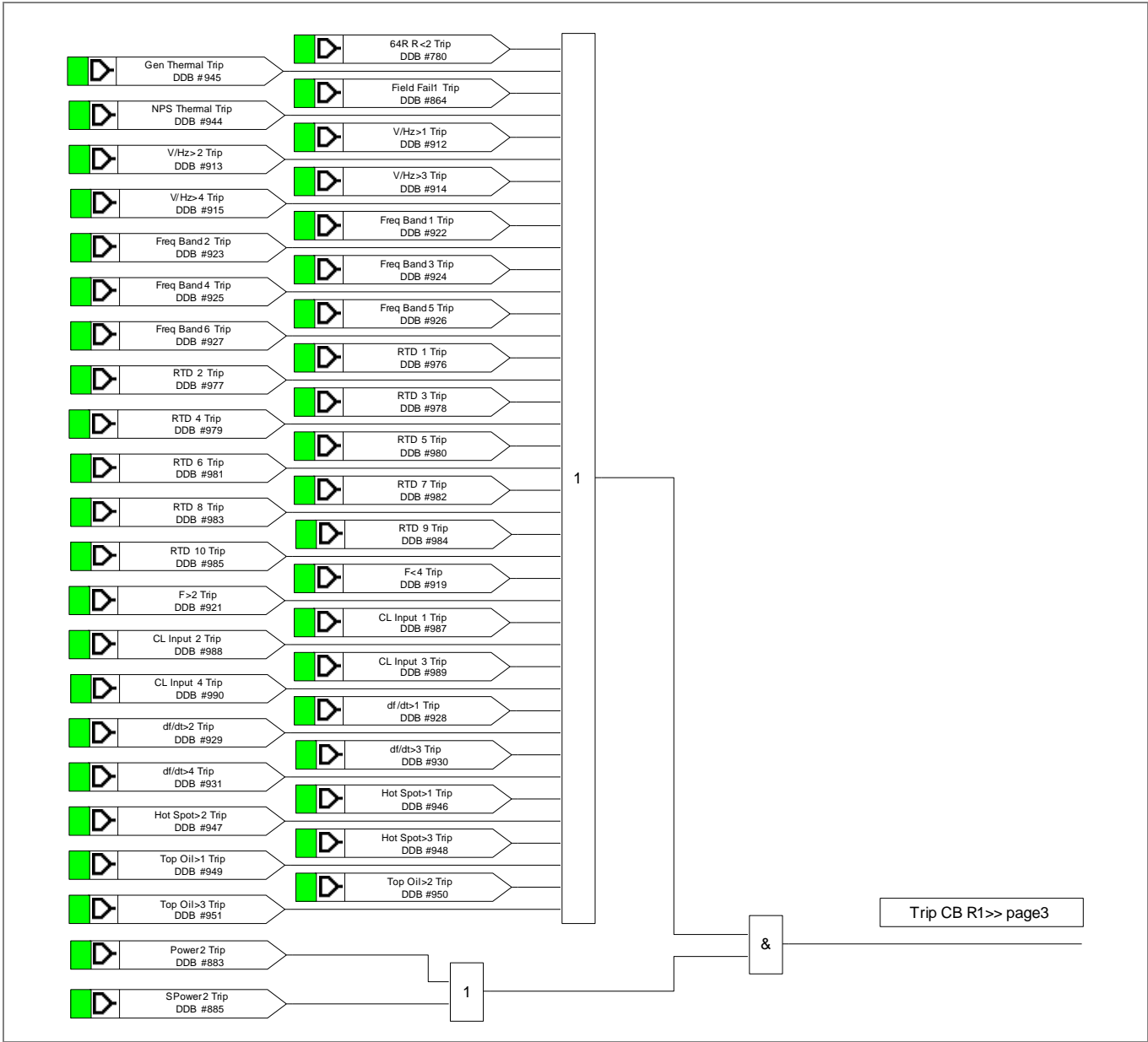
Figure 22 - Output relay R1 (Trip CB) mappings
