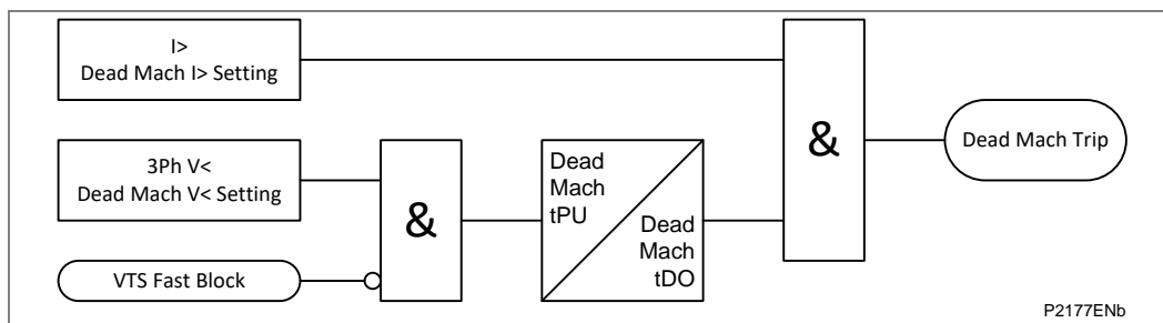
Figure 63 - Fixed scheme logic for unintentional energization of standstill protection
