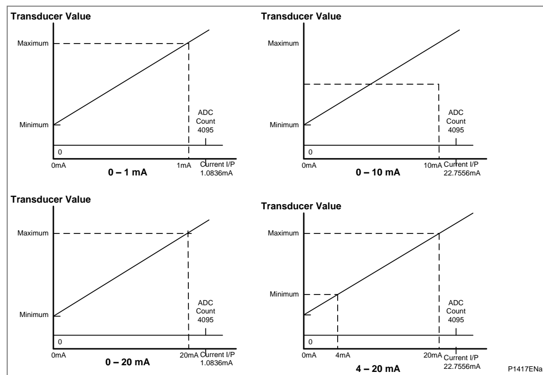
Figure 75 – Relationship between the Transducer measuring quantity and the current input range
