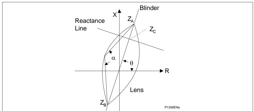
Figure 52 - Pole slipping protection using blinder and lenticular characteristic
