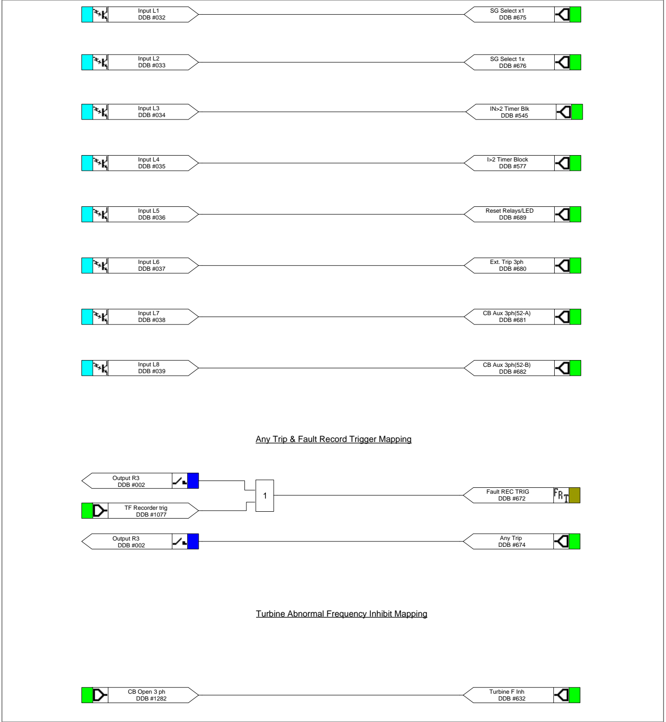
Figure 21 - Opto input mappings
