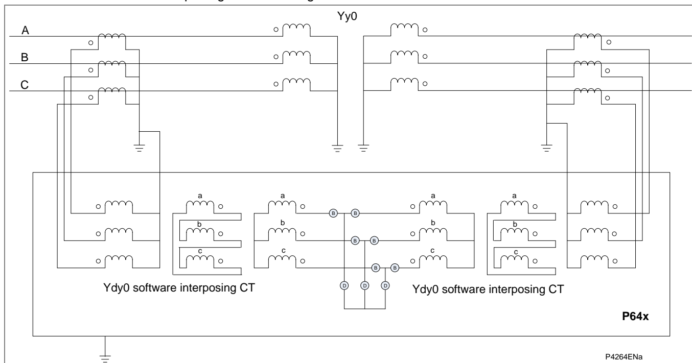
Figure 11 - Software interposing CTs for a Yy0 transformer
