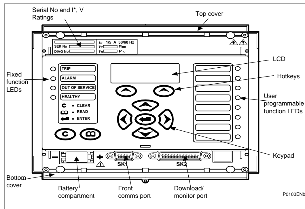
Figure 1 - Relay front view (P342) (40TE case)
