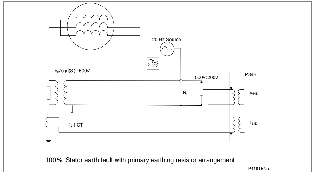
Figure 40 - 64S Connection for generators earthed via primary resistor
