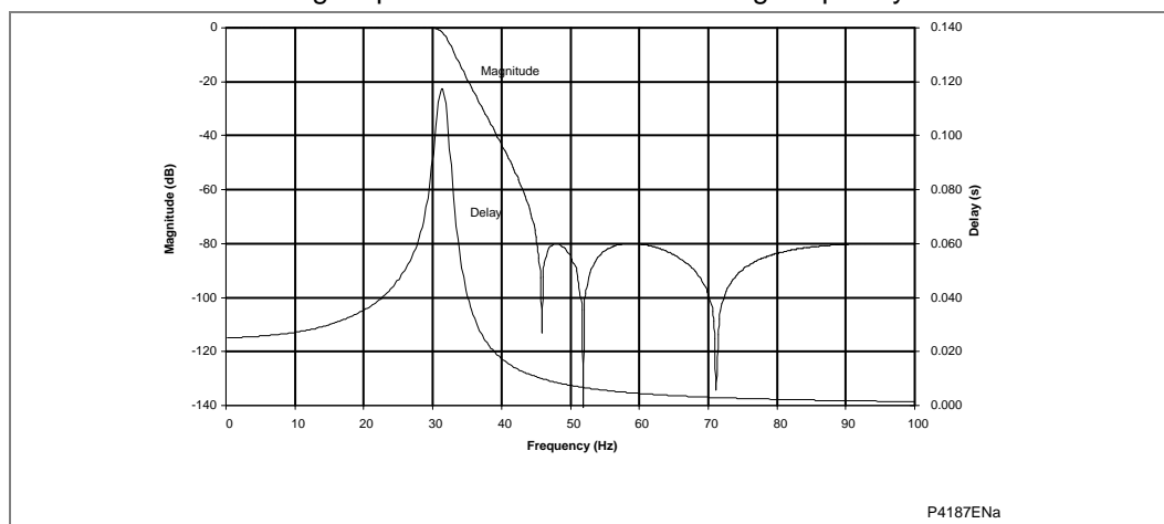
Figure 58 - 64S elliptic 8th order low pass filter discrete frequency response
