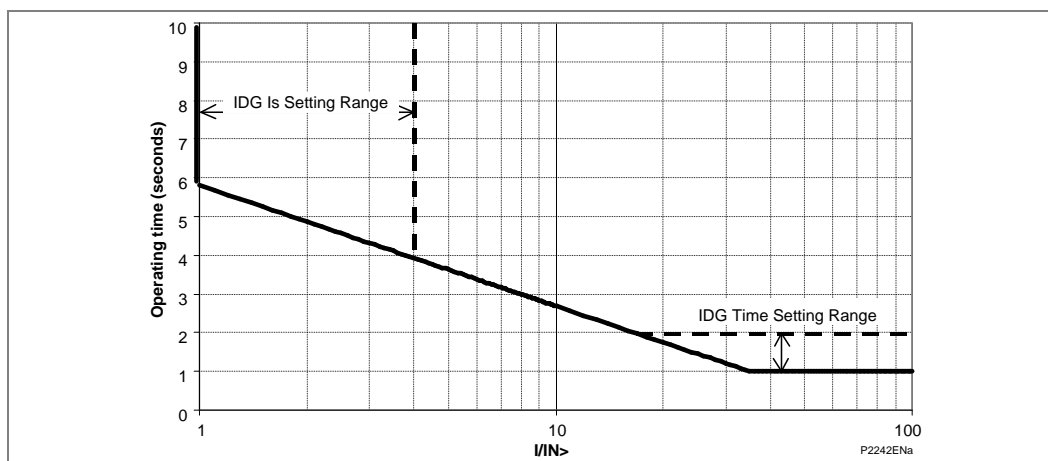
Figure 44 - IDG characteristic
