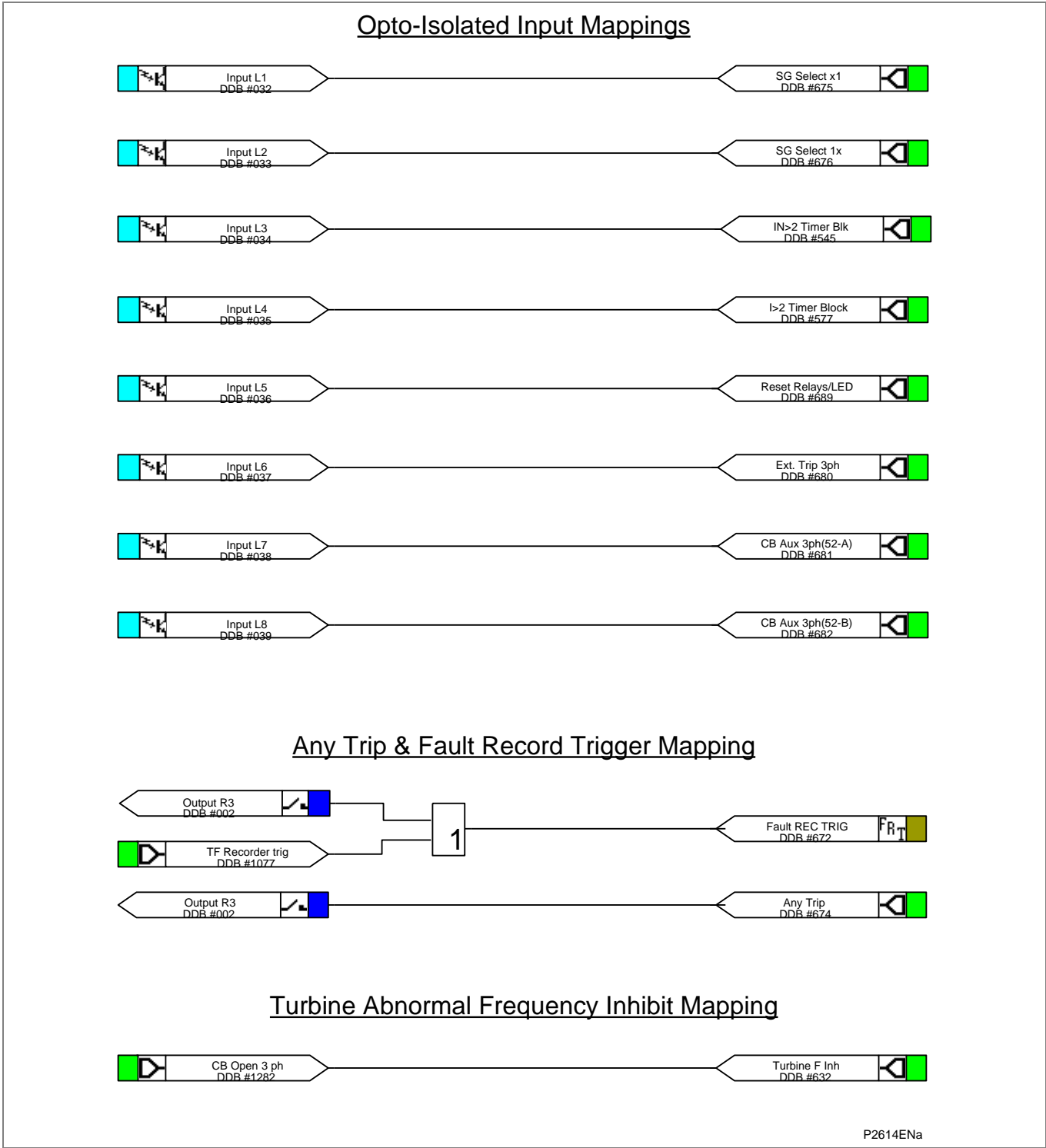
Figure 1 - Opto input mappings
