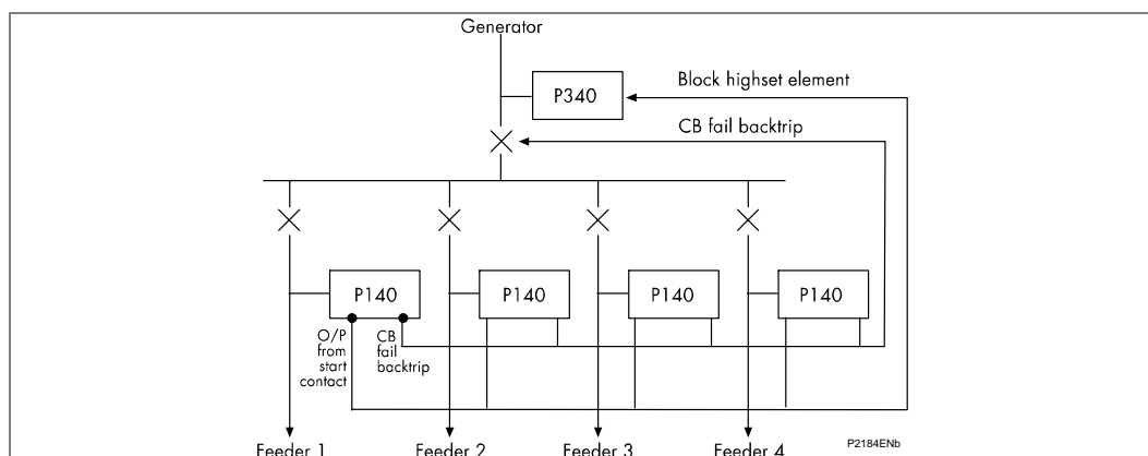
Figure 59 - Simple busbar blocking scheme (single incomer)
