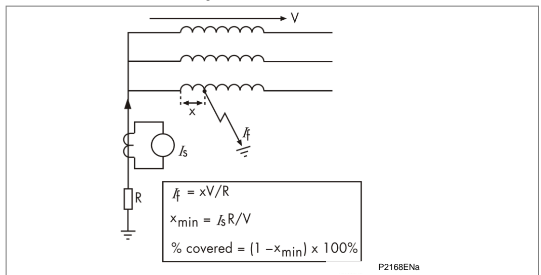
Figure 35 - Effective coverage of stator earth fault protection
