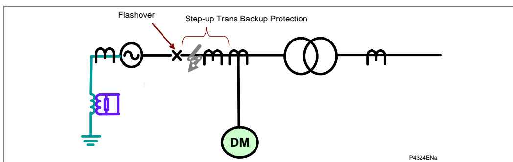
Figure 48 - GCB flashover and transformer back-up protection
