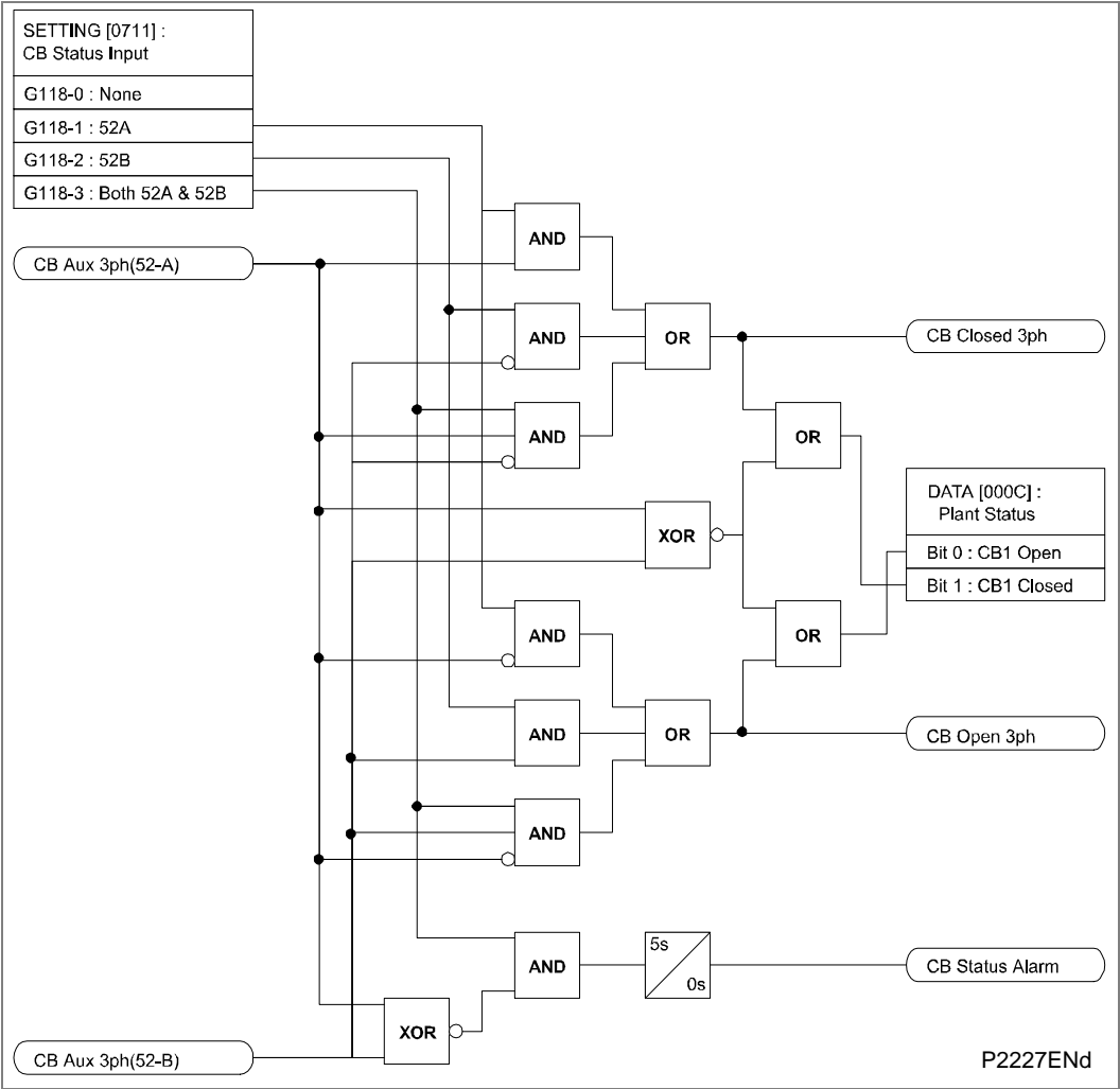
Figure 91 - CB state monitoring
