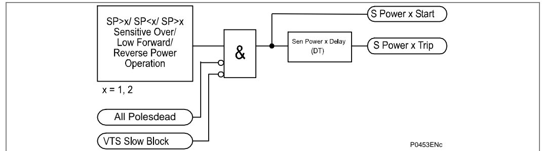
Figure 42 - Sensitive power logic diagram
