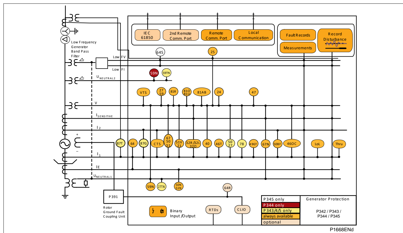
Figure 1 - Functional diagram
