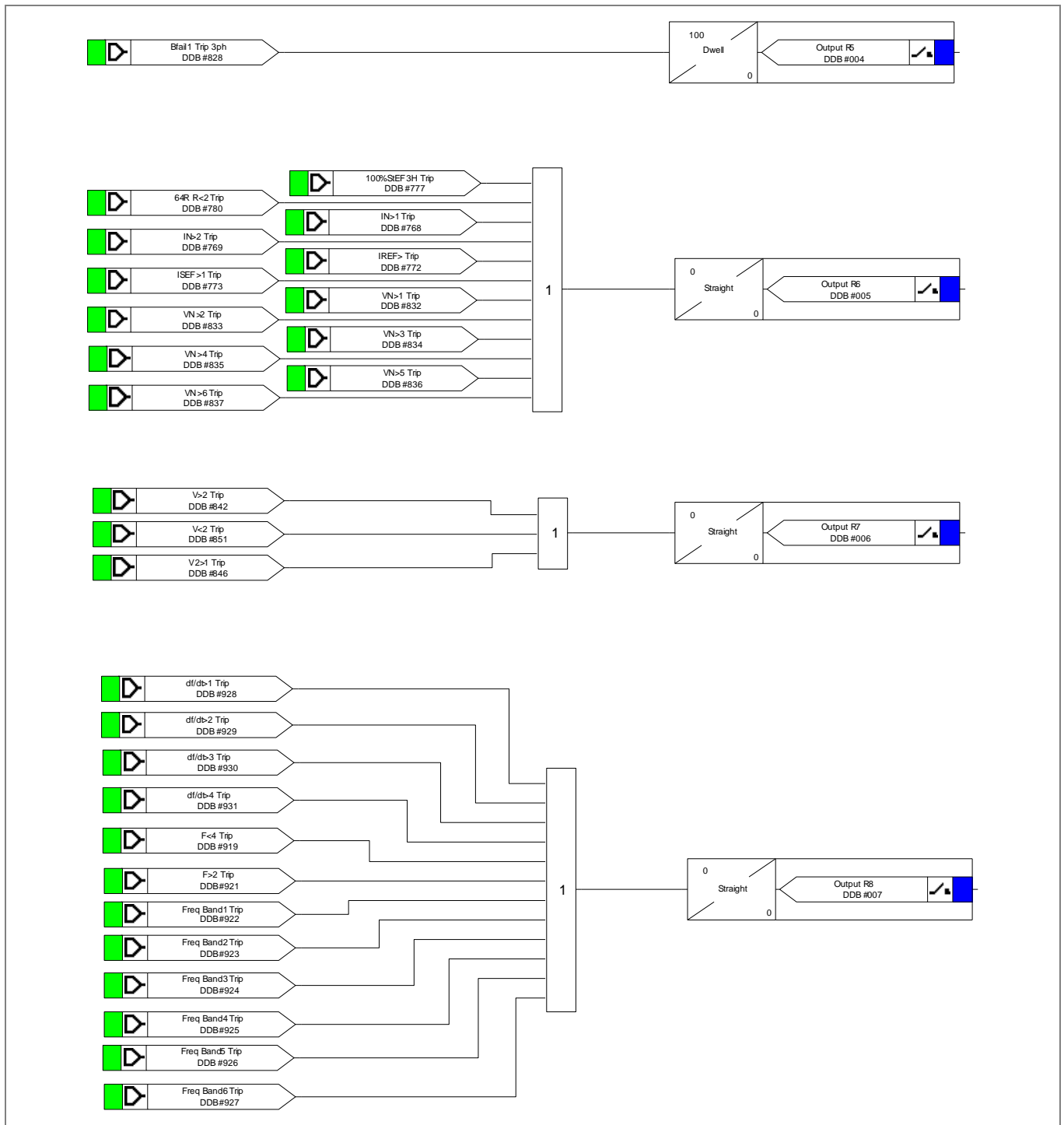
Figure 29 - Output relay mappings
