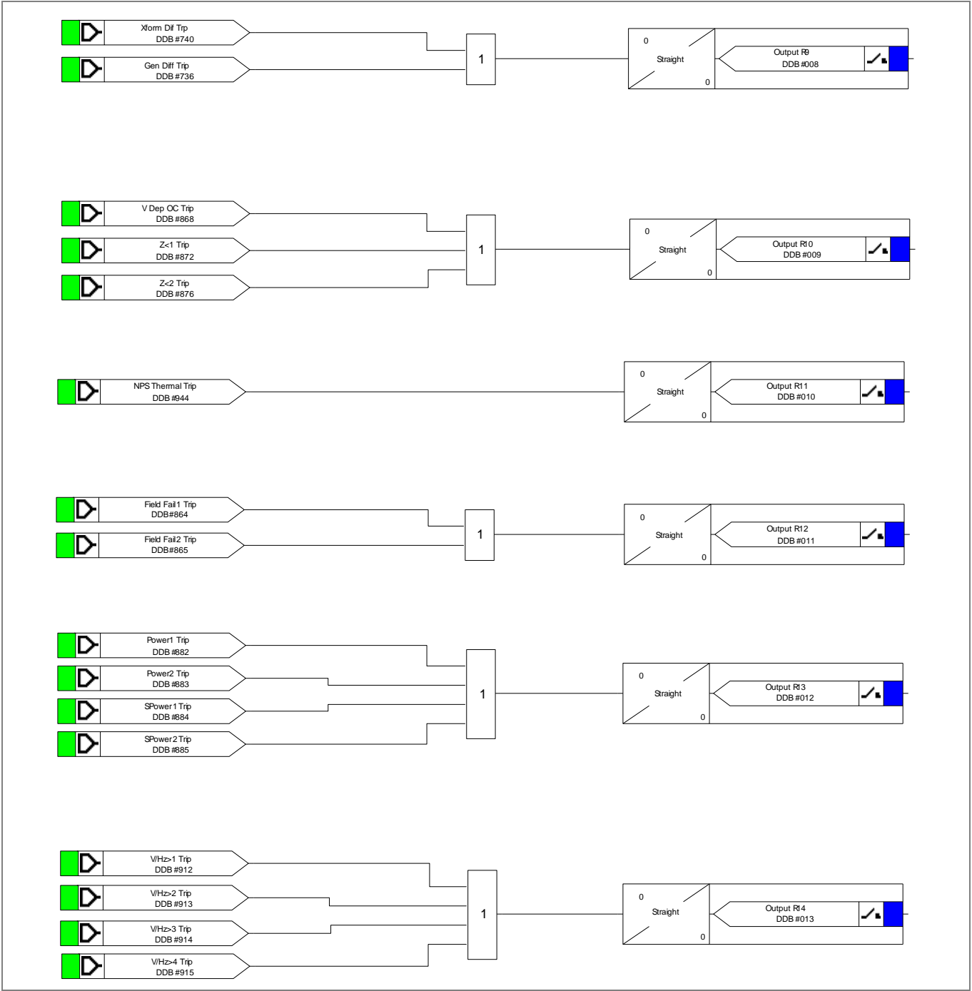
Figure 30 - Output relay mappings
