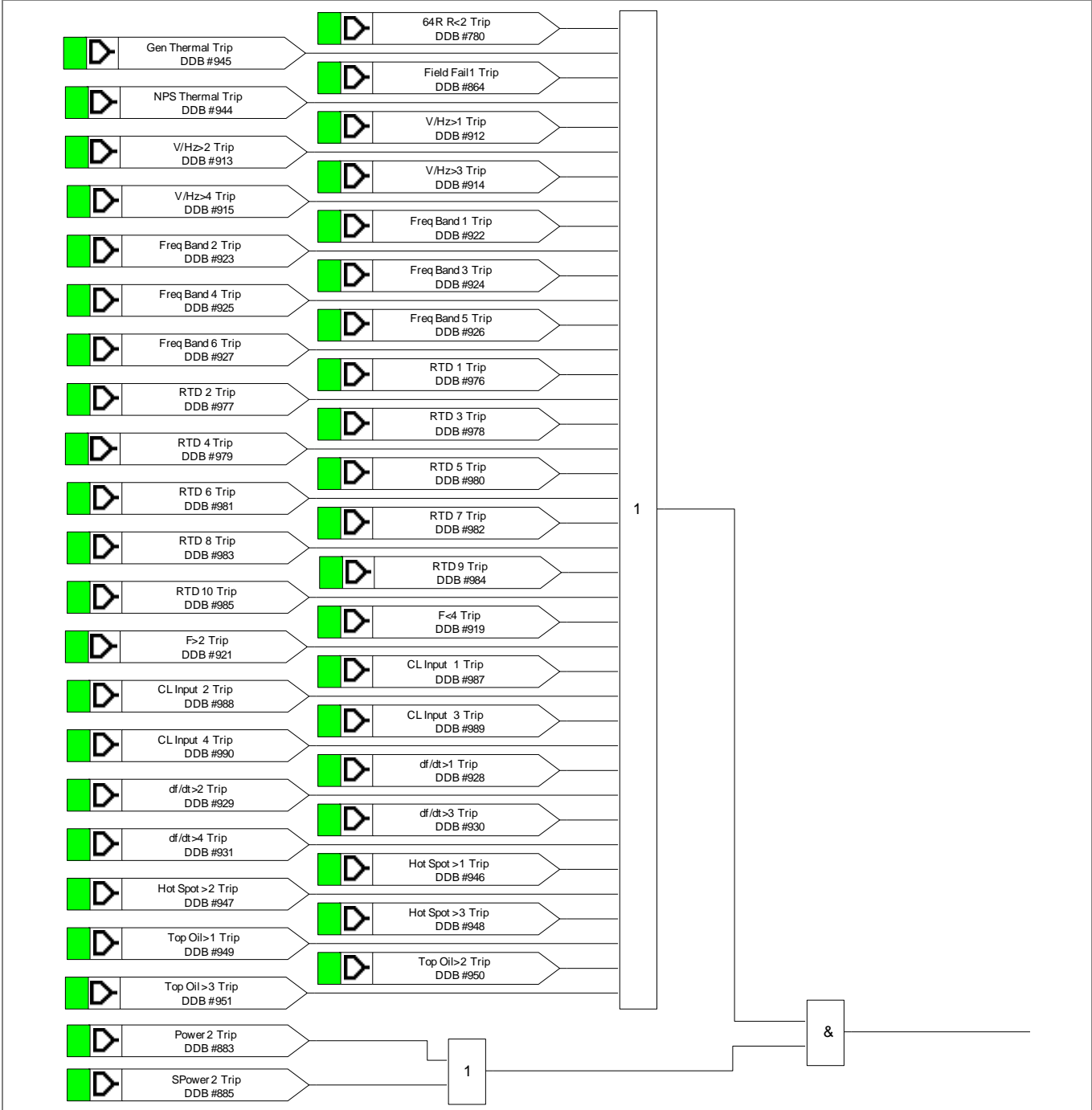
Figure 10 - Output relay R1 (Trip CB) mappings
