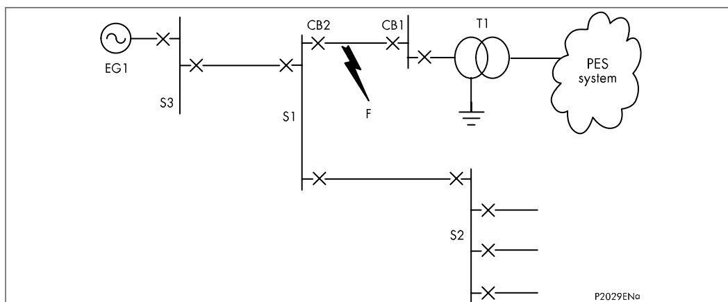
Figure 47 - Typical system with embedded generation
