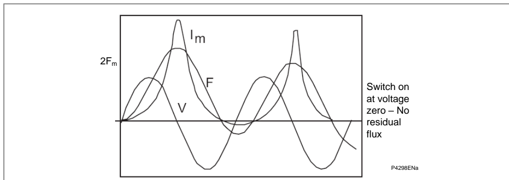
Figure 26 - Magnetizing inrush current during energization
