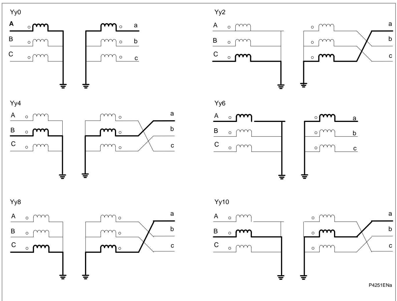
Figure 5 - Yy transformer connections
