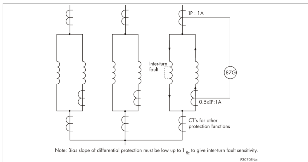
Figure 12 - Generator differential and interturn protection
