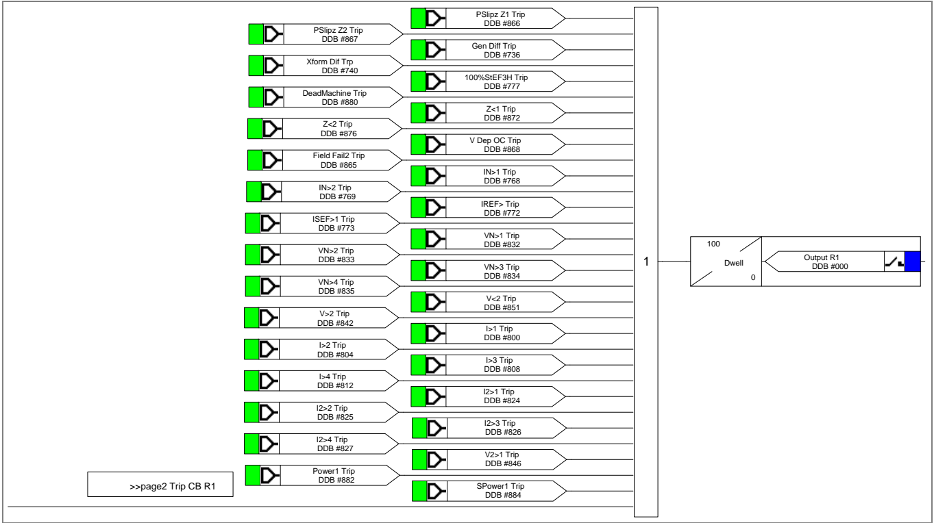
Figure 11 - Output relay R1 (Trip CB) mappings
