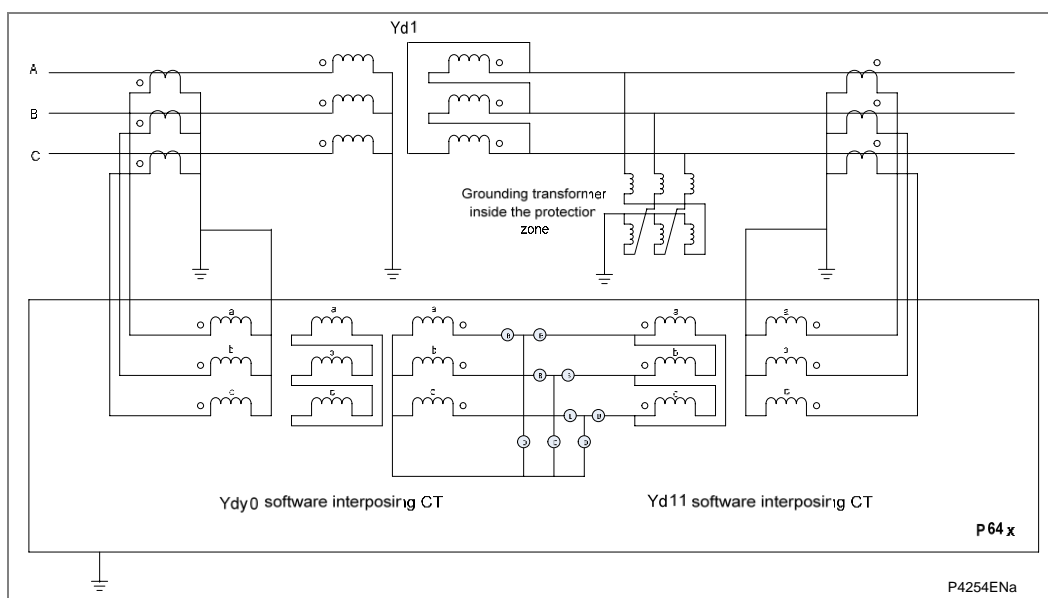
Figure 8 - Yd transformer connections
