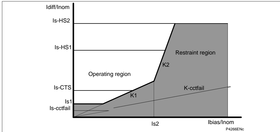
Figure 19 - Relay triple slope (flat, K1, K2) biased differential protection
