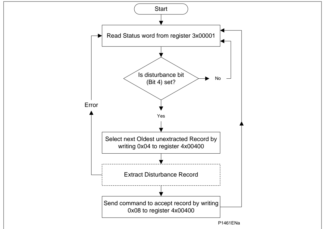
Figure 11 - Automatic selection of a disturbance - option 1
