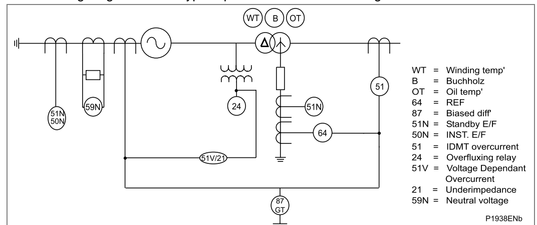
Figure 5 - Typical protection package for a generator-transformer
