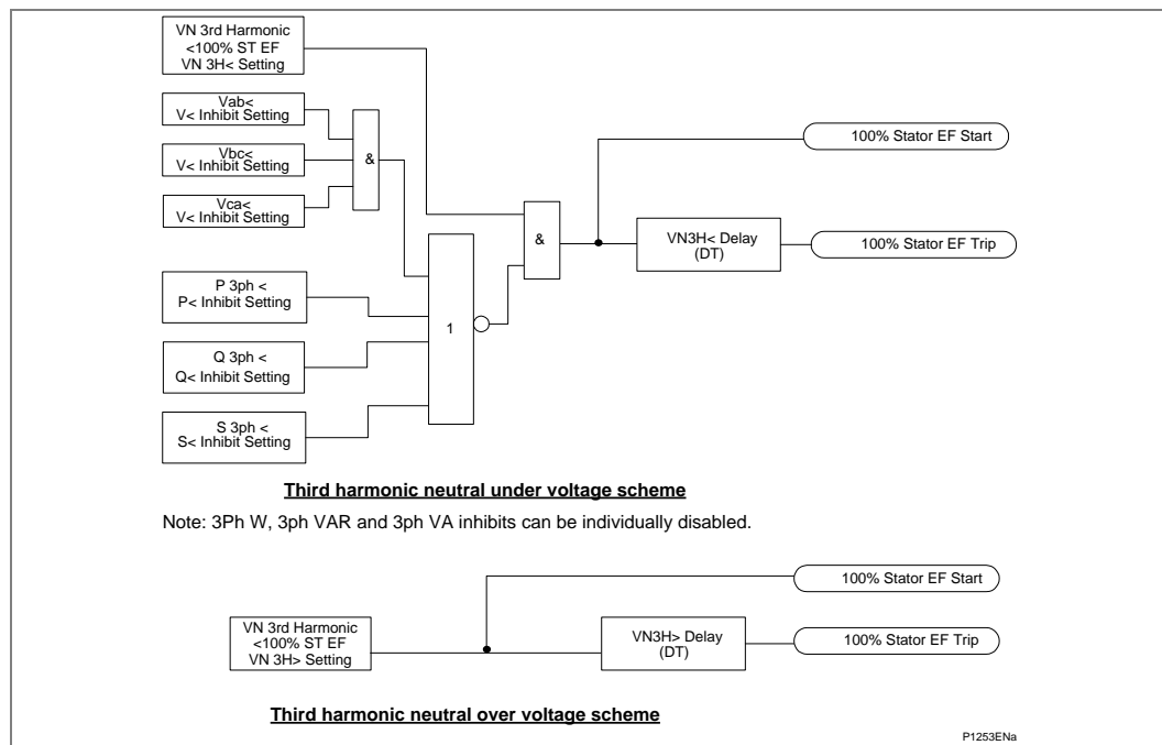
Figure 54 - 100% stator earth fault protection block diagram
