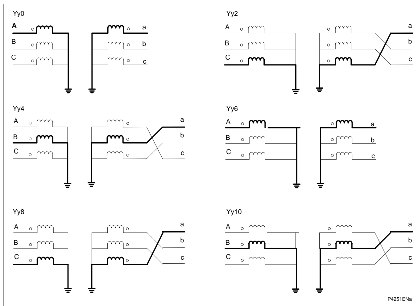
Figure 10 - Yy transformer connections
