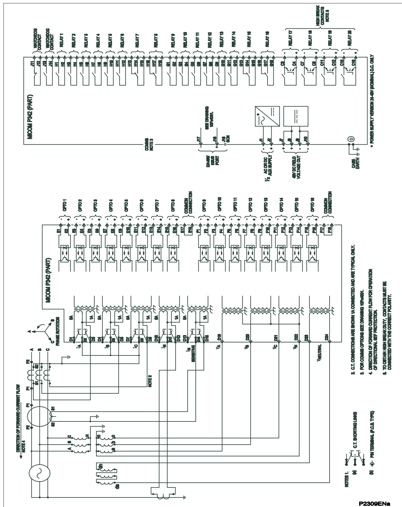
Figure 20 - P342 (60TE) for small generator (16 I/P &amp; 20 O/P (4HB))
