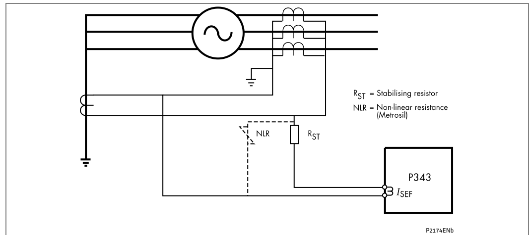
Figure 53 - Relay connections for high impedance REF protection
