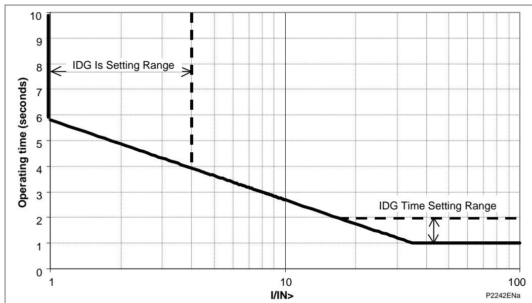
Figure 4 - IDG Characteristic
