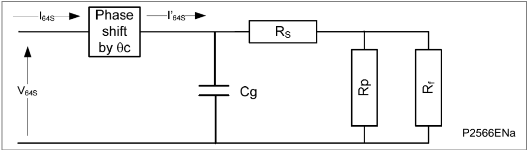
Figure 14 - Calibration model for the 64S
