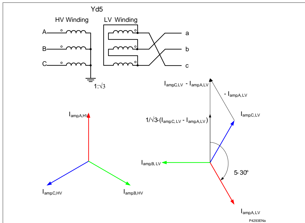
Figure 21 - Yd5 transformer example
