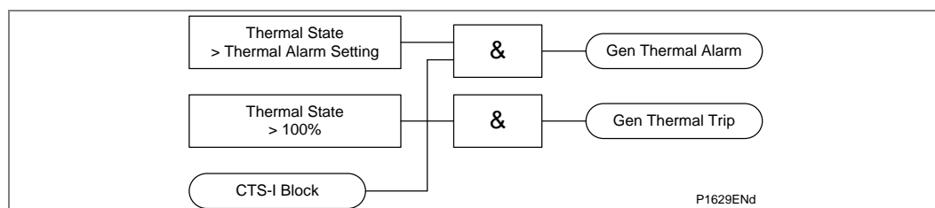
Figure 72 - Thermal overload protection logic diagram
