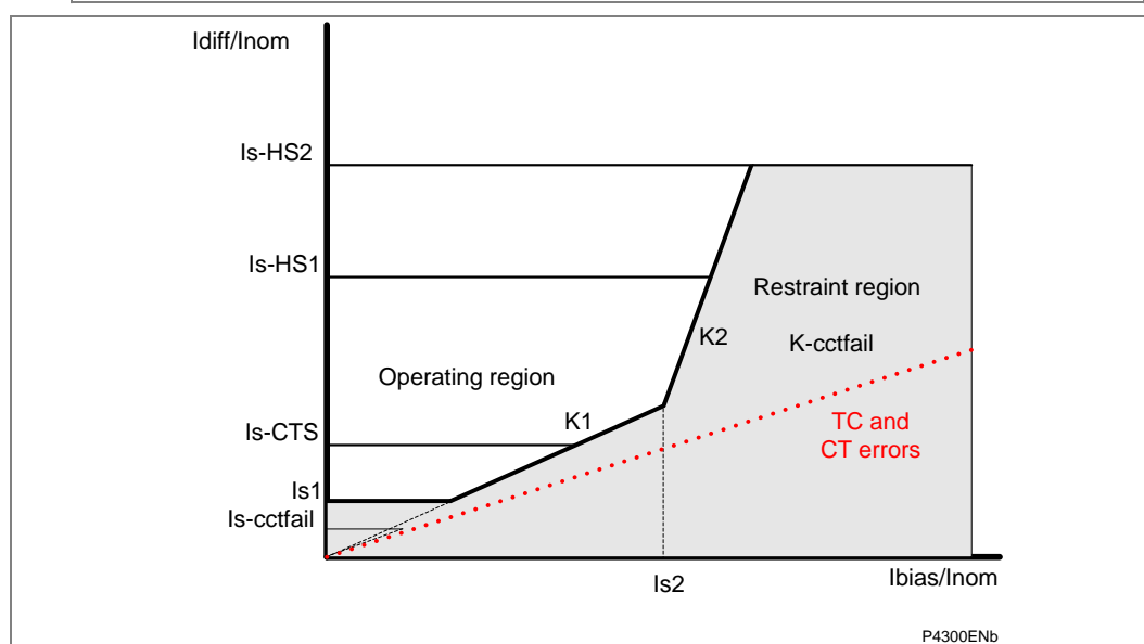
Figure 28 - Tap changer and CT combined errors
