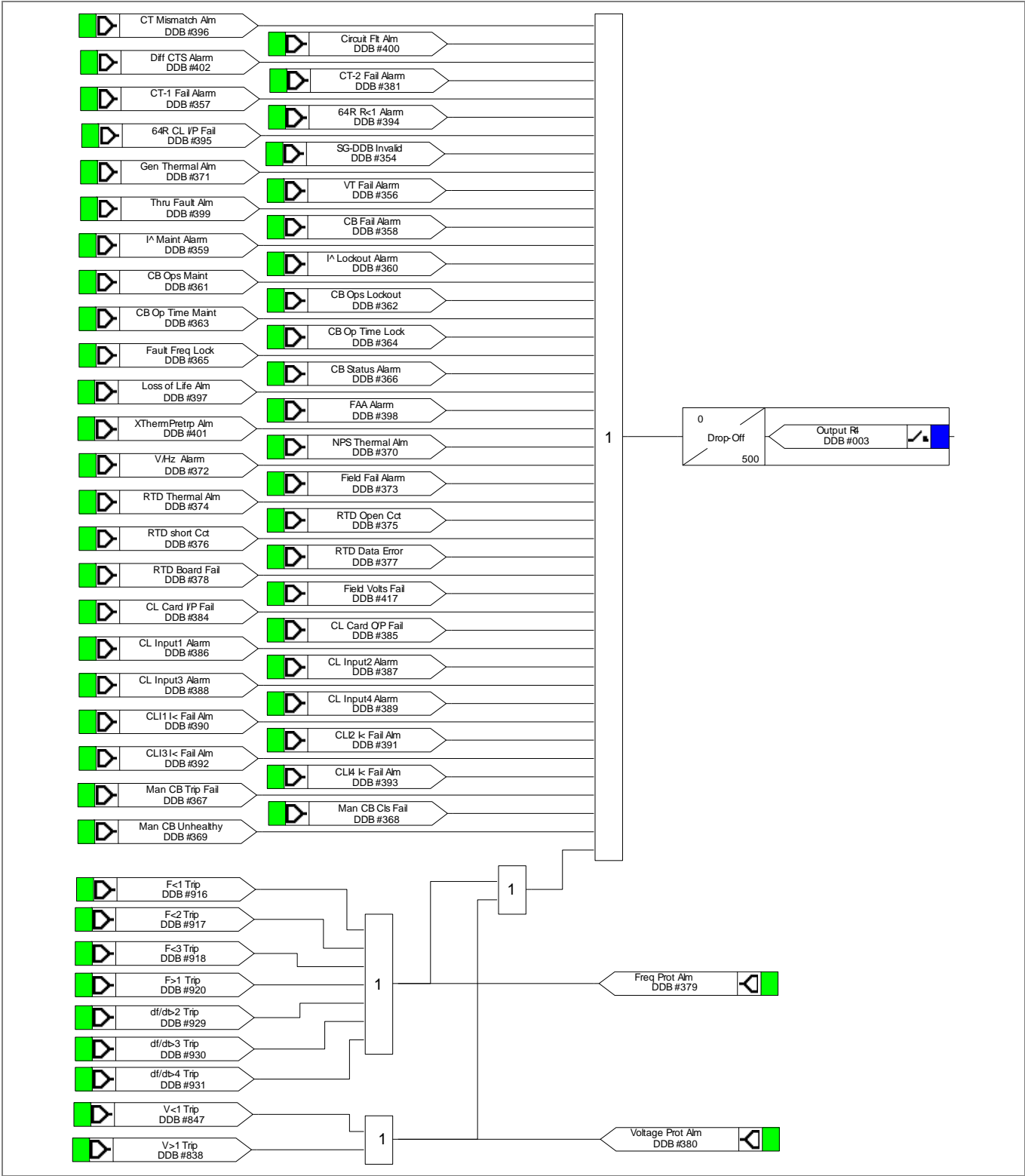
Figure 28 - Output relay mappings
