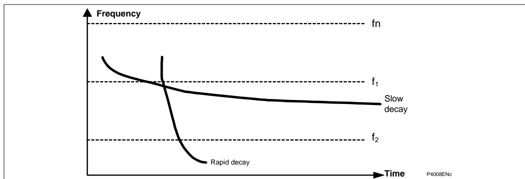
Figure 46 - Rate of change of frequency protection
