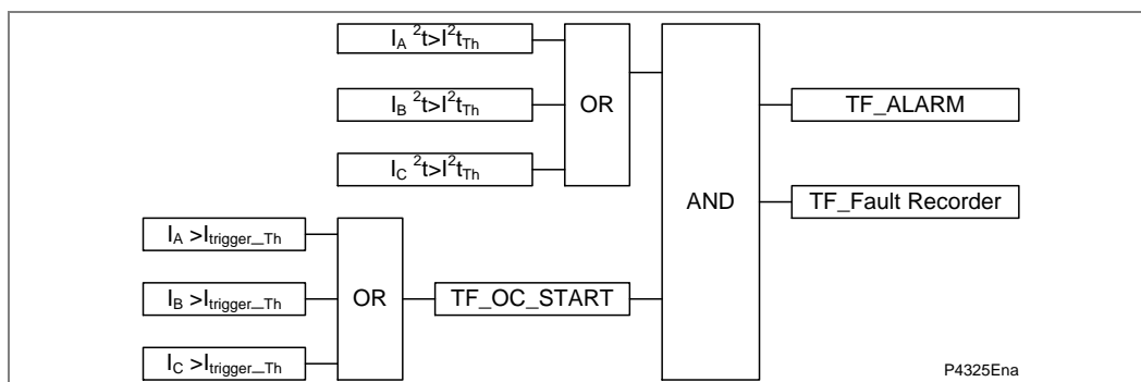
Figure 73 - Through fault monitoring logic
