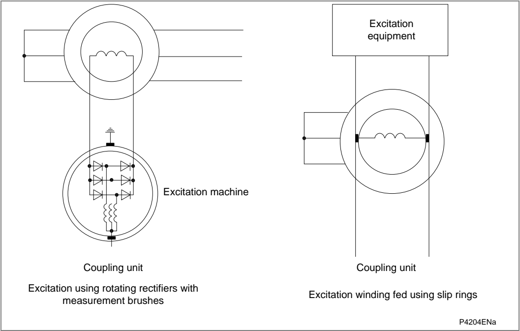
Figure 17 - Types of excitation
