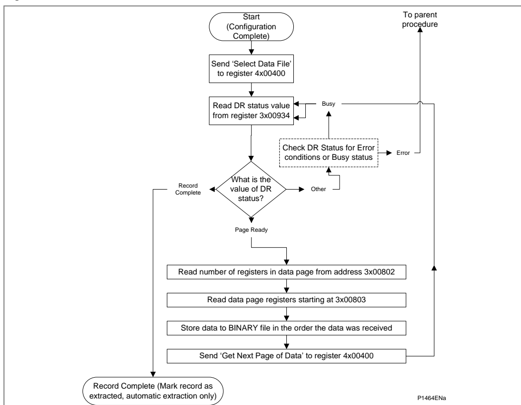
Figure 14 - Extracting the COMTRADE binary data file
