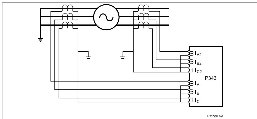
Figure 4 - Relay connections for biased differential protection
