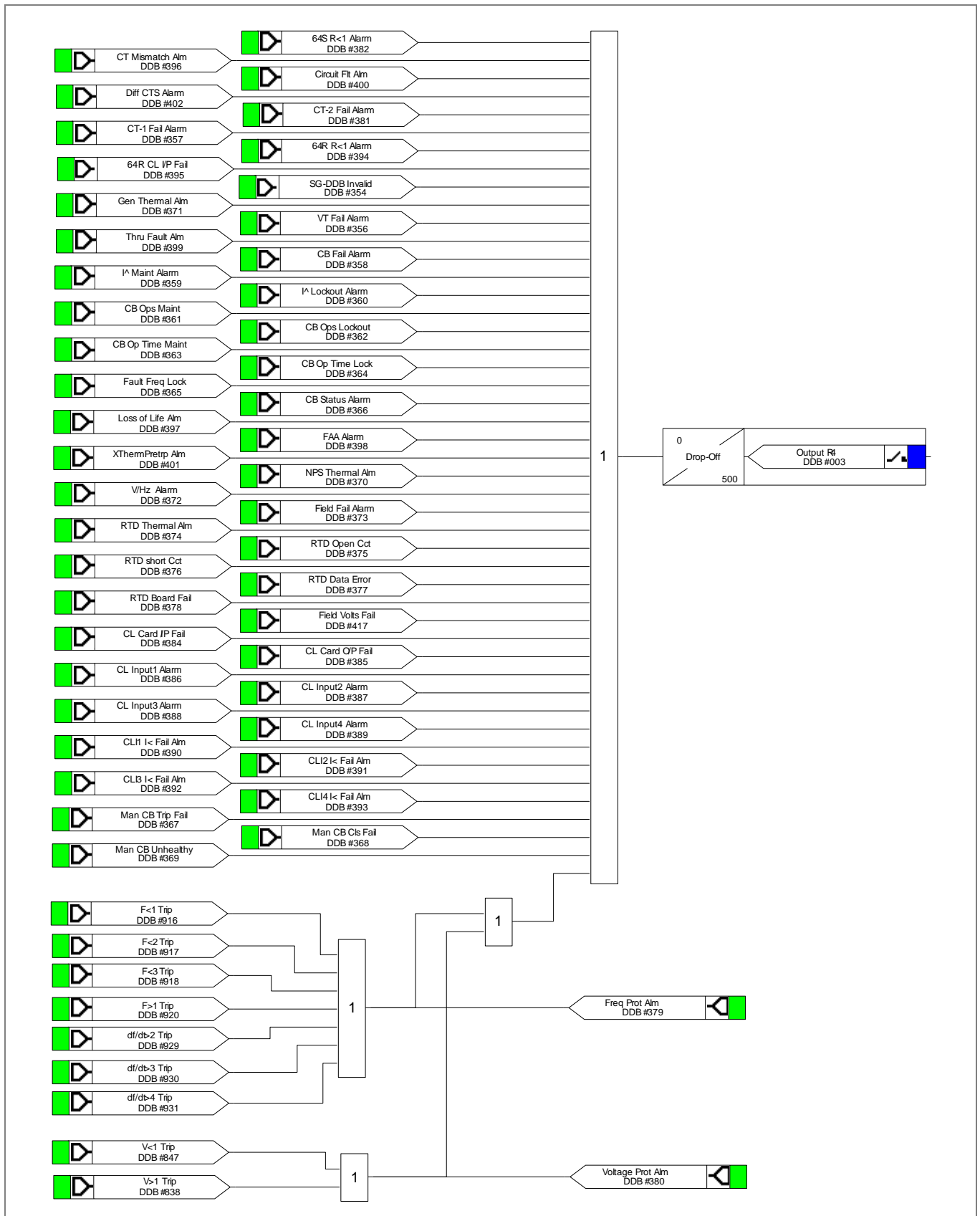
Figure 41 - Output relay mappings
