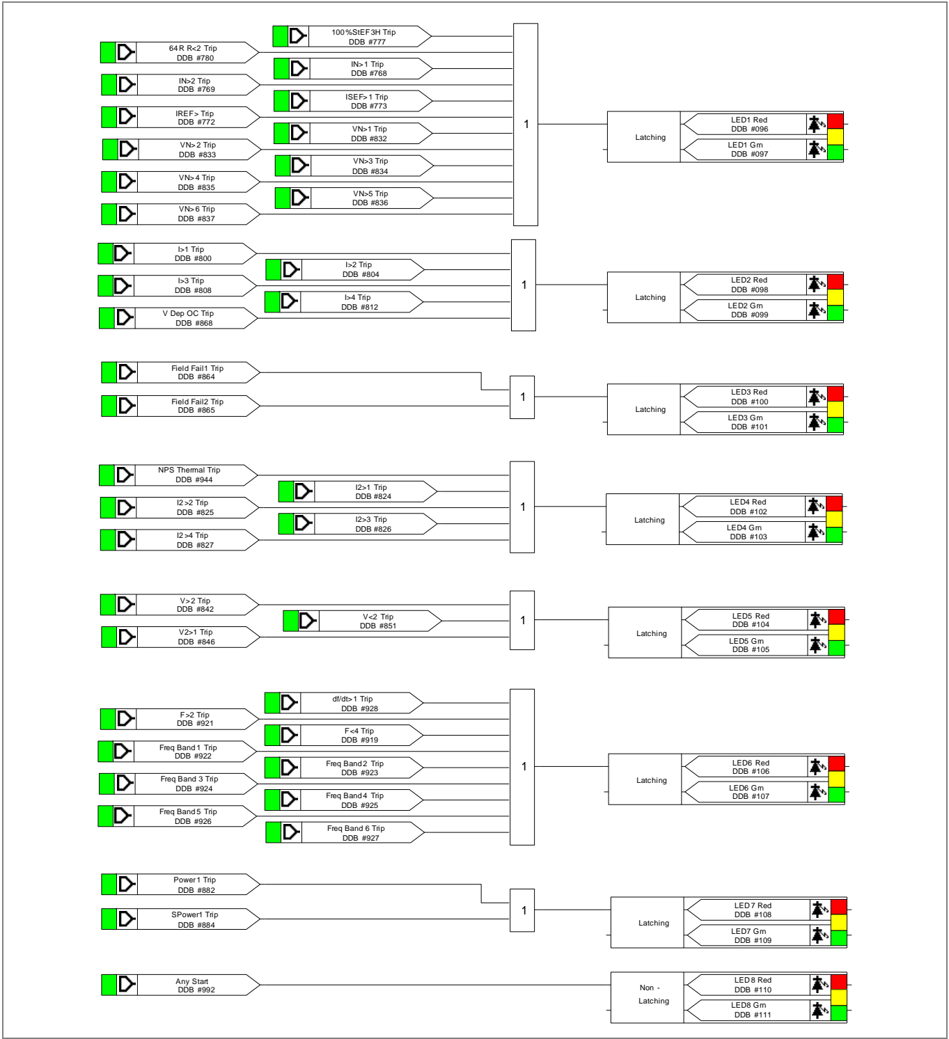
Figure 32 - LED output mapping
