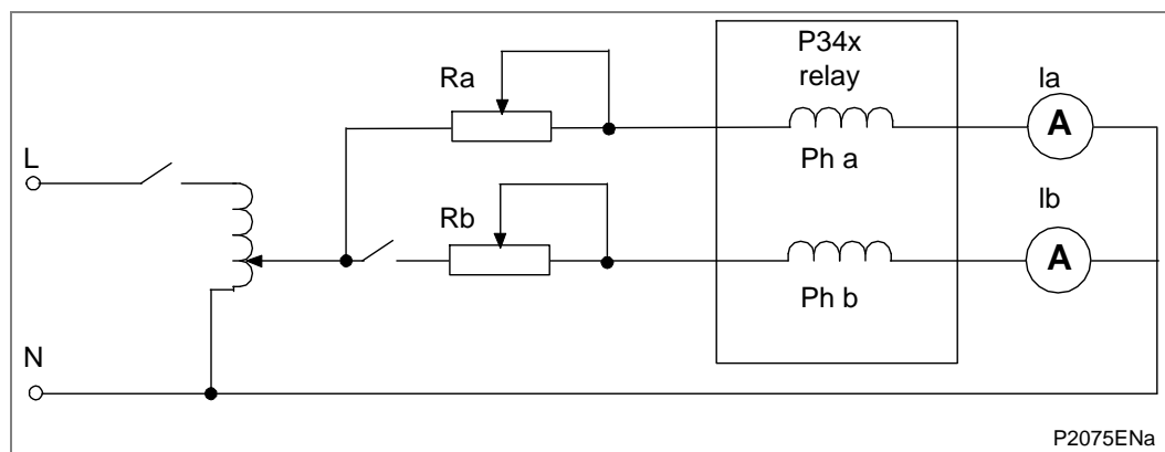
Figure 3 - Connection for testing
