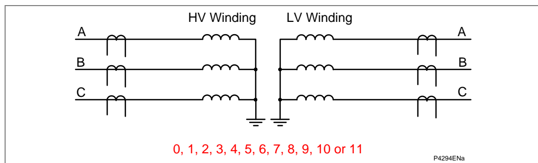
Figure 22 - Vector group selection
