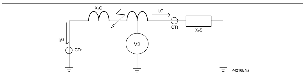
Figure 17 - Negative sequence diagram for internal fault
