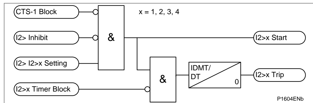
Figure 23 - Negative sequence overcurrent non-directional operation
