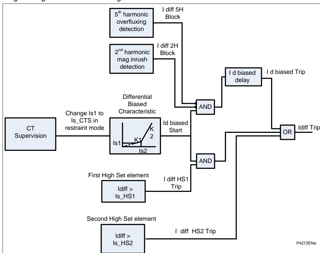
Figure 19 - Differential protection
