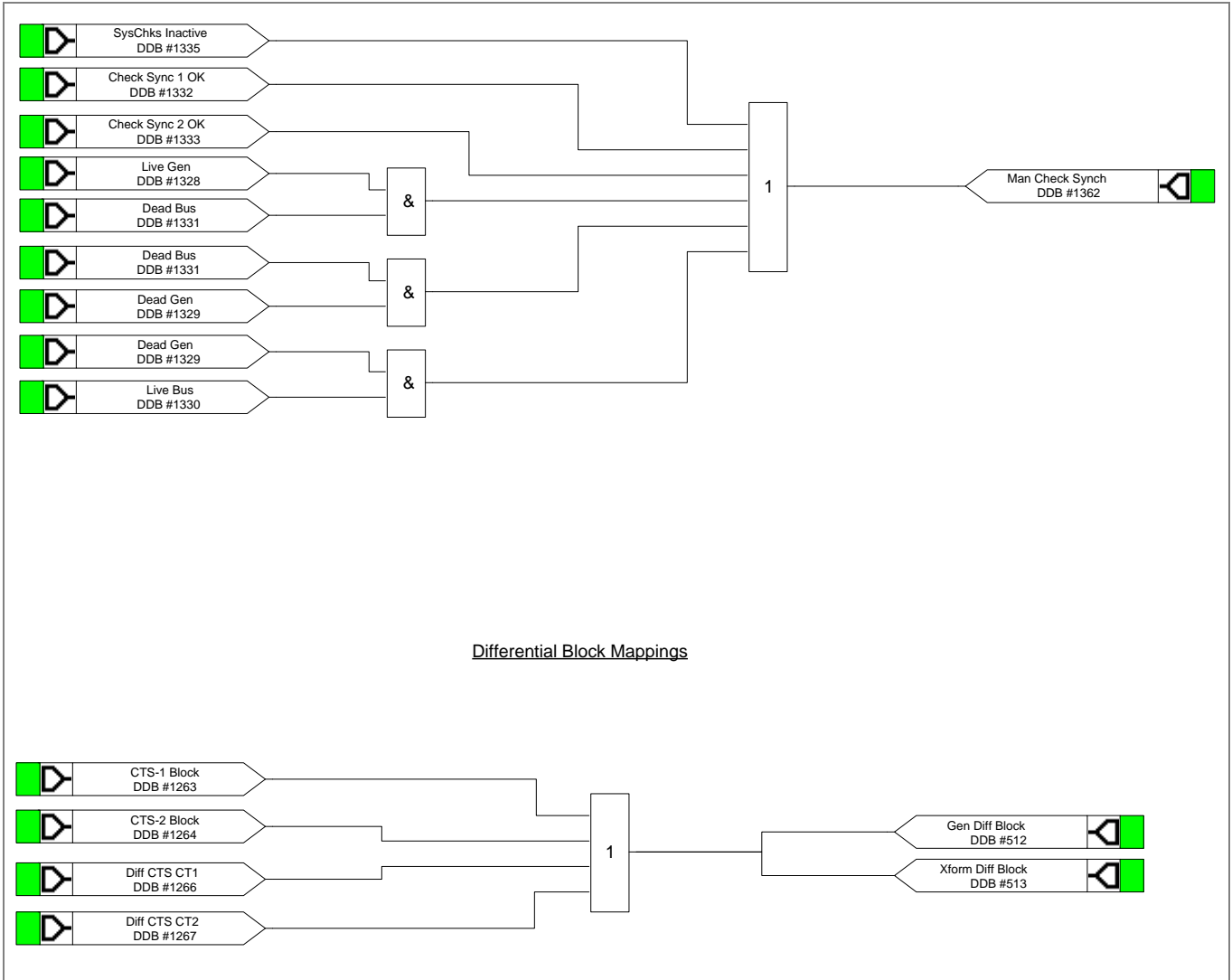
Figure 33 - Check synch and voltage monitor mapping
