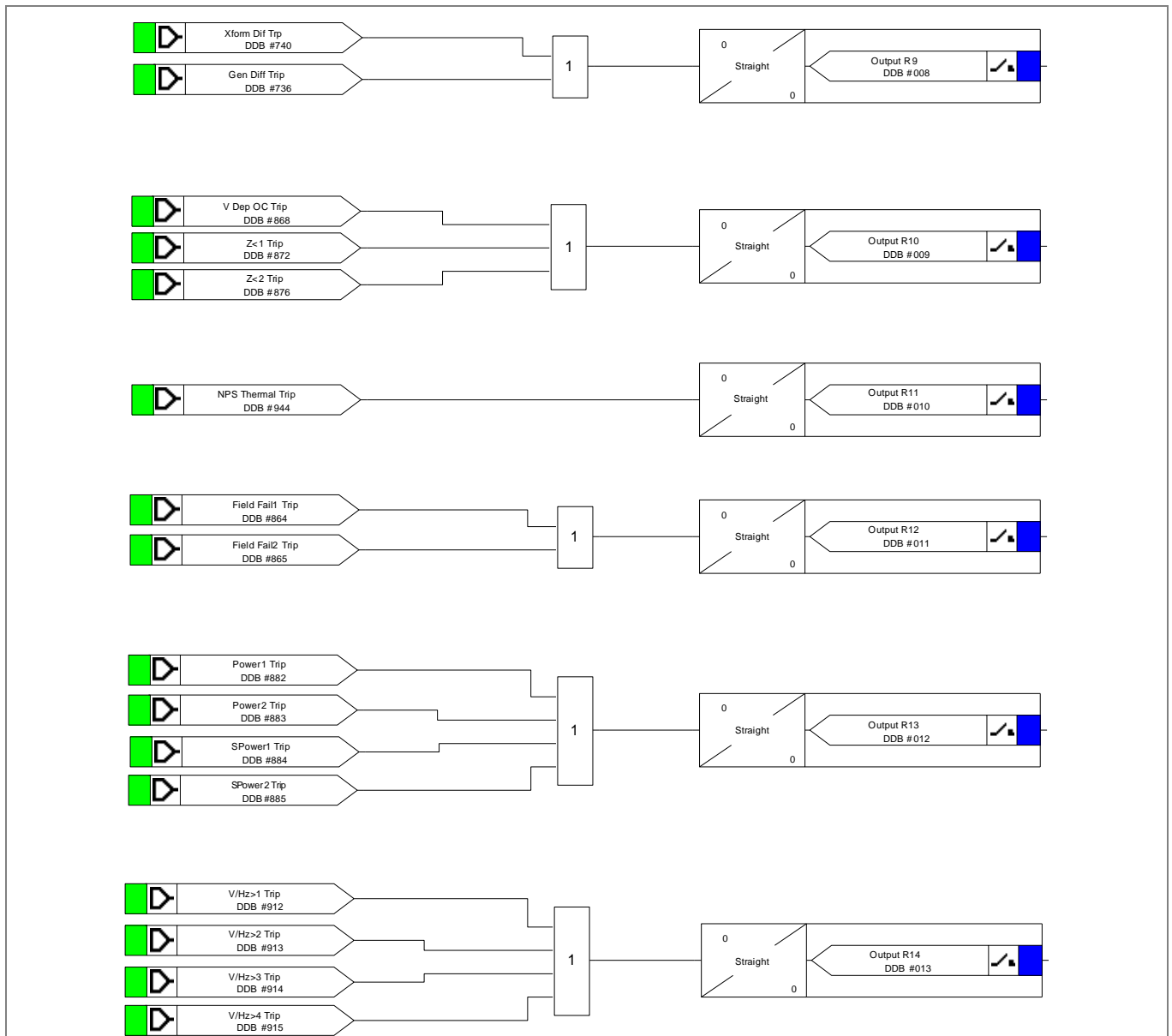
Figure 17 - Output relay mappings
