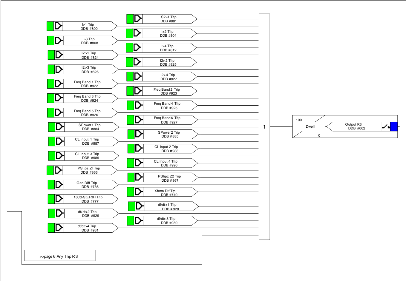
Figure 40 - Output relay mappings
