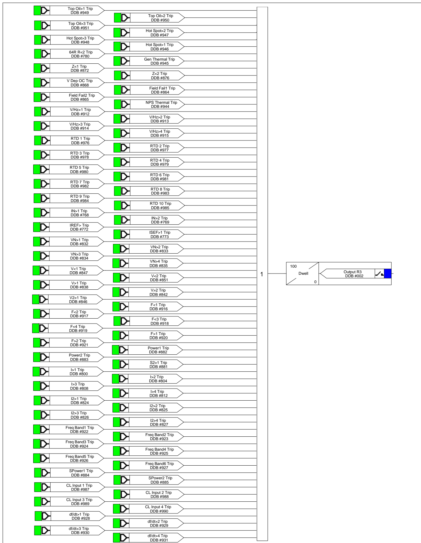
Figure 4 - Output relay R3 (Any Trip) mappings
