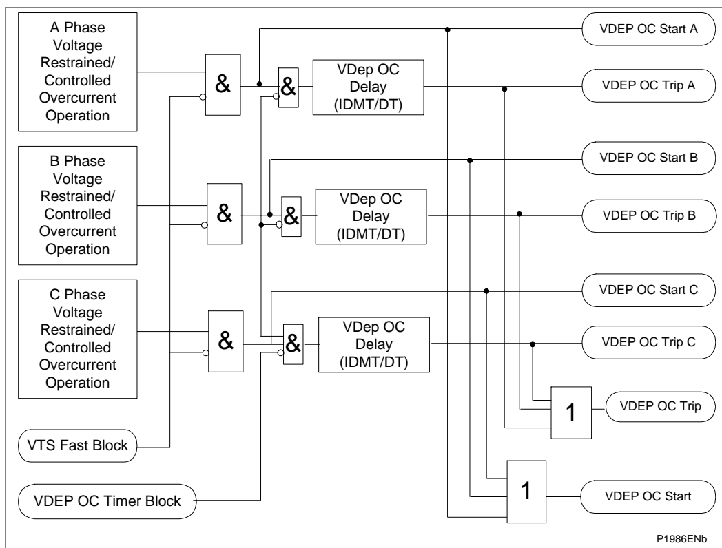
Figure 25 - Voltage restrained / controlled overcurrent logic diagram
