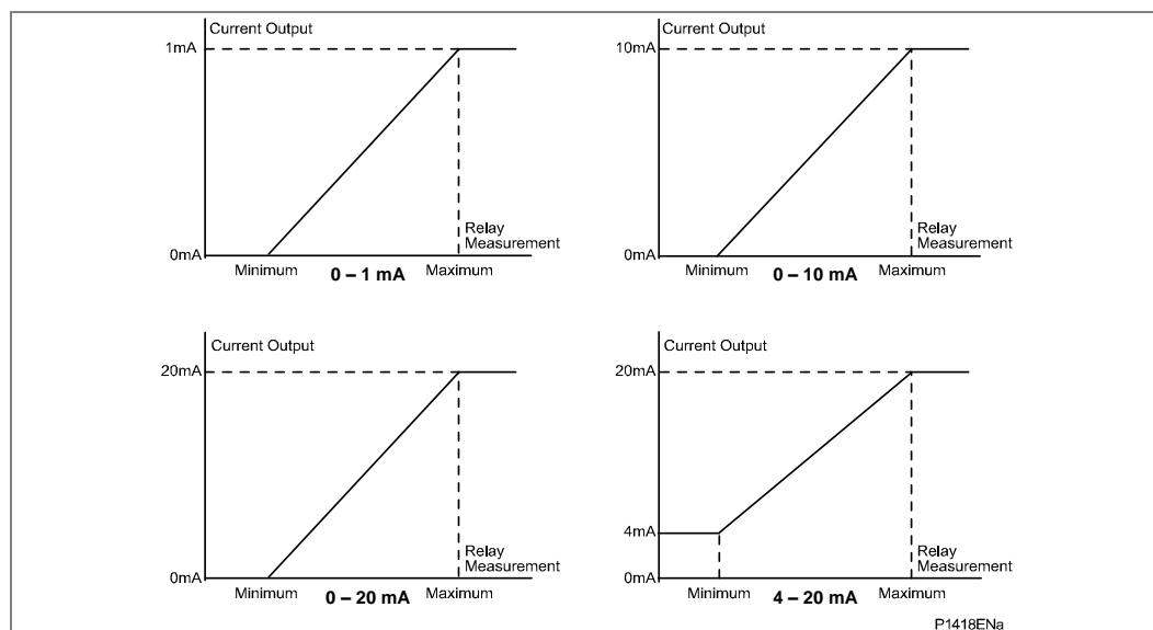
Figure 77 - Relationship between the current output and the relay measurement
