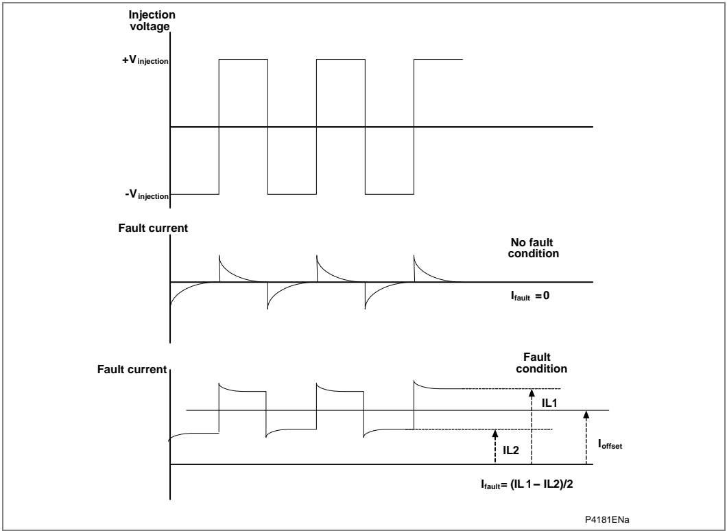
Figure 79 - Waveforms for calculating the fault current
