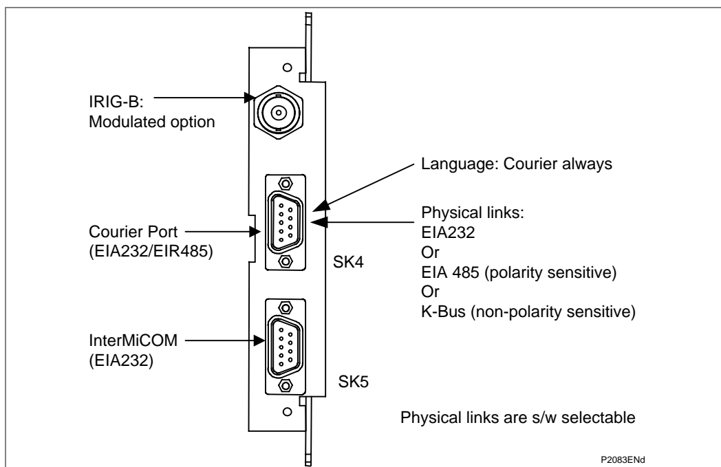
Figure 5 - Rear communications port
