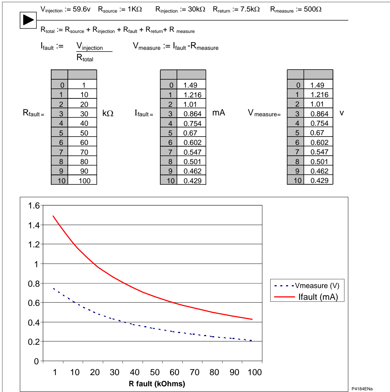
Figure 81 - Relationship between fault current and fault resistance
