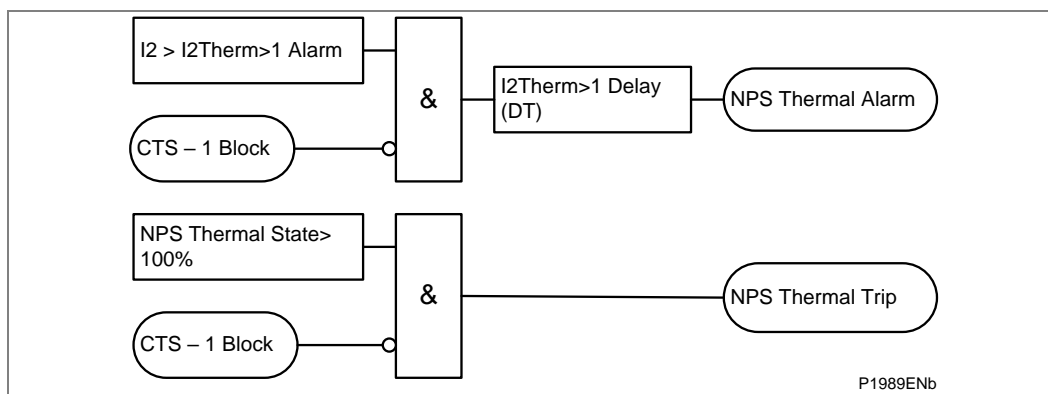
Figure 40 - NPS thermal logic diagram
