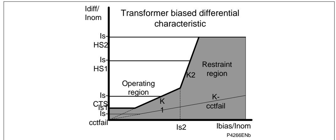
Figure 13 - Tripping characteristic of differential protection
