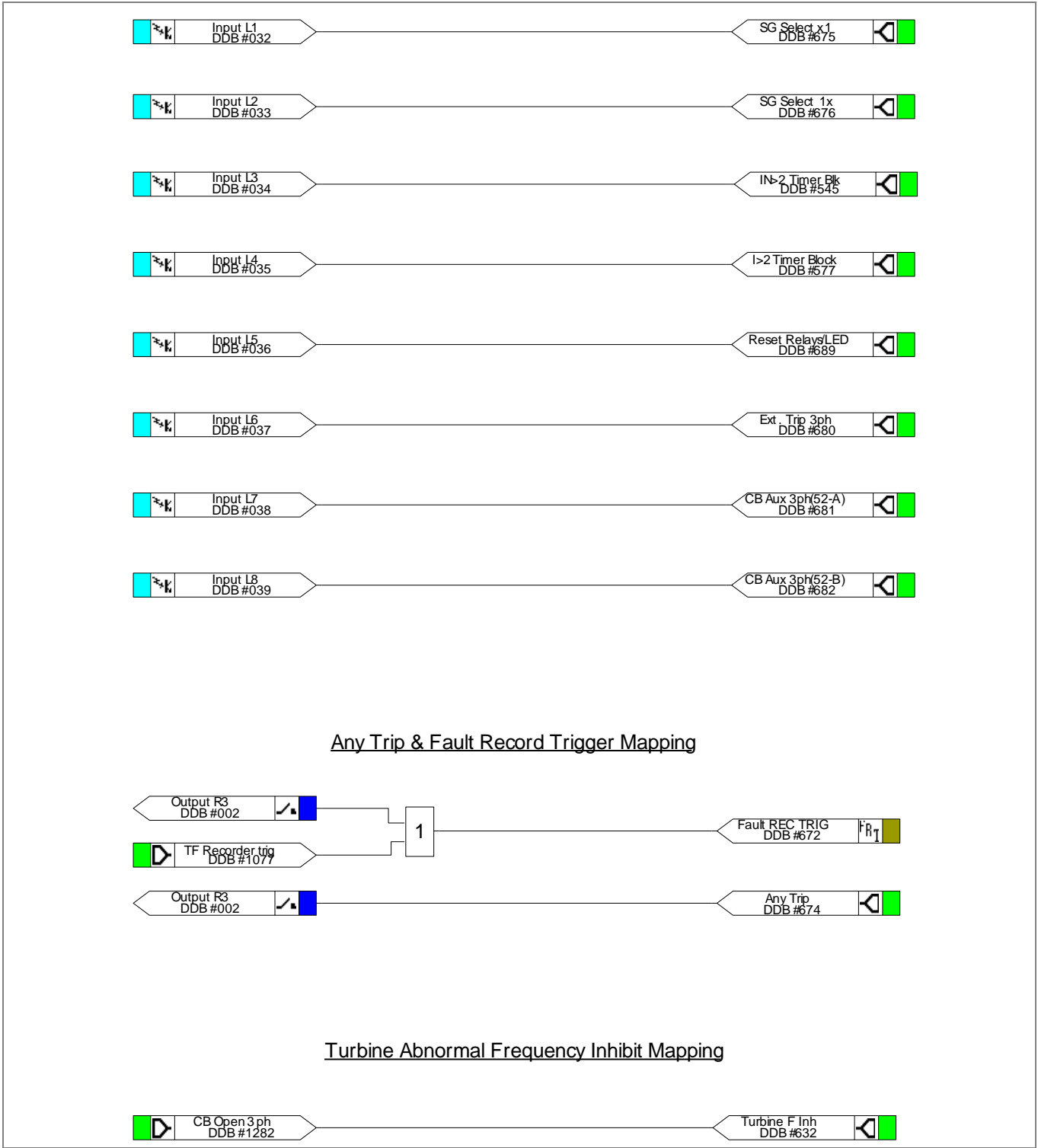
Figure 9 - Opto input mappings
