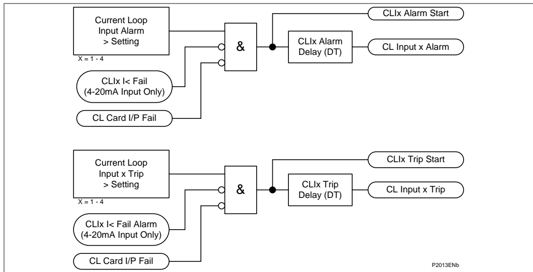
Figure 76 - Current loop input logic diagram
