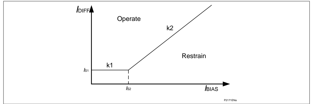
Figure 50 - REF biased principle
