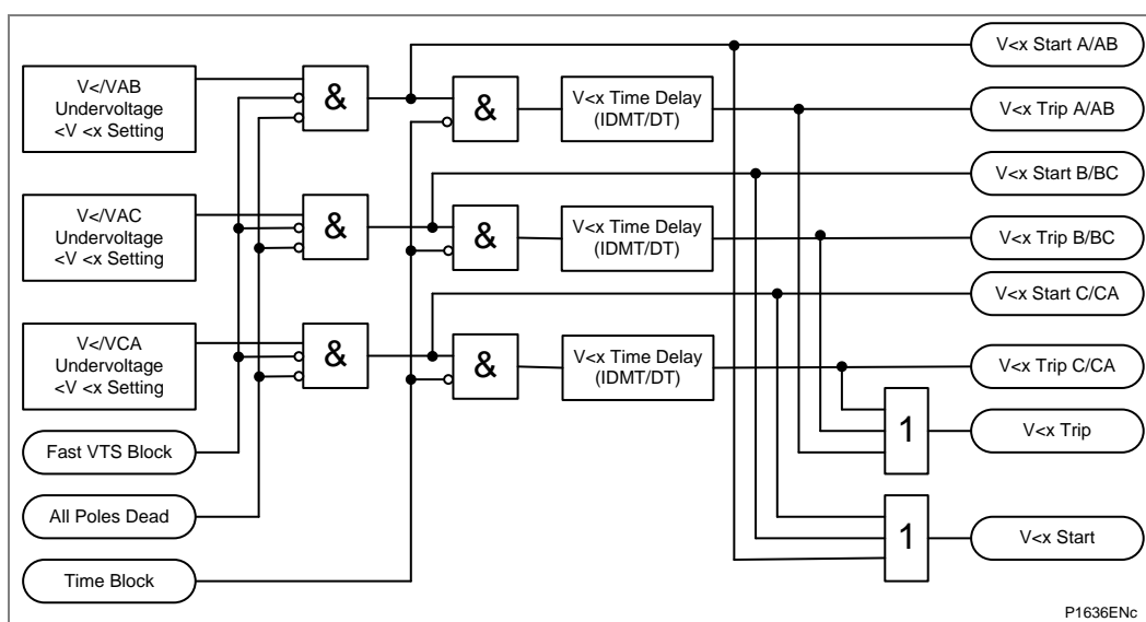
Figure 30 - Undervoltage - single and three phase tripping mode (single stage)
