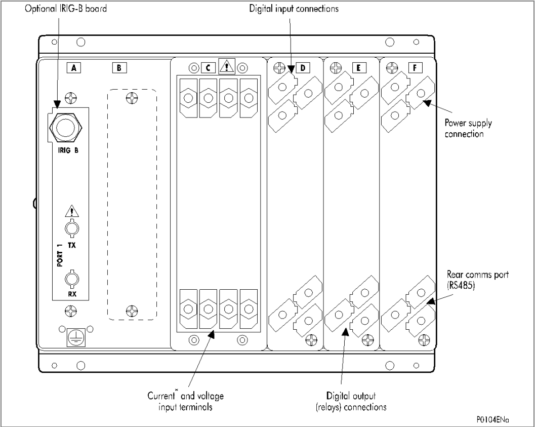
Figure 3 - Relay rear view (40TE case)
