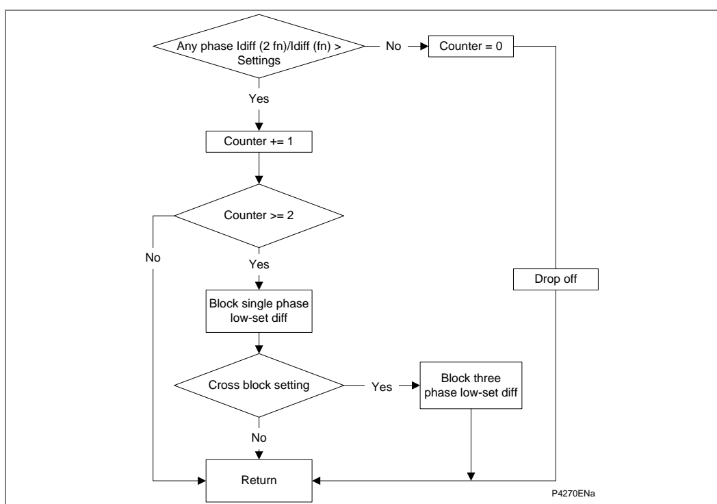
Figure 17 - Inrush stabilization (second harmonic blocking)
