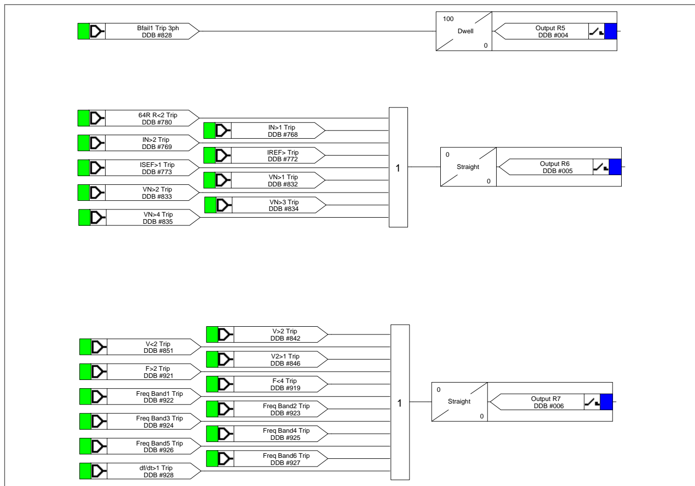
Figure 6 - Output relay mappings
