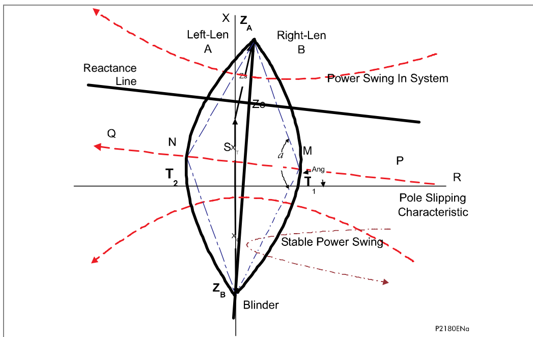
Figure 53 - Lenticular scheme characteristic
