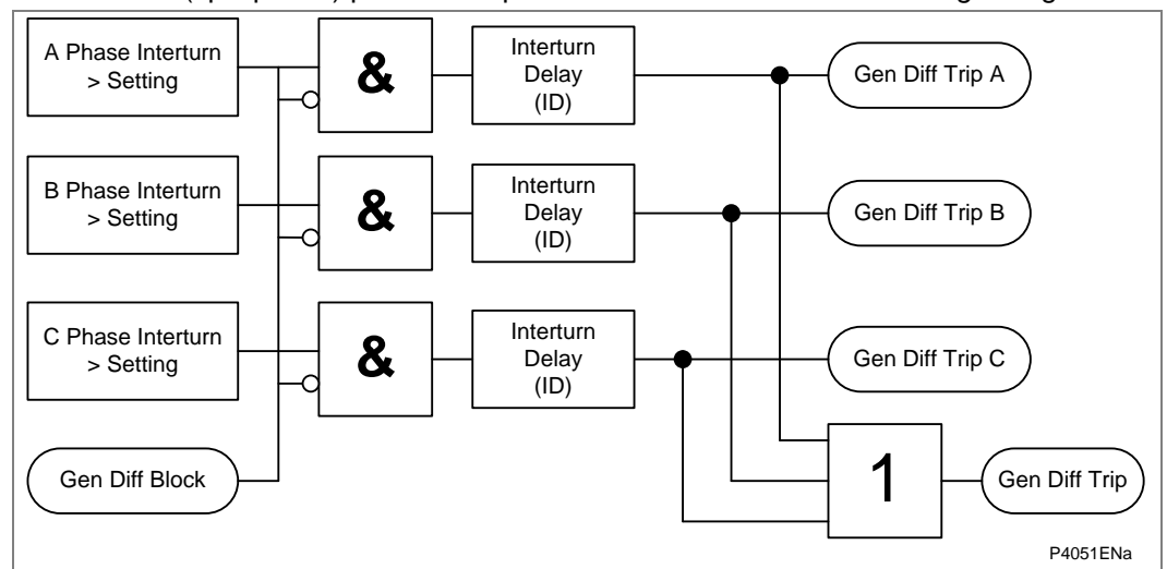
Figure 7 - Interturn logic diagram
