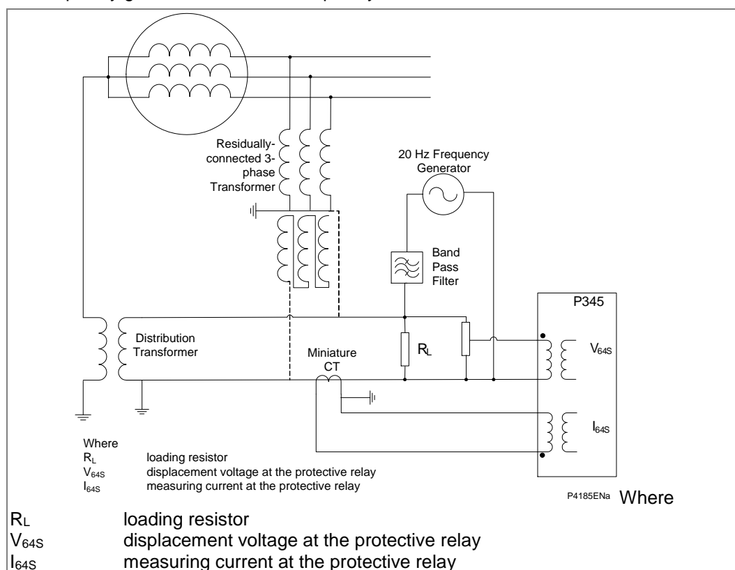
Figure 38 - 100% stator earth fault protection with earthing (broken delta) transformer or neutral transformer
