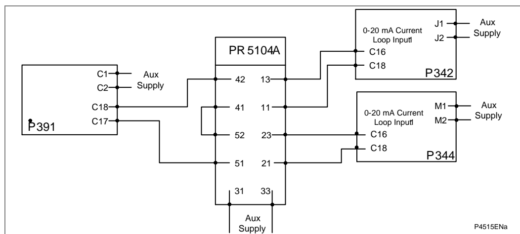
Figure 61 - Redundant rotor earth fault connection
