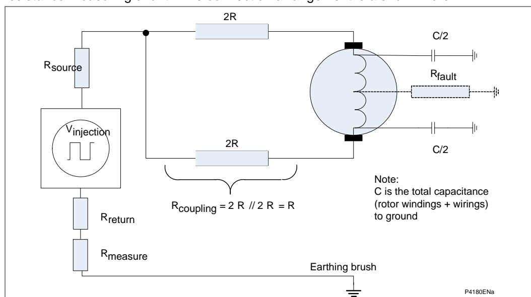
Figure 78 - Rotor earth fault protection low frequency injection arrangement
