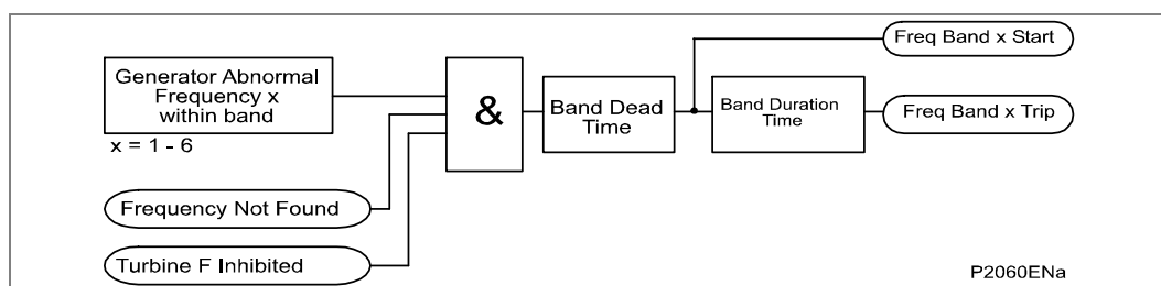
Figure 36 - Generator turbine abnormal frequency logic diagram
