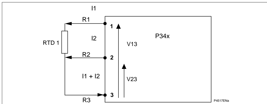
Figure 66 - Principle of RTD connection
