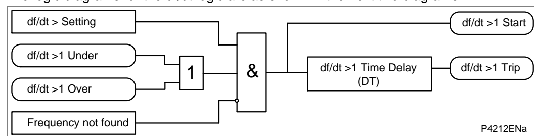
Figure 61 - Rate of change of frequency logic diagram for df/dt>1
