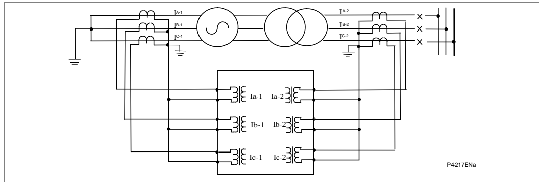
Figure 18 - P34x & P391 typical connection for generator-transformer unit connection
