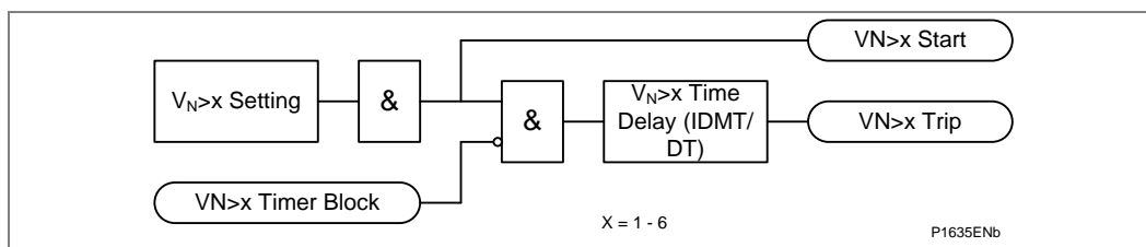
Figure 46 - Residual overvoltage logic (single stage)
