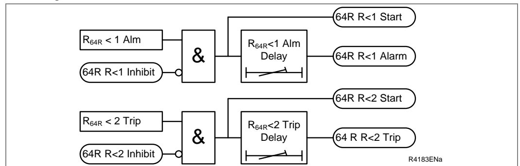
Figure 83 - Rotor earth fault protection block diagram
