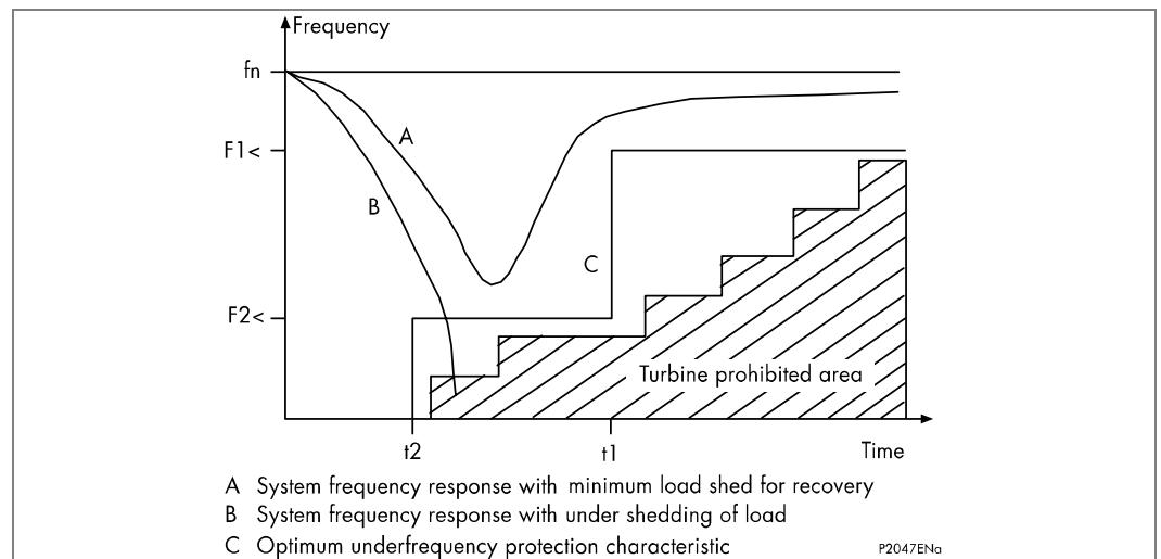
Figure 34 - Coordination of underfrequency protection function with system load shedding
