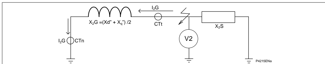
Figure 16 - Negative sequence diagram for external fault
