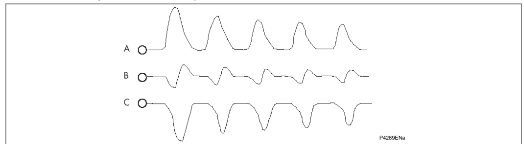
Figure 16 - Magnetizing inrush current waveforms
