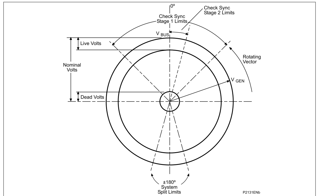
Figure 84 - Synchro check and synchro split functionality
