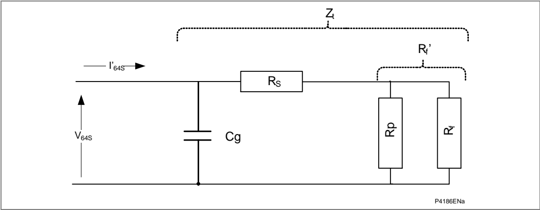
Figure 57 - Model for 100% stator earth fault by injection
