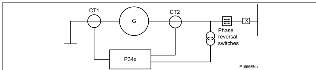
Figure 6 - Case 1 - phase reversal switches affecting all CTs and VTs
