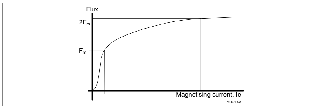
Figure 14 - Transformer magnetizing characteristic
