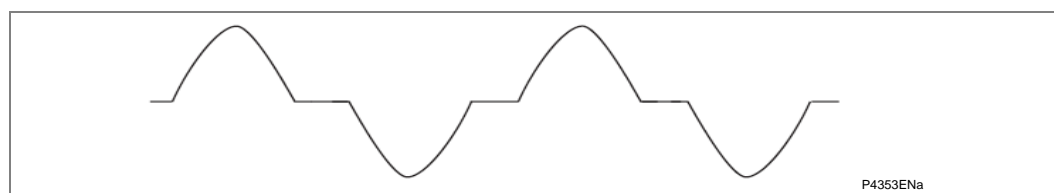
Figure 45 - Typical overflux current waveform
