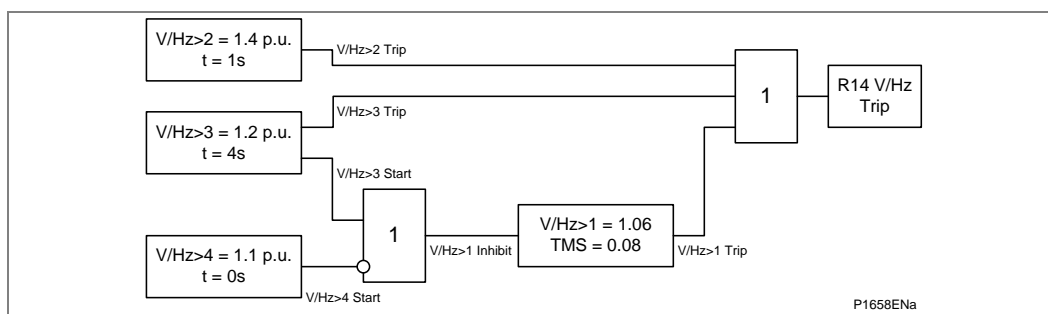
Figure 42 - Scheme logic for large generator multi-stage overfluxing characteristic
