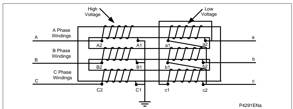
Figure 4 - Yd1 transformer configuration
