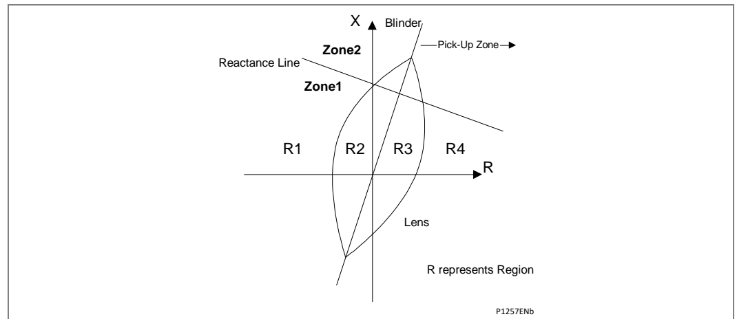
Figure 71 - Regions and zones definition (motoring mode)
