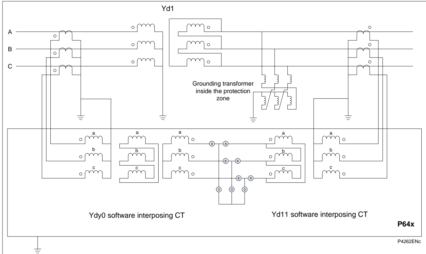
Figure 9 - Software interposing CTs for a Yd1 transformer
