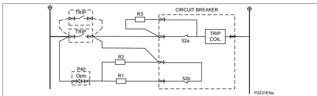
Figure 72 - TCS scheme 2
