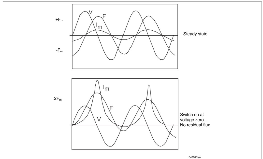
Figure 15 - Magnetizing inrush phenomenon
