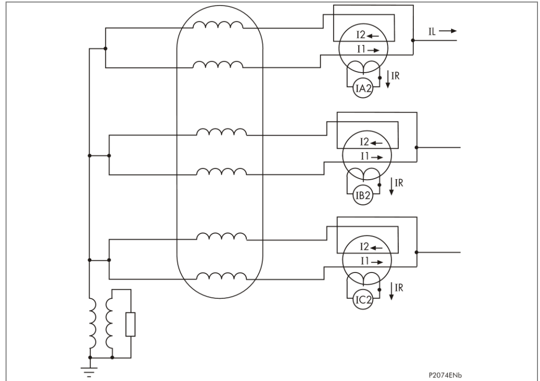
Figure 10 - Generator interturn protection using core balance (window) CTs
