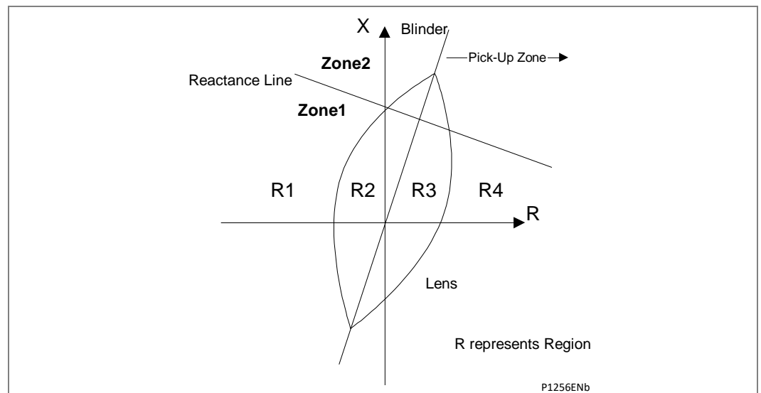
Figure 54 - Pole slipping protection using blinder and lenticular characteristic
