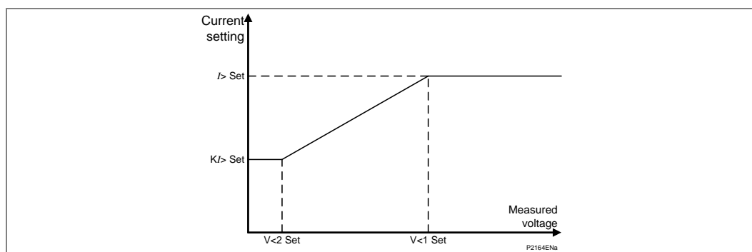
Figure 27 - Current pickup level for voltage restrained overcurrent protection
