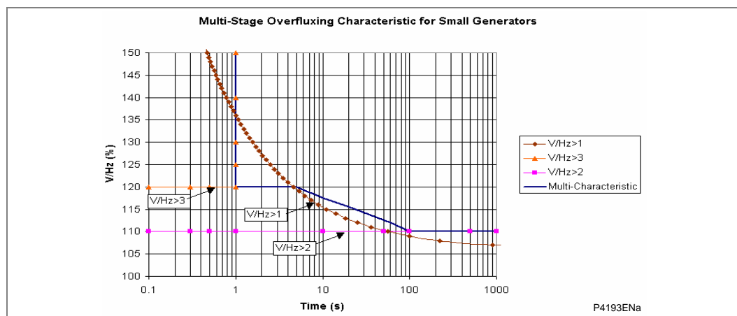
Figure 43 - Multi-stage overfluxing characteristic for small generators
