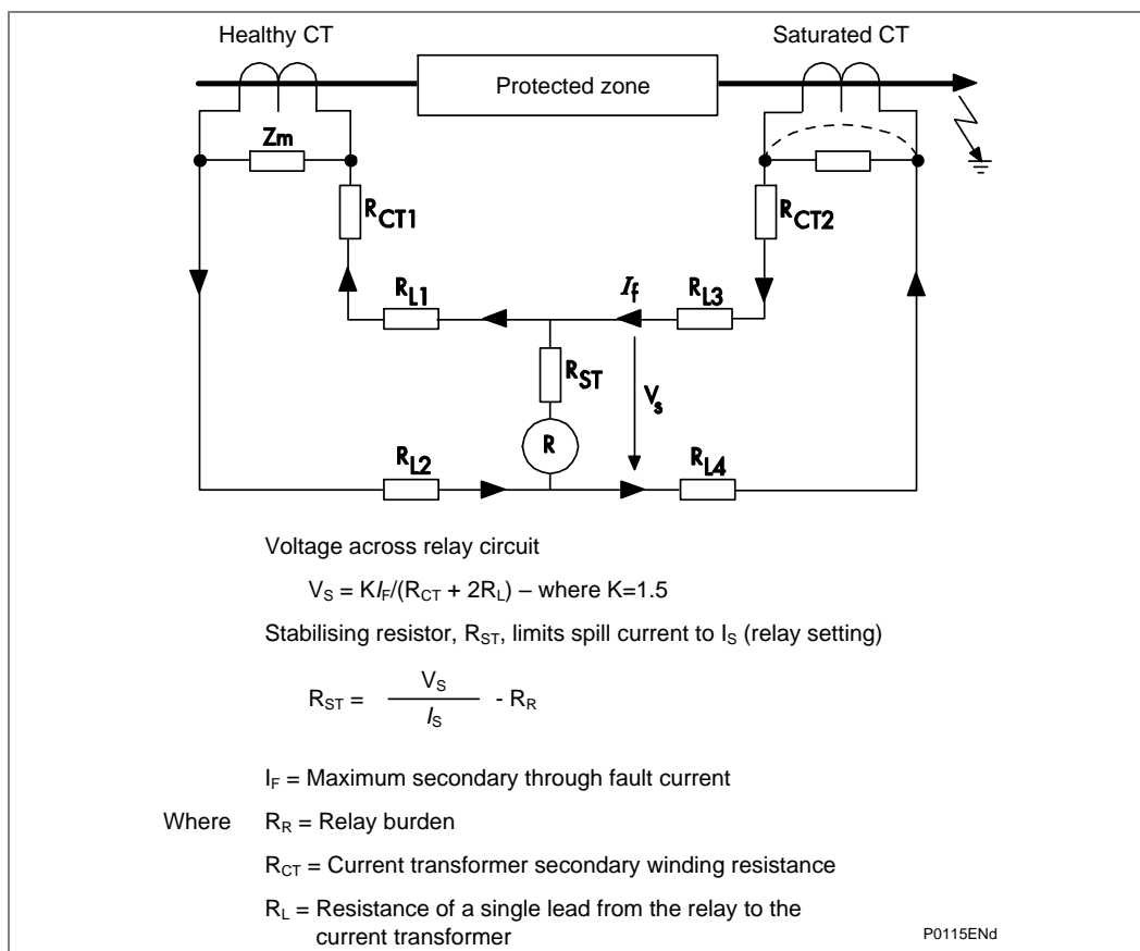
Figure 5 - Principle of high impedance differential protection
