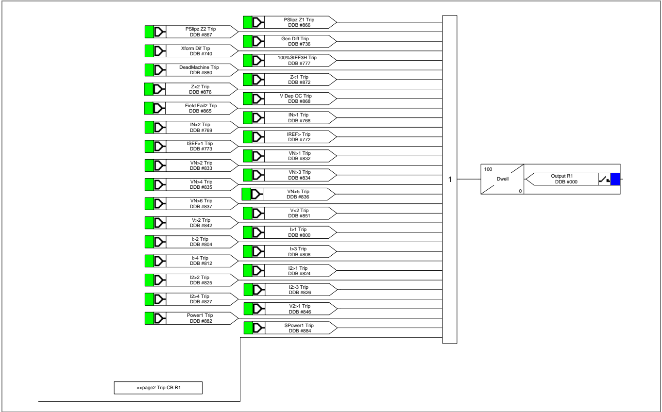
Figure 23 - Output relay R2 (Trip Prime Mover) mappings
