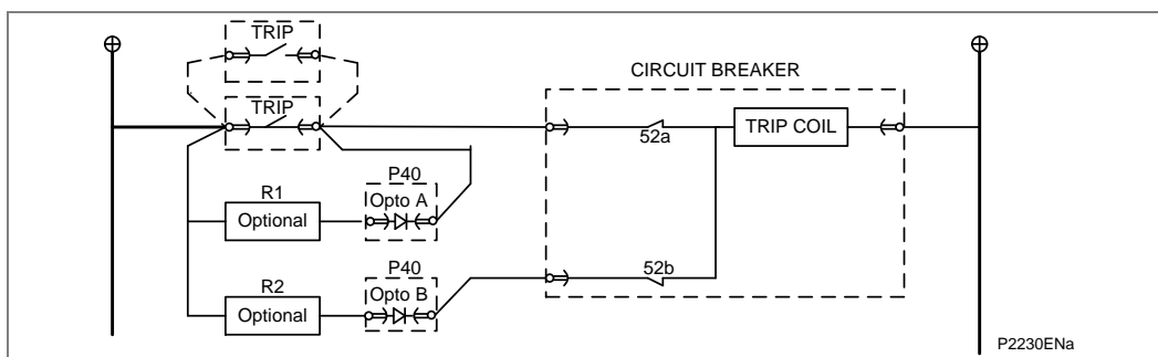
Figure 70 - TCS scheme 2
