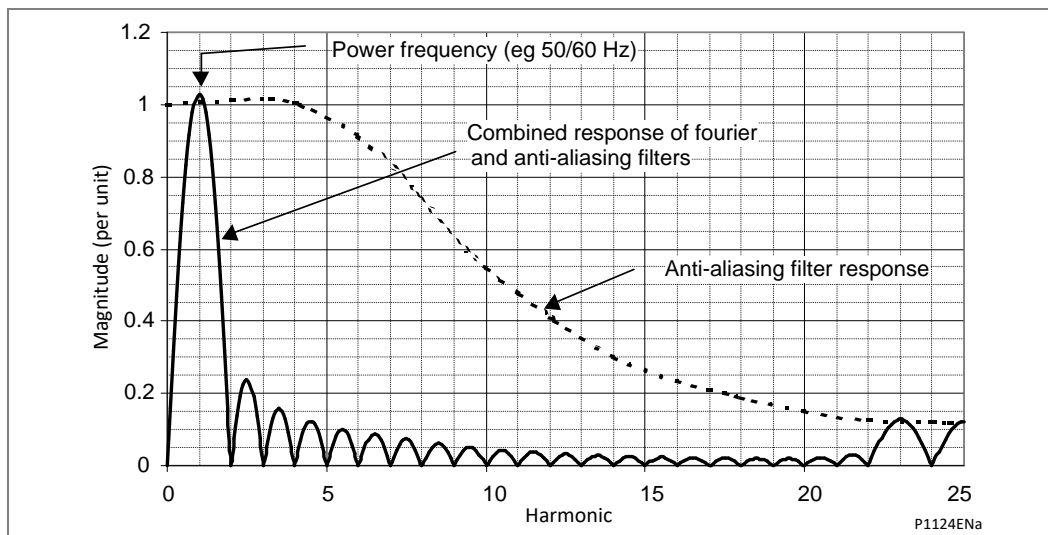
Figure 8 - Frequency response
