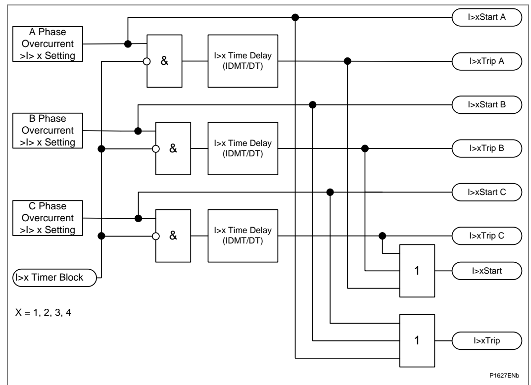
Figure 21 - Non-directional overcurrent logic diagram
